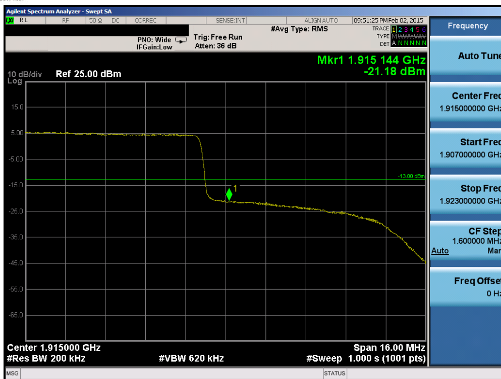
Plot 6-168. Upper Band Edge Plot (Band 25 – 20.0MHz QPSK – RB Size 100)
