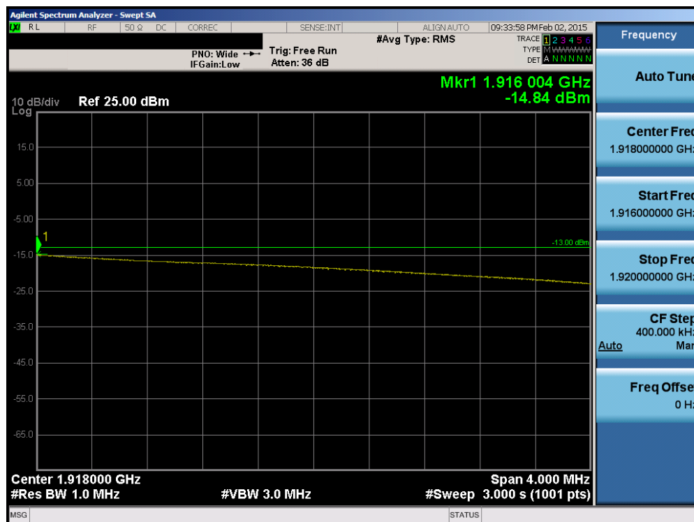
Plot 6-161. Upper Extended Band Edge Plot (Band 25 – 10.0MHz QPSK – RB Size 50)
