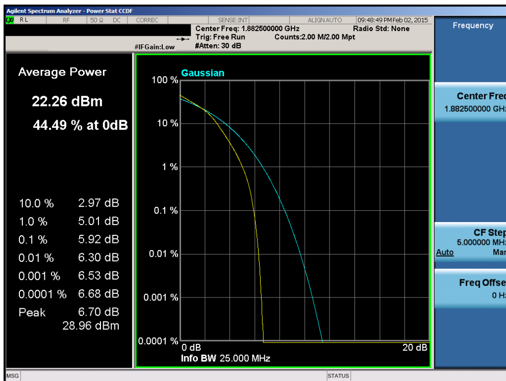
Plot 6-181. PAR Plot (Band 25 – 20.0MHz 16-QAM – RB Size 100)
