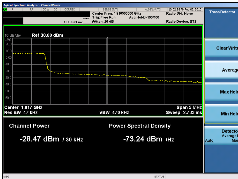
Plot 6-153. Upper Extended Band Edge Plot (Band 25 – 3.0MHz QPSK – RB Size 15)
