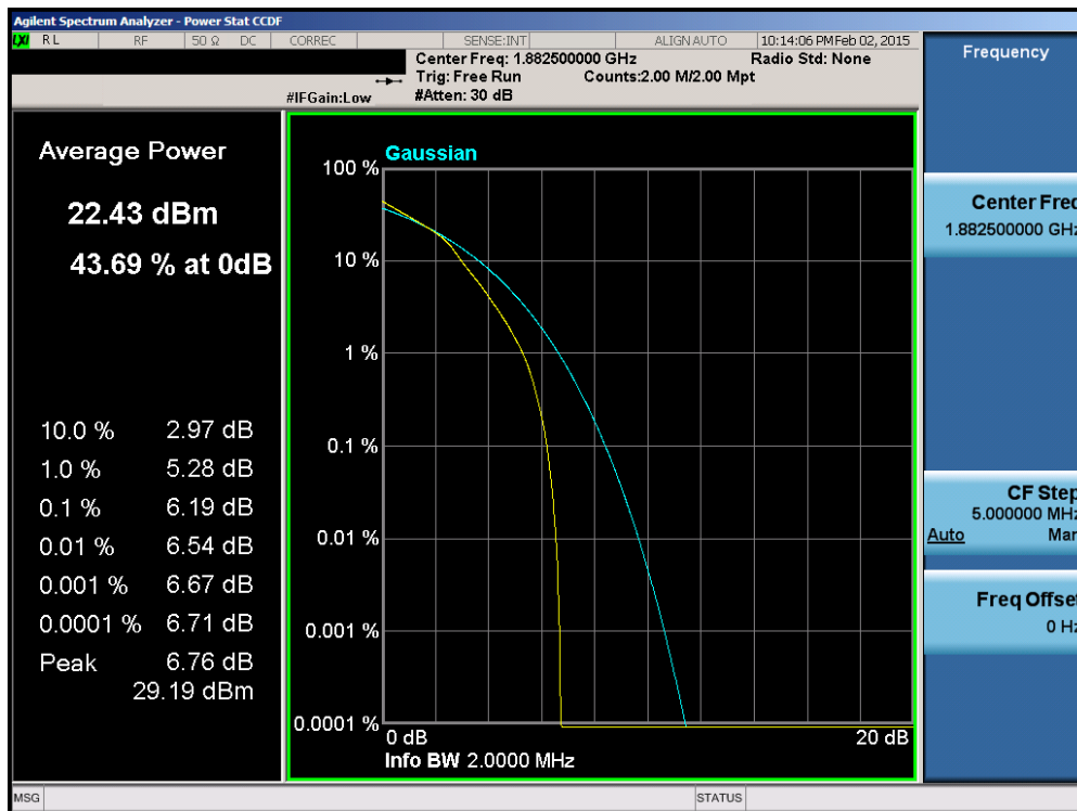
Plot 6-171. PAR Plot (Band 25 – 1.4MHz 16-QAM – RB Size 6)
