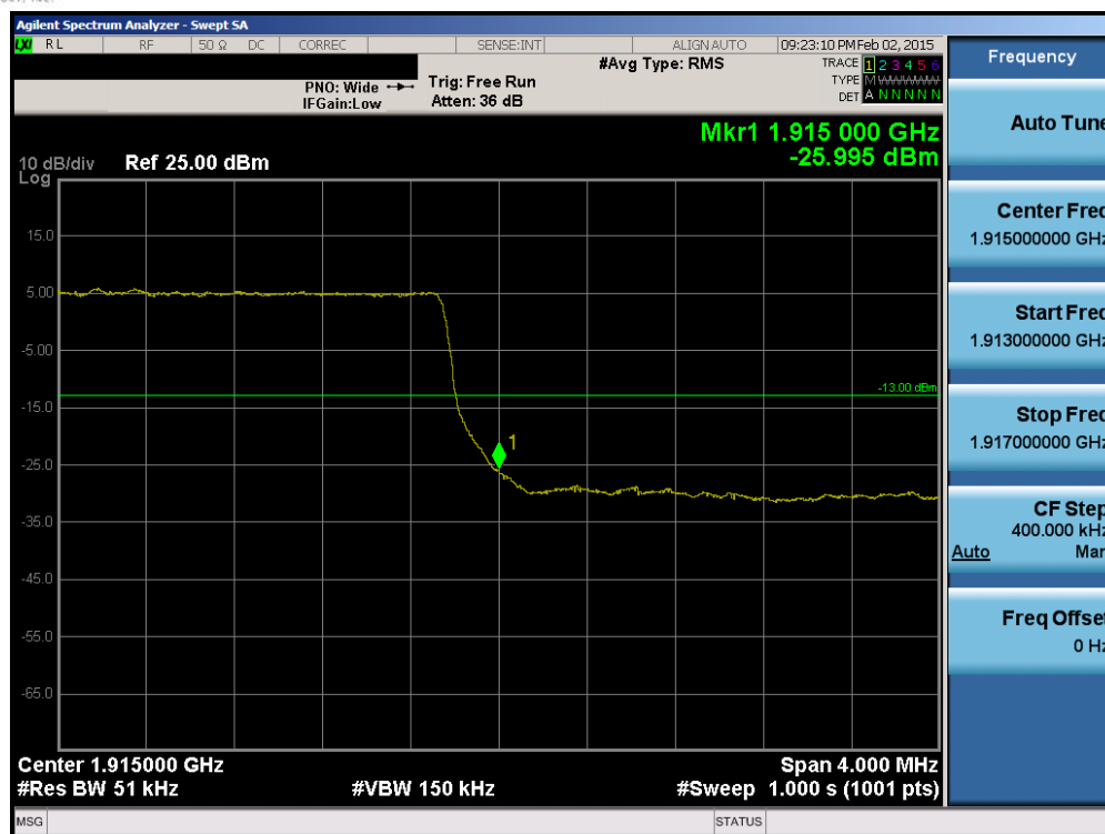
Plot 6-156. Upper Band Edge Plot (Band 25 – 5.0MHz QPSK – RB Size 25)
