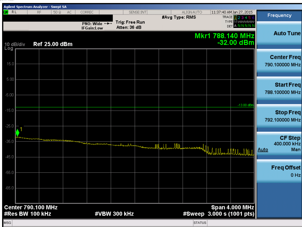
Plot 6-102. Upper Extended Band Edge Plot (Band 13 – 5.0MHz QPSK – RB Size 25)
