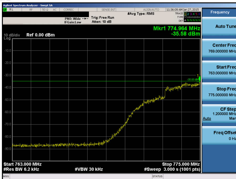
Plot 6-100. Lower Emission Mask Plot (Band 13 – 5.0MHz QPSK – RB Size 25)
