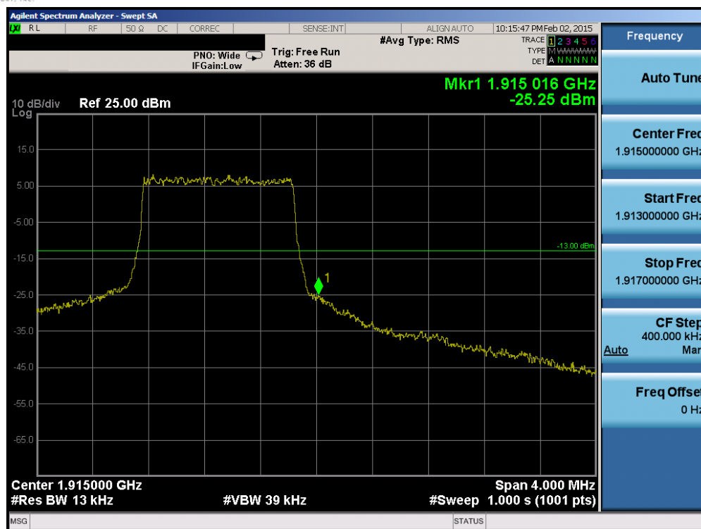
Plot 6-148. Upper Band Edge Plot (Band 25 – 1.4MHz QPSK – RB Size 6)
