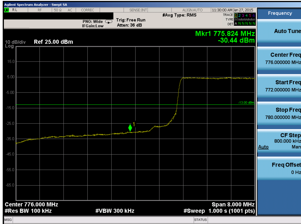
Plot 6-104. Lower Band Edge Plot (Band 13 – 10.0MHz QPSK – RB Size 50)
