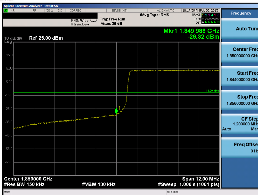
Plot 6-162. Lower Band Edge Plot (Band 25 – 15.0MHz QPSK – RB Size 75)
