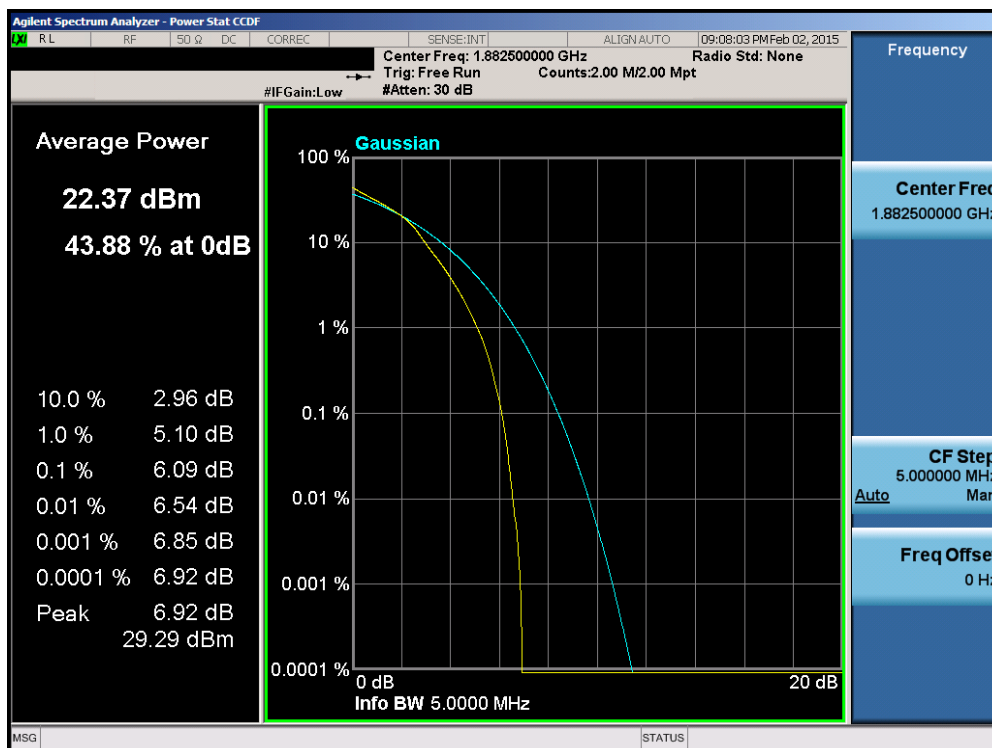
Plot 6-175. PAR Plot (Band 25 – 5.0MHz 16-QAM – RB Size 25)
