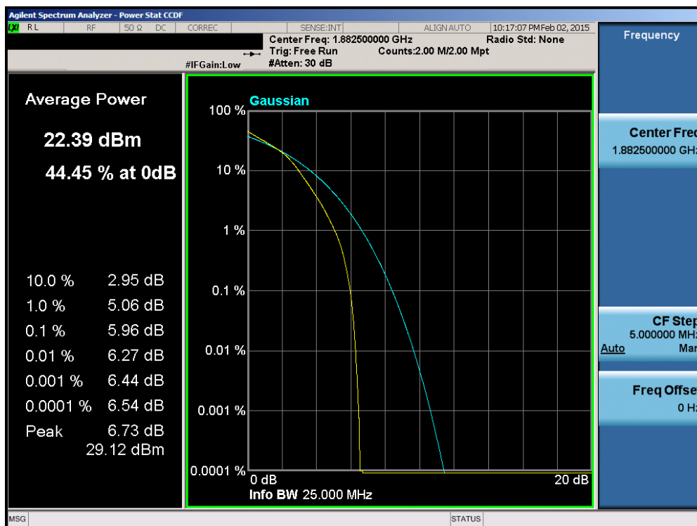
Plot 6-179. PAR Plot (Band 25 – 15.0MHz 16-QAM – RB Size 75)
