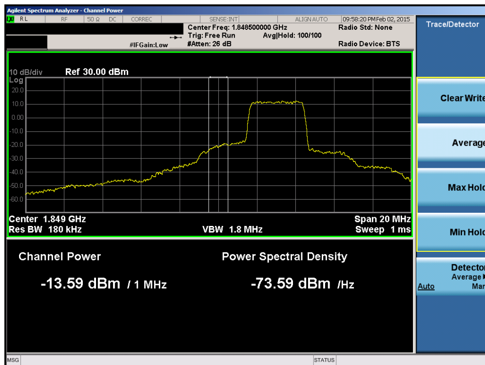
Plot 6-151. Lower Extended Band Edge Plot (Band 25 – 3.0MHz QPSK – RB Size 15)
