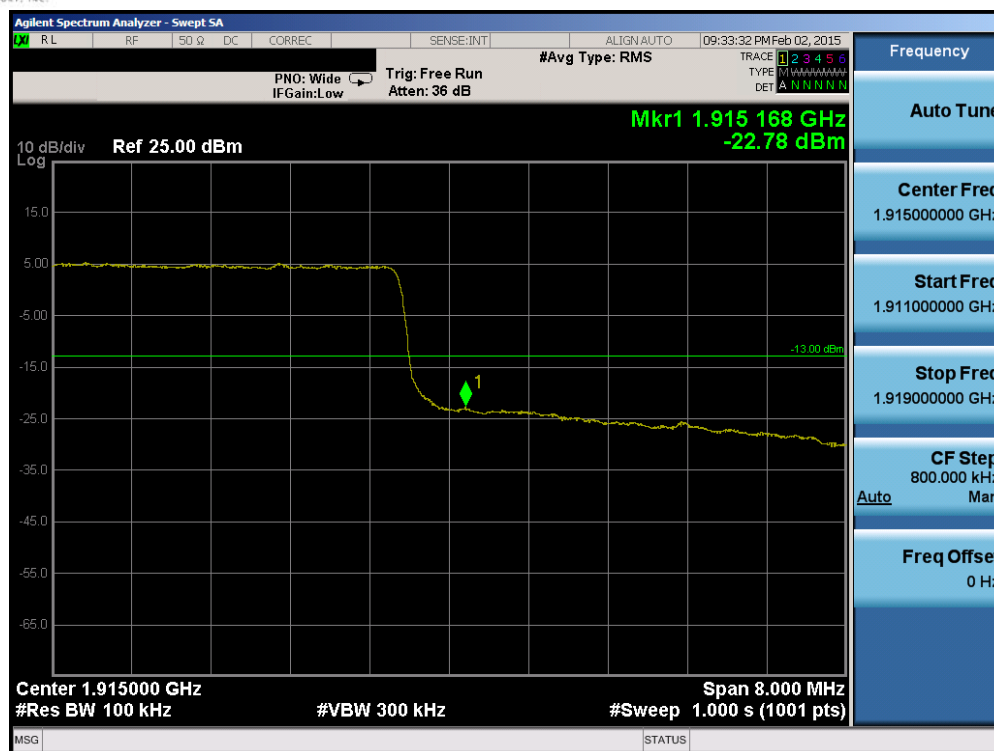
Plot 6-160. Upper Band Edge Plot (Band 25 – 10.0MHz QPSK – RB Size 50)
