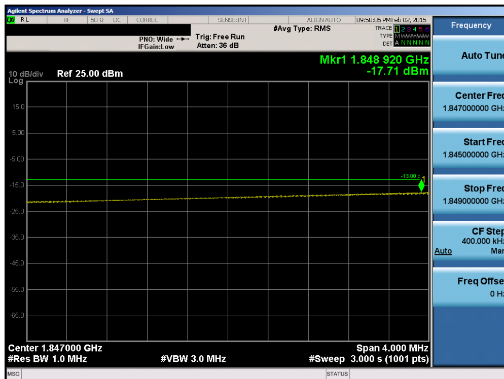
Plot 6-167. Lower Extended Band Edge Plot (Band 25 – 20.0MHz QPSK – RB Size 100)
