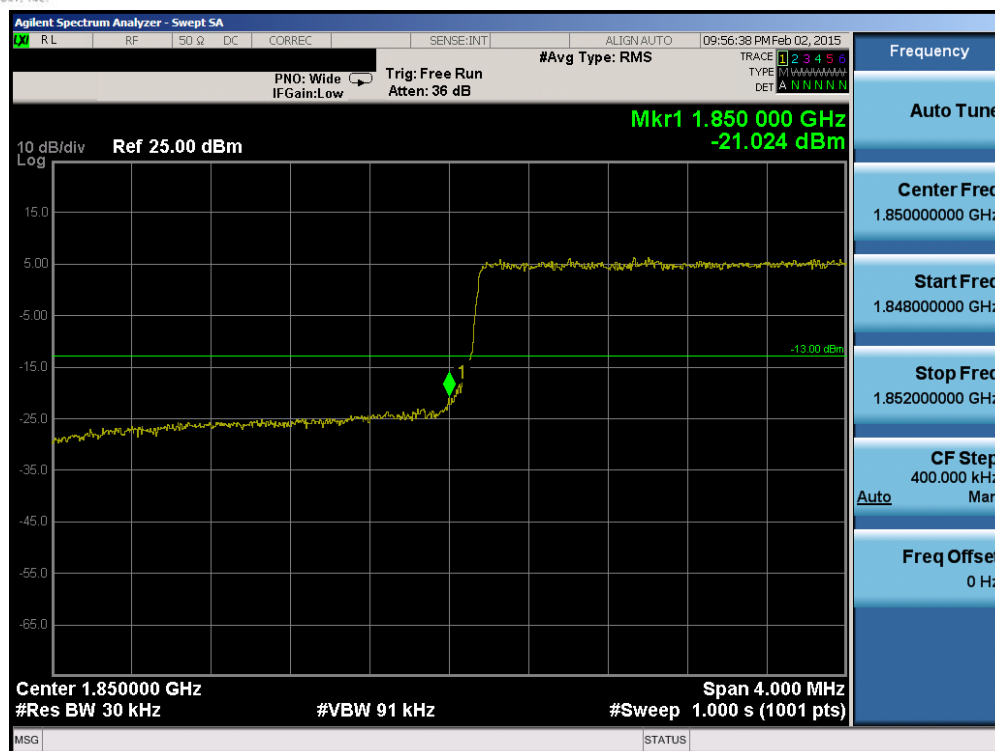
Plot 6-150. Lower Band Edge Plot (Band 25 – 3.0MHz QPSK – RB Size 15)
