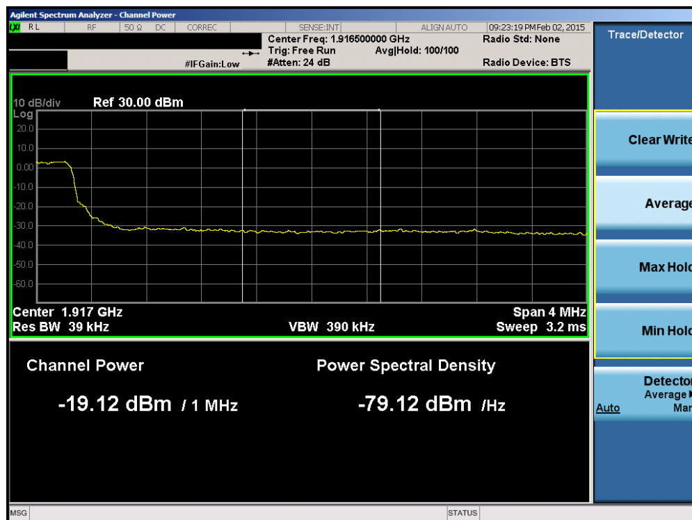
Plot 6-157. Upper Extended Band Edge Plot (Band 25 – 5.0MHz QPSK – RB Size 25)
