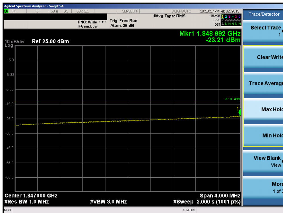
Plot 6-163. Lower Extended Band Edge Plot (Band 25 – 15.0MHz QPSK – RB Size 75)
