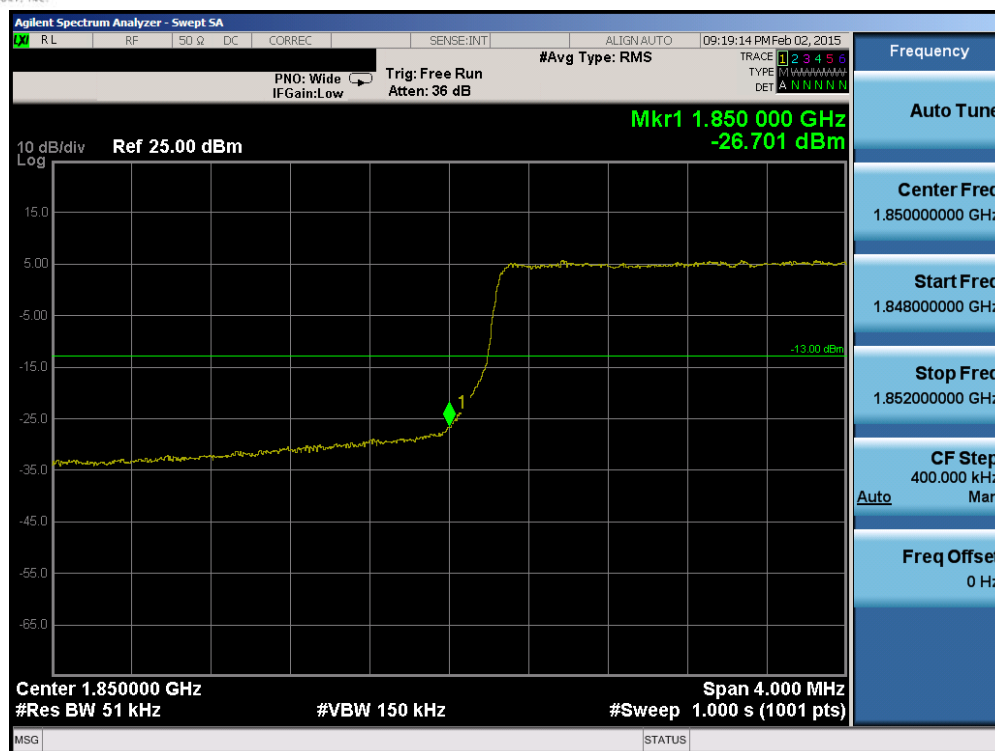
Plot 6-154. Lower Band Edge Plot (Band 25 – 5.0MHz QPSK – RB Size 25)
