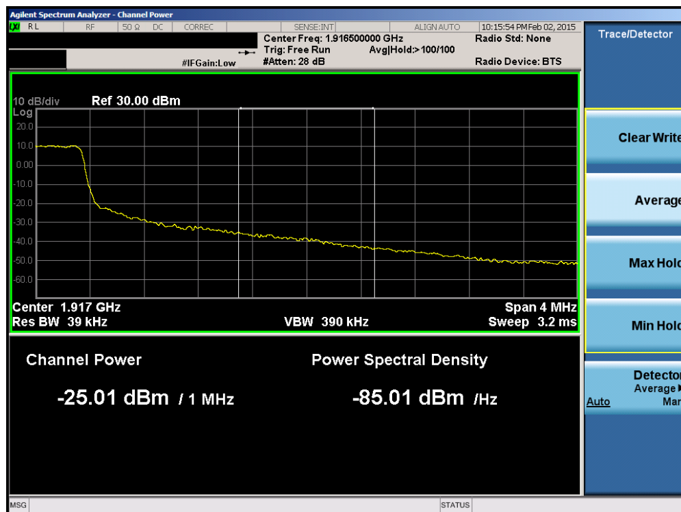
Plot 6-149. Upper Extended Band Edge Plot (Band 25 – 1.4MHz QPSK – RB Size 6)
