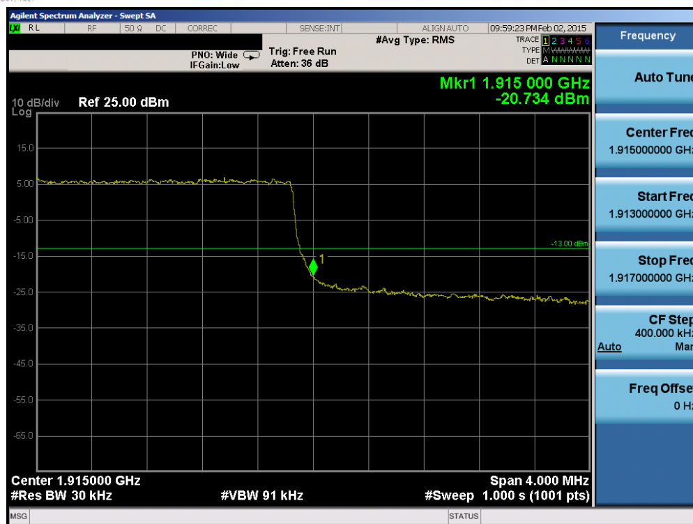
Plot 6-152. Upper Band Edge Plot (Band 25 – 3.0MHz QPSK – RB Size 15)
