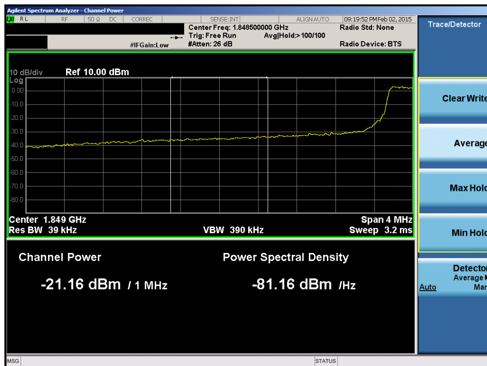
Plot 6-155. Lower Extended Band Edge Plot (Band 25 – 5.0MHz QPSK – RB Size 25)
