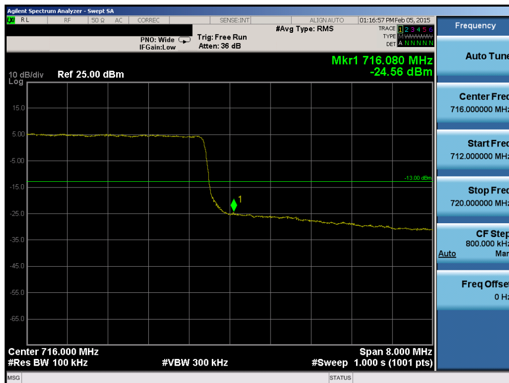
Plot 6-97. Upper Band Edge Plot (Band 12 – 10.0MHz QPSK – RB Size 50)
