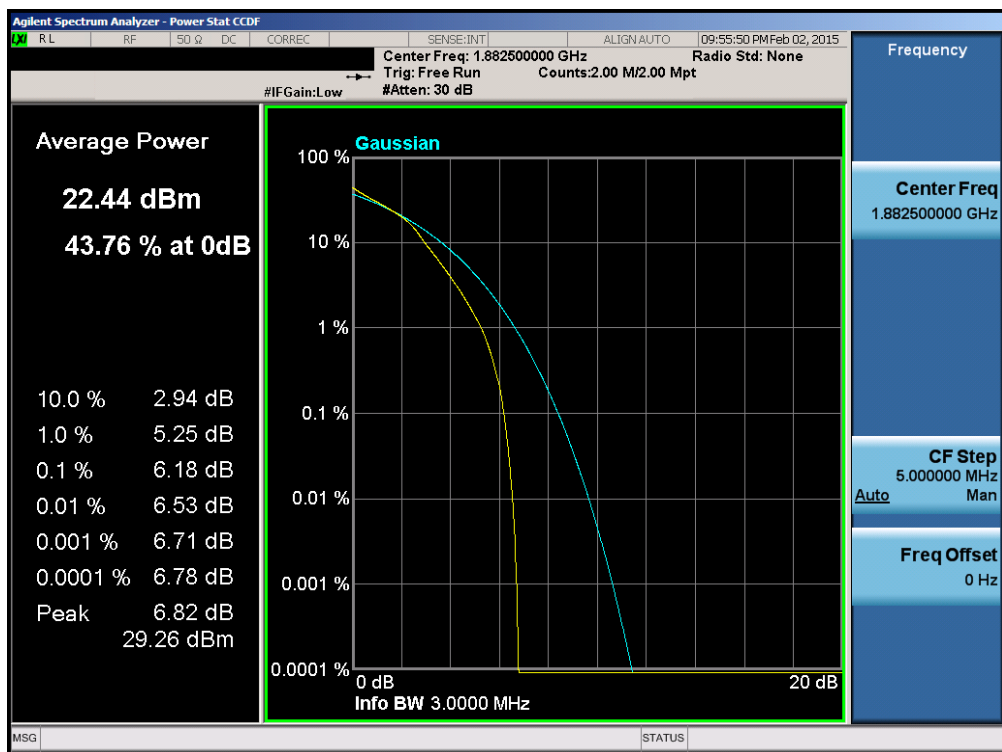
Plot 6-173. PAR Plot (Band 25 – 3.0MHz 16-QAM – RB Size 15)
