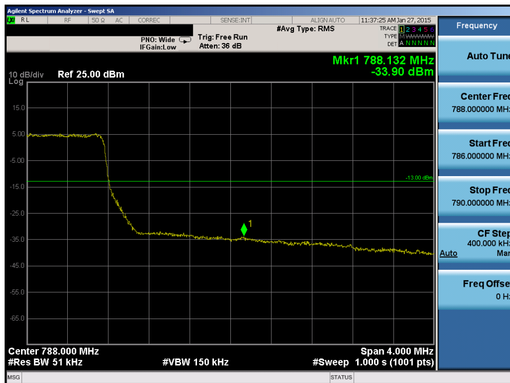
Plot 6-101. Upper Band Edge Plot (Band 13 – 5.0MHz QPSK – RB Size 25)
