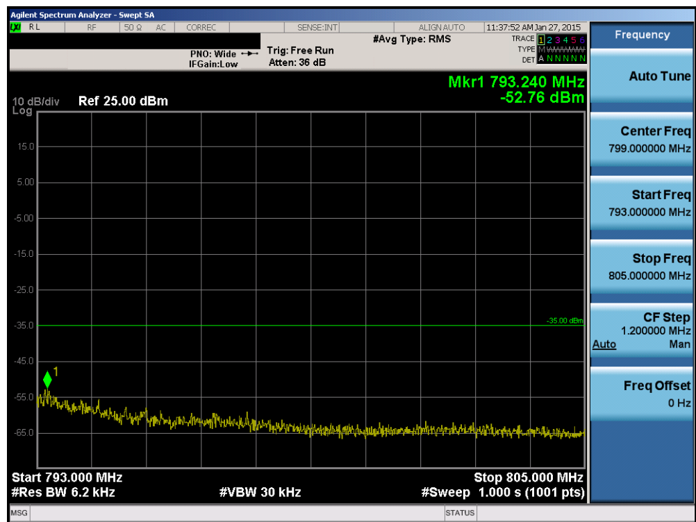
Plot 6-103. Upper Emission Mask Plot (Band 13 – 5.0MHz QPSK – RB Size 25)
