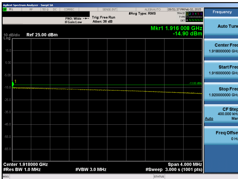
Plot 6-169. Upper Extended Band Edge Plot (Band 25 – 20.0MHz QPSK – RB Size 100)
