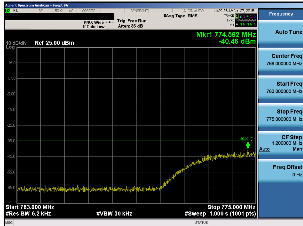
Plot 6-105. Lower Emission Mask Plot (Band 13 – 10.0MHz QPSK – RB Size 50)
