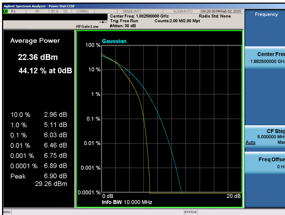
Plot 6-177. PAR Plot (Band 25 – 10.0MHz 16-QAM – RB Size 50)
