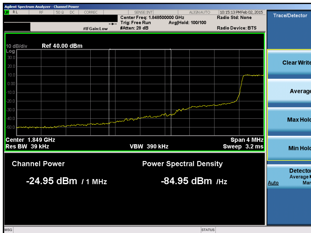
Plot 6-147. Lower Extended Band Edge Plot (Band 25 – 1.4MHz QPSK – RB Size 6)
