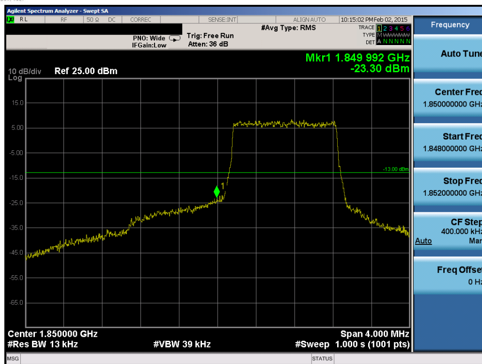
Plot 6-146. Lower Band Edge Plot (Band 25 – 1.4MHz QPSK – RB Size 6)
