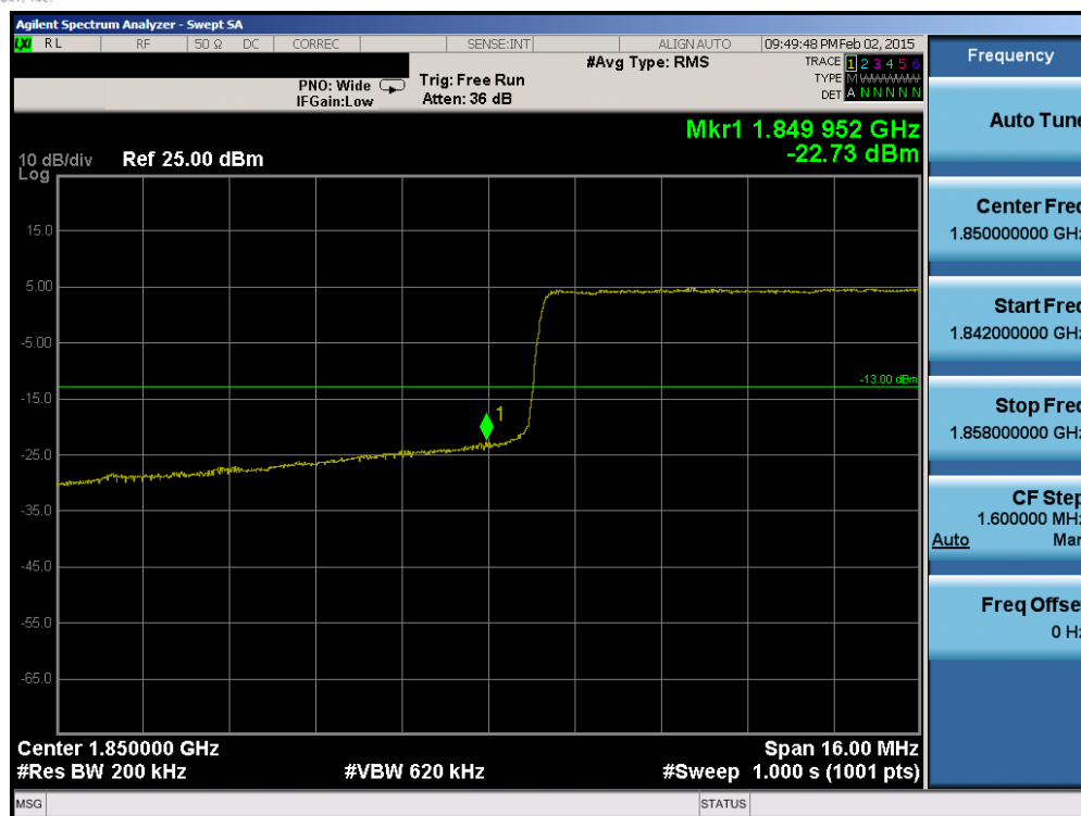
Plot 6-166. Lower Band Edge Plot (Band 25 – 20.0MHz QPSK – RB Size 100)
