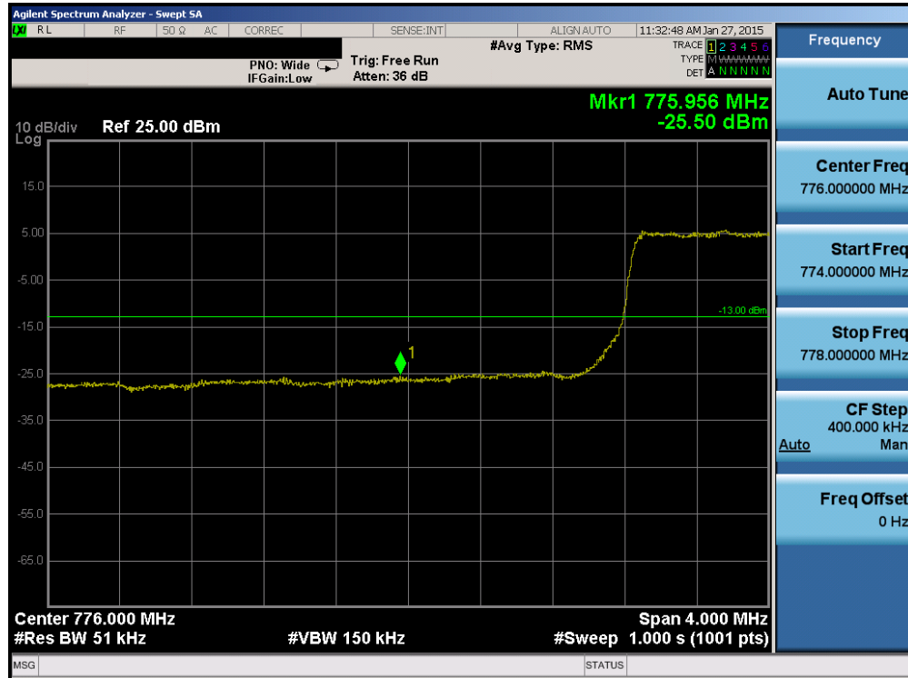
Plot 6-98. Lower Band Edge Plot (Band 13 – 5.0MHz QPSK – RB Size 25)
