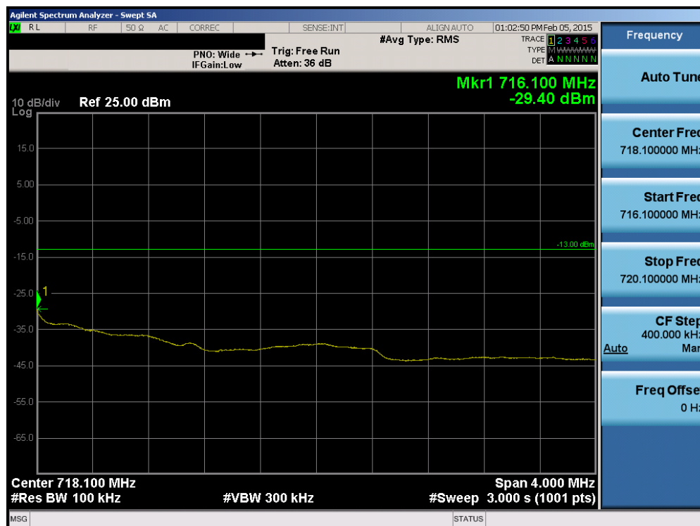
Plot 6-91. Upper Extended Band Edge Plot (Band 12 – 3.0MHz QPSK – RB Size 15)
