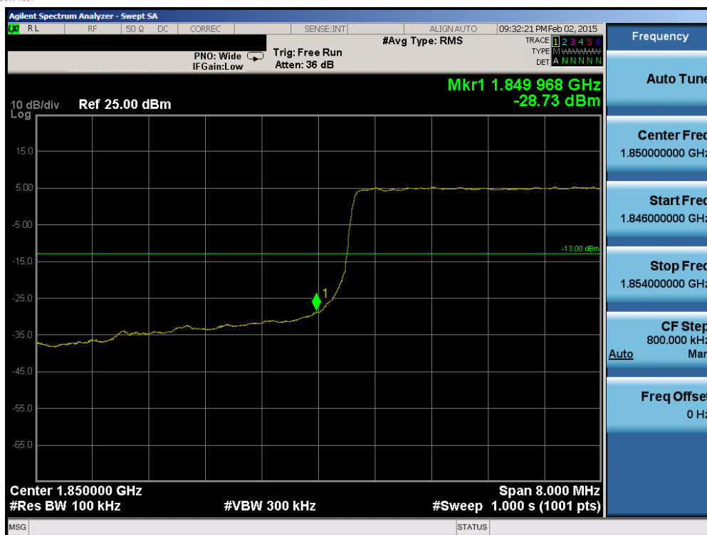
Plot 6-158. Lower Band Edge Plot (Band 25 – 10.0MHz QPSK – RB Size 50)
