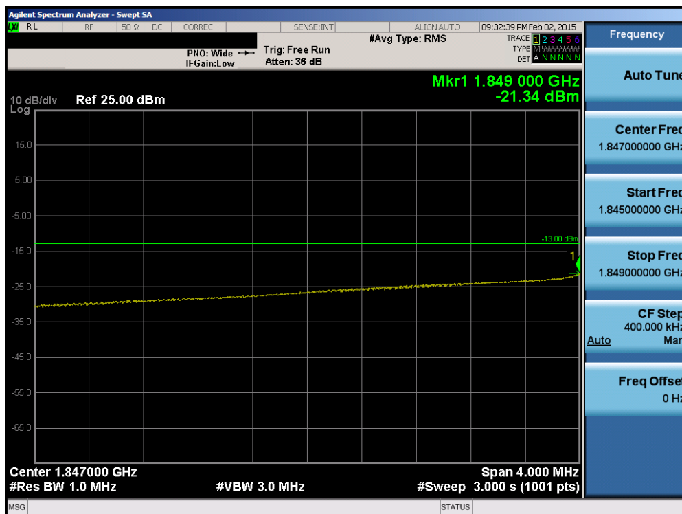
Plot 6-159. Lower Extended Band Edge Plot (Band 25 – 10.0MHz QPSK – RB Size 50)
