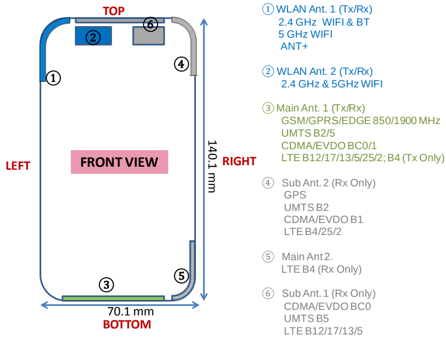
Figure F-1 DUT Antenna Locations
