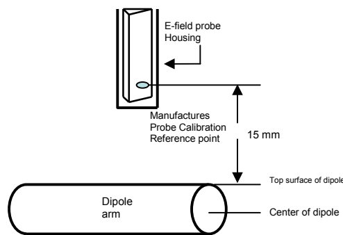
Figure 6-1 Separation Distance from Dipole to Field Probe
