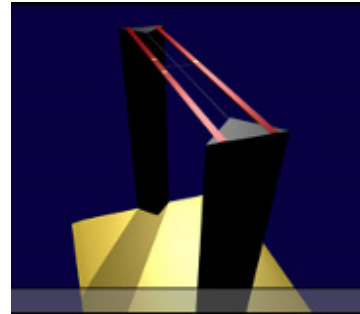
Figure 5-3 HAC Phantom
