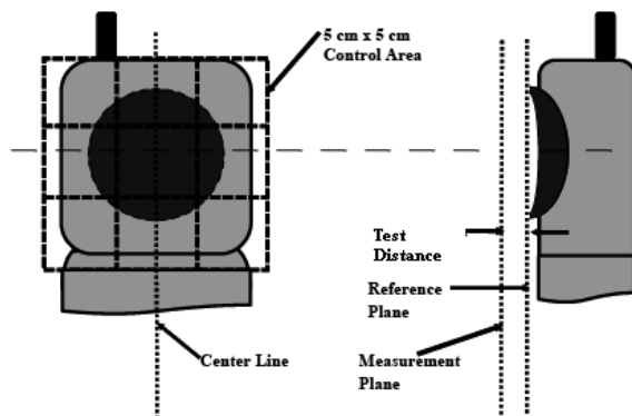
Figure 5-2 E-Field Emissions Test Setup Diagram (See Test Photographs for actual WD scan grid overlay)
