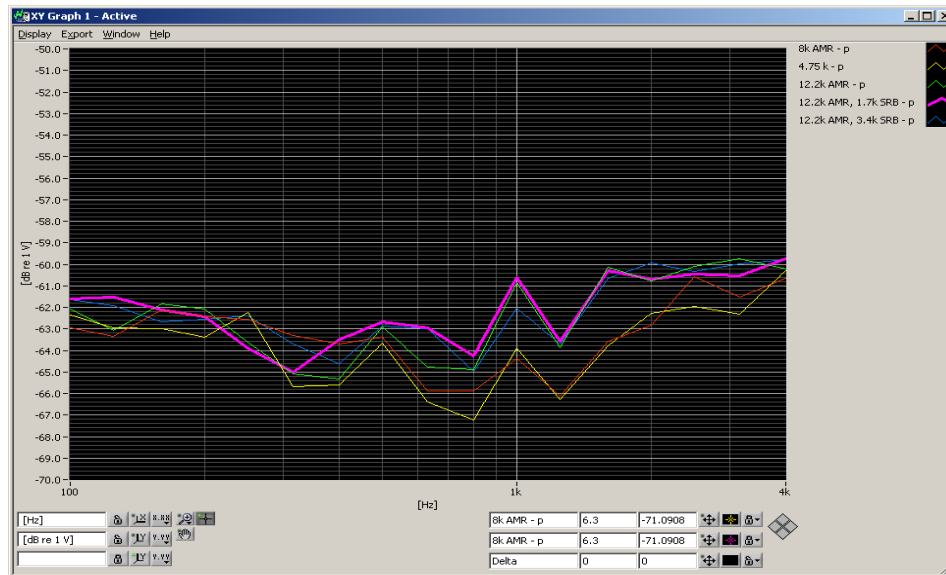
Figure 5-1 UMTS Audio Band Magnetic Noise
