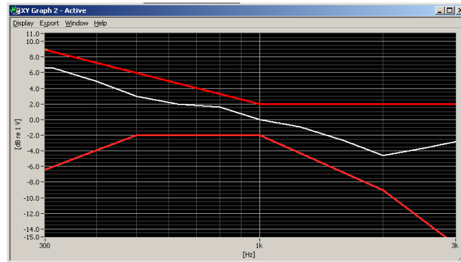
Figure 6-1 Axial Frequency Response
