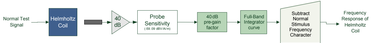
Figure 4-6 Frequency Response Validation
