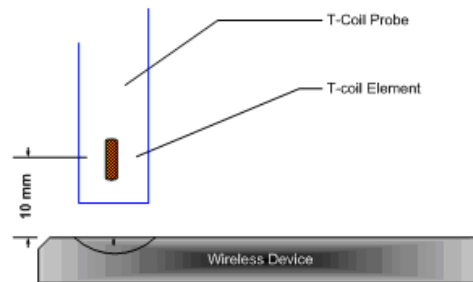
Figure 4-10 Measurement Distance
