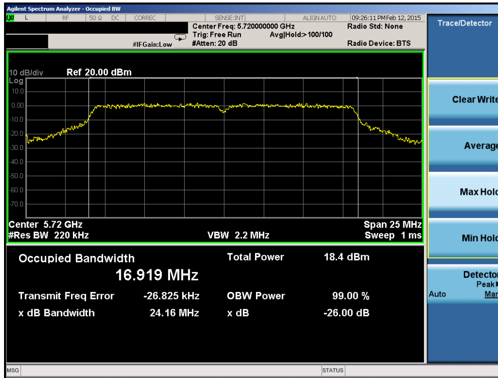
Plot 6-50. 26dB Bandwidth Plot (20MHz BW 802.11a (UNII Band 2C) – Ch. 144)
