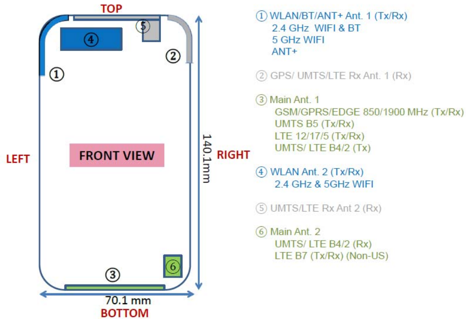
Figure F-1 DUT Antenna Locations
