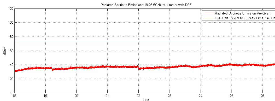
Plot 6-25. Radiated Spurious Plot above 18GHz (Pol. V)
