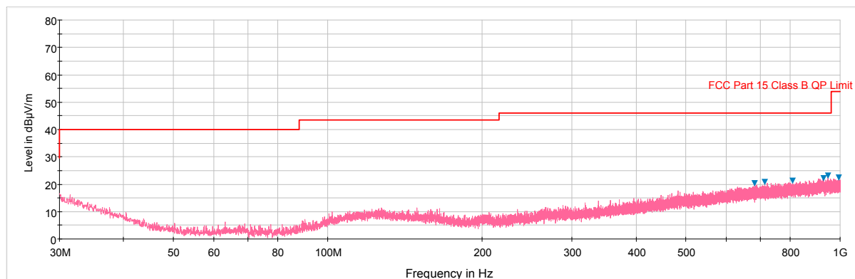
Plot 6-29. Radiated Spurious Plot below 1GHz (Pol. V)
