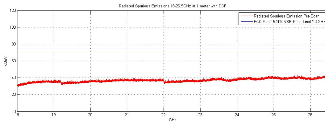
Plot 6-24. Radiated Spurious Plot above 18GHz (Pol. H)
