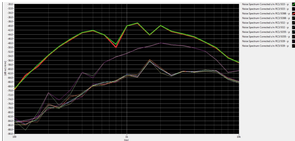
Figure 5-1 CDMA Audio Band Magnetic Noise
