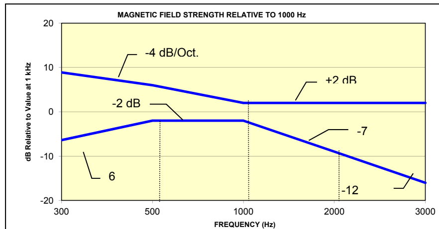
Figure 3-2 Magnetic Field frequency response for wireless devices with an axial field that exceeds -15 dB(A/m) at 1 kHz
