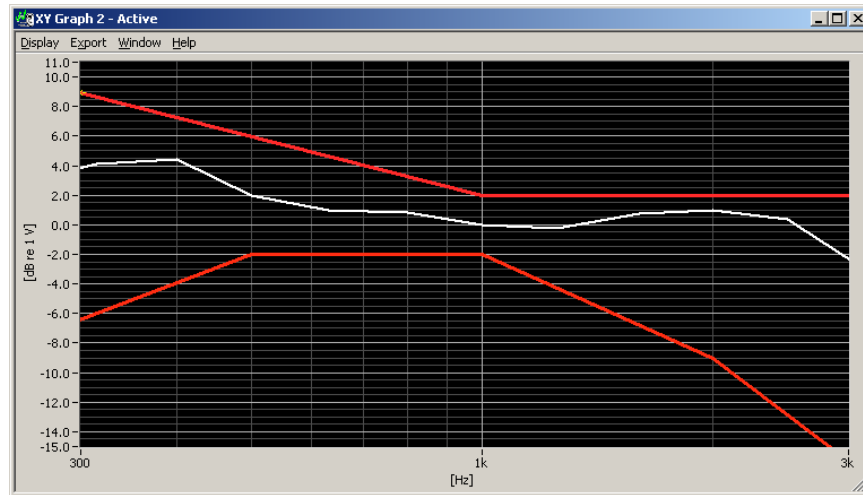
Figure 6-1 Axial Frequency Response
