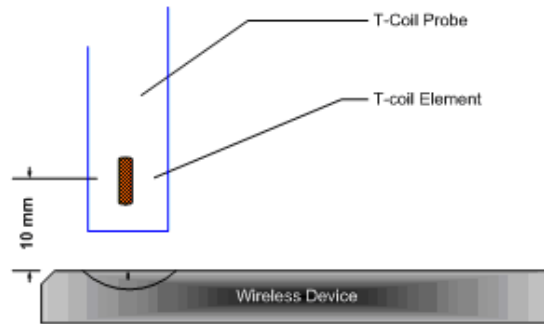
Figure 4-10 Measurement Distance
