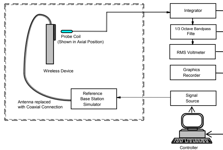
Figure 4-13 Audio Magnetic Field Test Setup
