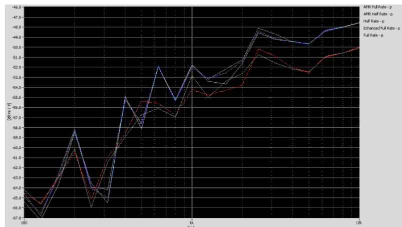
Figure 4-11 Vocoder Analysis for ABM Noise for GSM
