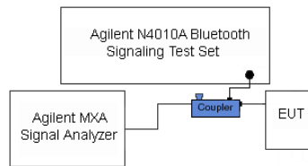
Figure 6-2. Test Instrument & Measurement Setup
