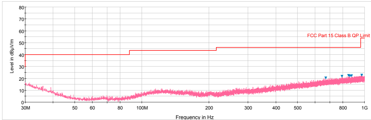
Plot 6-236. Radiated Spurious Plot below 1GHz (802.11a – U3, Ant. Pol. H)
