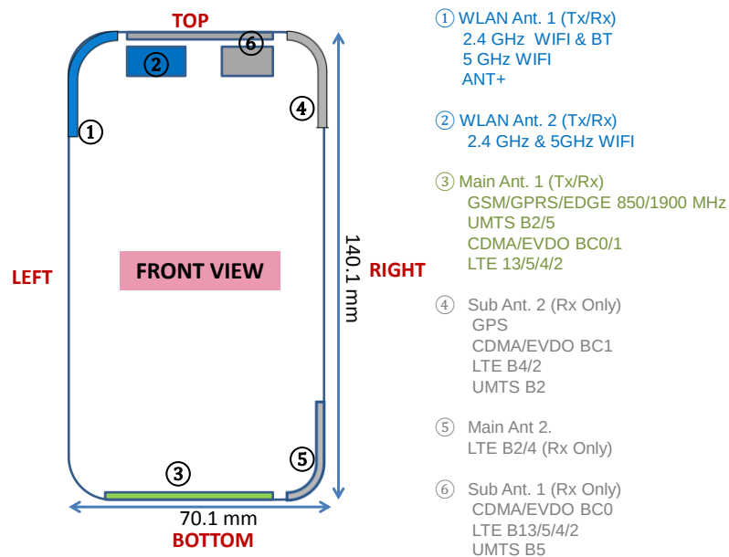
Figure E-1 DUT Antenna Locations
