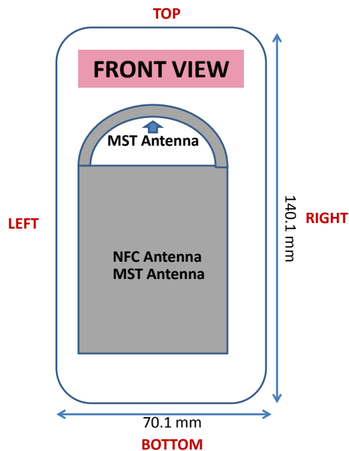
Figure E-2 NFC Antenna Location
