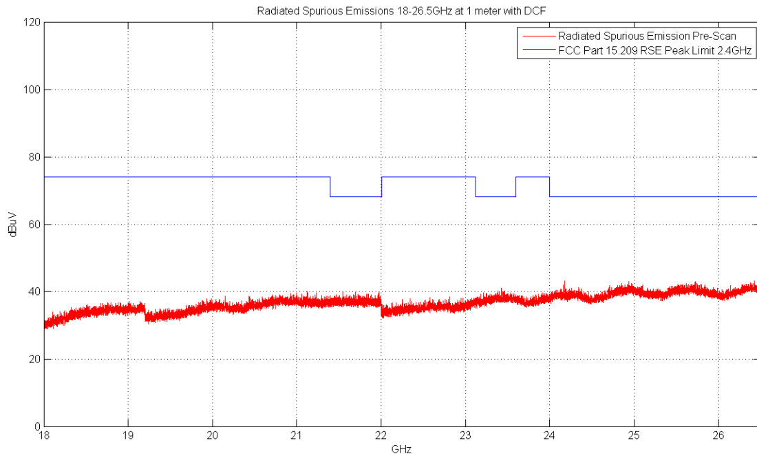
Plot 6-49. Radiated Spurious Plot above 18GHz (Pol. H)
