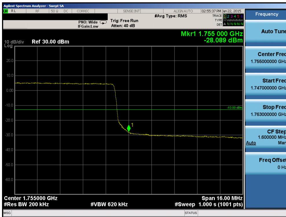
Plot 6-148. Upper Band Edge Plot (Band 4 – 20.0MHz QPSK – RB Size 100)
