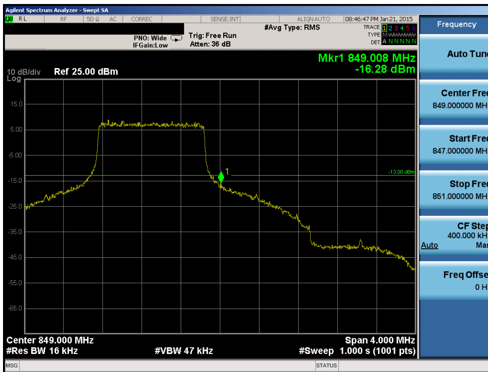
Plot 6-114. Upper Band Edge Plot (Band 5 - 1.4MHz QPSK - RB Size 6)
