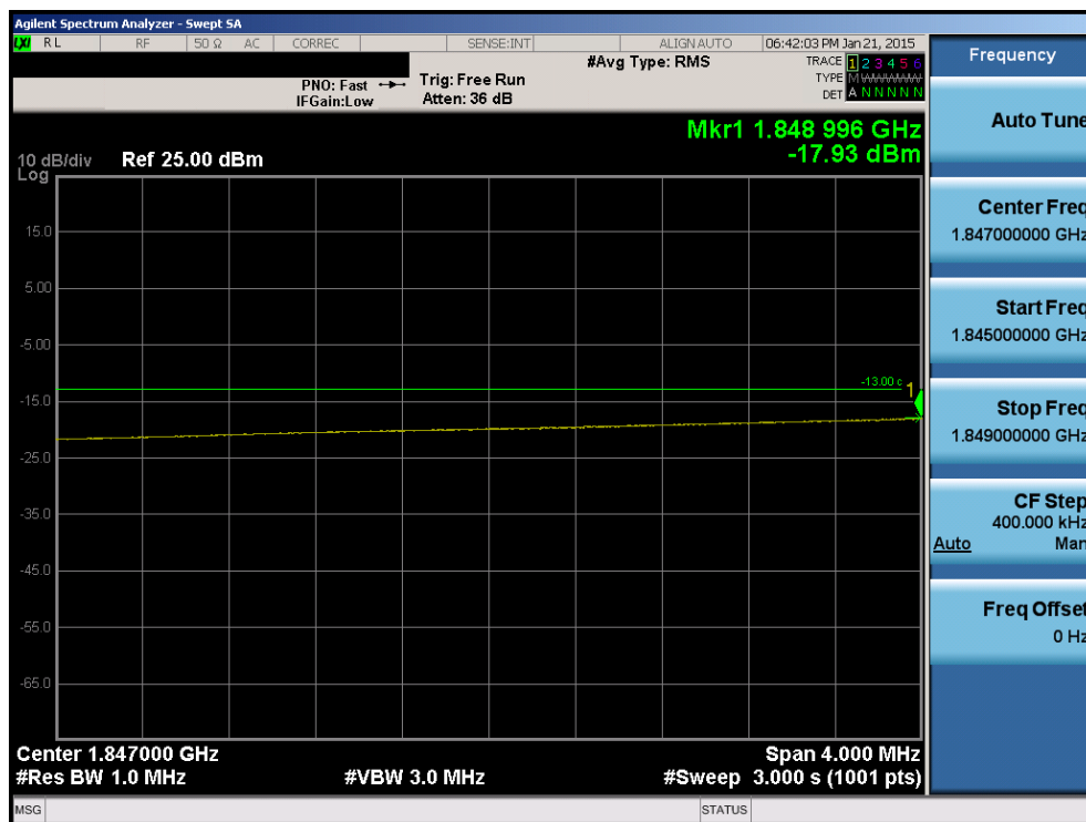
Plot 6-167. Lower Extended Band Edge Plot (Band 2 – 15.0MHz QPSK – RB Size 75)
