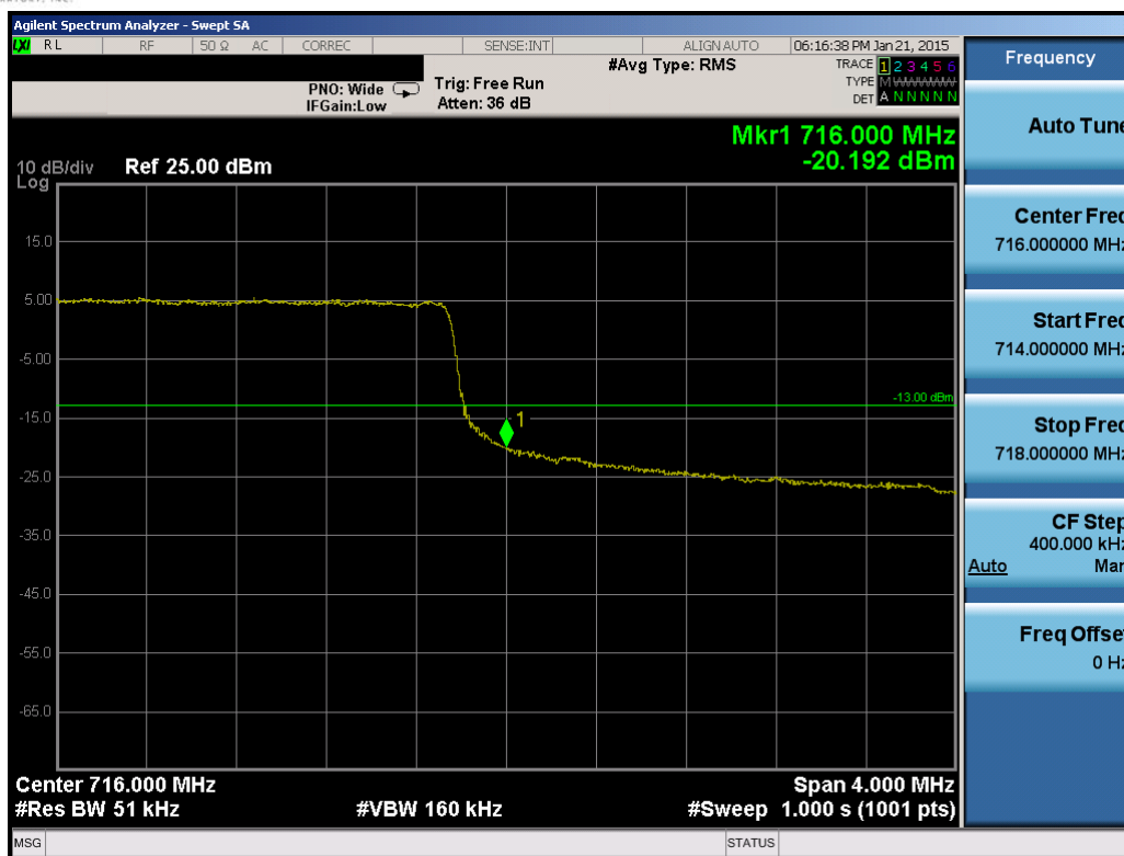
Plot 6-100. Upper Band Edge Plot (Band 12/17 – 5.0MHz QPSK – RB Size 25)
