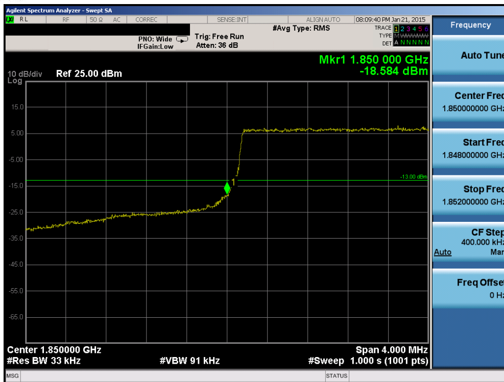
Plot 6-154. Lower Band Edge Plot (Band 2 – 3.0MHz QPSK – RB Size 15)
