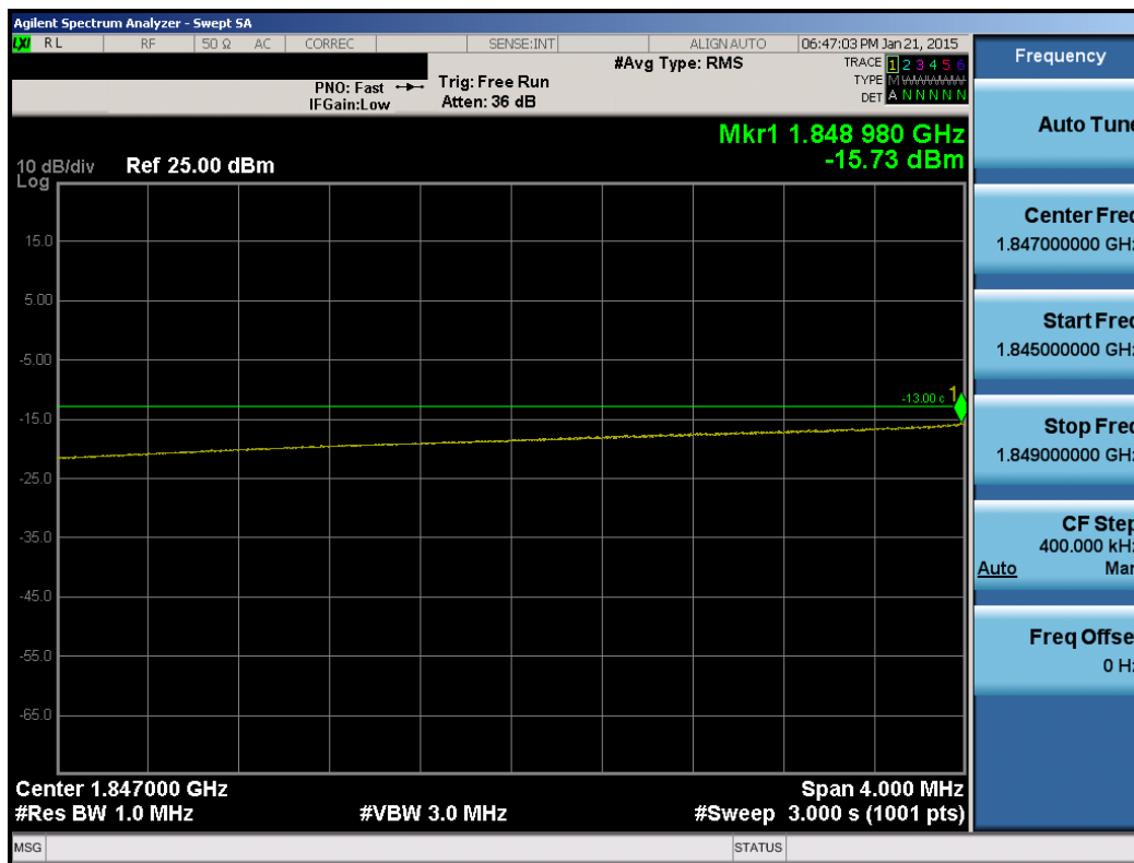
Plot 6-163. Lower Extended Band Edge Plot (Band 2 – 10.0MHz QPSK – RB Size 50)
