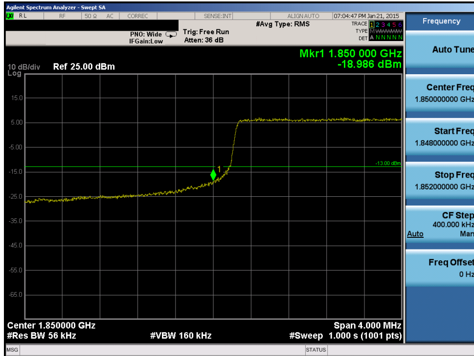
Plot 6-158. Lower Band Edge Plot (Band 2 – 5.0MHz QPSK – RB Size 25)
