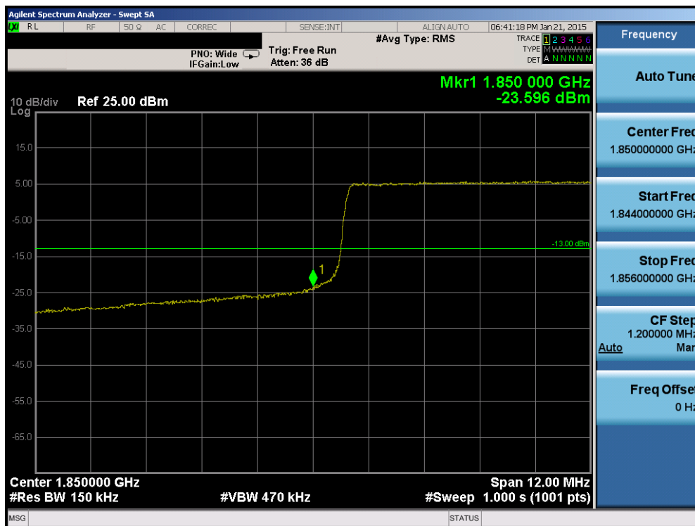
Plot 6-166. Lower Band Edge Plot (Band 2 – 15.0MHz QPSK – RB Size 75)
