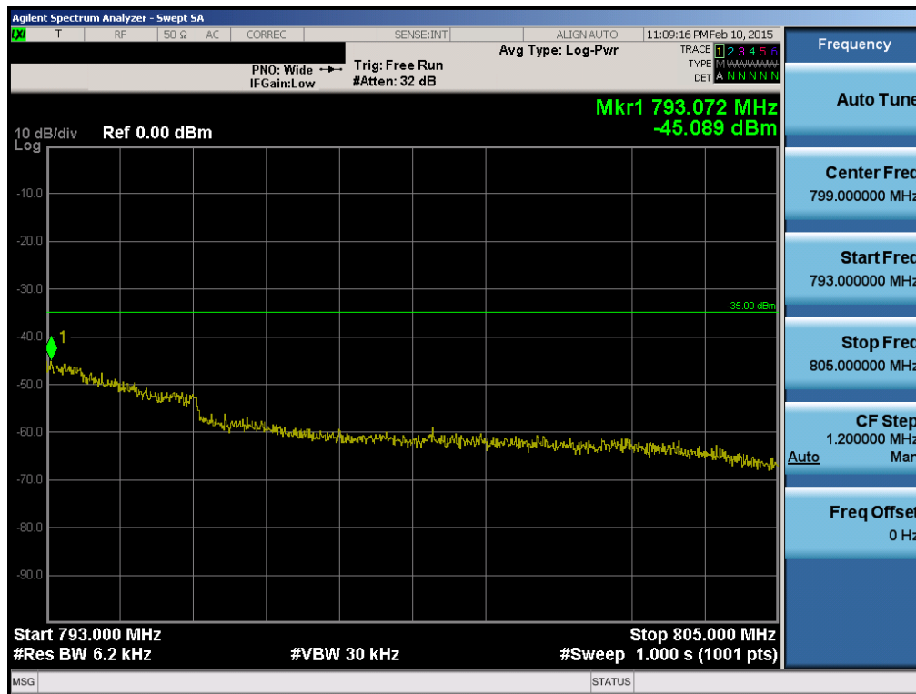
Plot 6-111. Upper Extended Band Edge Plot (Band 13 – 10.0MHz QPSK – RB Size 50)
