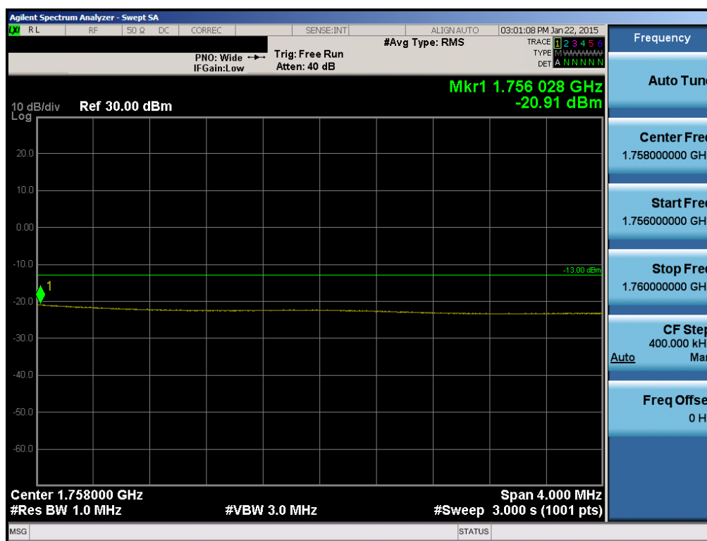
Plot 6-145. Upper Extended Band Edge Plot (Band 4 – 15.0MHz QPSK – RB Size 75)
