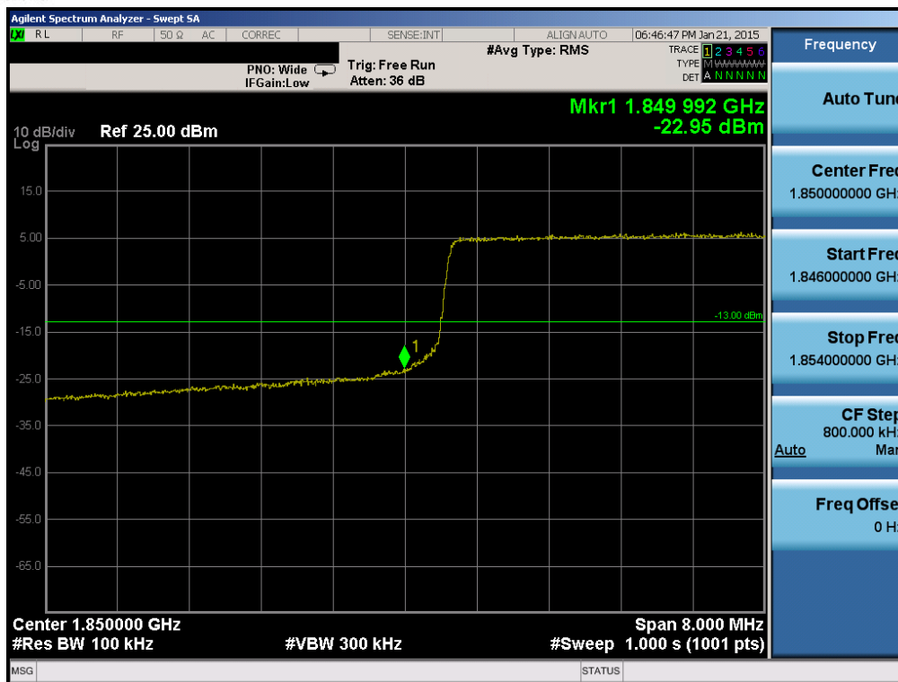
Plot 6-162. Lower Band Edge Plot (Band 2 – 10.0MHz QPSK – RB Size 50)
