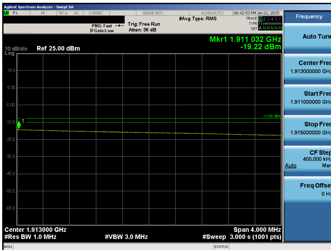
Plot 6-169. Upper Extended Band Edge Plot (Band 2 - 15.0MHz QPSK - RB Size 75)
