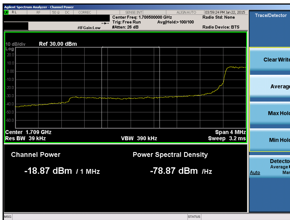
Plot 6-127. Lower Extended Band Edge Plot (Band 4 – 1.4MHz QPSK – RB Size 6)
