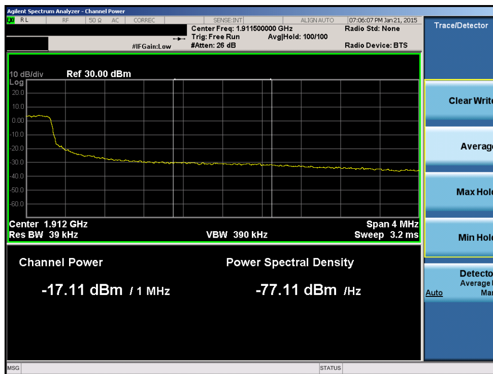
Plot 6-161. Upper Extended Band Edge Plot (Band 2 – 5.0MHz QPSK – RB Size 25)
