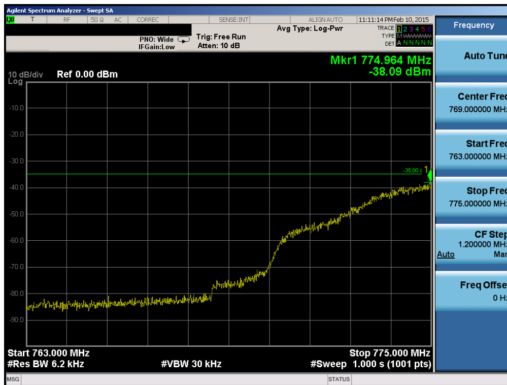
Plot 6-109. Lower Extended Band Edge Plot (Band 13 - 10.0MHz QPSK - RB Size 50)
