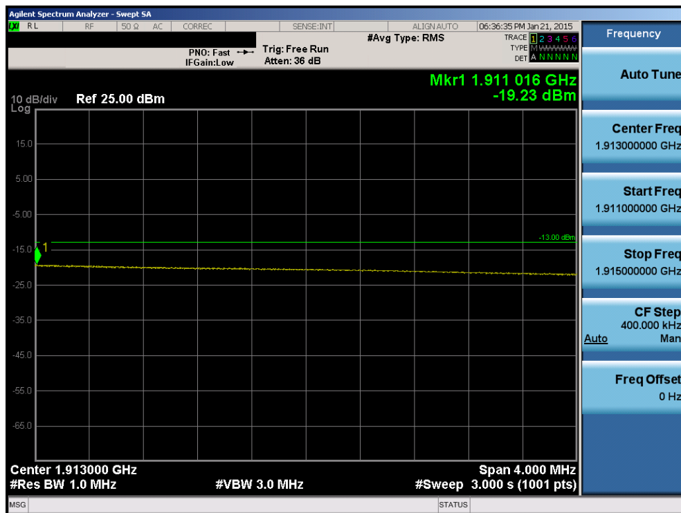
Plot 6-173. Upper Extended Band Edge Plot (Band 2 – 20.0MHz QPSK – RB Size 100)
