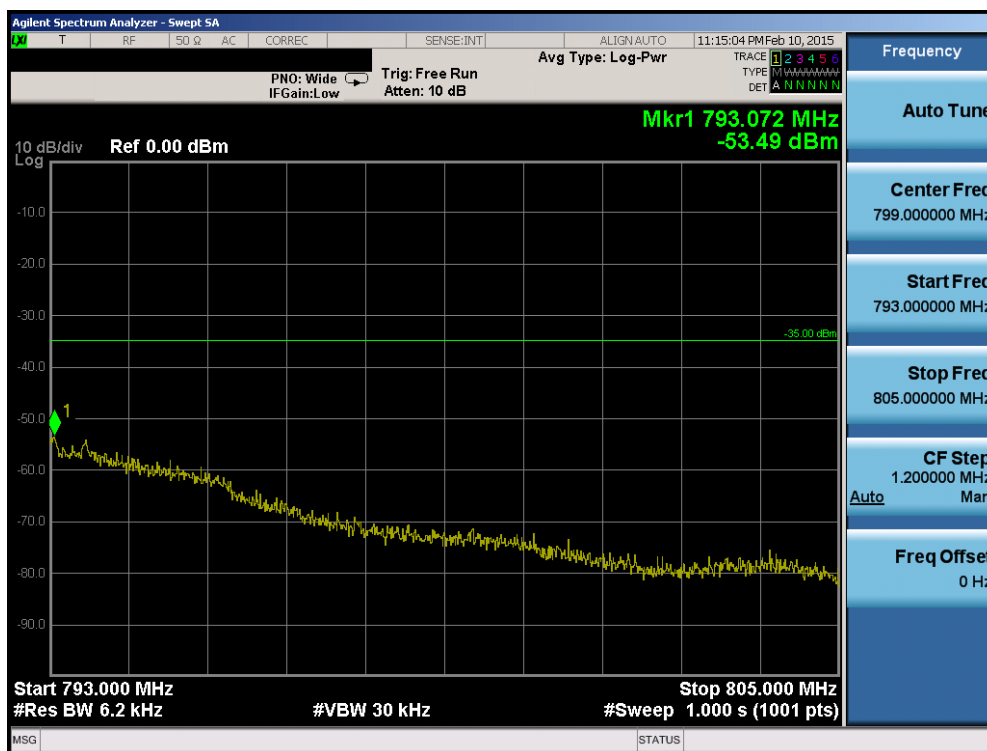
Plot 6-107. Upper Extended Band Edge Plot (Band 13 – 5.0MHz QPSK – RB Size 25)
