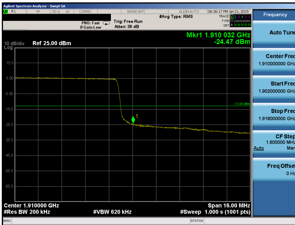
Plot 6-172. Upper Band Edge Plot (Band 2 – 20.0MHz QPSK – RB Size 100)
