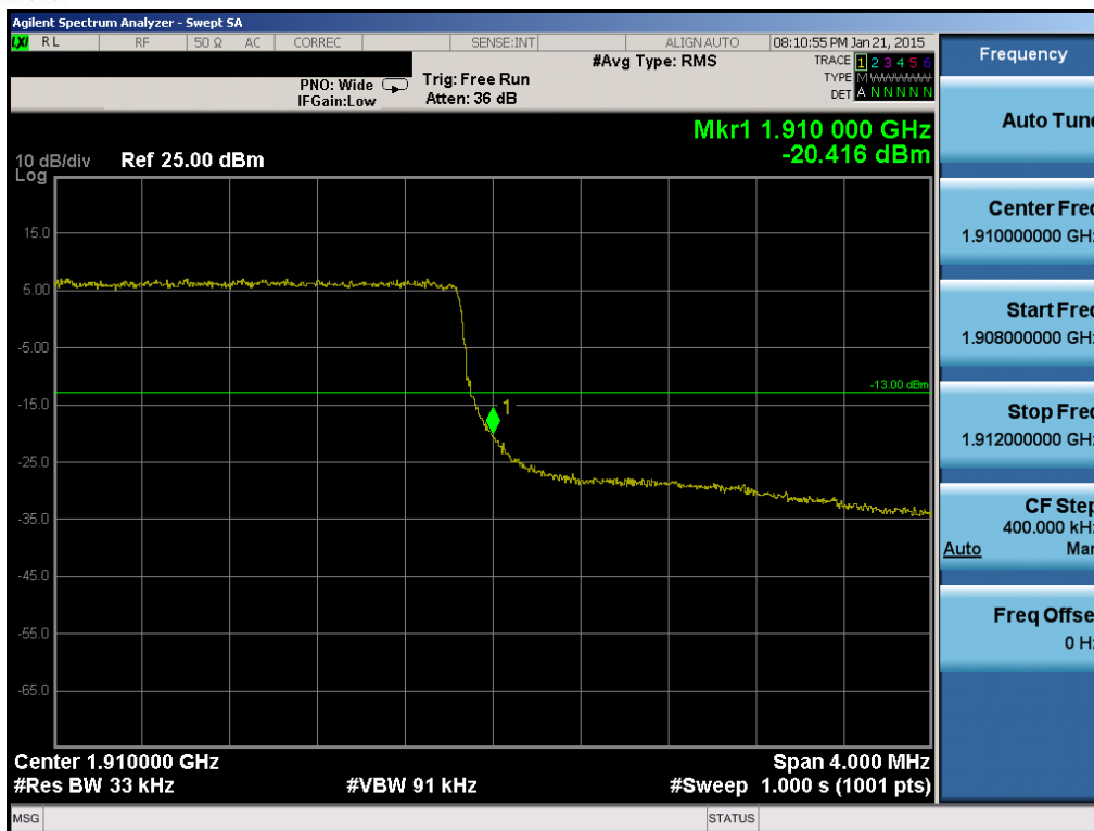
Plot 6-156. Upper Band Edge Plot (Band 2 – 3.0MHz QPSK – RB Size 15)
