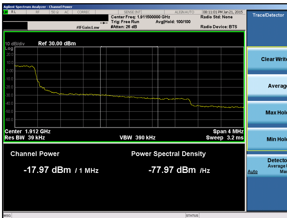
Plot 6-157. Upper Extended Band Edge Plot (Band 2 – 3.0MHz QPSK – RB Size 15)
