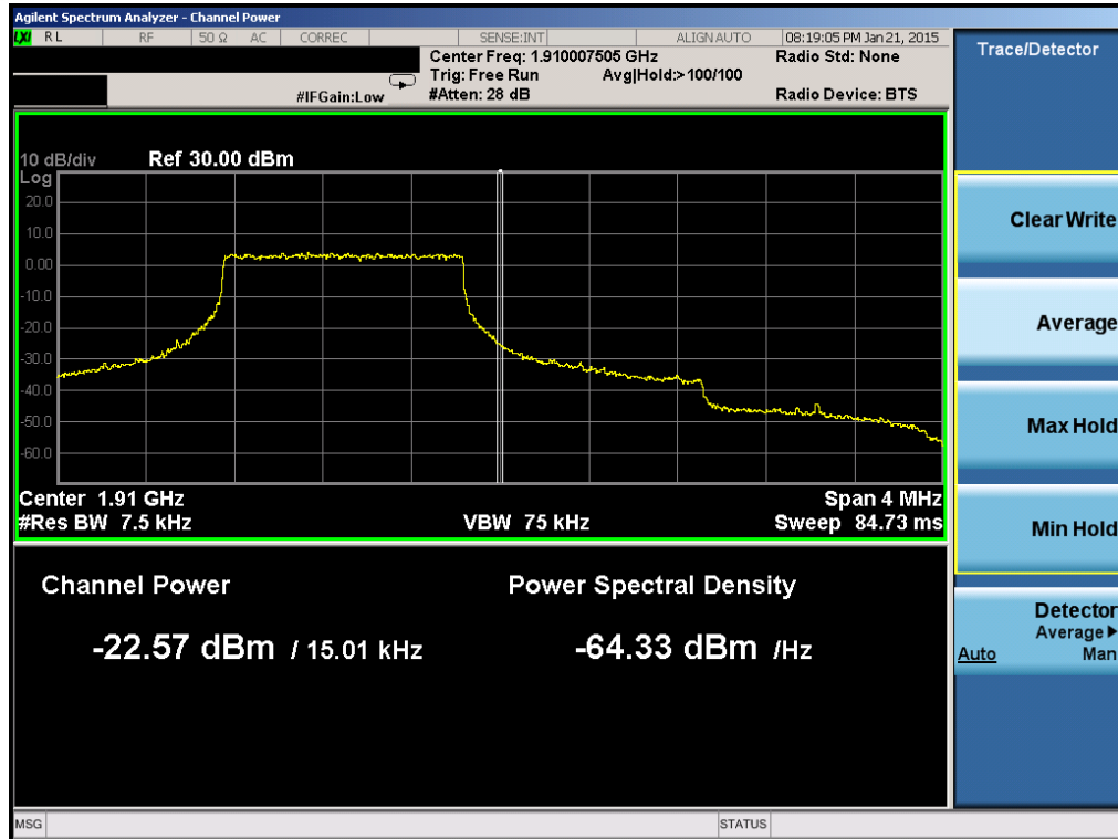
Plot 6-152. Upper Band Edge Plot (Band 2 – 1.4MHz QPSK – RB Size 6)
