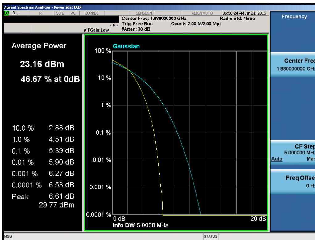
Plot 6-179. PAR Plot (Band 2 – 5.0MHz 16-QAM – RB Size 25)
