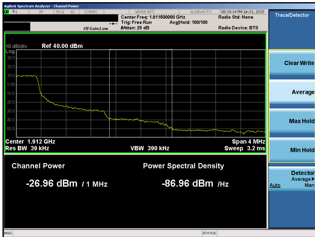
Plot 6-153. Upper Extended Band Edge Plot (Band 2 – 1.4MHz QPSK – RB Size 6)
