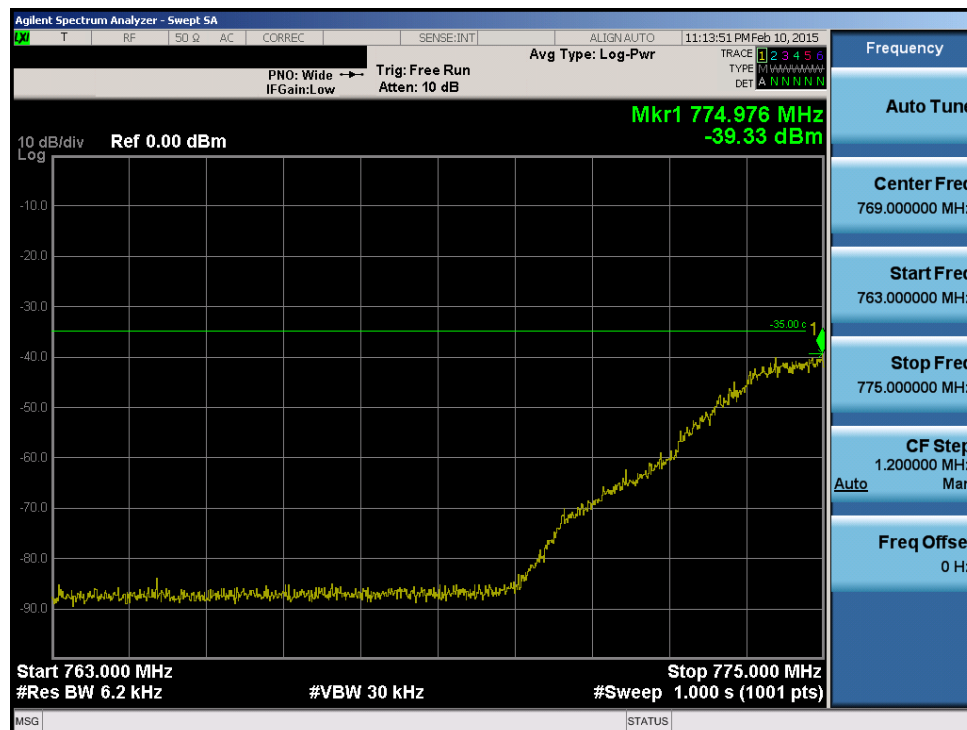
Plot 6-105. Lower Extended Band Edge Plot (Band 13 – 5.0MHz QPSK – RB Size 25)
