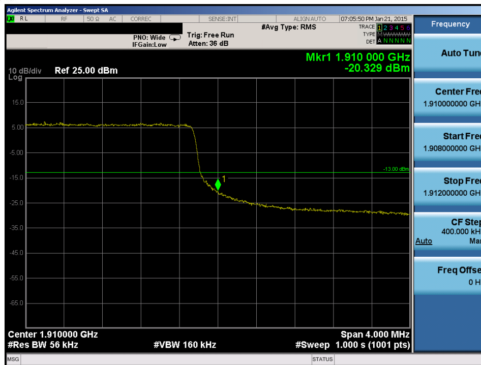
Plot 6-160. Upper Band Edge Plot (Band 2 – 5.0MHz QPSK – RB Size 25)
