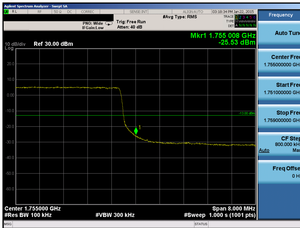
Plot 6-140. Upper Band Edge Plot (Band 4 – 10.0MHz QPSK – RB Size 50)
