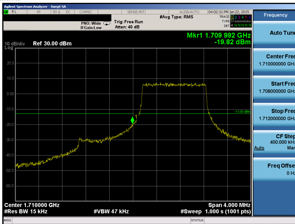
Plot 6-126. Lower Band Edge Plot (Band 4 – 1.4MHz QPSK – RB Size 6)
