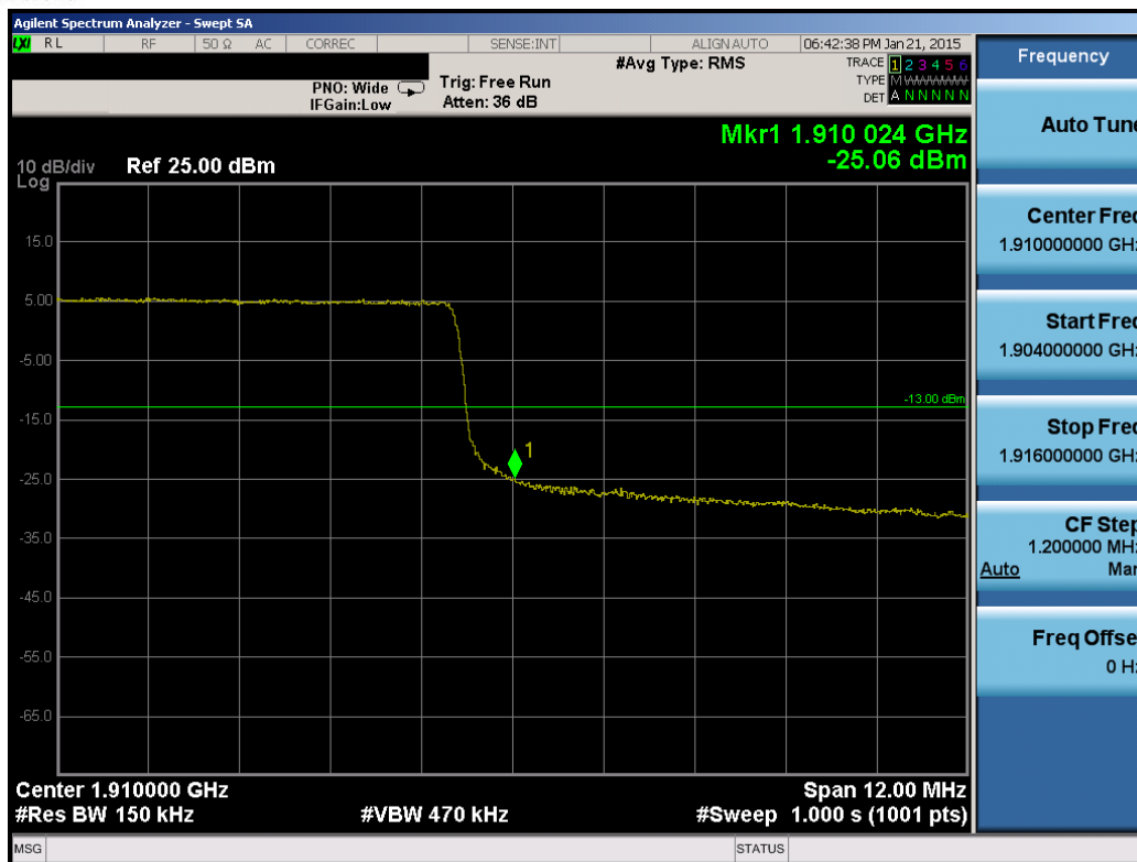
Plot 6-168. Upper Band Edge Plot (Band 2 - 15.0MHz QPSK - RB Size 75)
