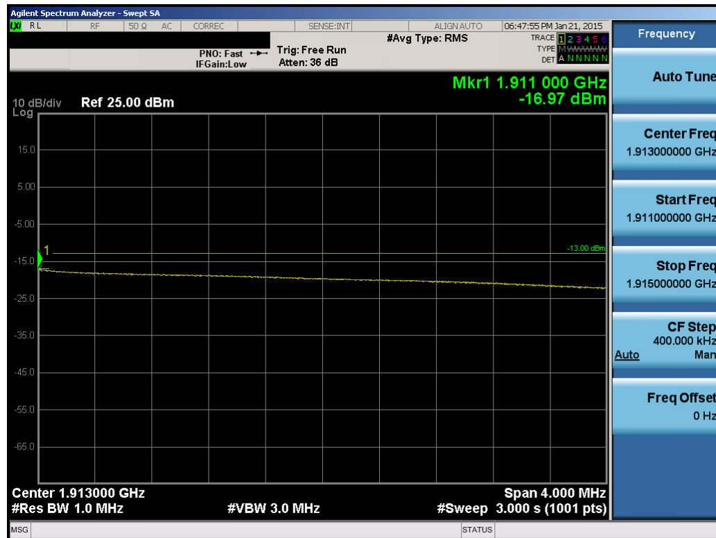
Plot 6-165. Upper Extended Band Edge Plot (Band 2 – 10.0MHz QPSK – RB Size 50)
