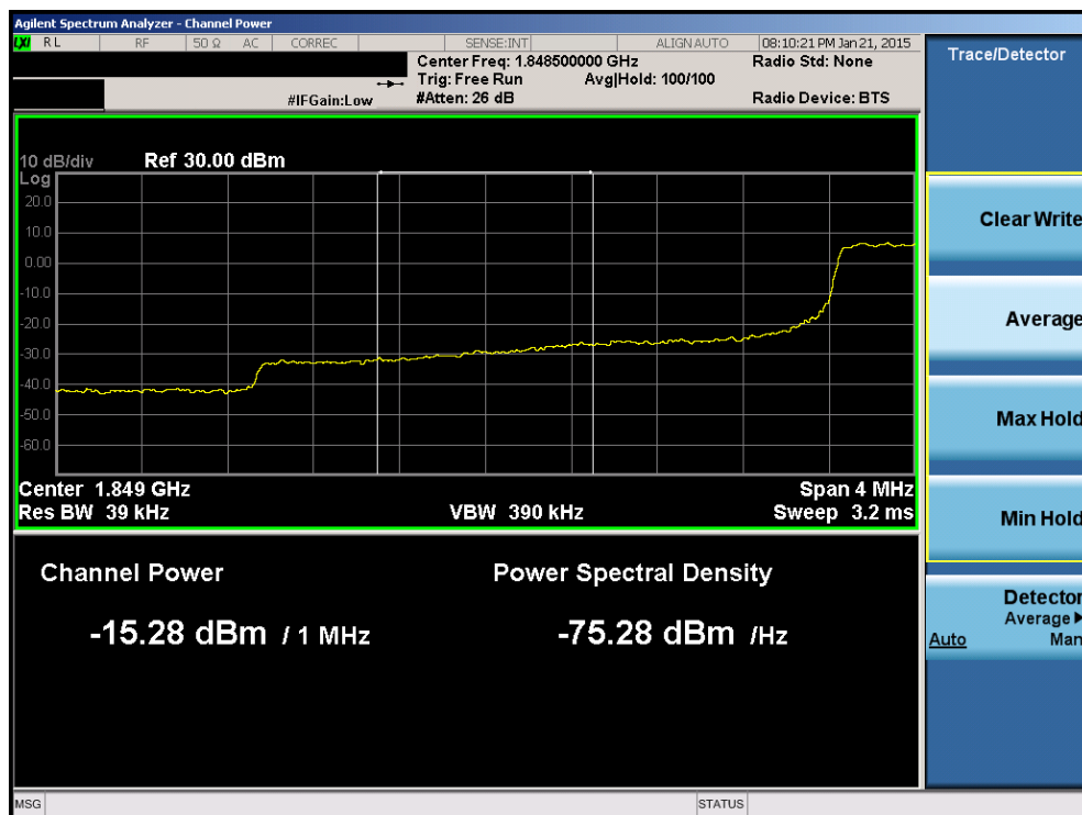
Plot 6-155. Lower Extended Band Edge Plot (Band 2 – 3.0MHz QPSK – RB Size 15)
