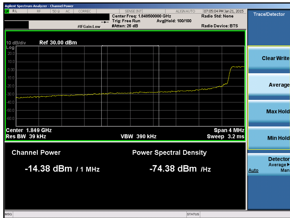
Plot 6-159. Lower Extended Band Edge Plot (Band 2 – 5.0MHz QPSK – RB Size 25)
