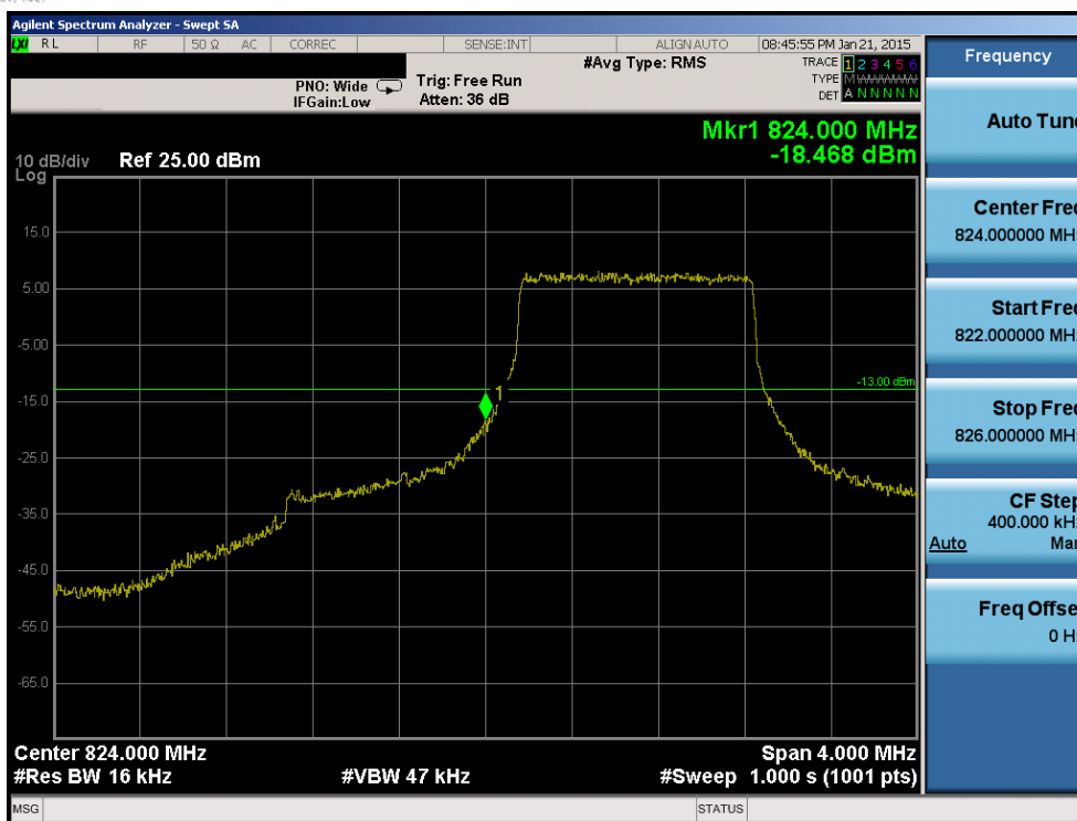
Plot 6-112. Lower Band Edge Plot (Band 5 – 1.4MHz QPSK – RB Size 6)
