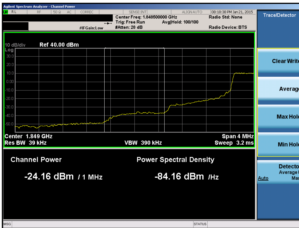
Plot 6-151. Lower Extended Band Edge Plot (Band 2 – 1.4MHz QPSK – RB Size 6)
