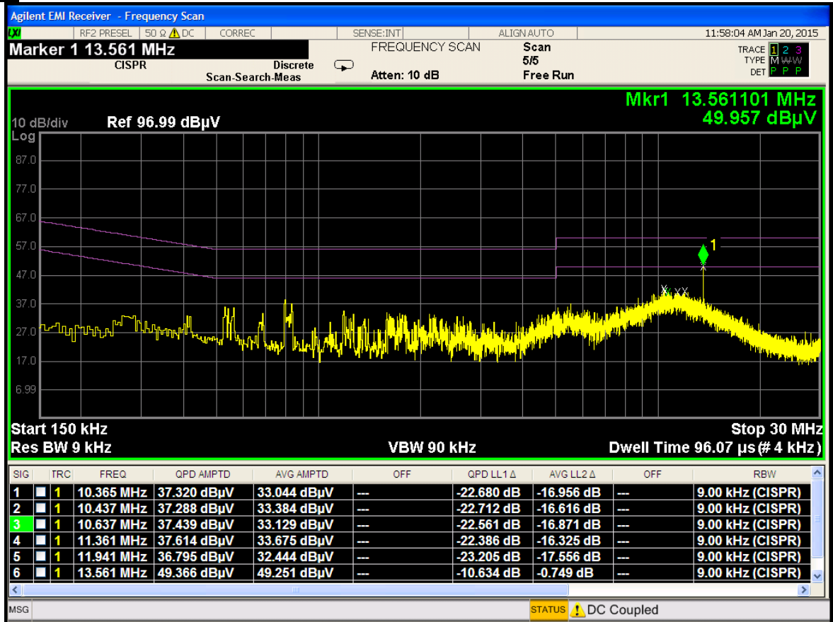
Plot 7-2. Line-Conducted Test Plot (N)
