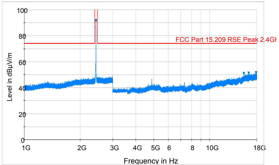
Plot 6-71. Radiated Spurious Plot above 1GHz (802.11b – Ch. 6, Ant. Pol. H)
