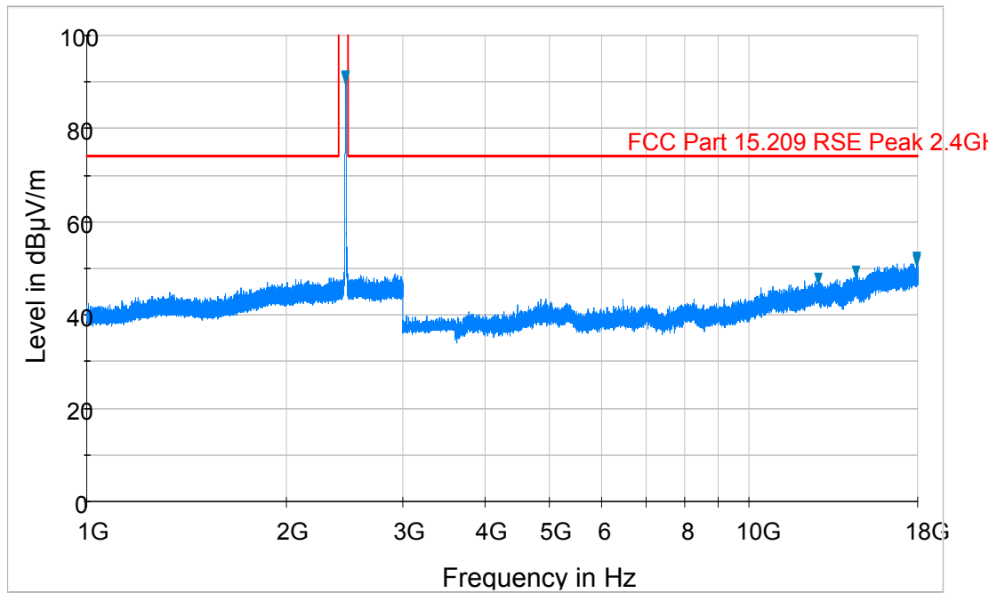
Plot 6-74. Radiated Spurious Plot above 1GHz (802.11b – Ch. 11, Ant. Pol. V)
