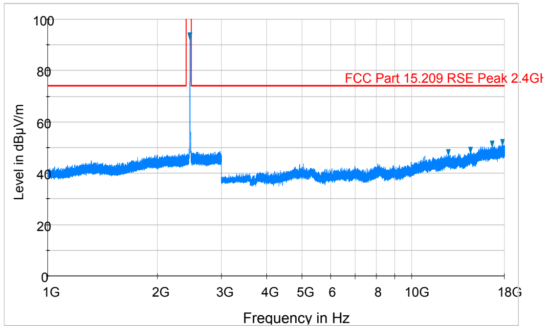
Plot 6-73. Radiated Spurious Plot above 1GHz (802.11b – Ch. 11, Ant. Pol. H)
