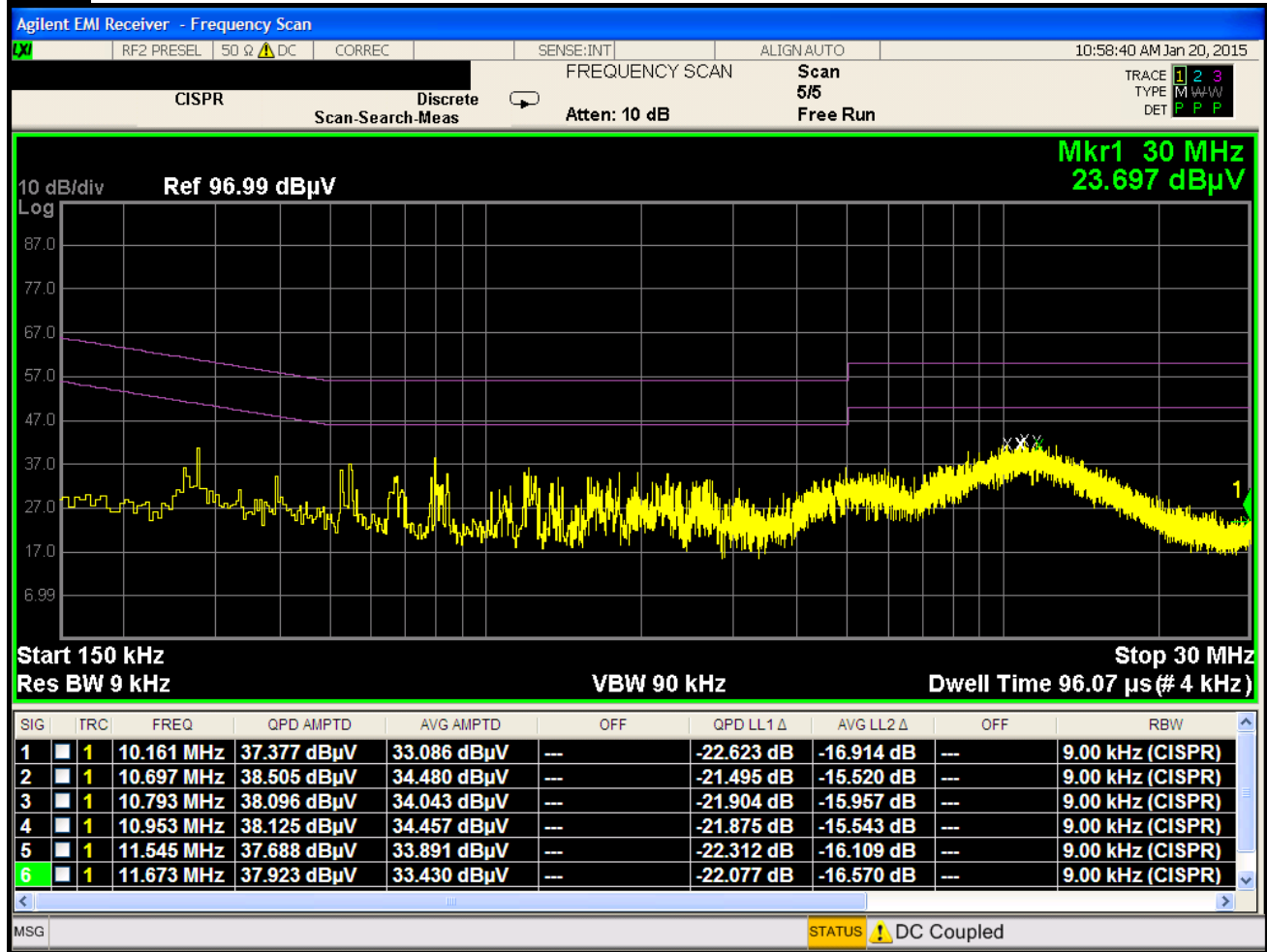
Plot 6-92. Line Conducted Plot with 802.11b (N)
