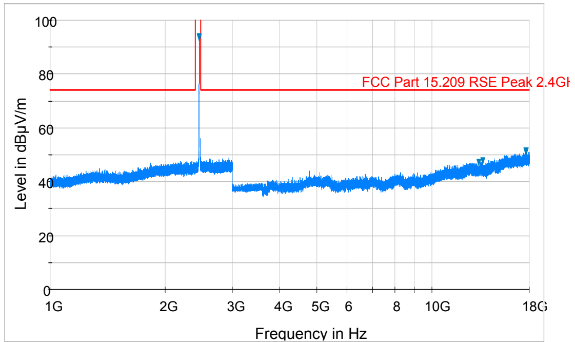
Plot 6-65. Radiated Spurious Plot above 1GHz (802.11b – Ch. 11, Ant. Pol. H)
