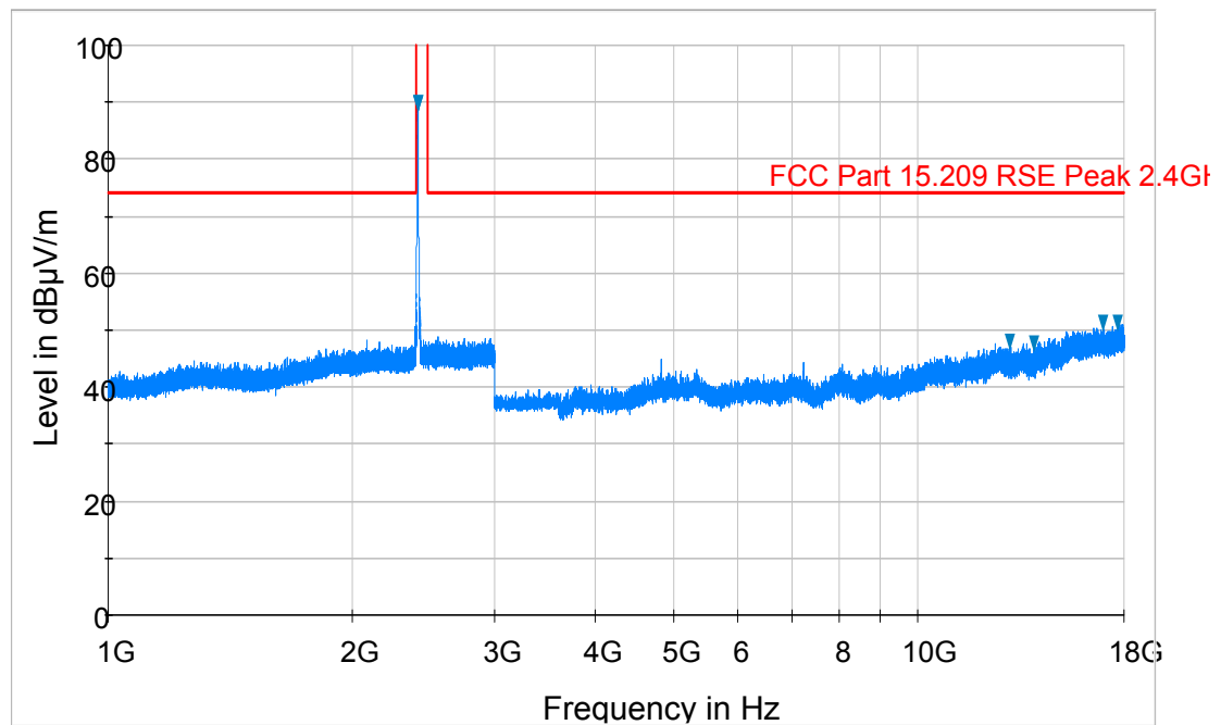
Plot 6-69. Radiated Spurious Plot above 1GHz (802.11b – Ch. 1, Ant. Pol. H)
