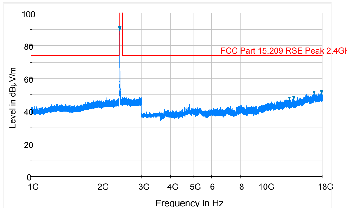
Plot 6-70. Radiated Spurious Plot above 1GHz (802.11b – Ch. 1, Ant. Pol. V)
