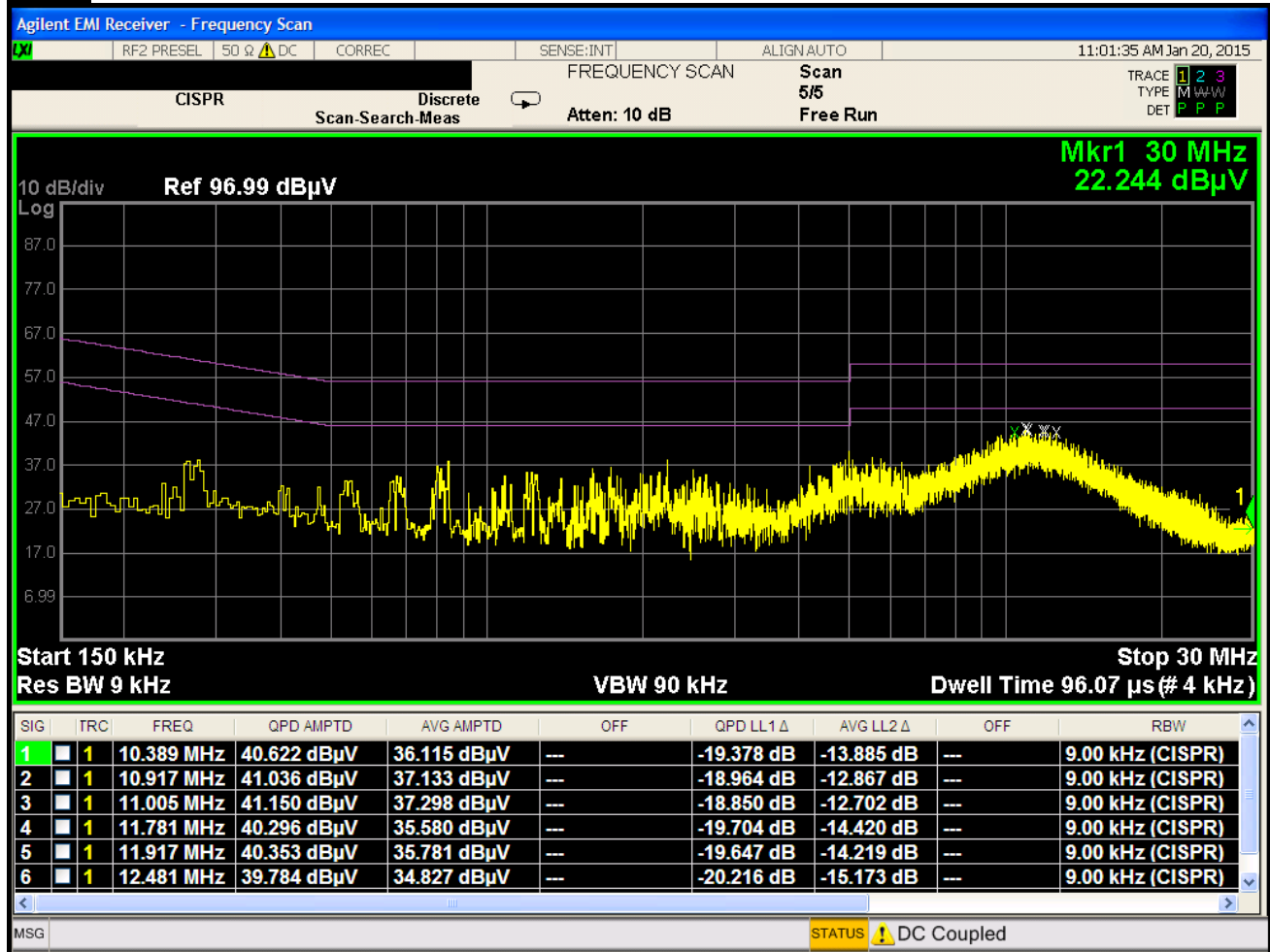
Plot 6-91. Line Conducted Plot with 802.11b (L1)
