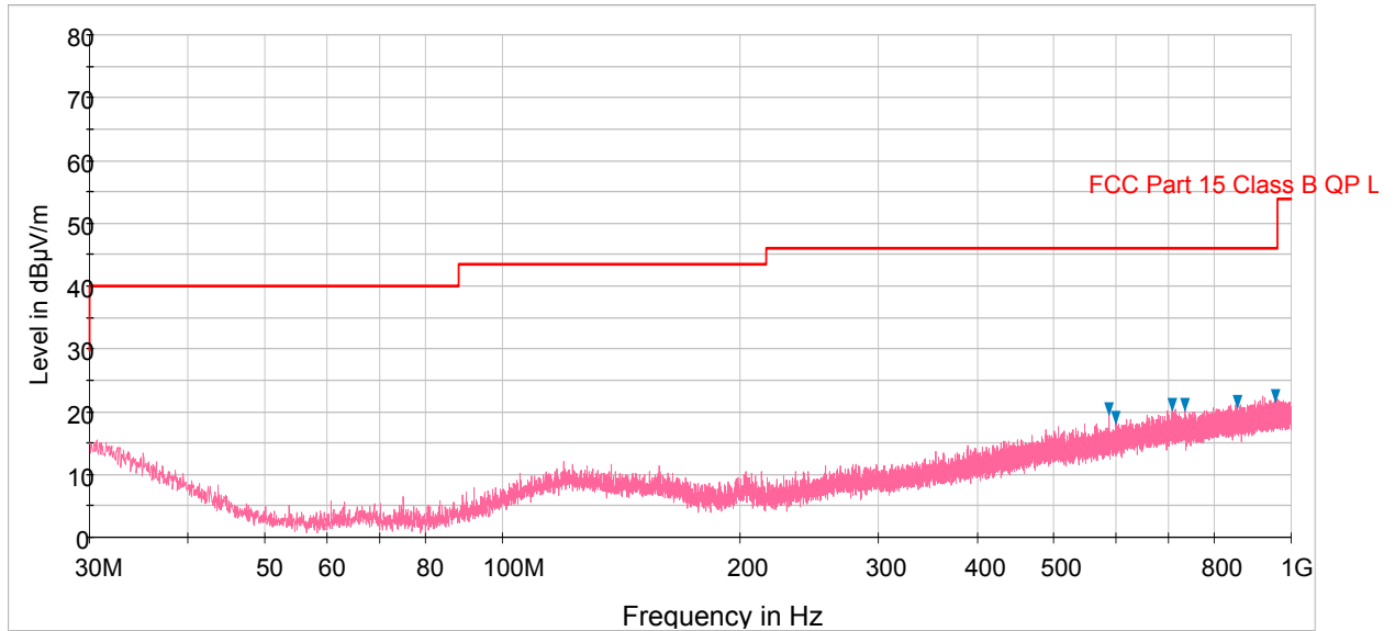
Plot 6-89. Radiated Spurious Plot below 1GHz (Pol. H)
