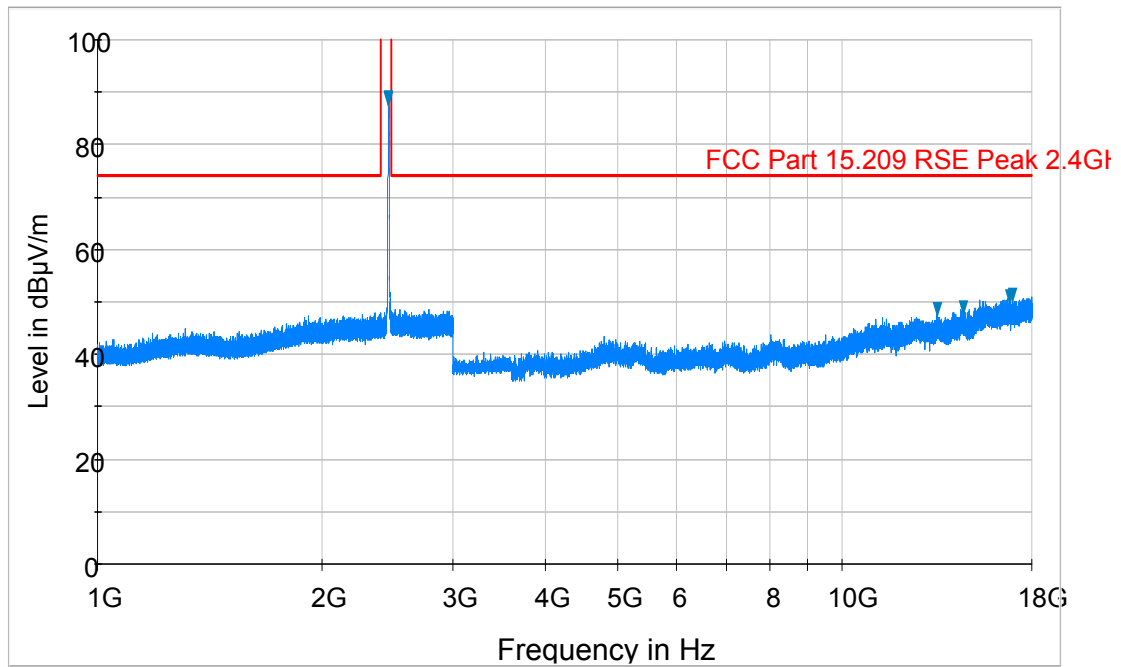
Plot 6-66. Radiated Spurious Plot above 1GHz (802.11b – Ch. 11, Ant. Pol. V)
