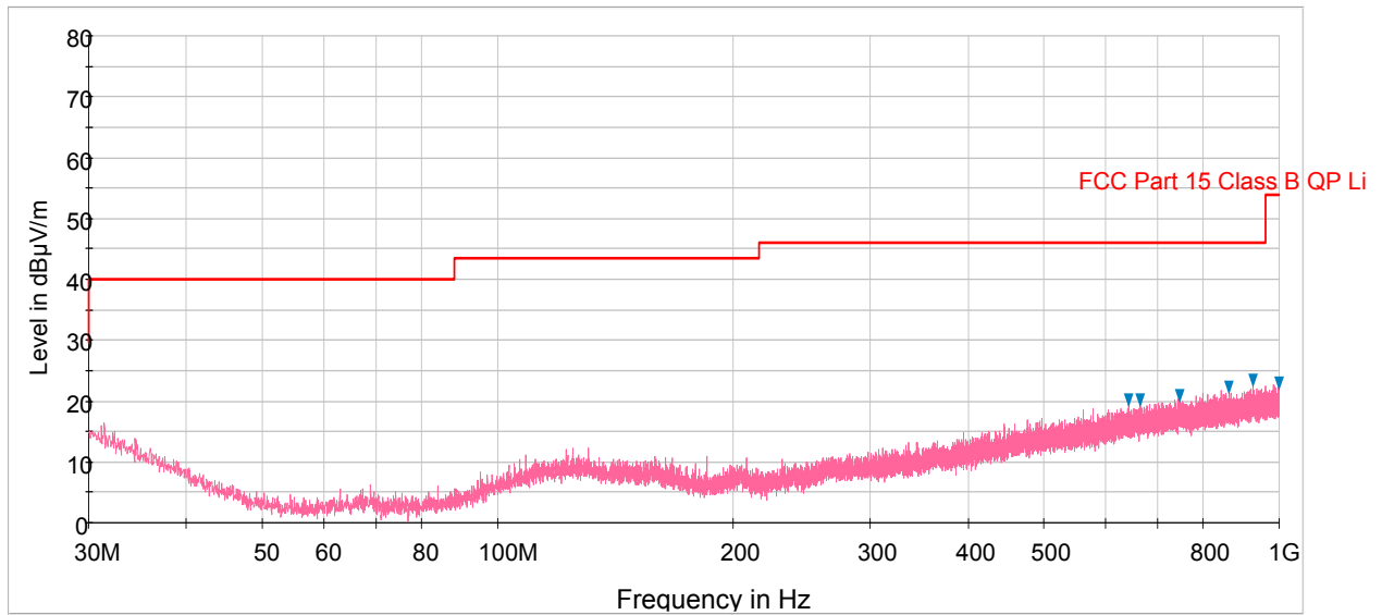
Plot 6-90. Radiated Spurious Plot below 1GHz (Pol. V)
