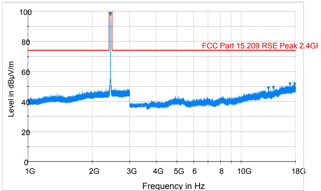
Plot 6-64. Radiated Spurious Plot above 1GHz (802.11b – Ch. 6, Ant. Pol. V)
