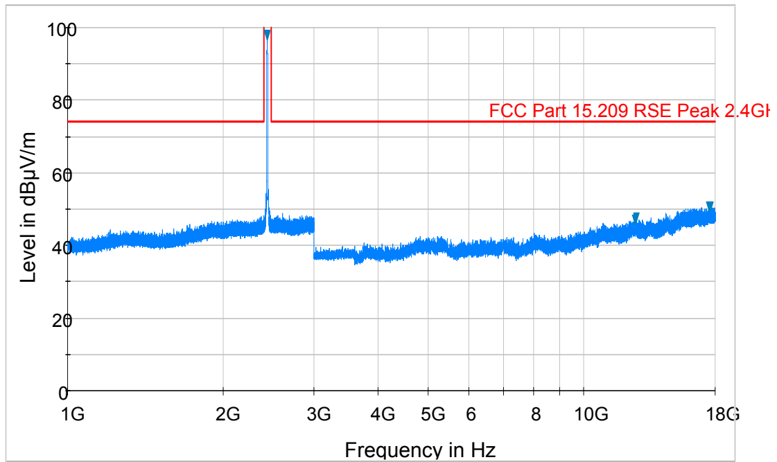
Plot 6-72. Radiated Spurious Plot above 1GHz (802.11b – Ch. 6, Ant. Pol. V)
