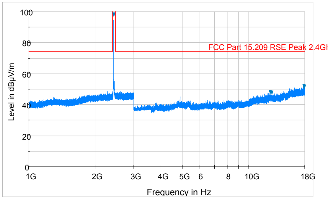
Plot 6-63. Radiated Spurious Plot above 1GHz (802.11b – Ch. 6, Ant. Pol. H)
