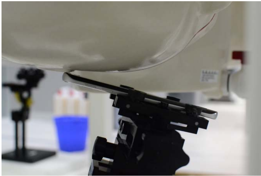
SAR Test Setup Photo 2: Right Tilt
