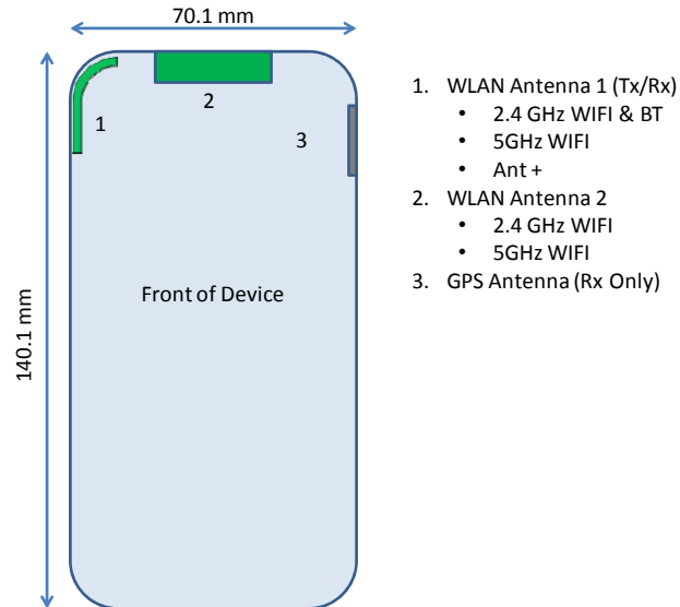
Figure F-1 DUT Antenna Locations
