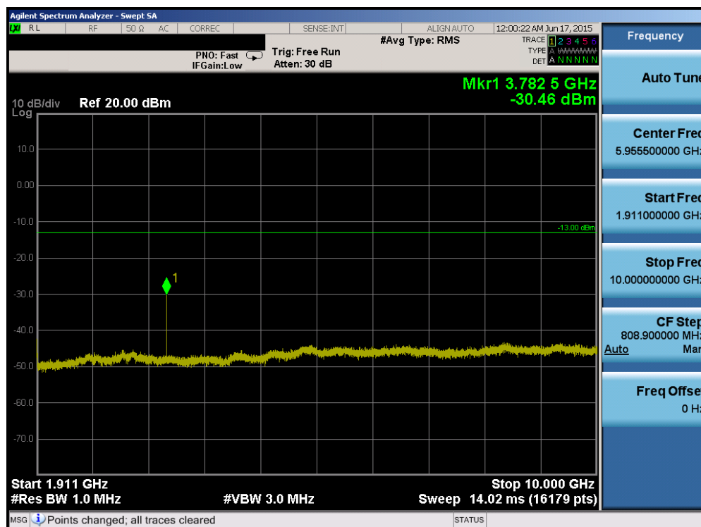
Plot 6-94. Conducted Spurious Plot (Band 2 – 20.0MHz QPSK – RB Size 1, RB Offset 0 – High Channel)
