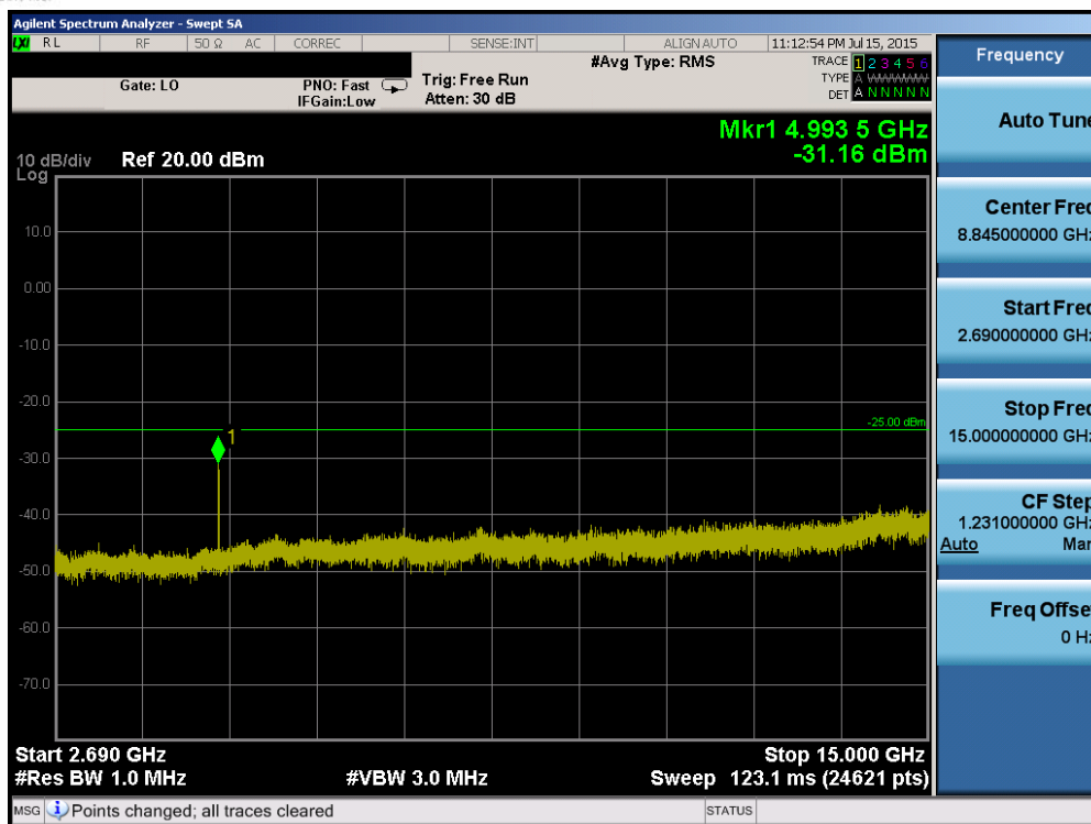
Plot 6-97. Conducted Spurious Plot (Band 41 – 15.0MHz QPSK – RB Size 1, RB Offset 0 – Low Channel)
