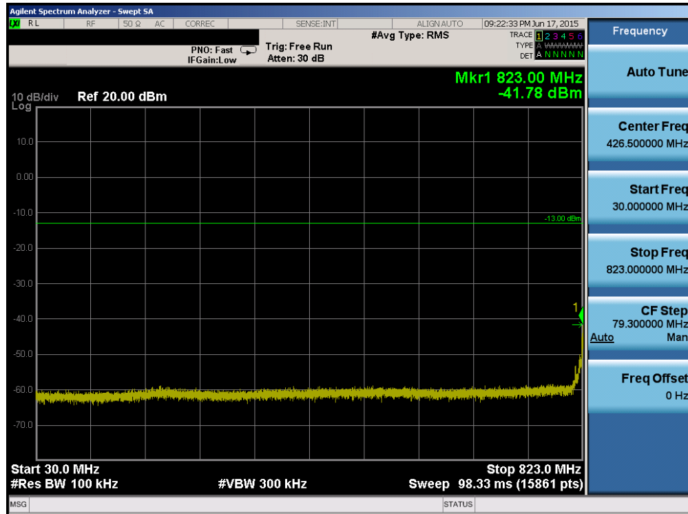
Plot 6-69. Conducted Spurious Plot (Band 26 – 15.0MHz QPSK – RB Size 1, RB Offset 0 – Low Channel)
