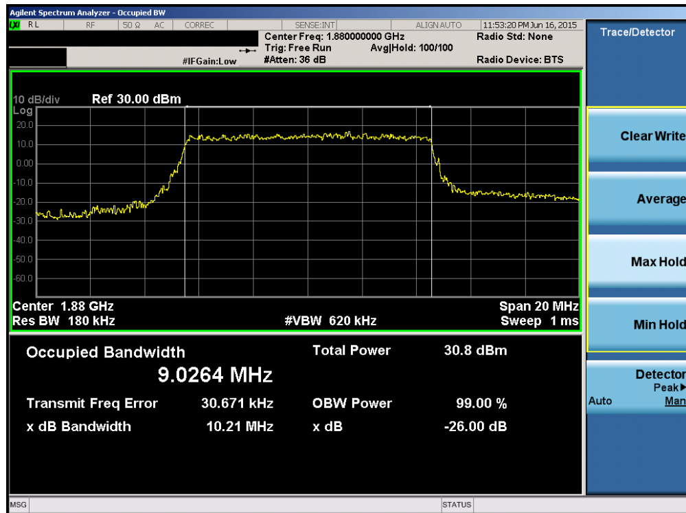
Plot 6-38. Occupied Bandwidth Plot (Band 2 – 10.0MHz 16-QAM – RB Size 50)
