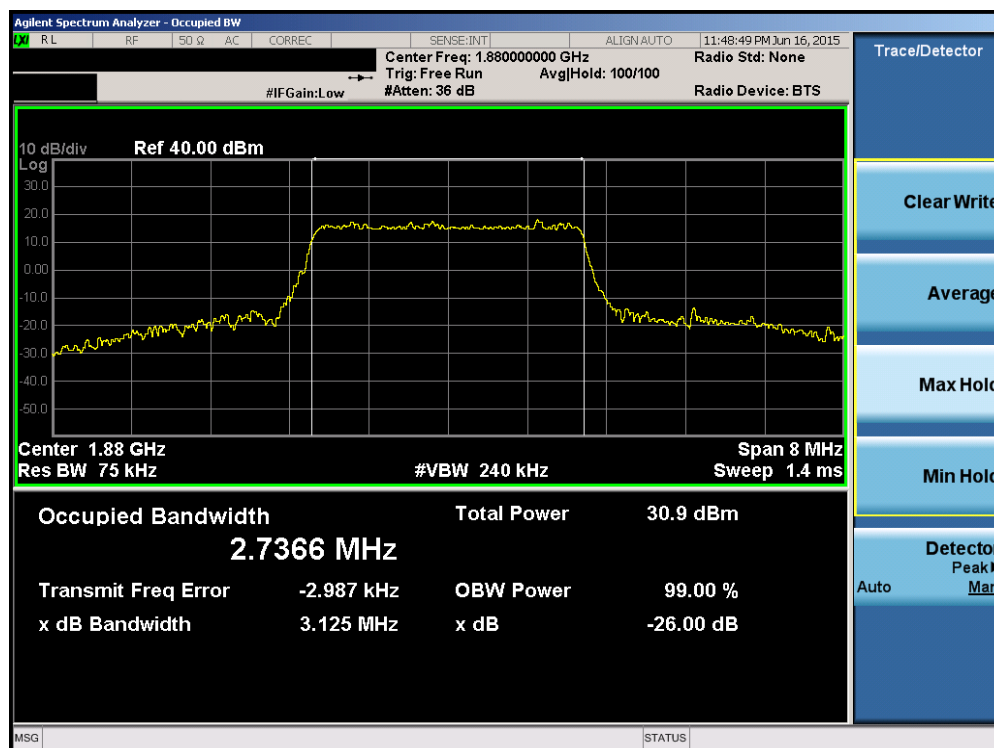
Plot 6-34. Occupied Bandwidth Plot (Band 2 – 3.0MHz 16-QAM – RB Size 15)
