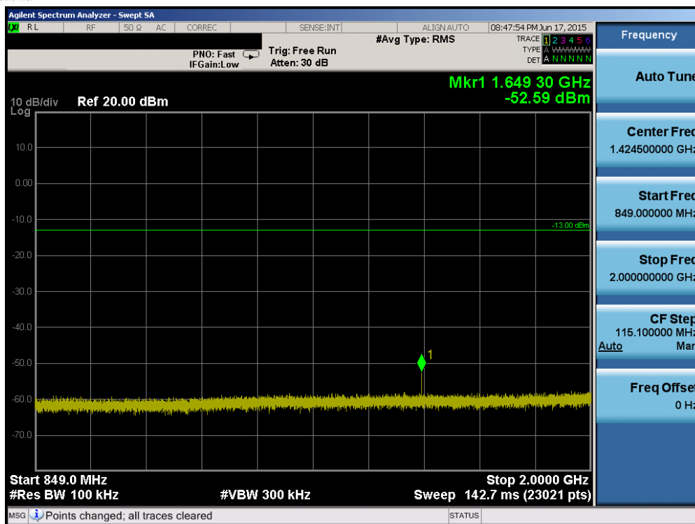
Plot 6-61. Conducted Spurious Plot (Band 5 – 10.0MHz QPSK – RB Size 1, RB Offset 0 – Low Channel)
