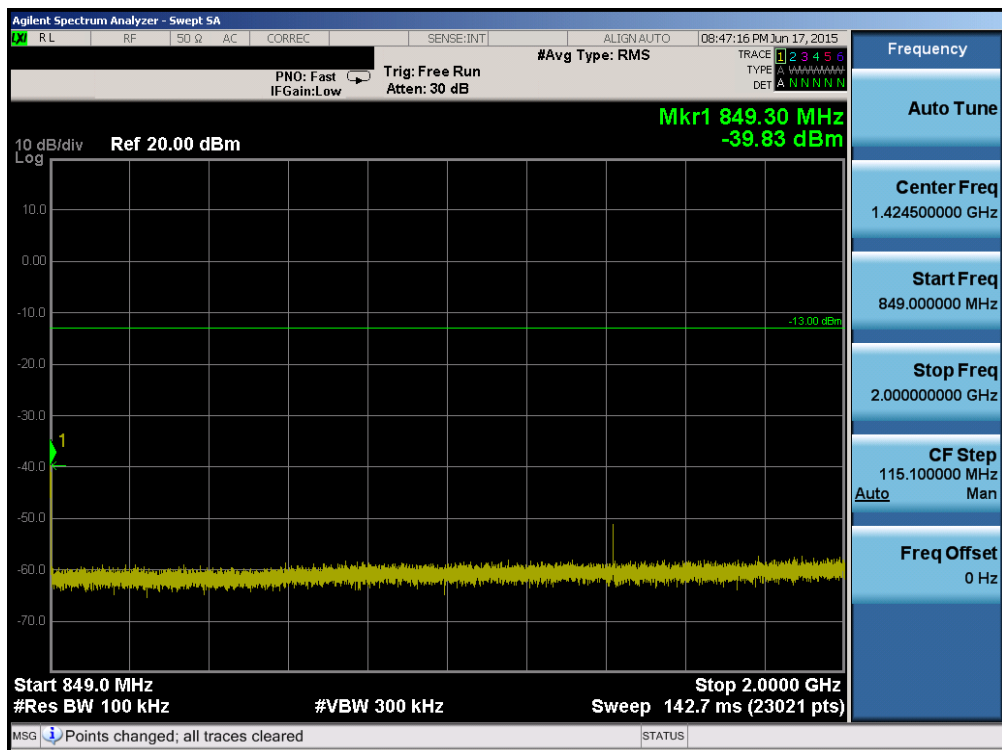
Plot 6-64. Conducted Spurious Plot (Band 5 – 10.0MHz QPSK – RB Size 1, RB Offset 0 – Mid Channel)
