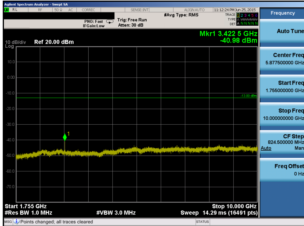
Plot 6-79. Conducted Spurious Plot (Band 4 – 20.0MHz QPSK – RB Size 1, RB Offset 0 – Low Channel)
