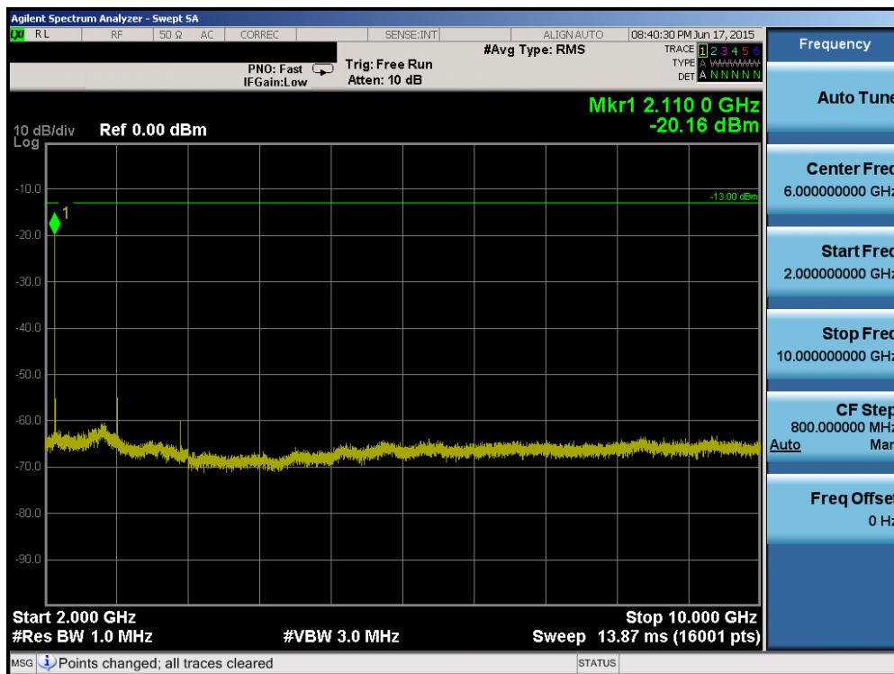
Plot 6-56. Conducted Spurious Plot (Band 12/17 – 10.0MHz QPSK – RB Size 1, RB Offset 0 – Mid Channel)
