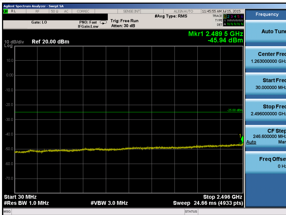
Plot 6-99. Conducted Spurious Plot (Band 41 – 15.0MHz QPSK – RB Size 1, RB Offset 0 – Mid Channel)
