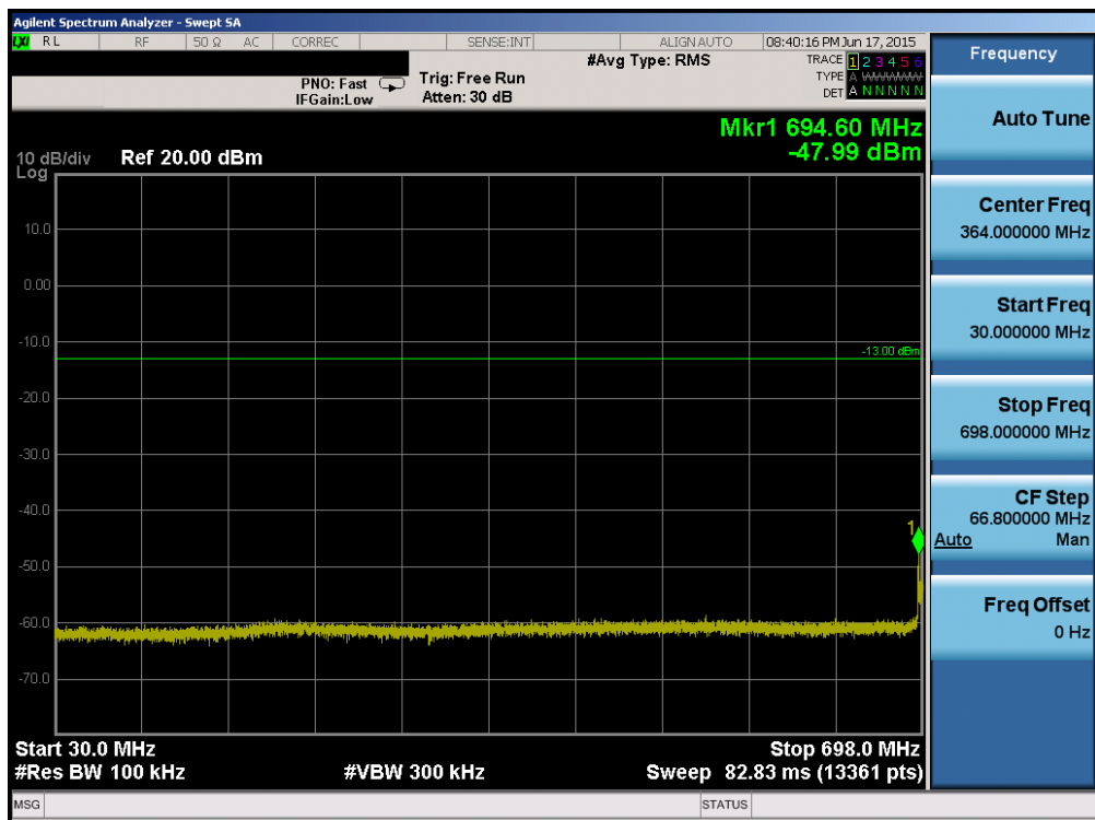
Plot 6-54. Conducted Spurious Plot (Band 12/17 – 10.0MHz QPSK – RB Size 1, RB Offset 0 – Mid Channel)
