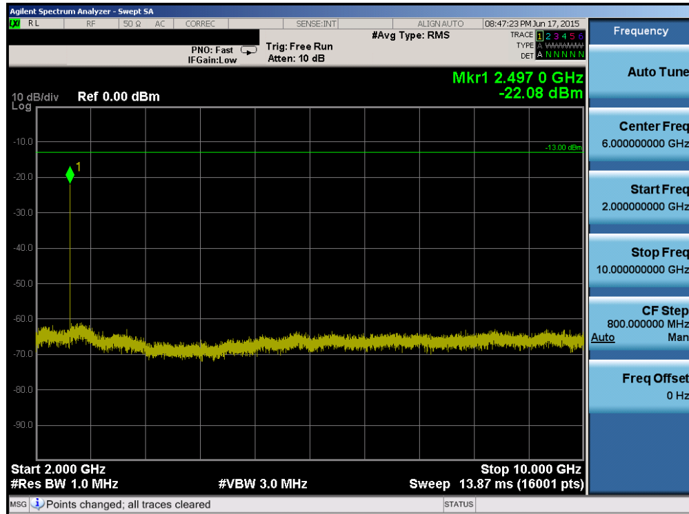
Plot 6-65. Conducted Spurious Plot (Band 5 – 10.0MHz QPSK – RB Size 1, RB Offset 0 – Mid Channel)
