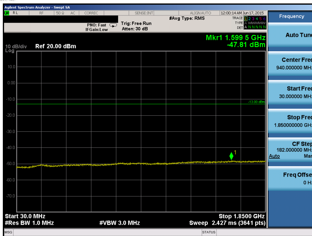
Plot 6-93. Conducted Spurious Plot (Band 2 – 20.0MHz QPSK – RB Size 1, RB Offset 0 – High Channel)
