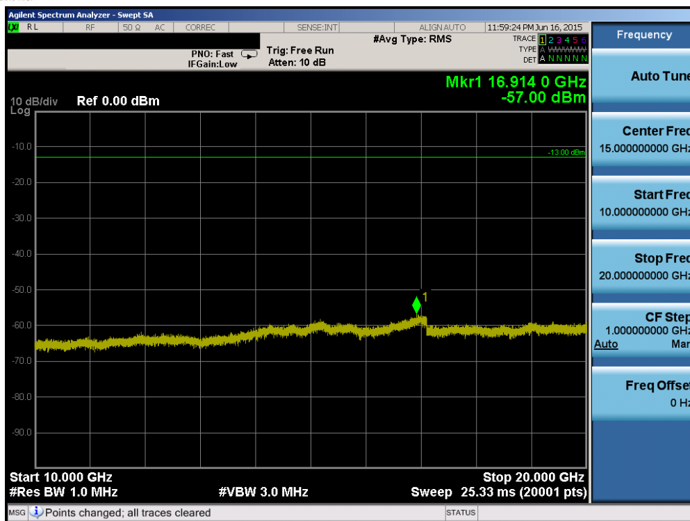
Plot 6-89. Conducted Spurious Plot (Band 2 – 20.0MHz QPSK – RB Size 1, RB Offset 0 – Low Channel)
