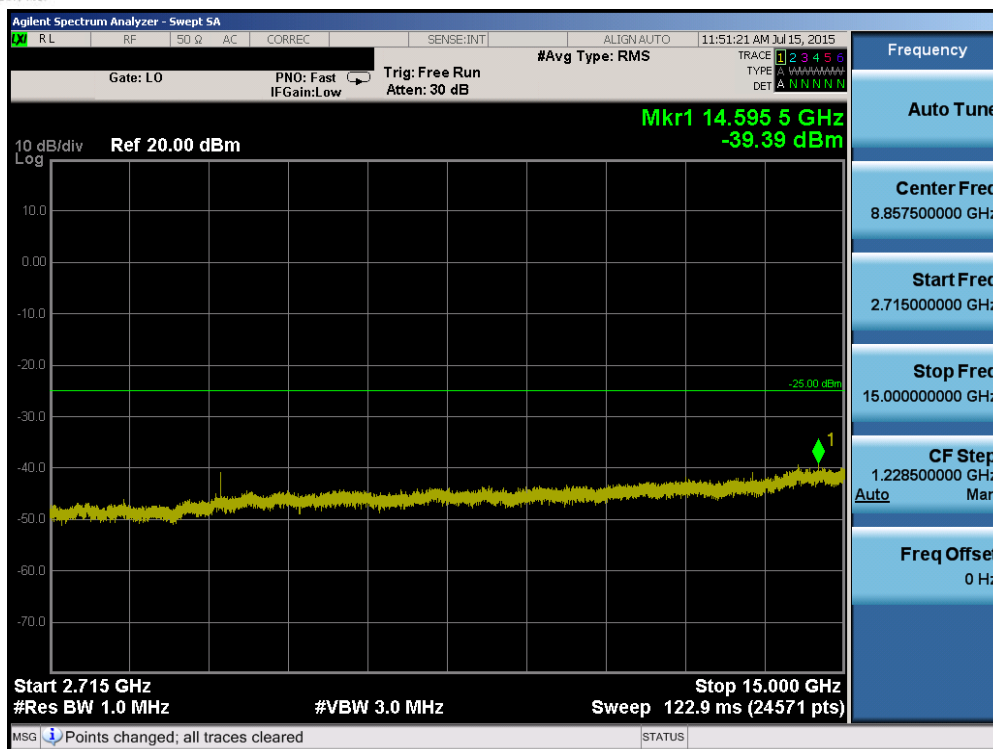
Plot 6-103. Conducted Spurious Plot (Band 41 – 15.0MHz QPSK – RB Size 1, RB Offset 0 – High Channel)
