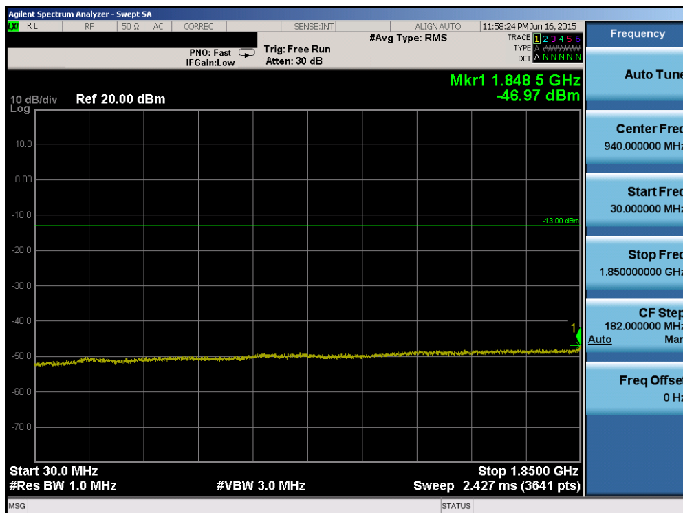
Plot 6-90. Conducted Spurious Plot (Band 2 – 20.0MHz QPSK – RB Size 1, RB Offset 0 – Mid Channel)
