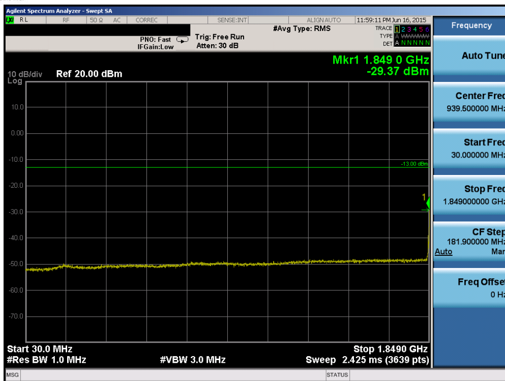
Plot 6-87. Conducted Spurious Plot (Band 2 – 20.0MHz QPSK – RB Size 1, RB Offset 0– Low Channel)
