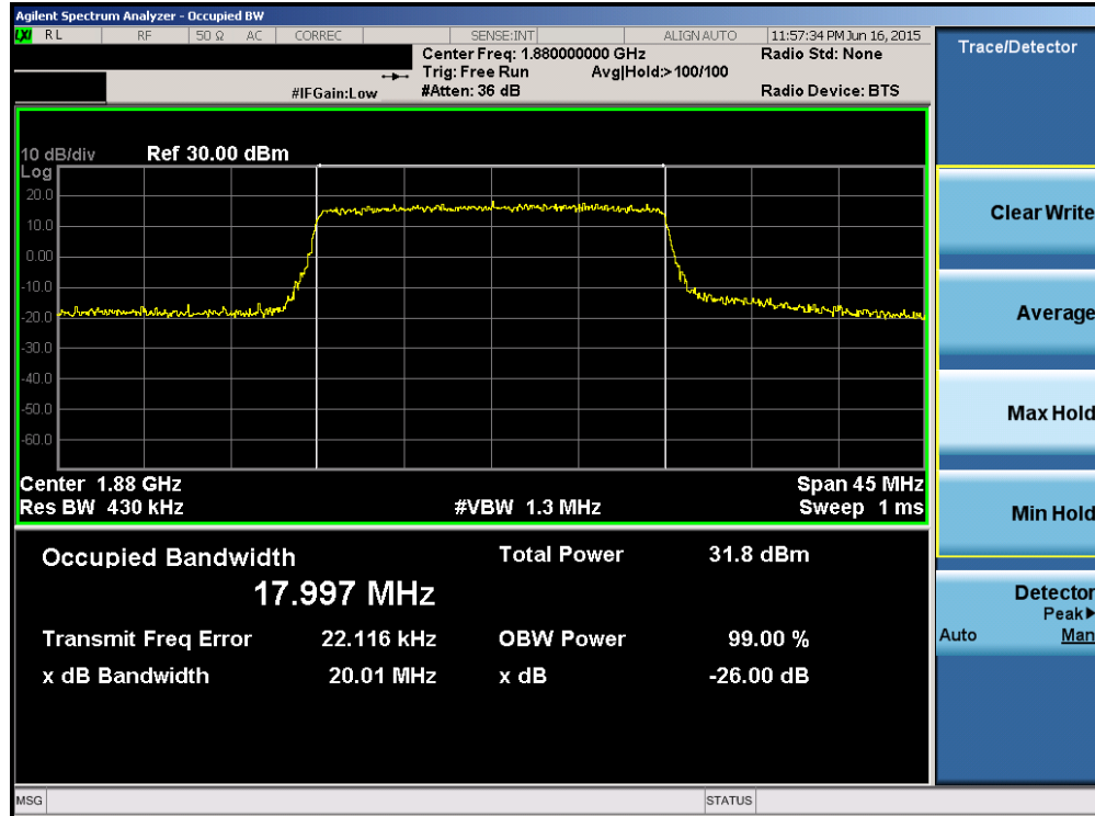
Plot 6-41. Occupied Bandwidth Plot (Band 2 – 20.0MHz QPSK – RB Size 100)
