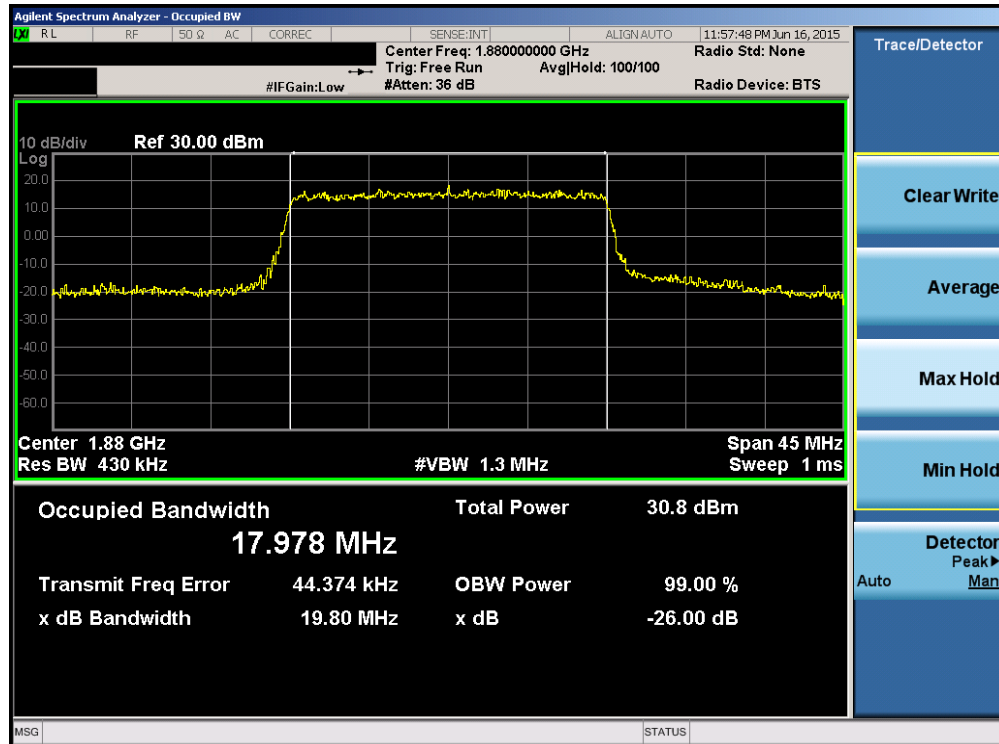
Plot 6-42. Occupied Bandwidth Plot (Band 2 – 20.0MHz 16-QAM – RB Size 100)
