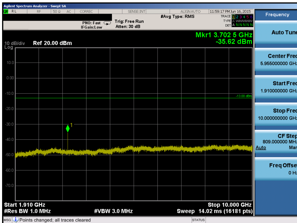
Plot 6-88. Conducted Spurious Plot (Band 2 – 20.0MHz QPSK – RB Size 1, RB Offset 0 – Low Channel)
