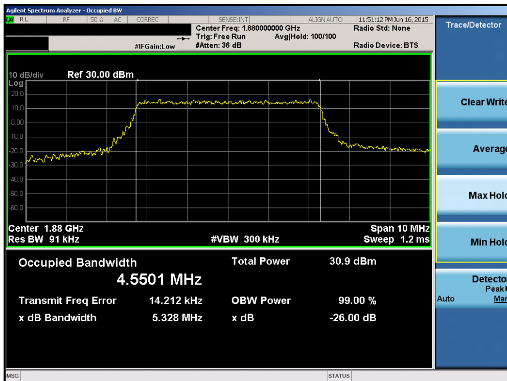
Plot 6-36. Occupied Bandwidth Plot (Band 2 – 5.0MHz 16-QAM – RB Size 25)
