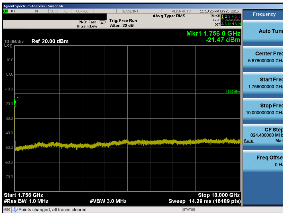
Plot 6-85. Conducted Spurious Plot (Band 4 – 20.0MHz QPSK – RB Size 1, RB Offset 0 – High Channel)
