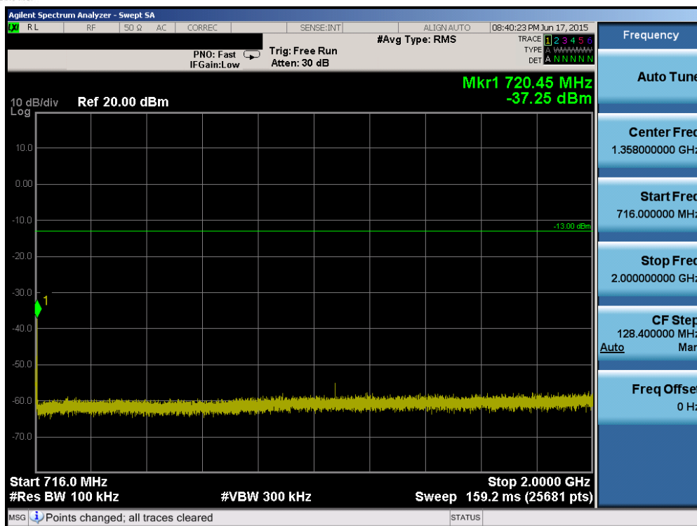
Plot 6-55. Conducted Spurious Plot (Band 12/17 – 10.0MHz QPSK – RB Size 1, RB Offset 0 – Mid Channel)
