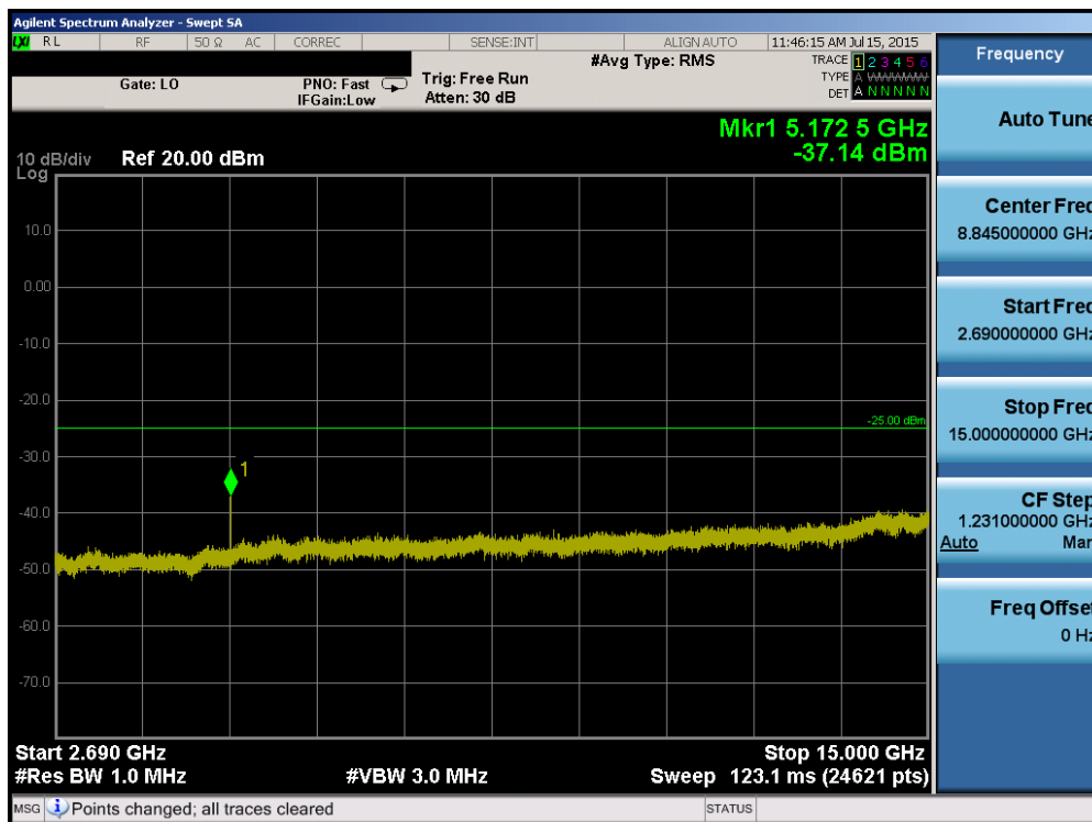
Plot 6-100. Conducted Spurious Plot (Band 41 – 15.0MHz QPSK – RB Size 1, RB Offset 0 – Mid Channel)
