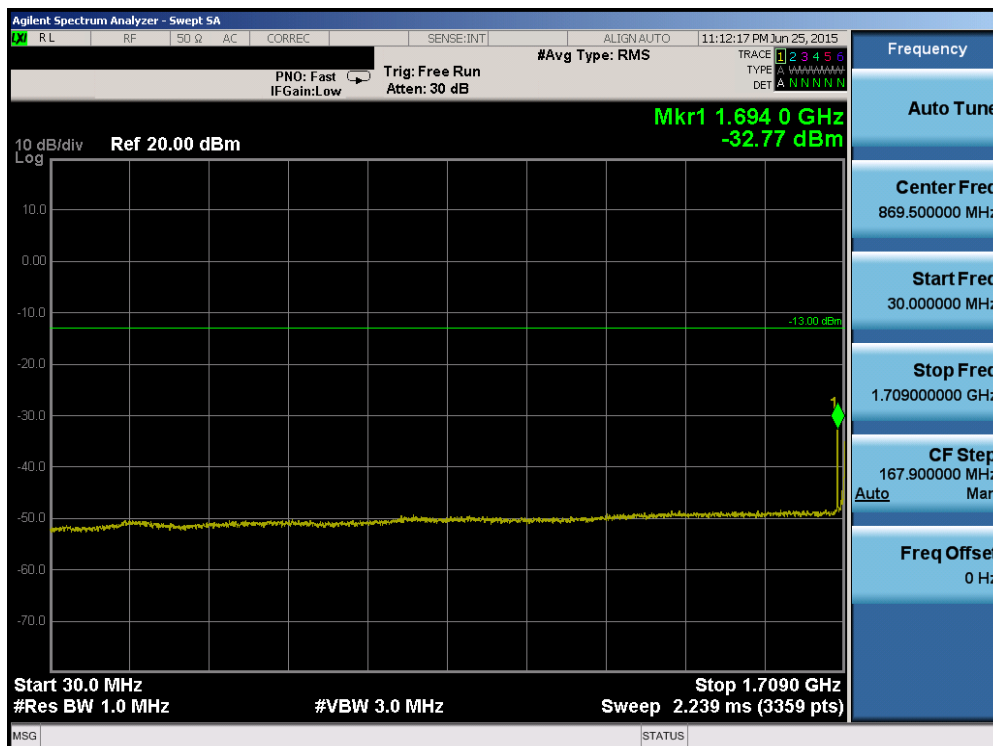
Plot 6-78. Conducted Spurious Plot (Band 4 – 20.0MHz QPSK – RB Size 1, RB Offset 0- Low Channel)
