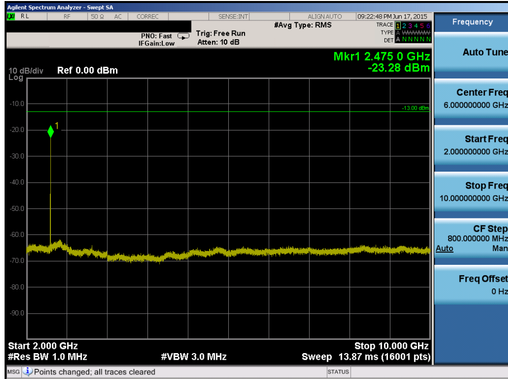
Plot 6-71. Conducted Spurious Plot (Band 26 – 15.0MHz QPSK – RB Size 1, RB Offset 0 – Low Channel)
