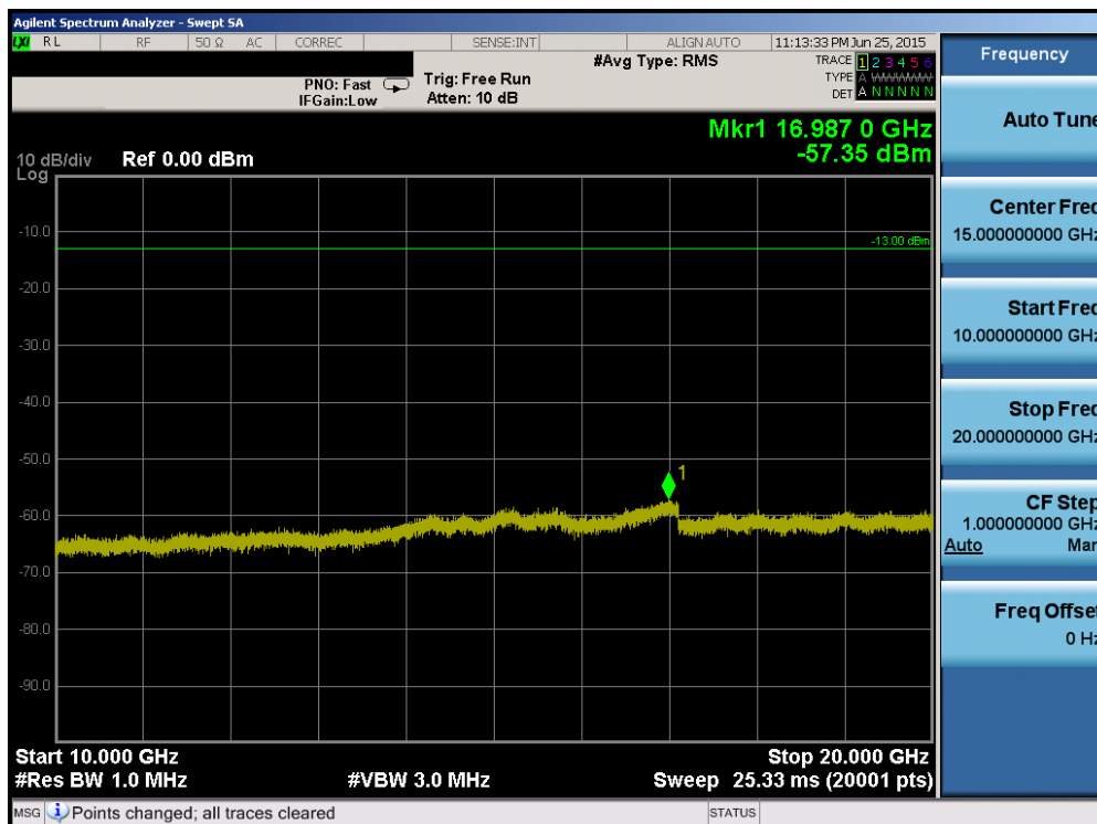
Plot 6-86. Conducted Spurious Plot (Band 4 – 20.0MHz QPSK – RB Size 1, RB Offset 0 – High Channel)
