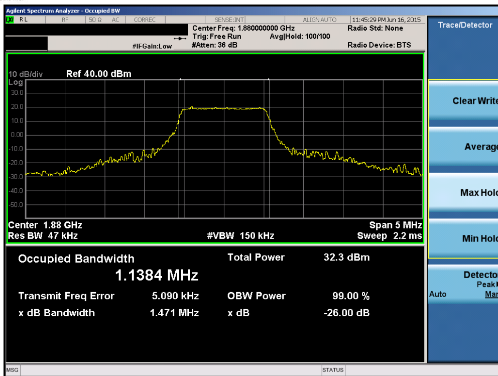
Plot 6-31. Occupied Bandwidth Plot (Band 2 – 1.4MHz QPSK – RB Size 6)
