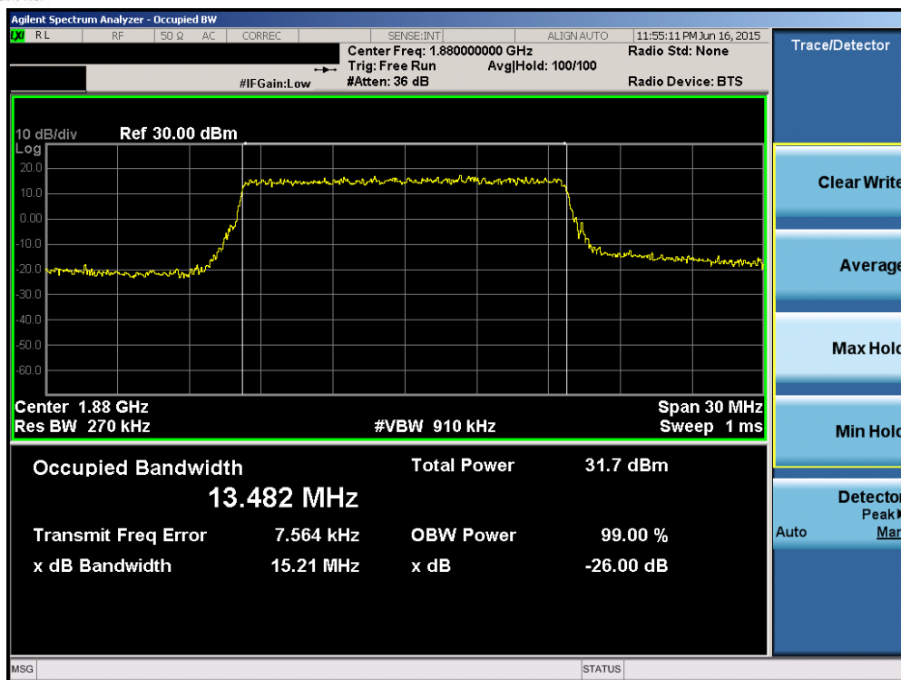
Plot 6-39. Occupied Bandwidth Plot (Band 2 – 15.0MHz QPSK – RB Size 75)
