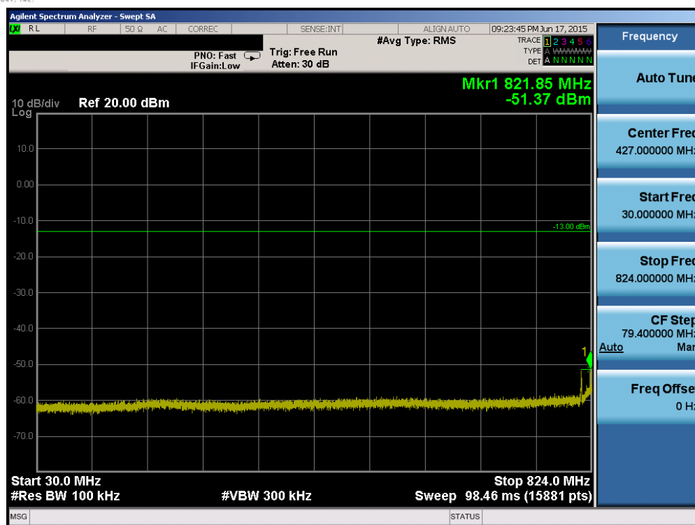
Plot 6-75. Conducted Spurious Plot (Band 26 – 15.0MHz QPSK – RB Size 1, RB Offset 0 – High Channel)
