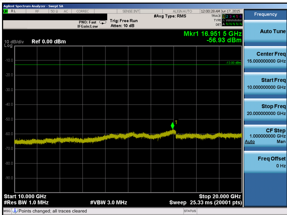
Plot 6-95. Conducted Spurious Plot (Band 2 – 20.0MHz QPSK – RB Size 1, RB Offset 0 – High Channel)
