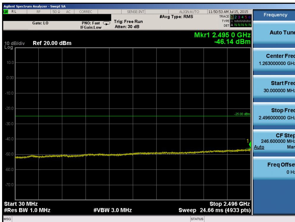
Plot 6-102. Conducted Spurious Plot (Band 41 – 15.0MHz QPSK – RB Size 1, RB Offset 0 – High Channel)
