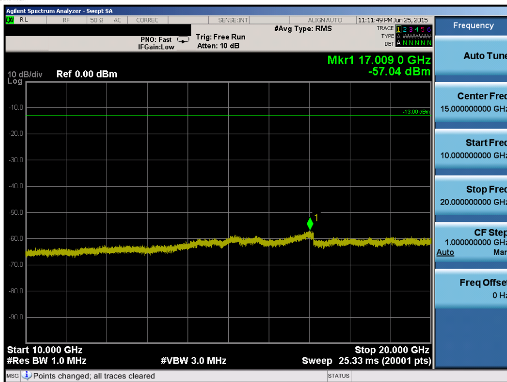
Plot 6-83. Conducted Spurious Plot (Band 4 - 20.0MHz QPSK - RB Size 1, RB Offset 0 - Mid Channel)
