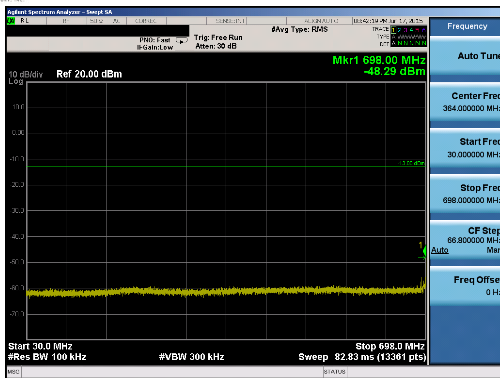
Plot 6-57. Conducted Spurious Plot (Band 12/17 – 10.0MHz QPSK – RB Size 1, RB Offset 0 – High Channel)
