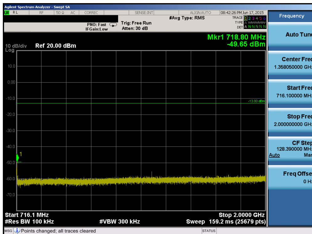
Plot 6-58. Conducted Spurious Plot (Band 12/17 – 10.0MHz QPSK – RB Size 1, RB Offset 0 – High Channel)
