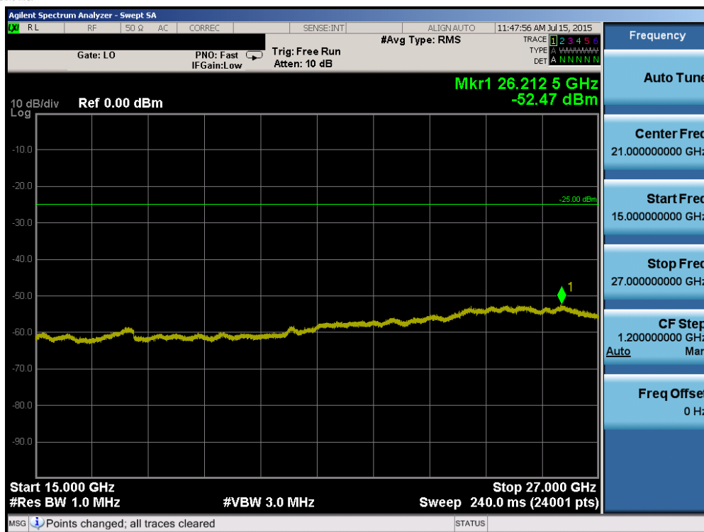
Plot 6-101. Conducted Spurious Plot (Band 41 – 15.0MHz QPSK – RB Size 1, RB Offset 0 – Mid Channel)
