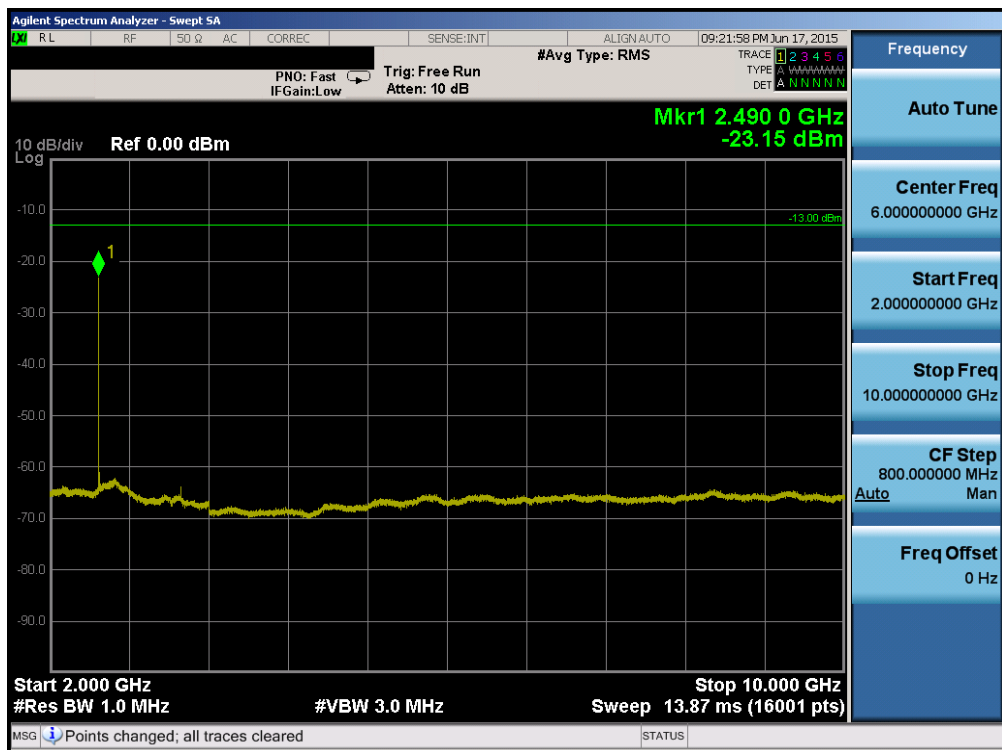
Plot 6-74. Conducted Spurious Plot (Band 26 – 15.0MHz QPSK – RB Size 1, RB Offset 0 – Mid Channel)
