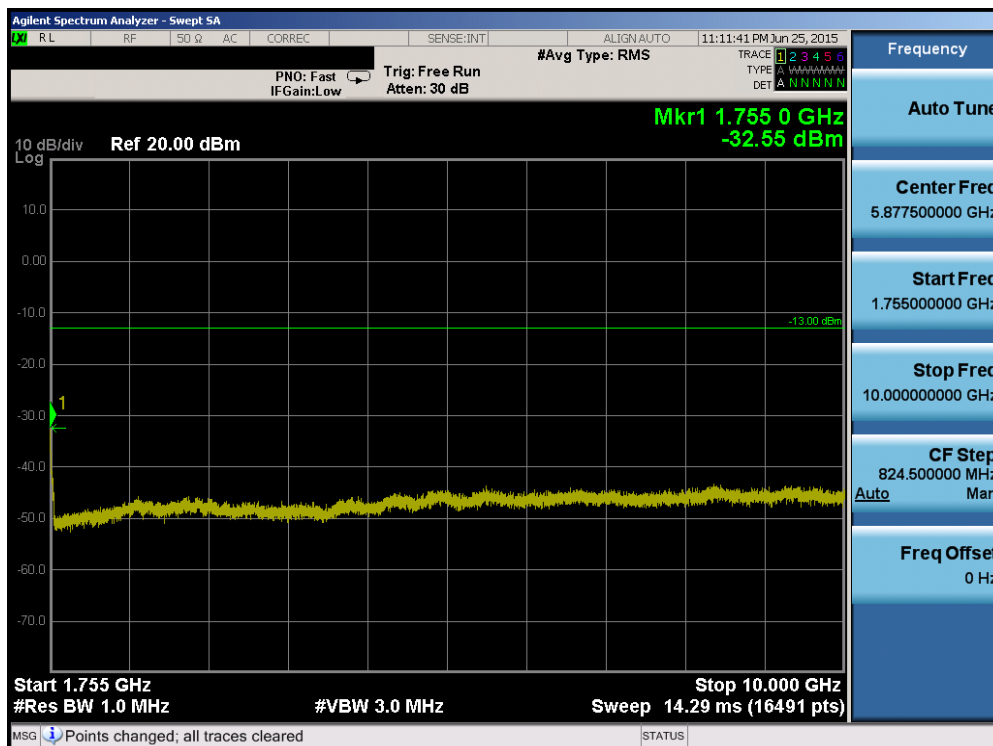
Plot 6-82. Conducted Spurious Plot (Band 4 – 20.0MHz QPSK – RB Size 1, RB Offset 0 – Mid Channel)
