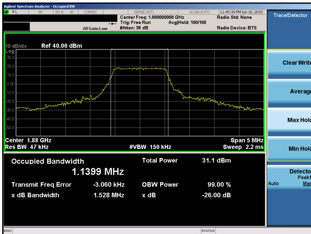
Plot 6-32. Occupied Bandwidth Plot (Band 2 – 1.4MHz 16-QAM – RB Size 6)
