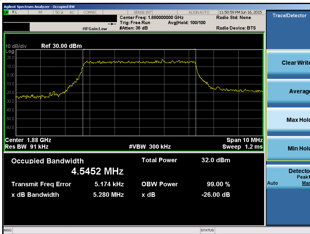
Plot 6-35. Occupied Bandwidth Plot (Band 2 – 5.0MHz QPSK – RB Size 25)
