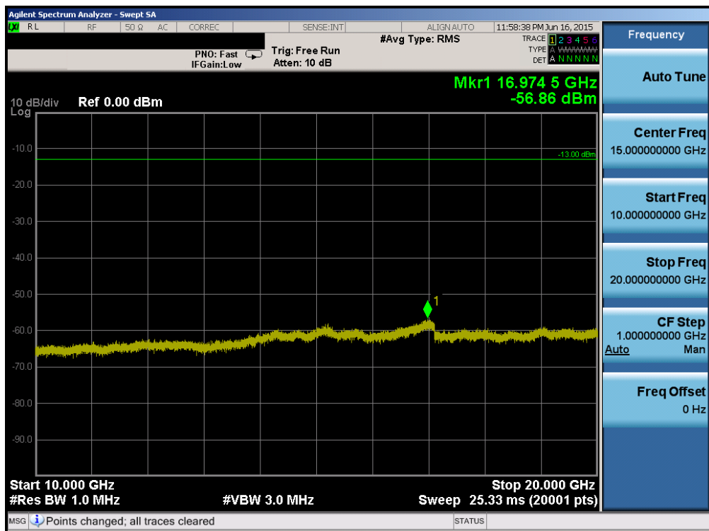
Plot 6-92. Conducted Spurious Plot (Band 2 – 20.0MHz QPSK – RB Size 1, RB Offset 0 – Mid Channel)
