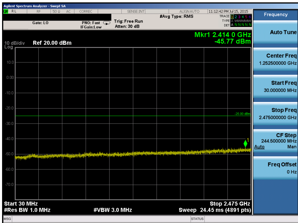
Plot 6-96. Conducted Spurious Plot (Band 41 – 15.0MHz QPSK – RB Size 1, RB Offset 0 – Low Channel)
