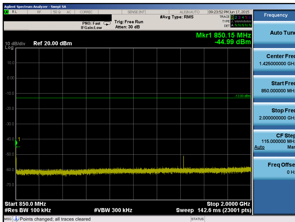
Plot 6-76. Conducted Spurious Plot (Band 26 – 15.0MHz QPSK – RB Size 1, RB Offset 0 – High Channel)
