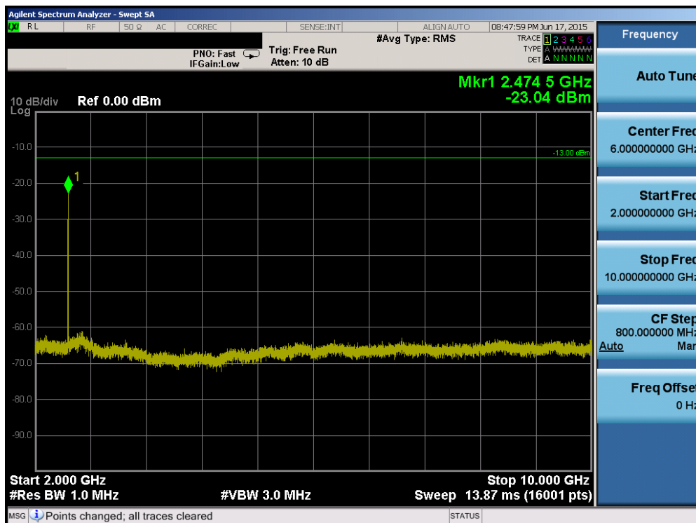
Plot 6-62. Conducted Spurious Plot (Band 5 – 10.0MHz QPSK – RB Size 1, RB Offset 0 – Low Channel)
