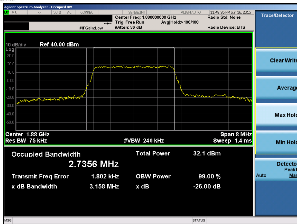
Plot 6-33. Occupied Bandwidth Plot (Band 2 – 3.0MHz QPSK – RB Size 15)
