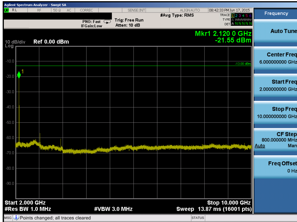
Plot 6-59. Conducted Spurious Plot (Band 12/17 – 10.0MHz QPSK – RB Size 1, RB Offset 0 – High Channel)
