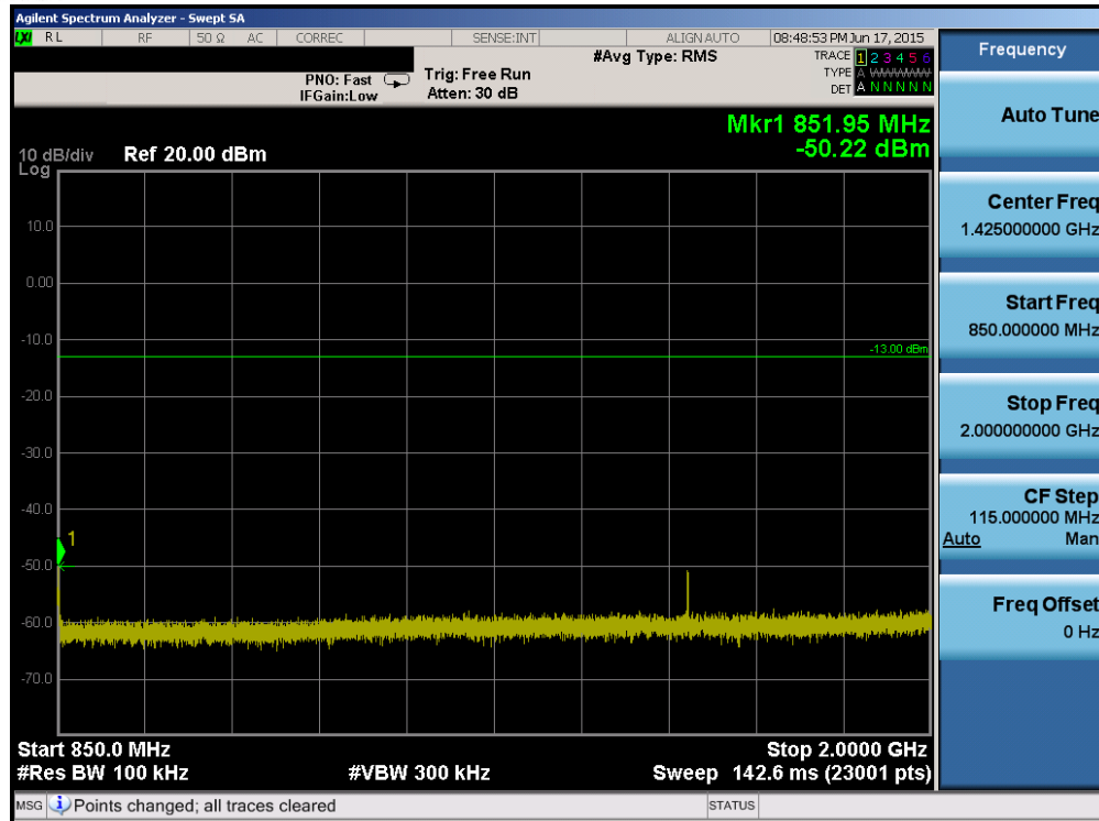
Plot 6-67. Conducted Spurious Plot (Band 5 – 10.0MHz QPSK – RB Size 1, RB Offset 0 – High Channel)
