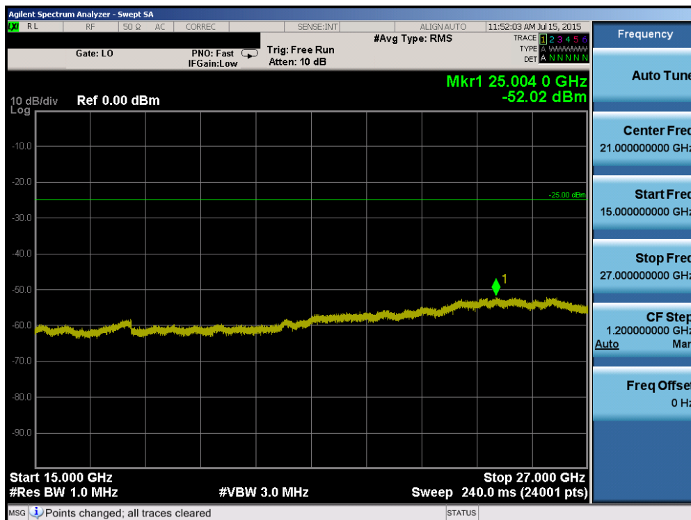
Plot 6-104. Conducted Spurious Plot (Band 41 – 15.0MHz QPSK – RB Size 1, RB Offset 0 – High Channel)
