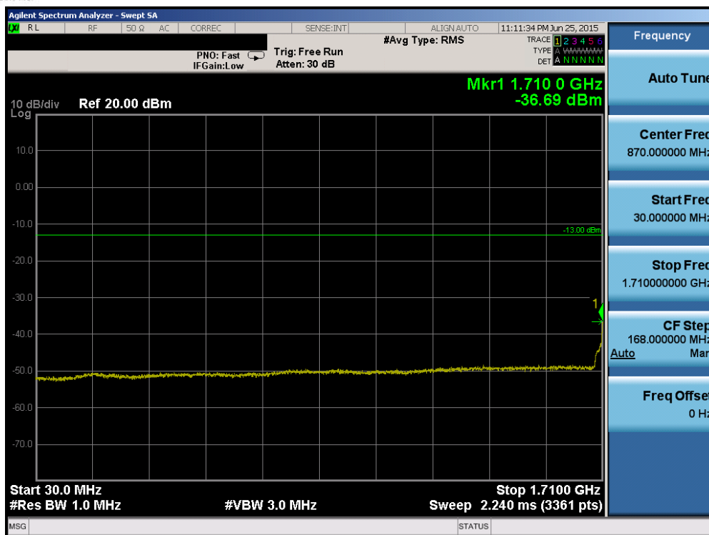
Plot 6-81. Conducted Spurious Plot (Band 4 – 20.0MHz QPSK – RB Size 1, RB Offset 0 – Mid Channel)
