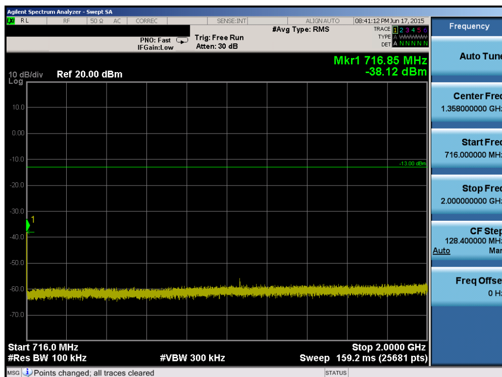
Plot 6-52. Conducted Spurious Plot (Band 12/17 – 10.0MHz QPSK – RB Size 1, RB Offset 0 – Low Channel)
