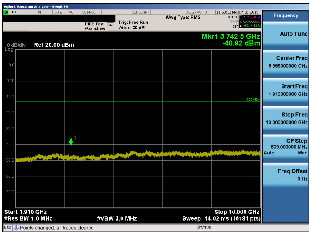
Plot 6-91. Conducted Spurious Plot (Band 2 – 20.0MHz QPSK – RB Size 1, RB Offset 0 – Mid Channel)
