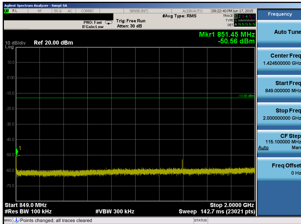
Plot 6-70. Conducted Spurious Plot (Band 26 – 15.0MHz QPSK – RB Size 1, RB Offset 0 – Low Channel)
