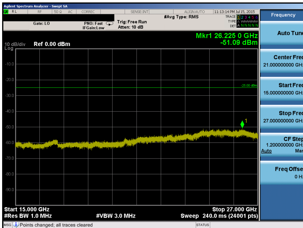
Plot 6-98. Conducted Spurious Plot (Band 41 – 15.0MHz QPSK – RB Size 1, RB Offset 0 – Low Channel)
