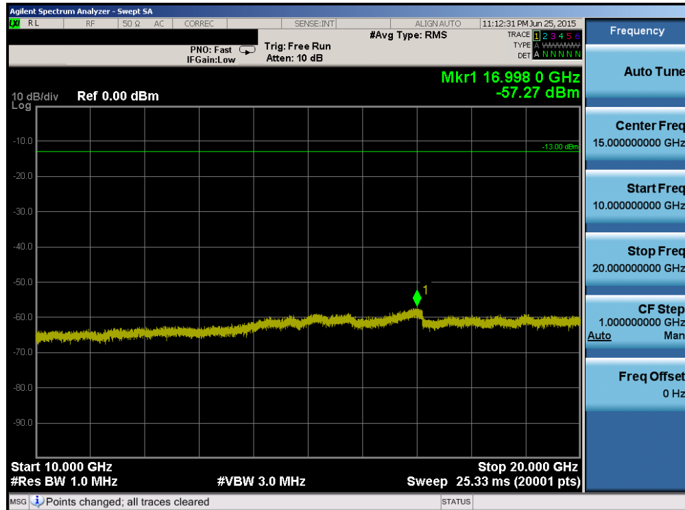
Plot 6-80. Conducted Spurious Plot (Band 4 – 20.0MHz QPSK – RB Size 1, RB Offset 0 – Low Channel)
