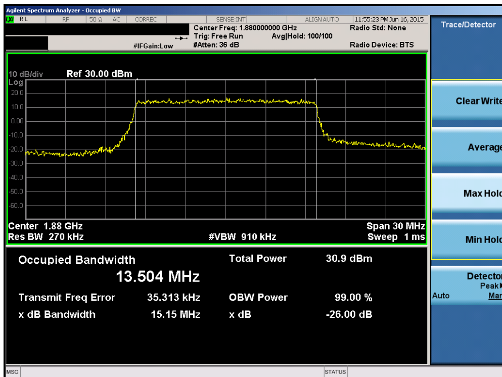
Plot 6-40. Occupied Bandwidth Plot (Band 2 – 15.0MHz 16-QAM – RB Size 75)
