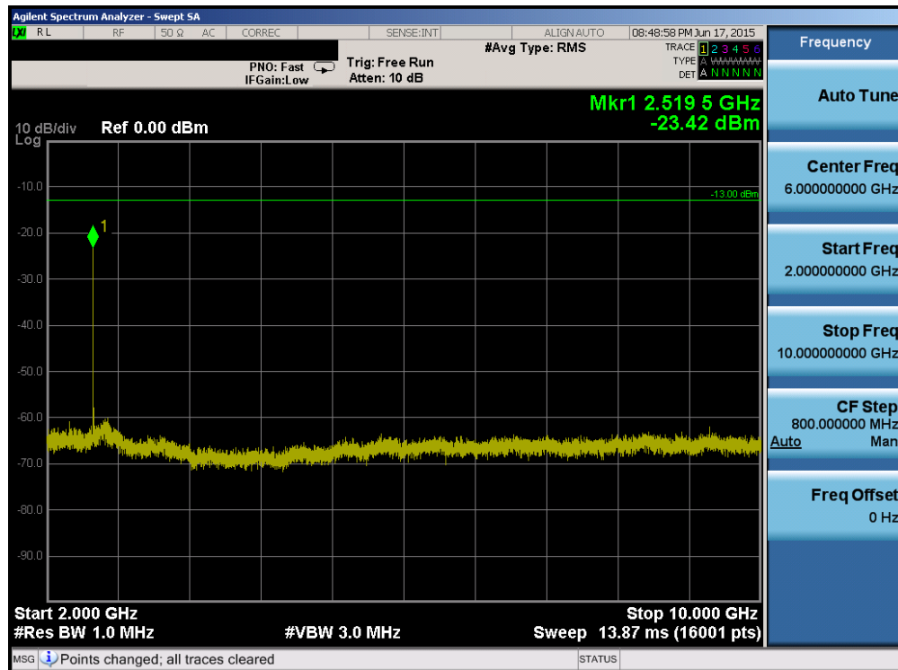
Plot 6-68. Conducted Spurious Plot (Band 5 – 10.0MHz QPSK – RB Size 1, RB Offset 0 – High Channel)
