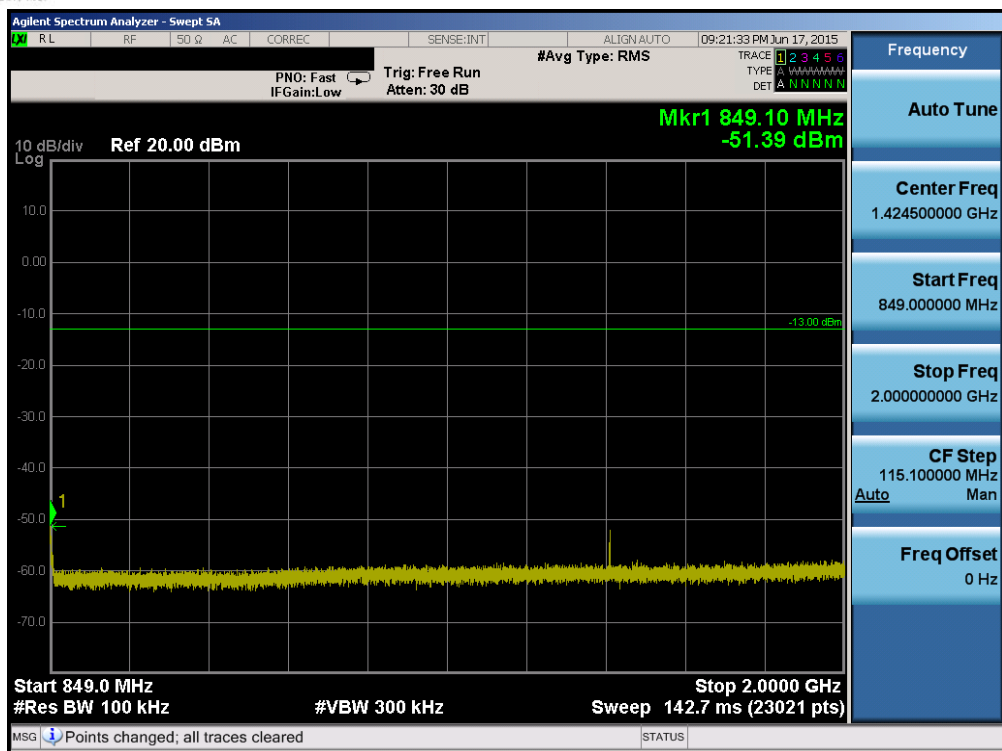
Plot 6-73. Conducted Spurious Plot (Band 26 – 15.0MHz QPSK – RB Size 1, RB Offset 0 – Mid Channel)
