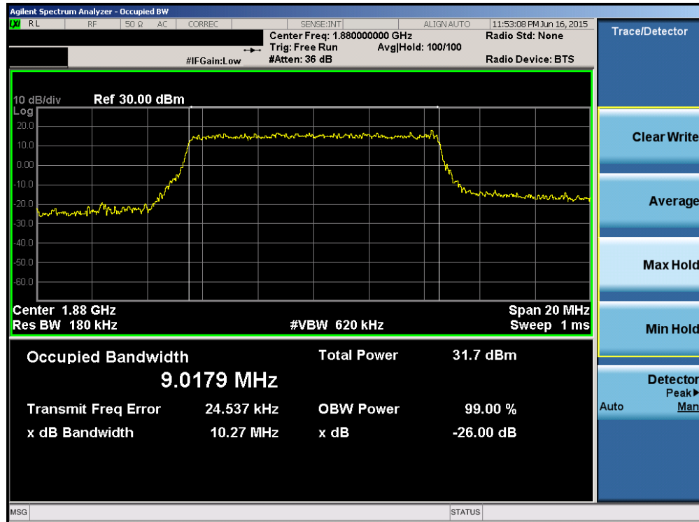
Plot 6-37. Occupied Bandwidth Plot (Band 2 – 10.0MHz QPSK – RB Size 50)
