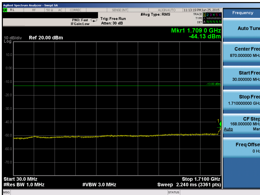
Plot 6-84. Conducted Spurious Plot (Band 4 - 20.0MHz QPSK - RB Size 1, RB Offset 0 - High Channel)
