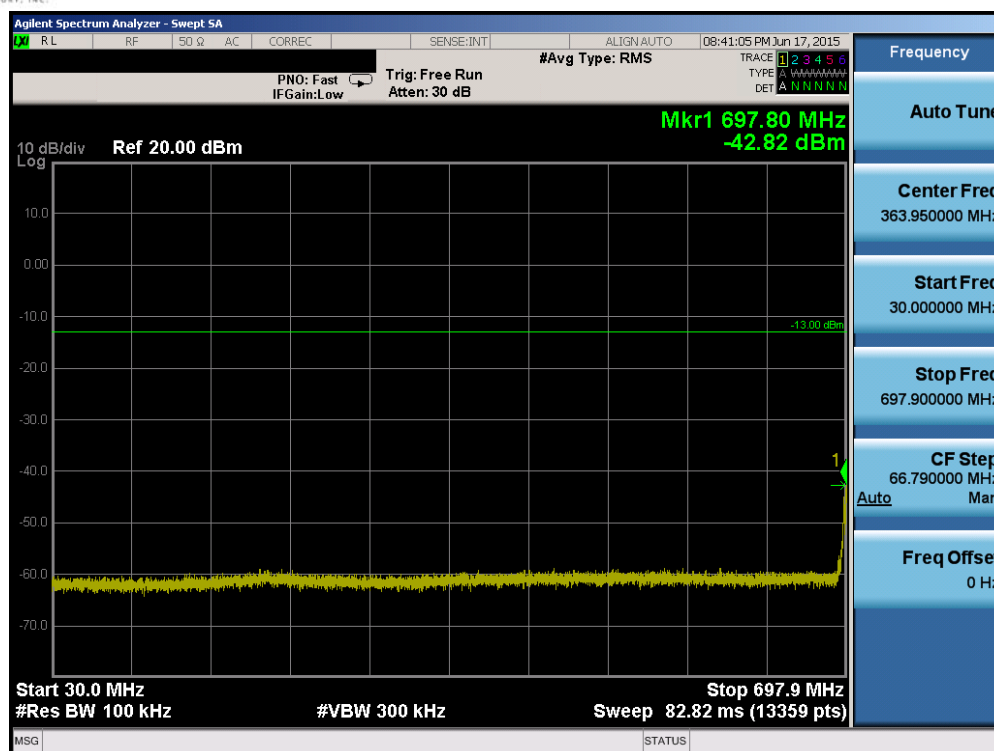
Plot 6-51. Conducted Spurious Plot (Band 12/17 – 10.0MHz QPSK – RB Size 1, RB Offset 0– Low Channel)
