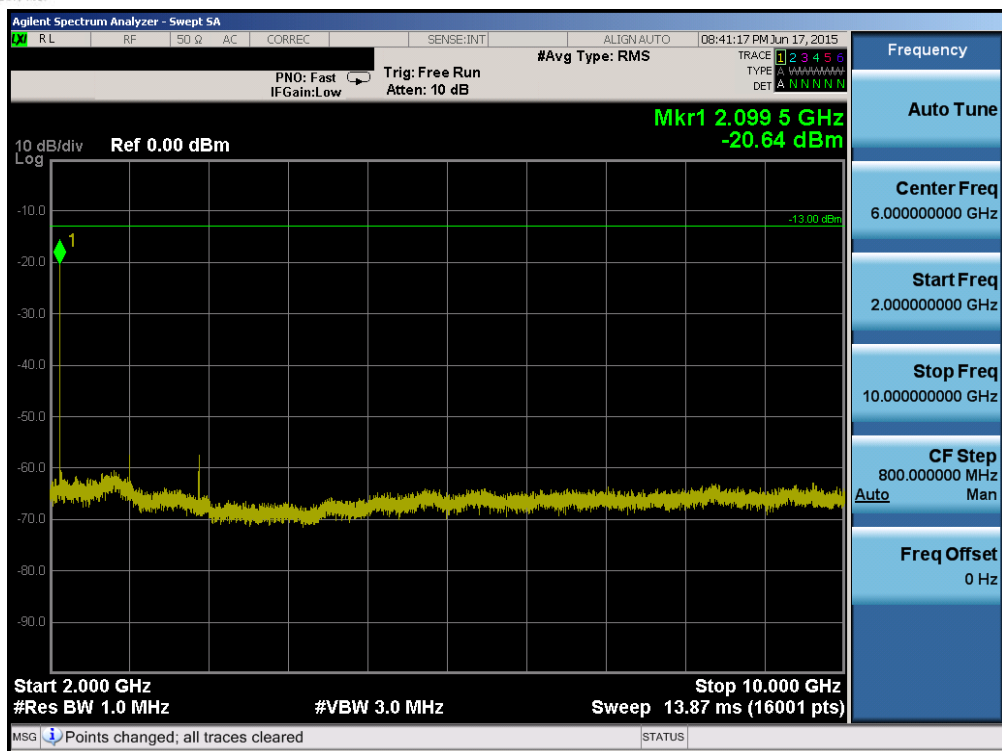
Plot 6-53. Conducted Spurious Plot (Band 12/17 – 10.0MHz QPSK – RB Size 1, RB Offset 0 – Low Channel)
