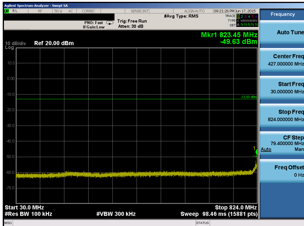
Plot 6-72. Conducted Spurious Plot (Band 26 – 15.0MHz QPSK – RB Size 1, RB Offset 0 – Mid Channel)
