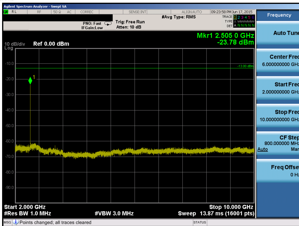
Plot 6-77. Conducted Spurious Plot (Band 26 – 15.0MHz QPSK – RB Size 1, RB Offset 0 – High Channel)
