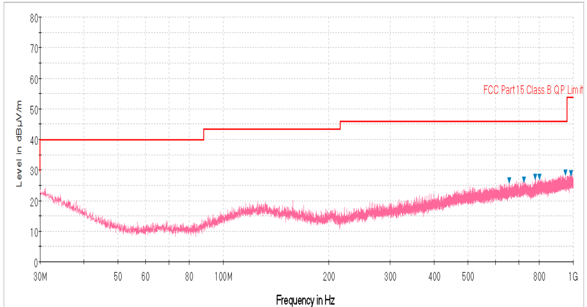
Plot 6-52. Radiated Spurious Plot below 1GHz (Pol. H)
