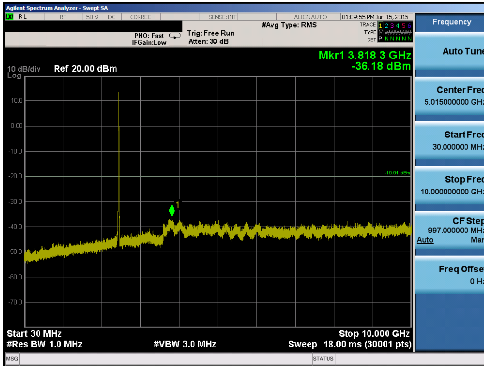
Plot 6-65. Conducted Spurious Plot (802.11b – Ch. 11)
