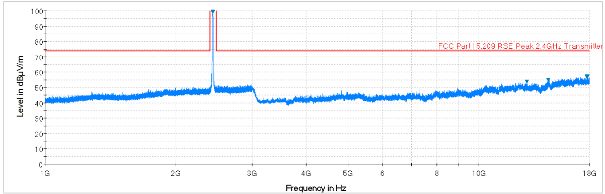
Plot 6-78. Radiated Spurious Plot above 1GHz (802.11b – Ch. 6, Ant. Pol. V)
