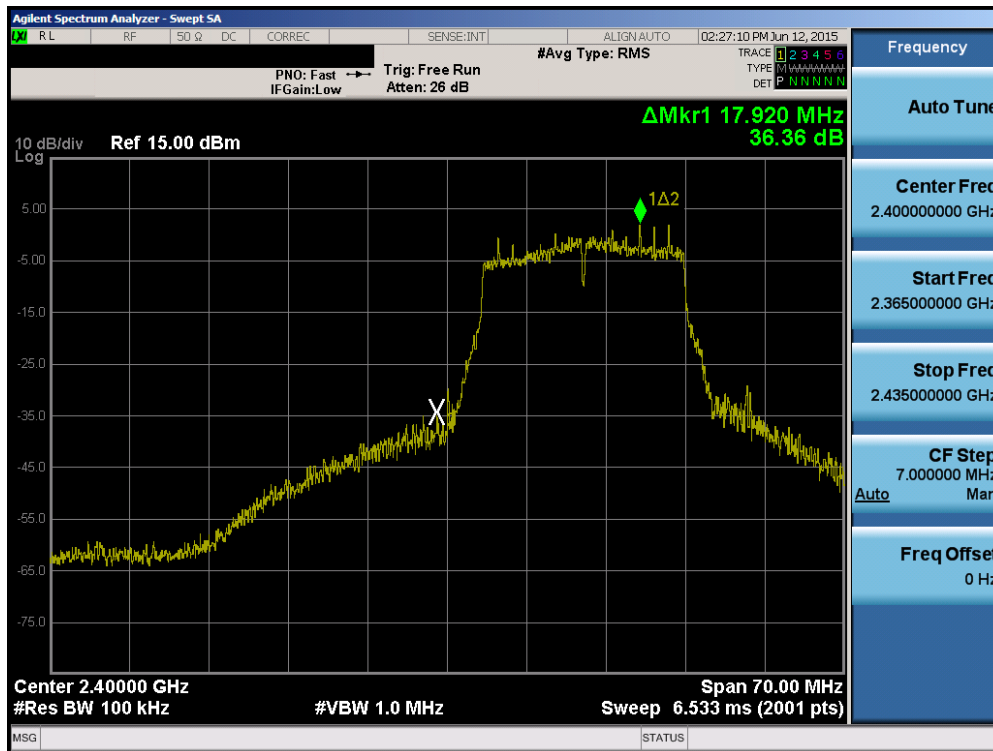
Plot 6-43. Band Edge Plot (802.11n (2.4GHz) – Ch. 1)
