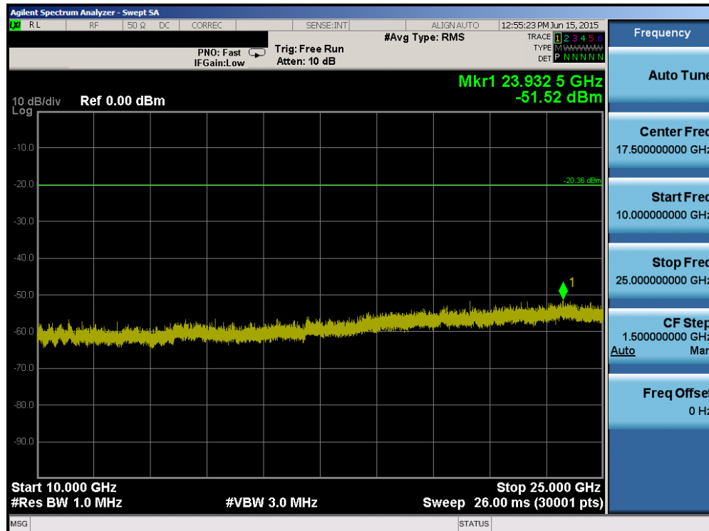
Plot 6-62. Conducted Spurious Plot (802.11b – Ch. 1)
