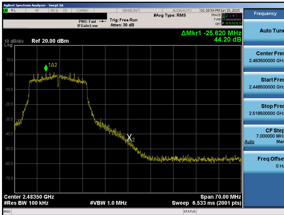
Plot 6-53. Band Edge Plot (802.11n (2.4GHz) – Ch. 11)
