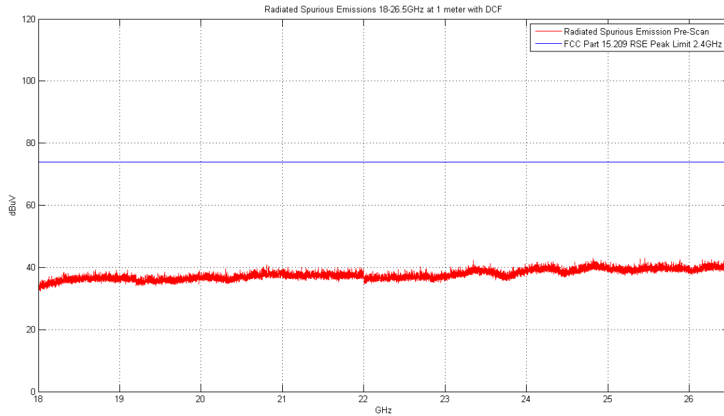
Plot 6-73. Radiated Spurious Plot above 18GHz (Pol. H)
