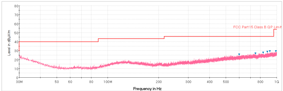
Plot 6-97. Radiated Spurious Plot below 1GHz (Pol. H)
