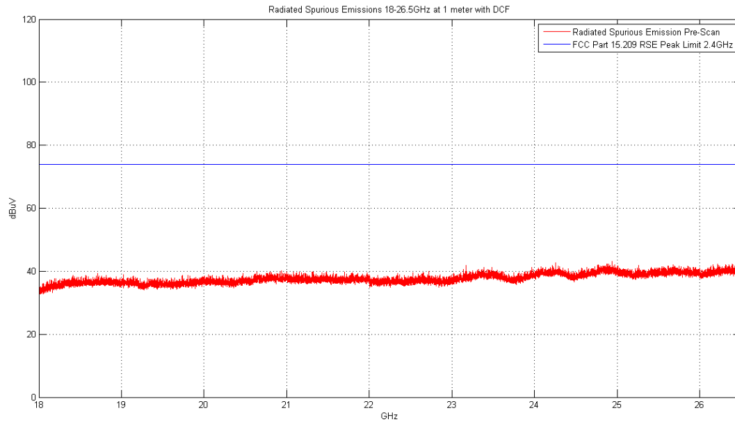
Plot 6-81. Radiated Spurious Plot above 18GHz (Pol. H)
