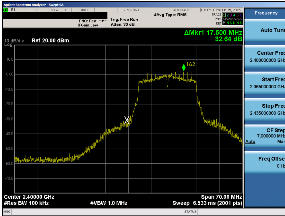
Plot 6-52. Band Edge Plot (802.11n (2.4GHz) – Ch. 1)
