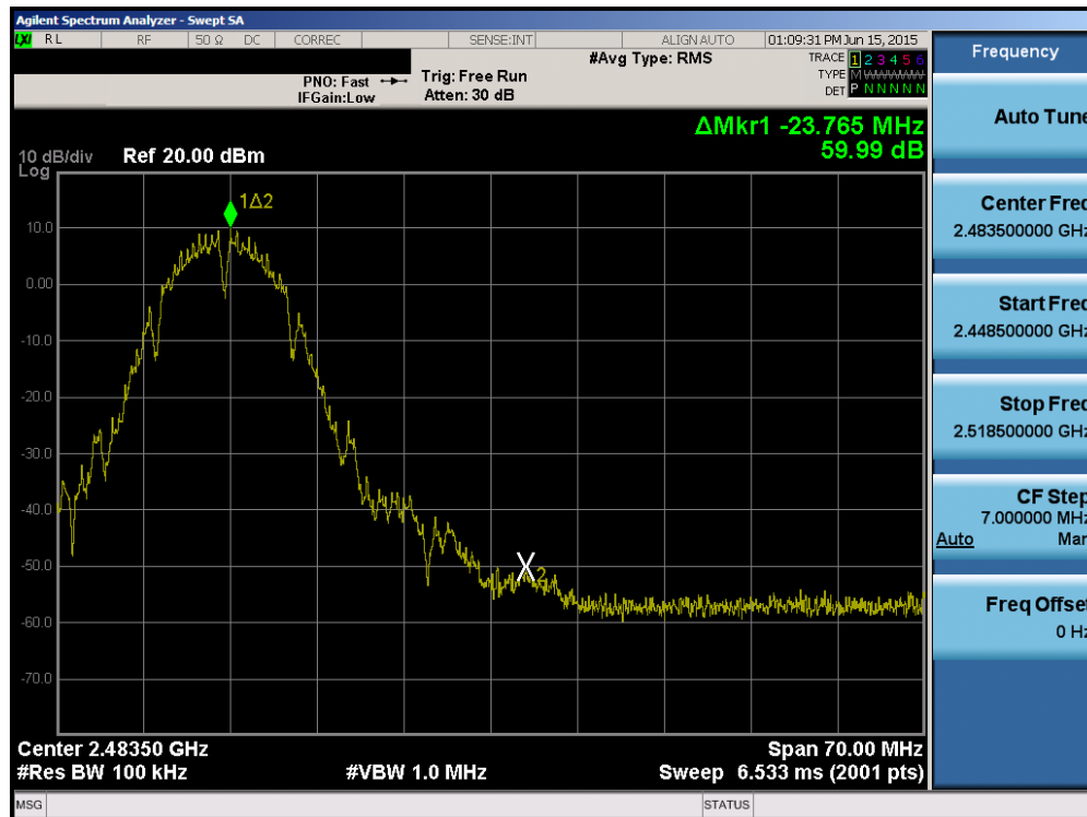
Plot 6-47. Band Edge Plot (802.11b – Ch. 11)
