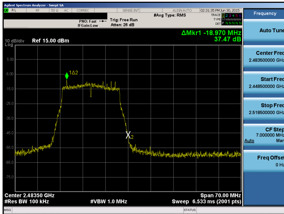
Plot 6-45. Band Edge Plot (802.11n (2.4GHz) – Ch. 13)
