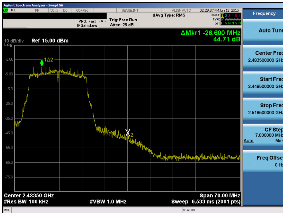
Plot 6-44. Band Edge Plot (802.11n (2.4GHz) – Ch. 11)
