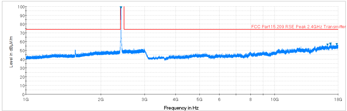
Plot 6-75. Radiated Spurious Plot above 1GHz (802.11b – Ch. 1, Ant. Pol. H)
