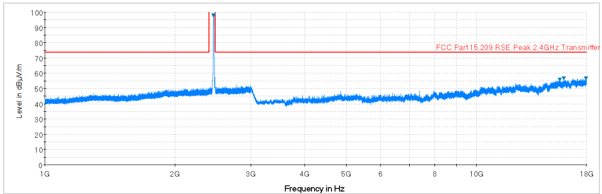
Plot 6-72. Radiated Spurious Plot above 1GHz (802.11b – Ch. 11, Ant. Pol. V)
