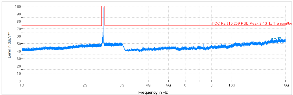
Plot 6-77. Radiated Spurious Plot above 1GHz (802.11b – Ch. 6, Ant. Pol. H)
