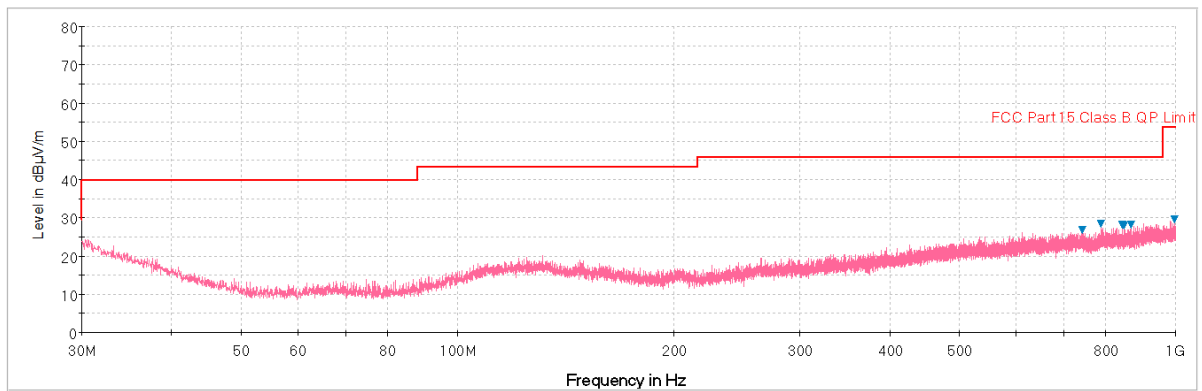
Plot 6-96. Radiated Spurious Plot below 1GHz (Pol. V)
