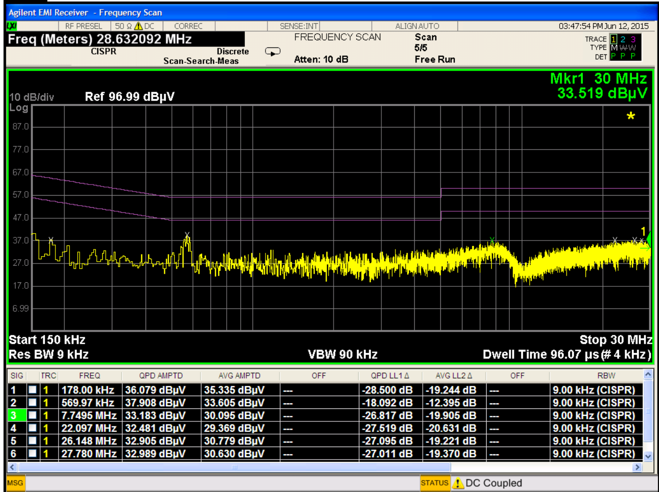
Plot 6-99. Line Conducted Plot with 802.11b (L1)
