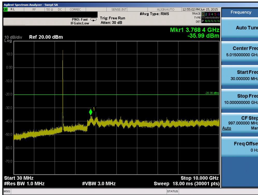
Plot 6-61. Conducted Spurious Plot (802.11b – Ch. 1)
