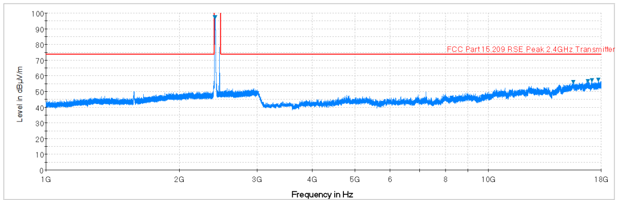
Plot 6-76. Radiated Spurious Plot above 1GHz (802.11b – Ch. 1, Ant. Pol. V)
