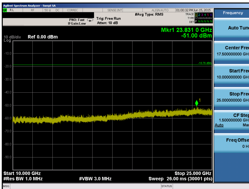
Plot 6-64. Conducted Spurious Plot (802.11b – Ch. 6)
