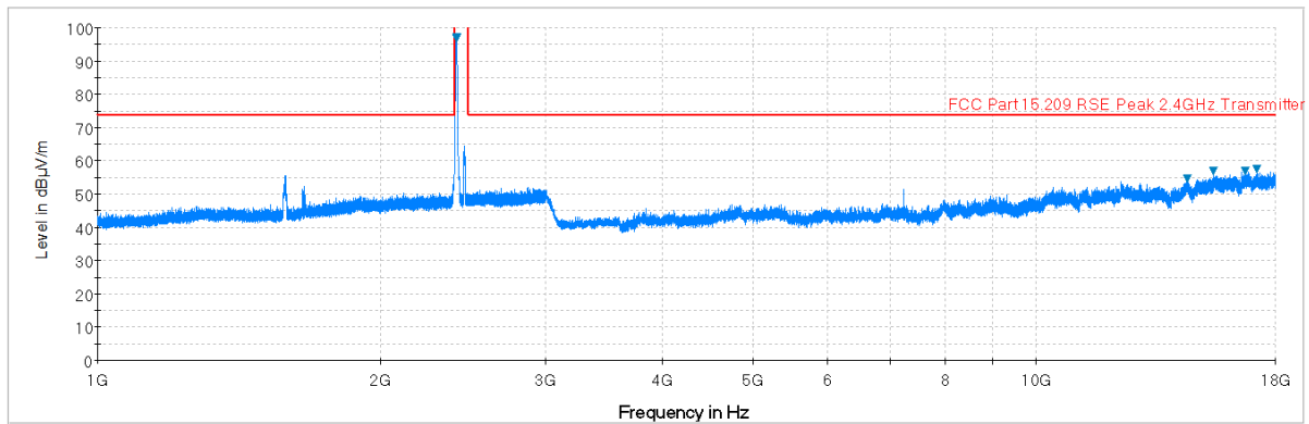
Plot 6-68. Radiated Spurious Plot above 1GHz (802.11b – Ch. 1, Ant. Pol. V)
