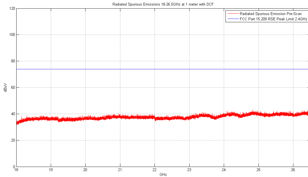
Plot 6-82. Radiated Spurious Plot above 18GHz (Pol. V)
