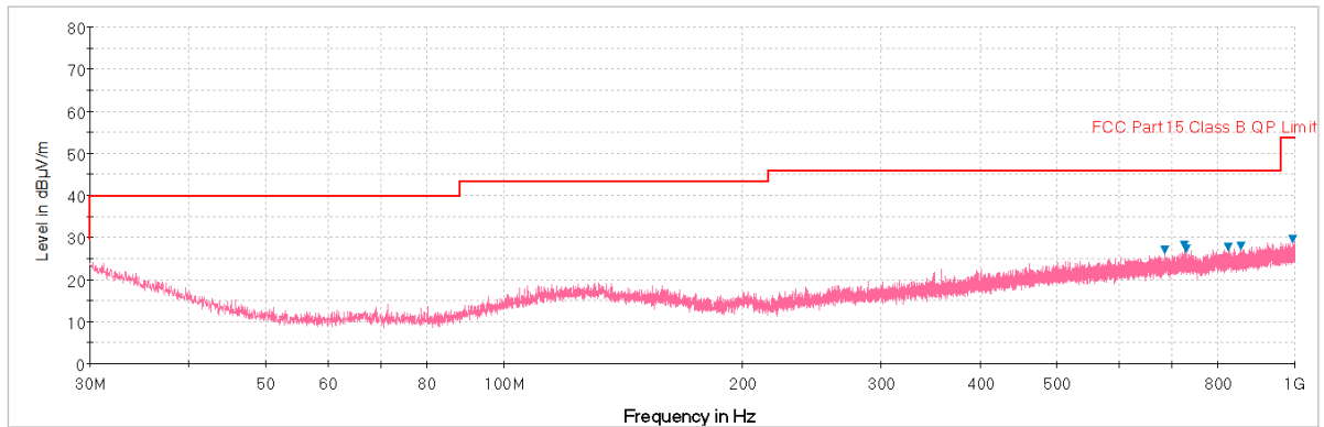
Plot 6-95. Radiated Spurious Plot below 1GHz (Pol. H)
