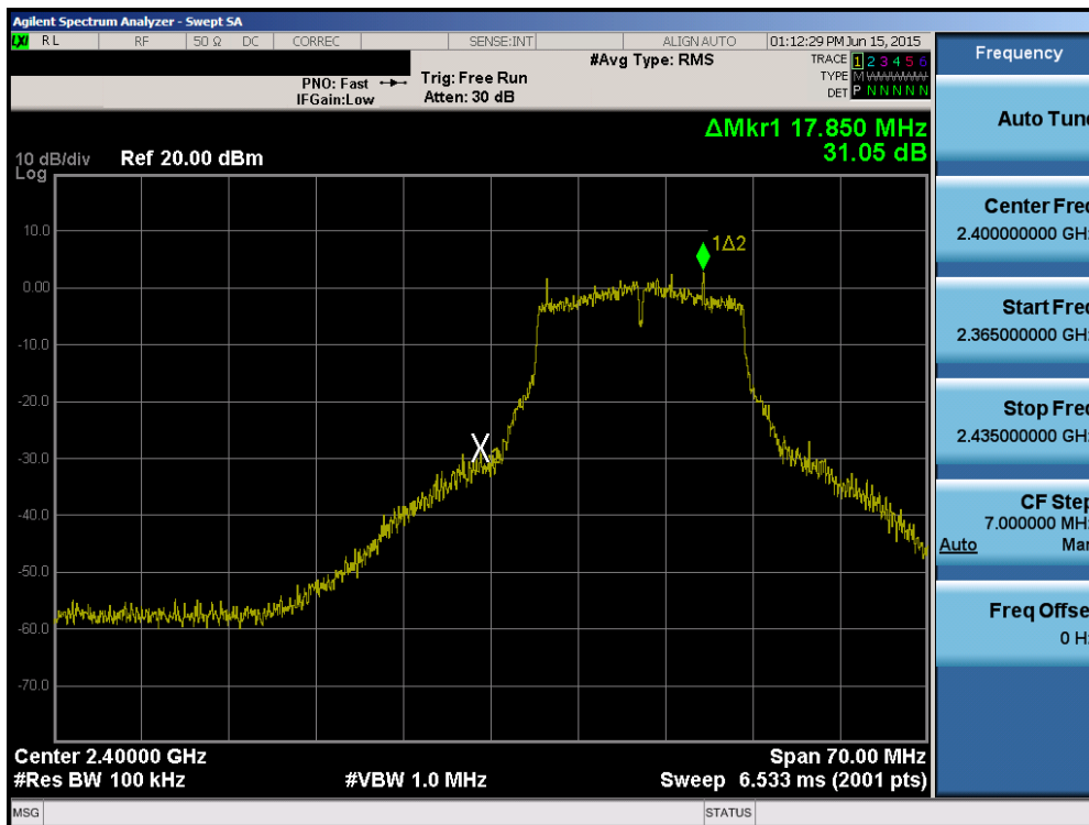
Plot 6-49. Band Edge Plot (802.11g – Ch. 1)
