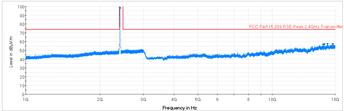
Plot 6-67. Radiated Spurious Plot above 1GHz (802.11b – Ch. 1, Ant. Pol. H)
