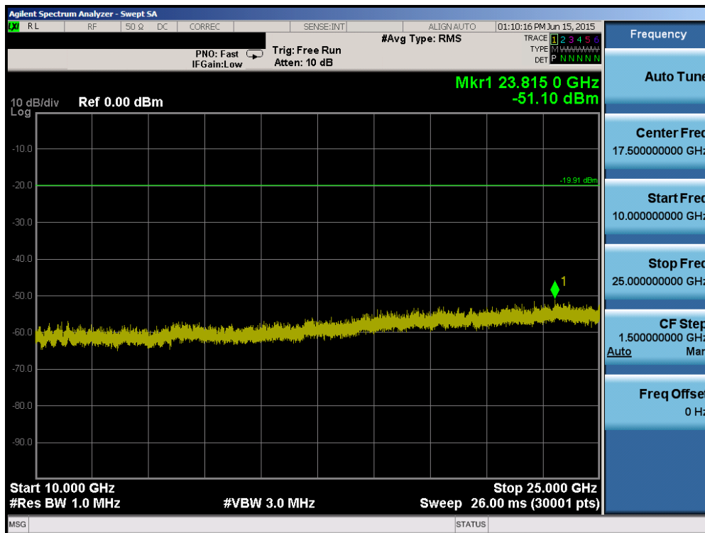
Plot 6-66. Conducted Spurious Plot (802.11b – Ch. 11)
