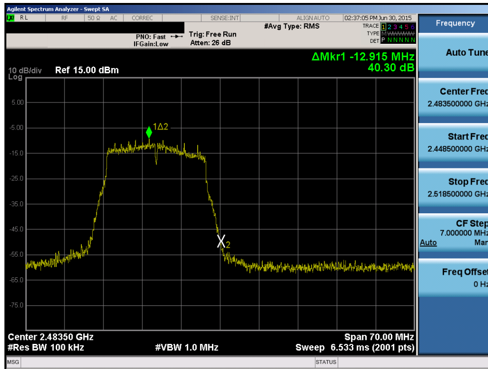
Plot 6-54. Band Edge Plot (802.11n (2.4GHz) – Ch. 13)
