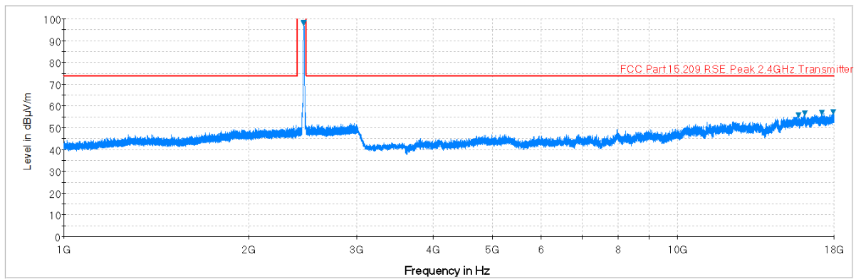
Plot 6-71. Radiated Spurious Plot above 1GHz (802.11b – Ch. 11, Ant. Pol. H)
