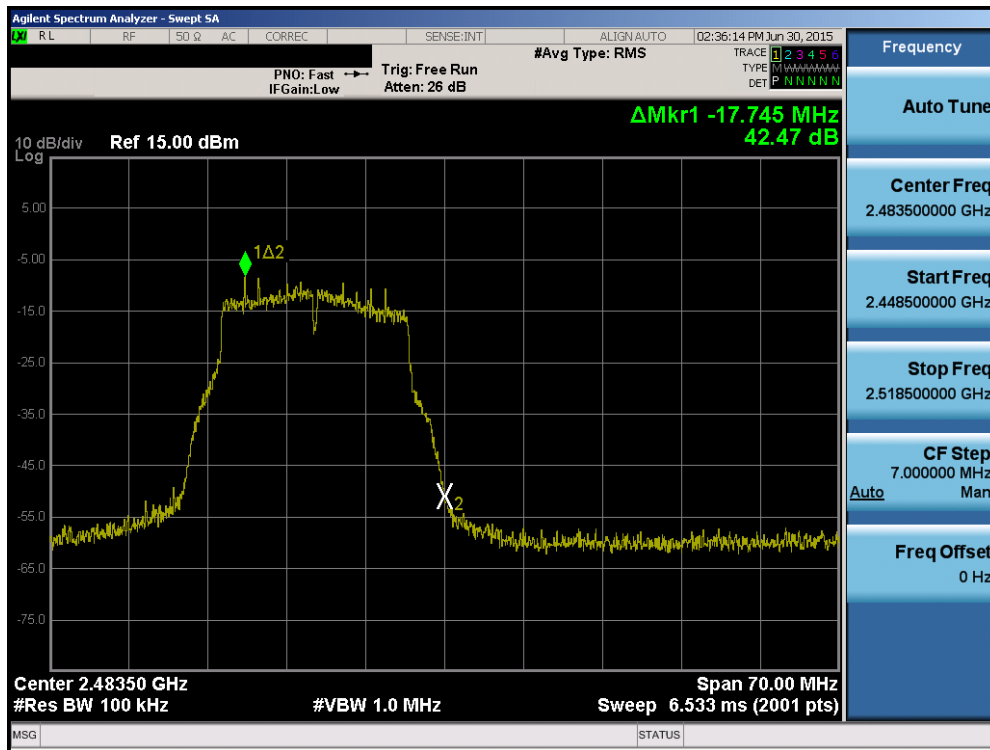
Plot 6-51. Band Edge Plot (802.11g – Ch. 13)
