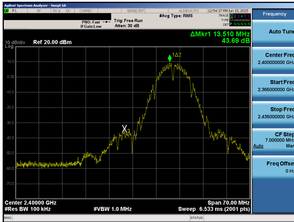
Plot 6-46. Band Edge Plot (802.11b – Ch. 1)
