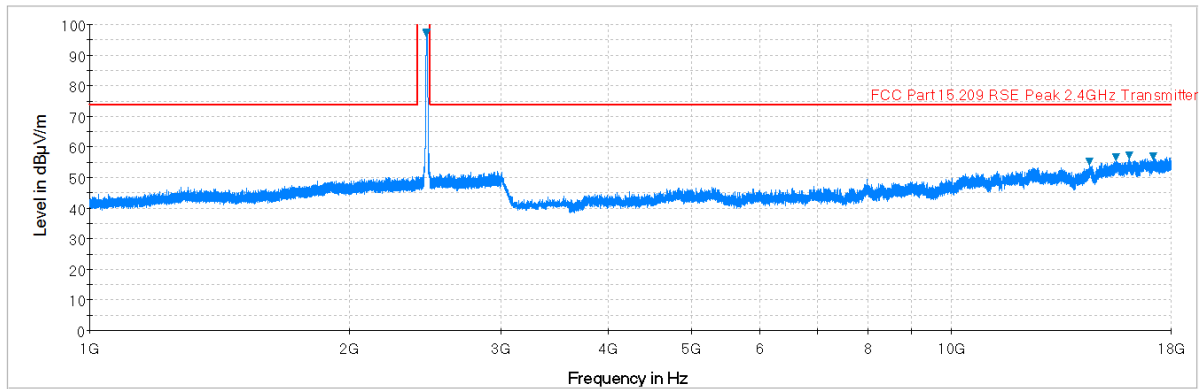
Plot 6-80. Radiated Spurious Plot above 1GHz (802.11b – Ch. 11, Ant. Pol. V)
