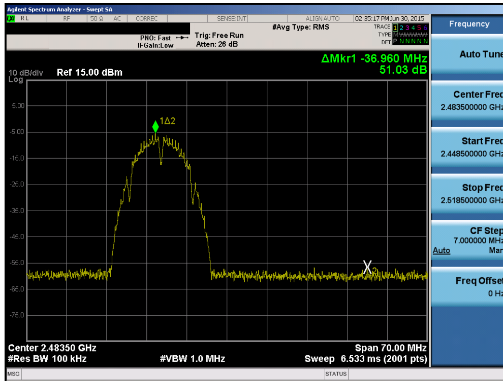
Plot 6-48. Band Edge Plot (802.1b – Ch. 13)
