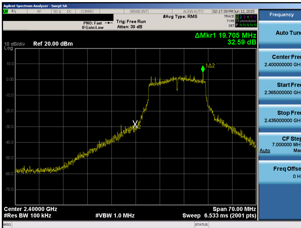
Plot 6-40. Band Edge Plot (802.11g– Ch. 1)
