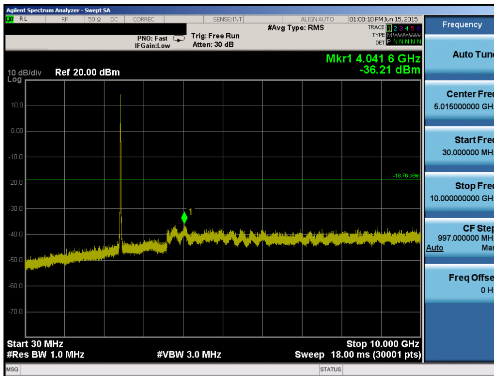
Plot 6-63. Conducted Spurious Plot (802.11b – Ch. 6)
