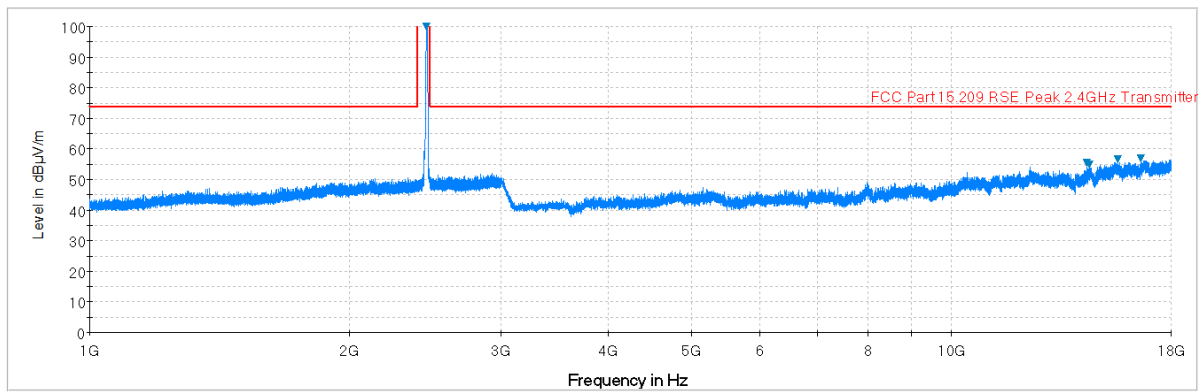
Plot 6-79. Radiated Spurious Plot above 1GHz (802.11b – Ch. 11, Ant. Pol. H)
