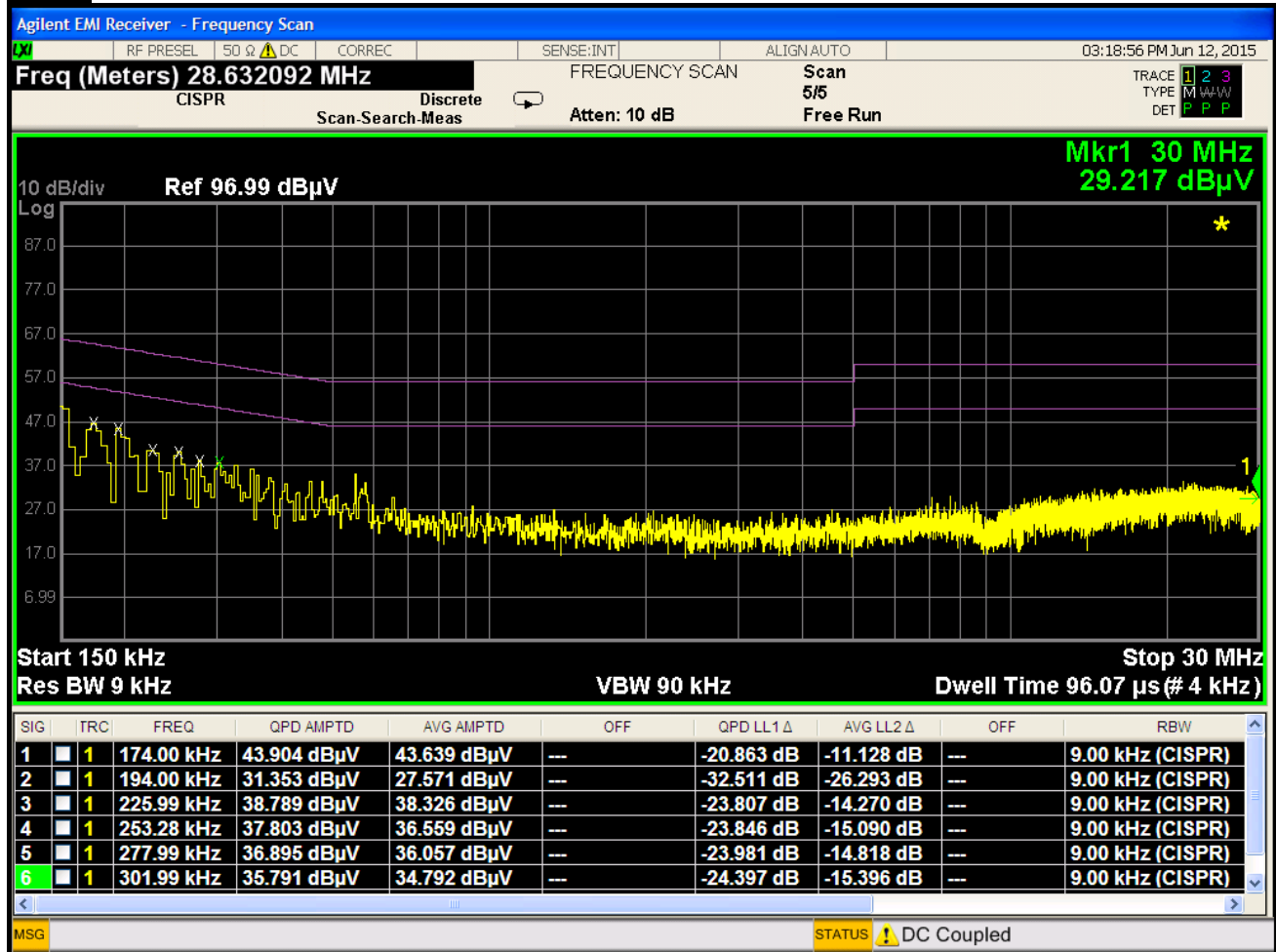
Plot 6-100. Line Conducted Plot with 802.11b (N)
