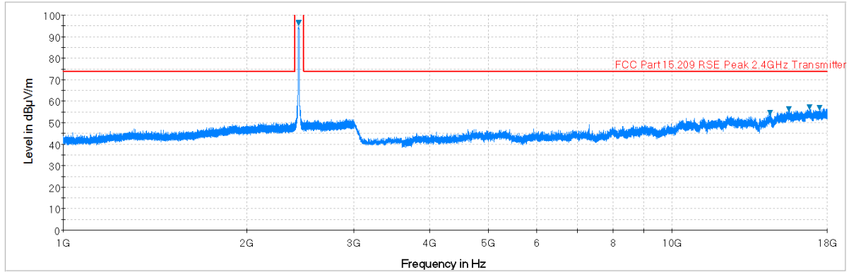
Plot 6-70. Radiated Spurious Plot above 1GHz (802.11b – Ch. 6, Ant. Pol. V)
