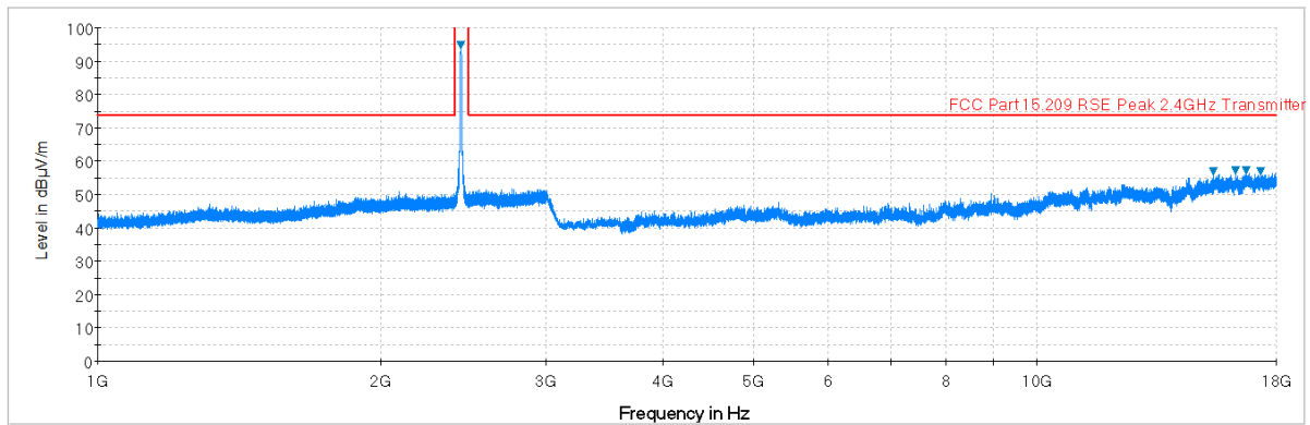
Plot 6-69. Radiated Spurious Plot above 1GHz (802.11b – Ch. 6, Ant. Pol. H)
