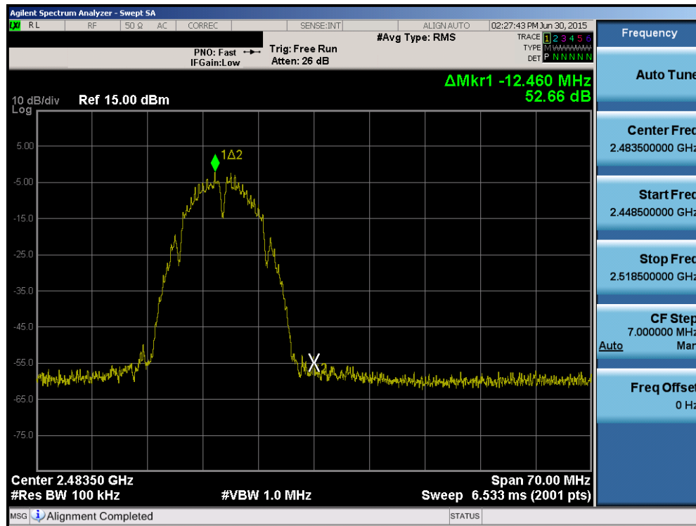
Plot 6-39. Band Edge Plot (802.11b – Ch. 13)
