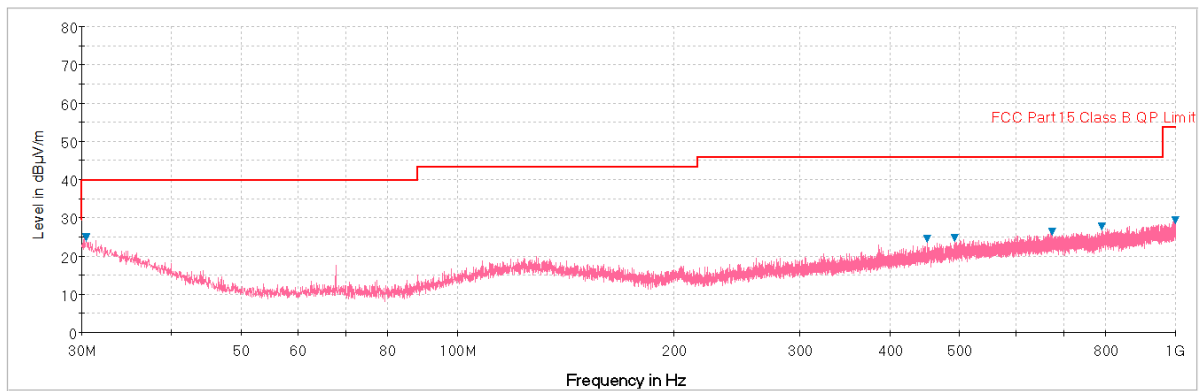
Plot 6-98. Radiated Spurious Plot below 1GHz (Pol. V)
