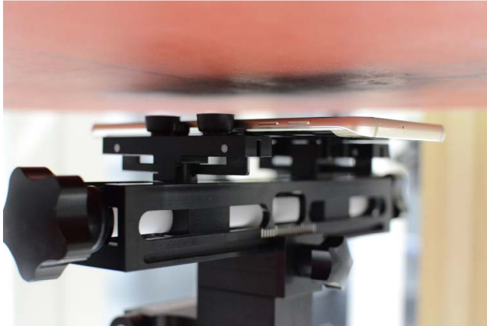
SAR Test Setup Photo 7– Back Side at 1.5 cm (Body-Worn)
