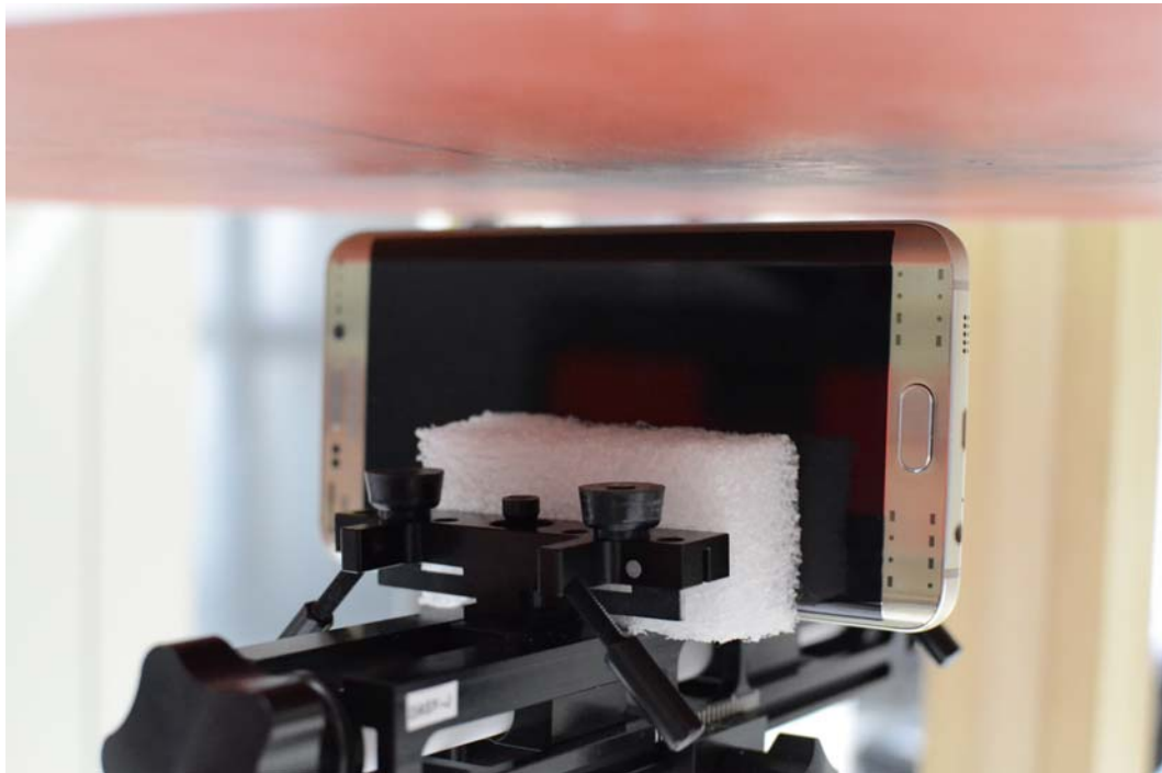
SAR Test Setup Photo 14 – Right Edge at 1.0 cm (Hotspot)
