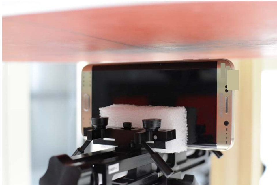
SAR Test Setup Photo 16 – Left Edge at 1.0 cm (Hotspot)
