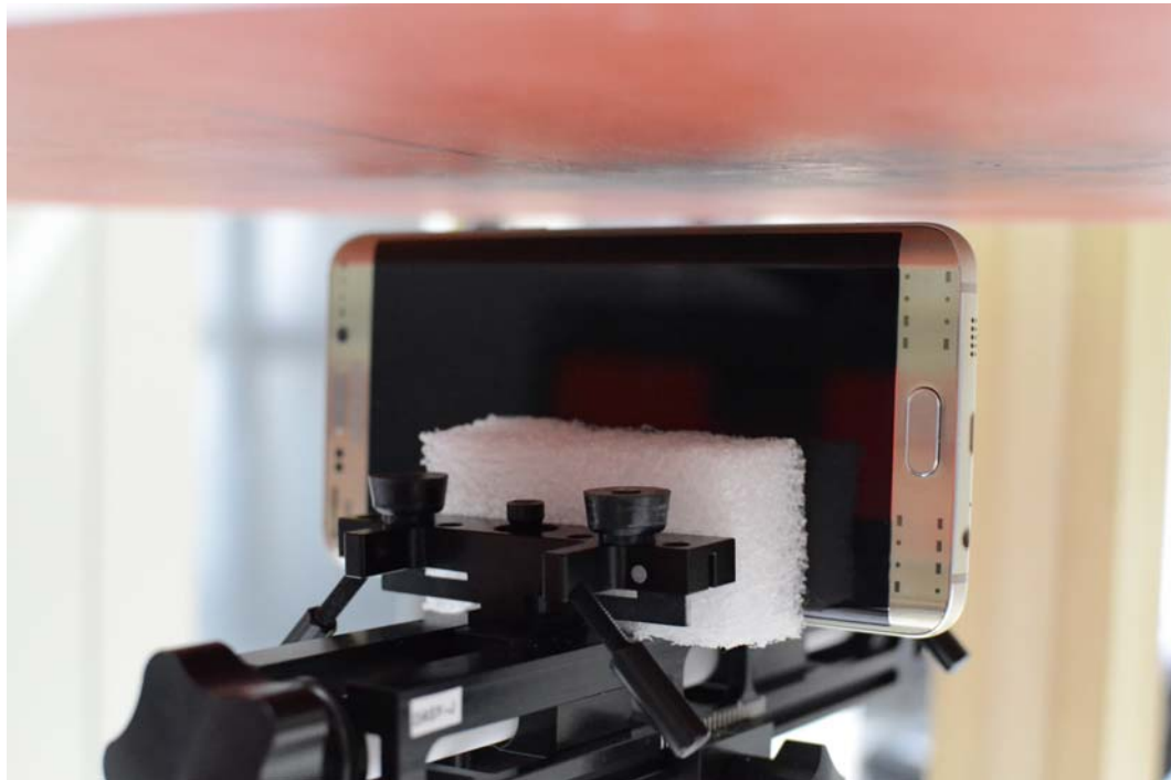
SAR Test Setup Photo 18 – Right Edge at 1.0 cm (Hotspot)
