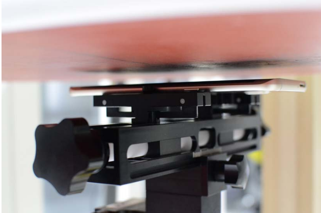
SAR Test Setup Photo 11- Front Side at 1.0 cm (Hotspot)
