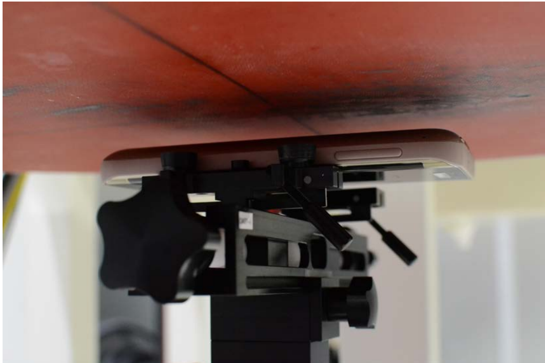
SAR Test Setup Photo 6 – Back Side at 1.5 cm (Body-worn)
