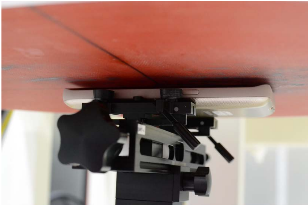
SAR Test Setup Photo 8 - Front Side at 0.4 cm (Phablet)
