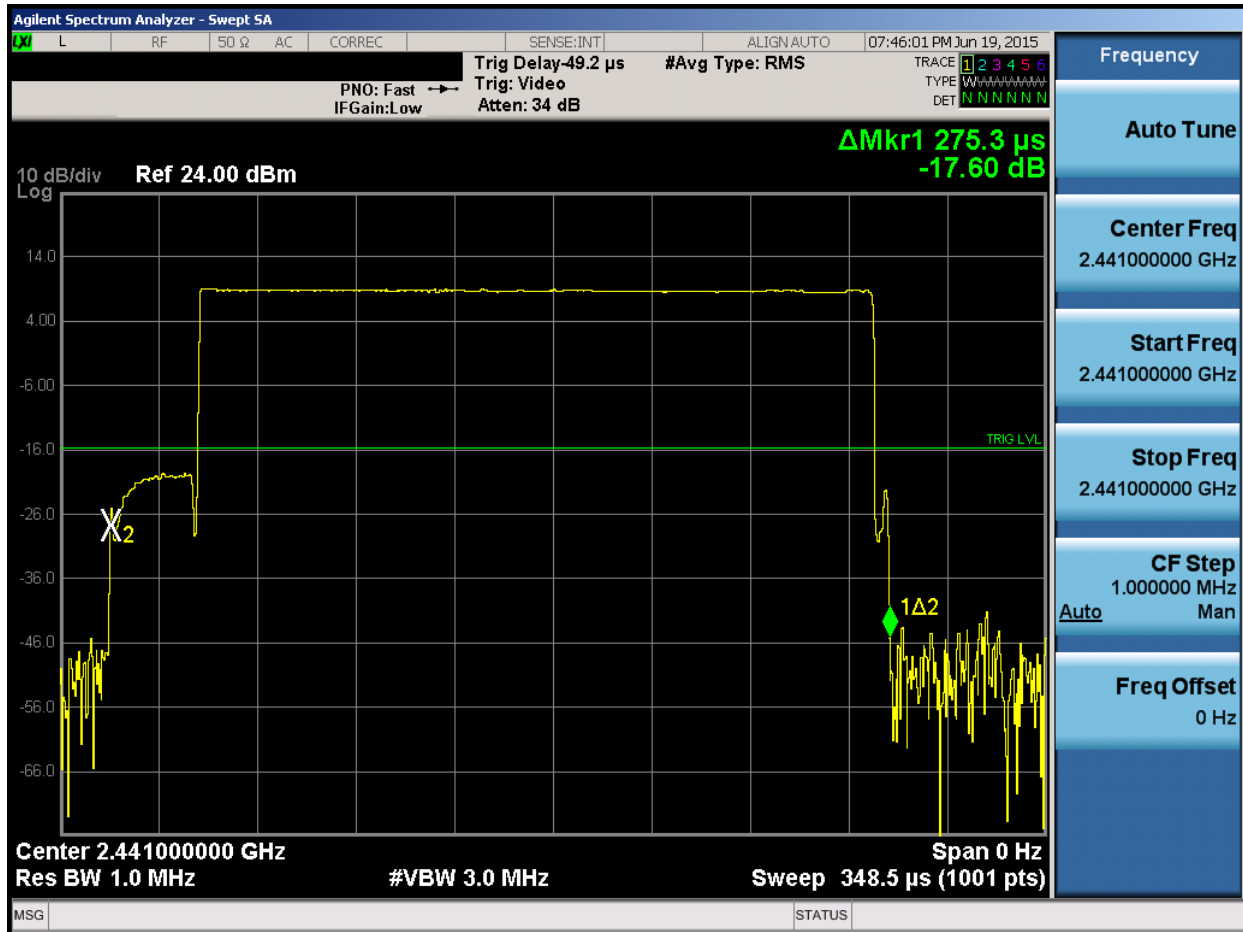
Plot 6-2. Pulse Width Measurement
