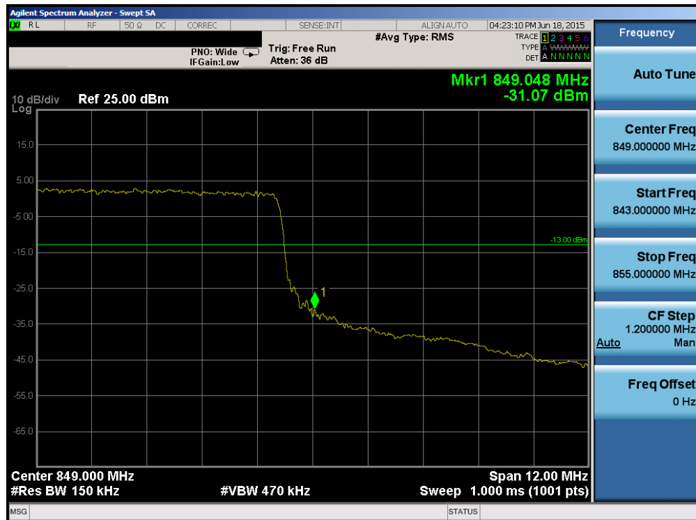
Plot 6-108. Upper Band Edge Plot (Band 26 – 15.0MHz QPSK – RB Size 75)
