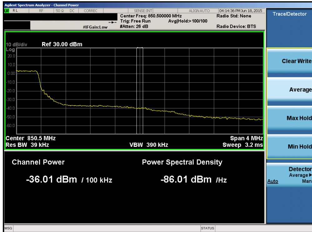
Plot 6-100. Upper Extended Band Edge Plot (Band 5/26 – 3.0MHz QPSK – RB Size 15)
