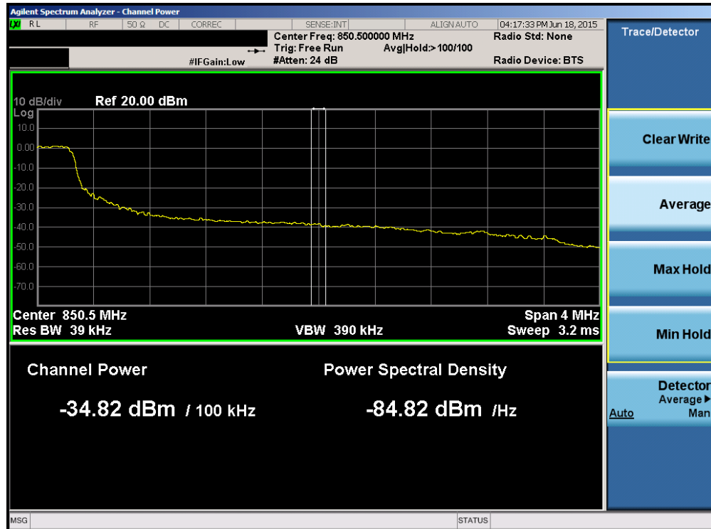
Plot 6-104. Upper Extended Band Edge Plot (Band 5/26 – 5.0MHz QPSK – RB Size 25)
