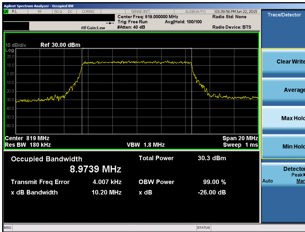
Plot 7-23. Occupied Bandwidth Plot (10MHz QPSK – RB Size 50)
