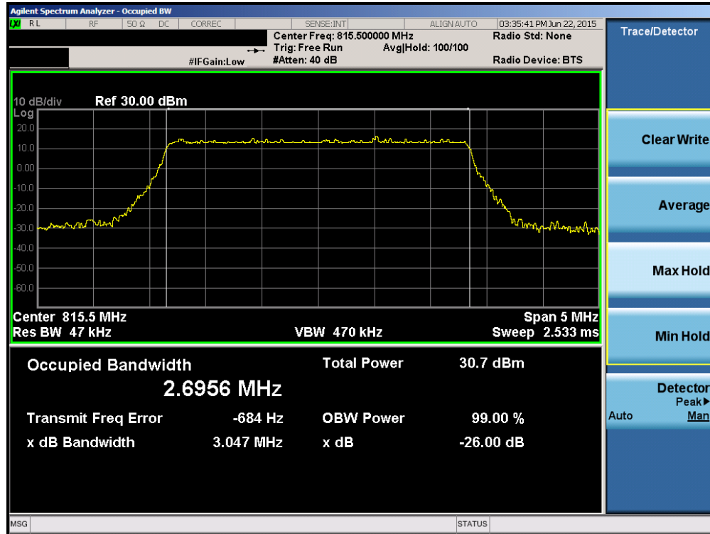
Plot 7-12. Occupied Bandwidth Plot (3MHz QPSK – RB Size 15– Low Channel)
