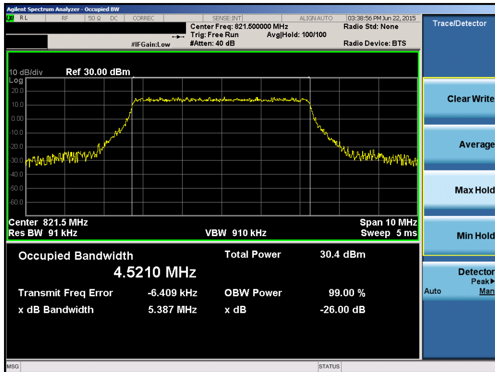
Plot 7-21. Bandwidth Plot (5MHz QPSK – RB Size 25– High Channel)
