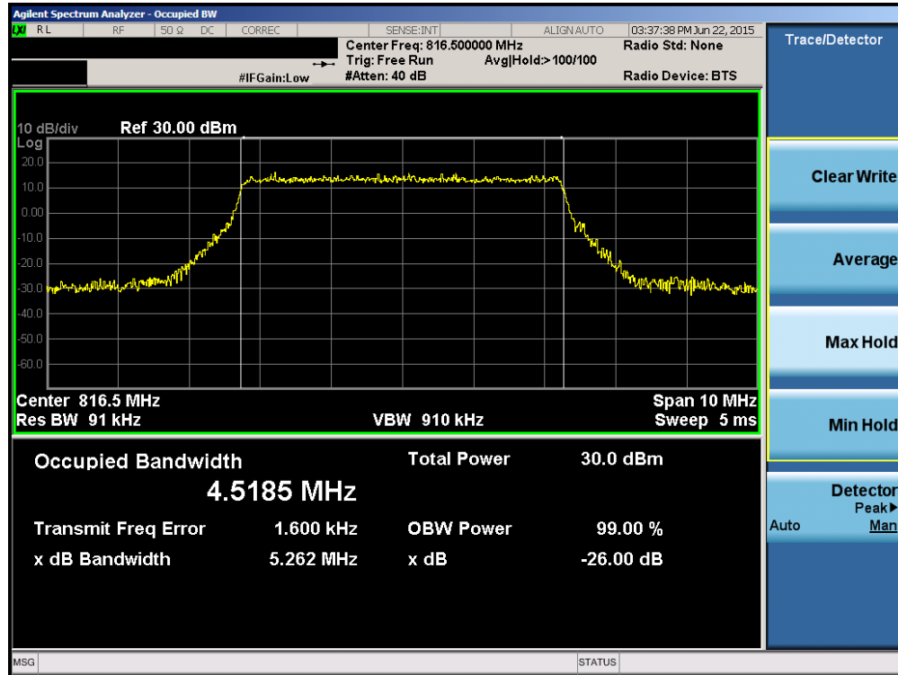
Plot 7-18. Occupied Bandwidth Plot (5MHz QPSK – RB Size 25– Low Channel)
