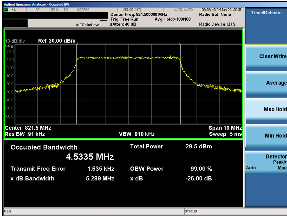
Plot 7-22. Bandwidth Plot (5MHz 16-QAM – RB Size 25– High Channel)
