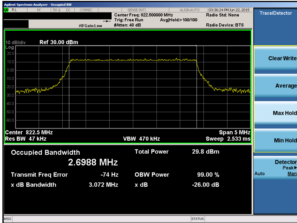
Plot 7-16. Bandwidth Plot (3MHz 16-QAM – RB Size 15– High Channel)
