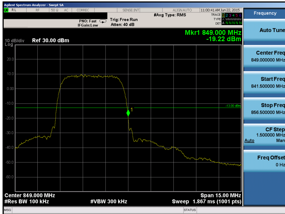
Plot 6-50. Band Edge Plot (Cellular WCDMA Mode – Ch. 4233)
