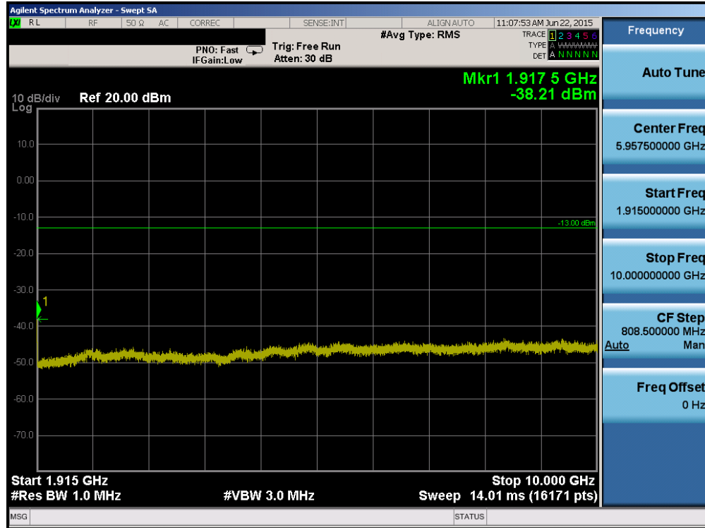
Plot 6-41. Conducted Spurious Plot (PCS WCDMA Mode – Ch. 9538)
