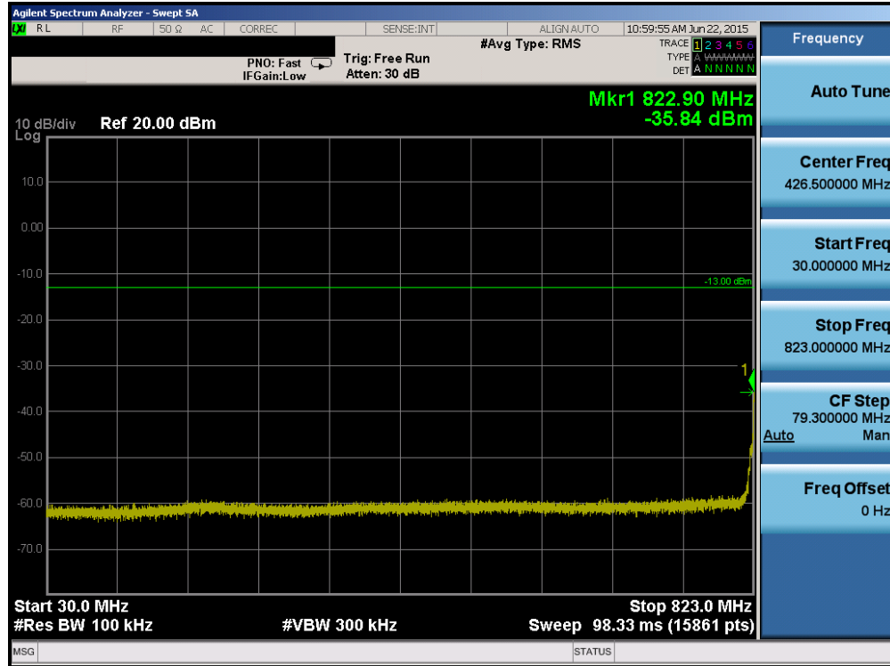
Plot 6-25. Conducted Spurious Plot (Cellular WCDMA Mode – Ch. 4132)
