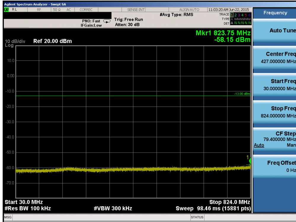
Plot 6-31. Conducted Spurious Plot (Cellular WCDMA Mode – Ch. 4233)
