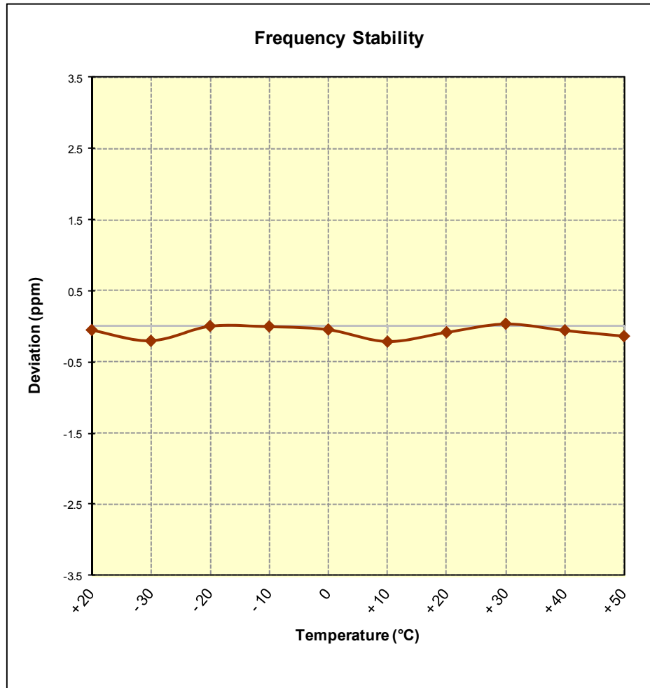
Figure 6-10. Frequency Stability Graph (PCS WCDMA Mode – Ch. 9400)
