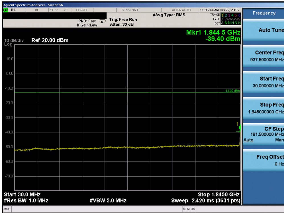
Plot 6-34. Conducted Spurious Plot (PCS WCDMA Mode – Ch. 9262)
