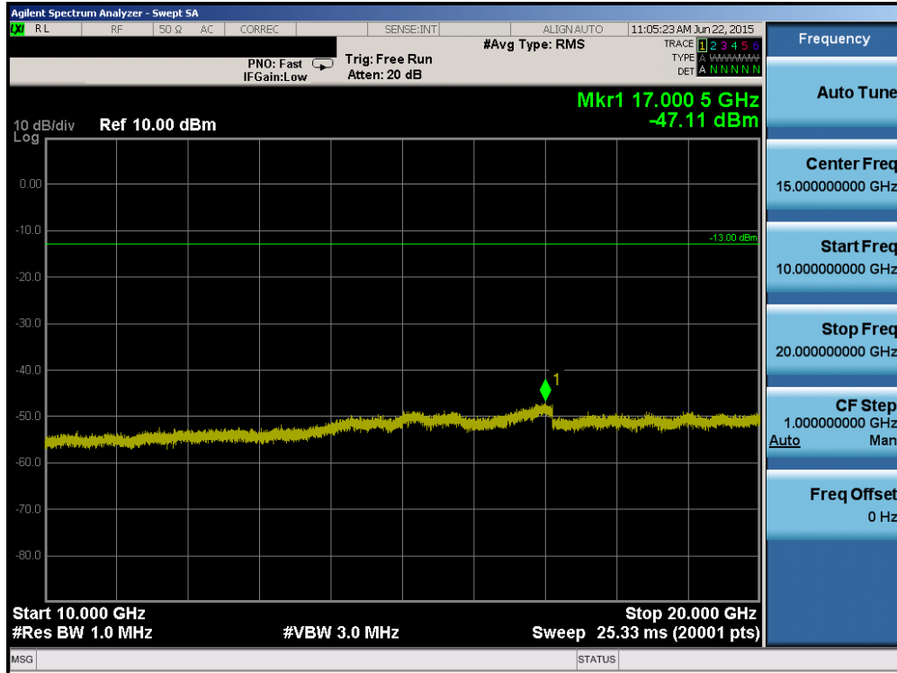
Plot 6-39. Conducted Spurious Plot (PCS WCDMA Mode – Ch. 9400)
