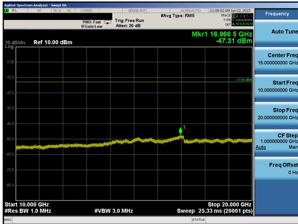
Plot 6-42. Conducted Spurious Plot (PCS WCDMA Mode – Ch. 9538)
