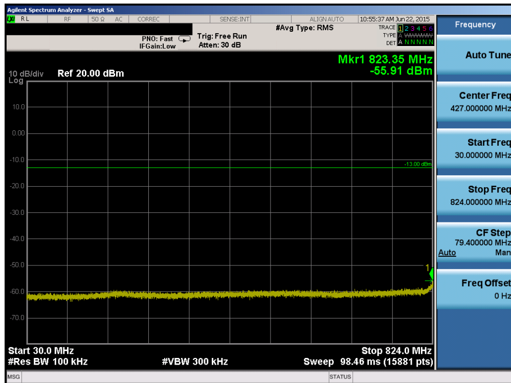
Plot 6-28. Conducted Spurious Plot (Cellular WCDMA Mode – Ch. 4183)
