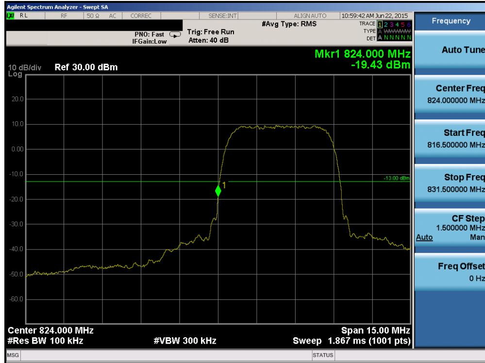
Plot 6-49. Band Edge Plot (Cellular WCDMA Mode – Ch. 4132)
