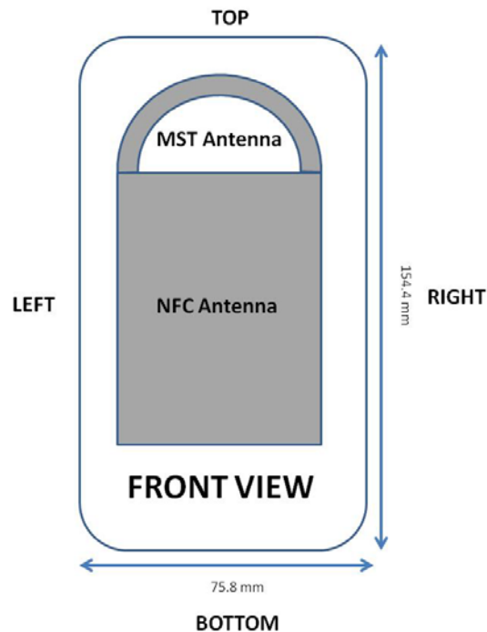
Figure F-2 NFC and MST Antenna Locations
