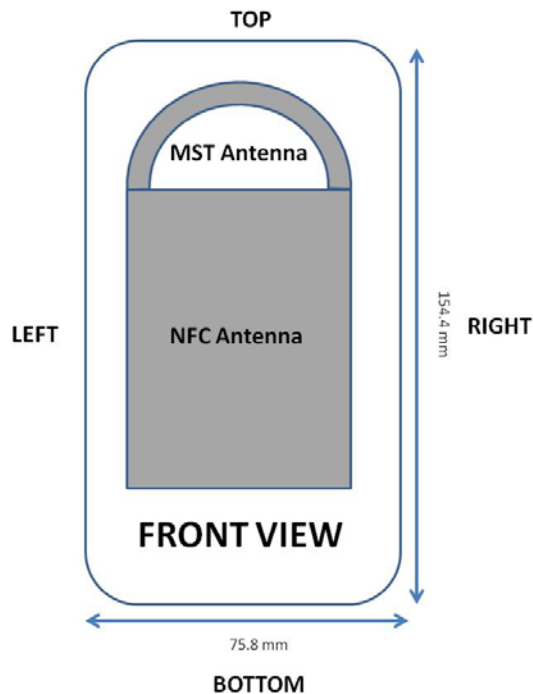
Figure F-2 NFC and MST Antenna Locations
