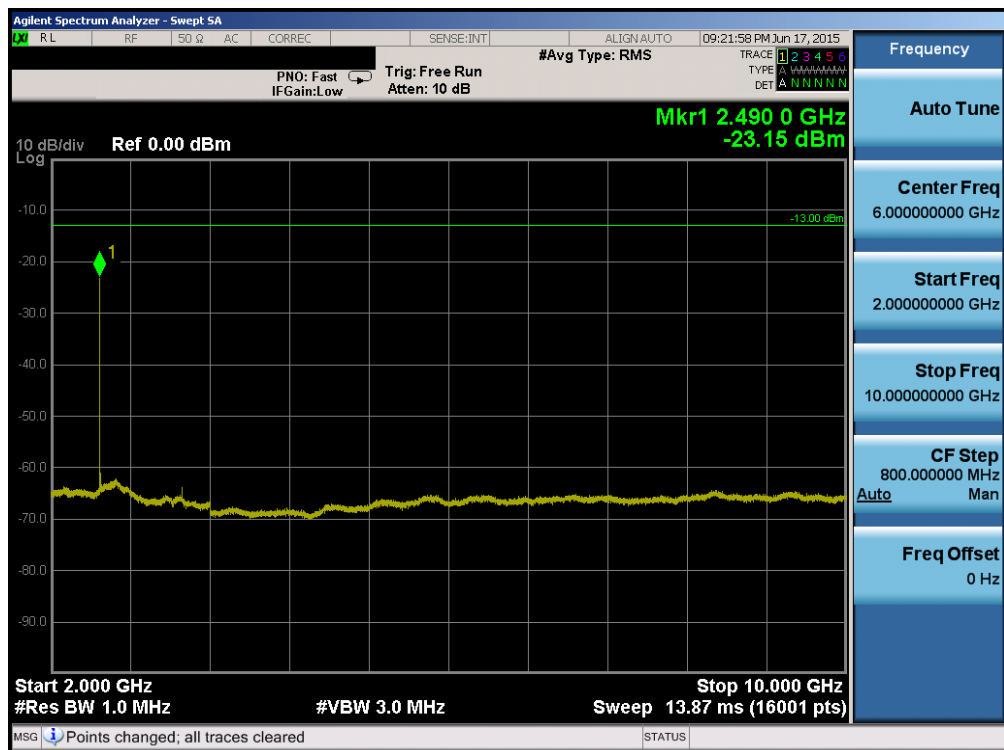
Plot 6-66. Conducted Spurious Plot (Band 26 – 15.0MHz QPSK – RB Size 1, RB Offset 0 – Mid Channel)
