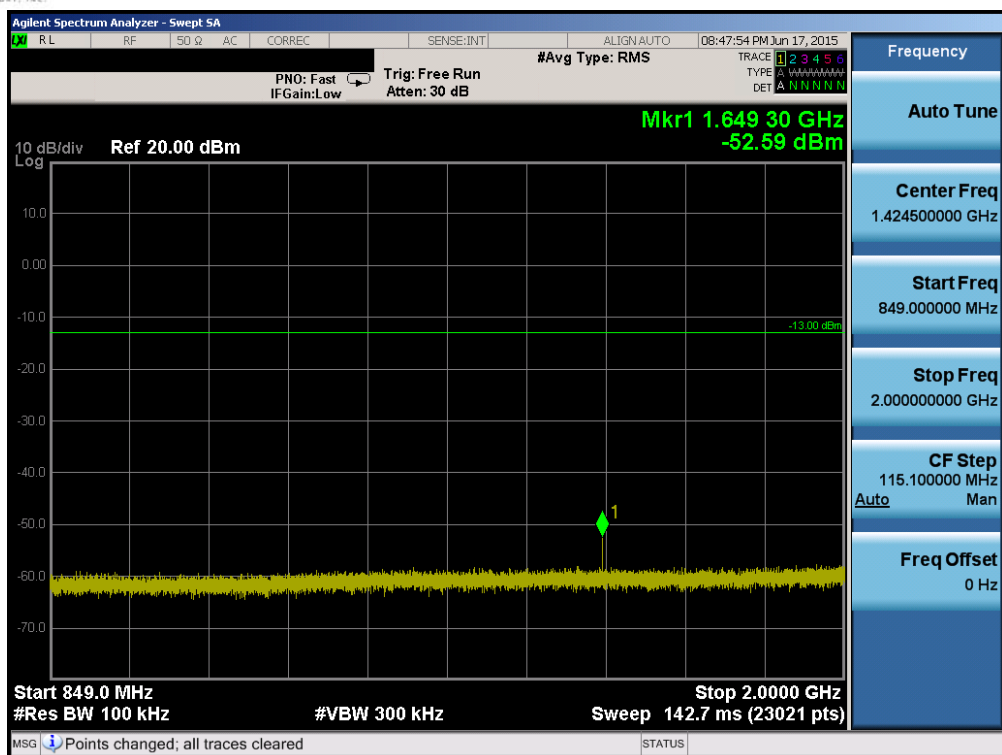
Plot 6-53. Conducted Spurious Plot (Band 5 – 10.0MHz QPSK – RB Size 1, RB Offset 0 – Low Channel)
