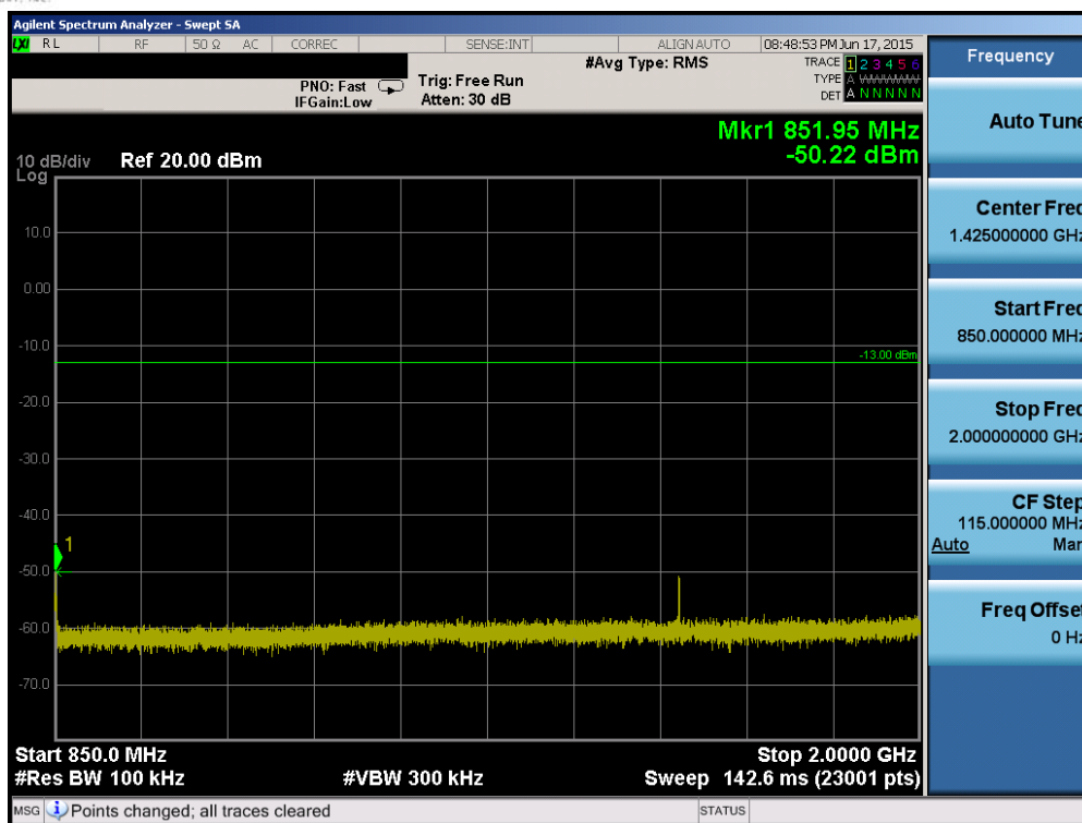
Plot 6-59. Conducted Spurious Plot (Band 5 – 10.0MHz QPSK – RB Size 1, RB Offset 0 – High Channel)
