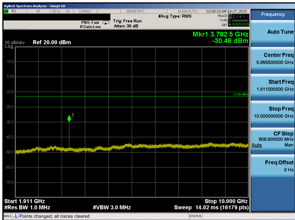
Plot 6-86. Conducted Spurious Plot (Band 2 – 20.0MHz QPSK – RB Size 1, RB Offset 0 – High Channel)
