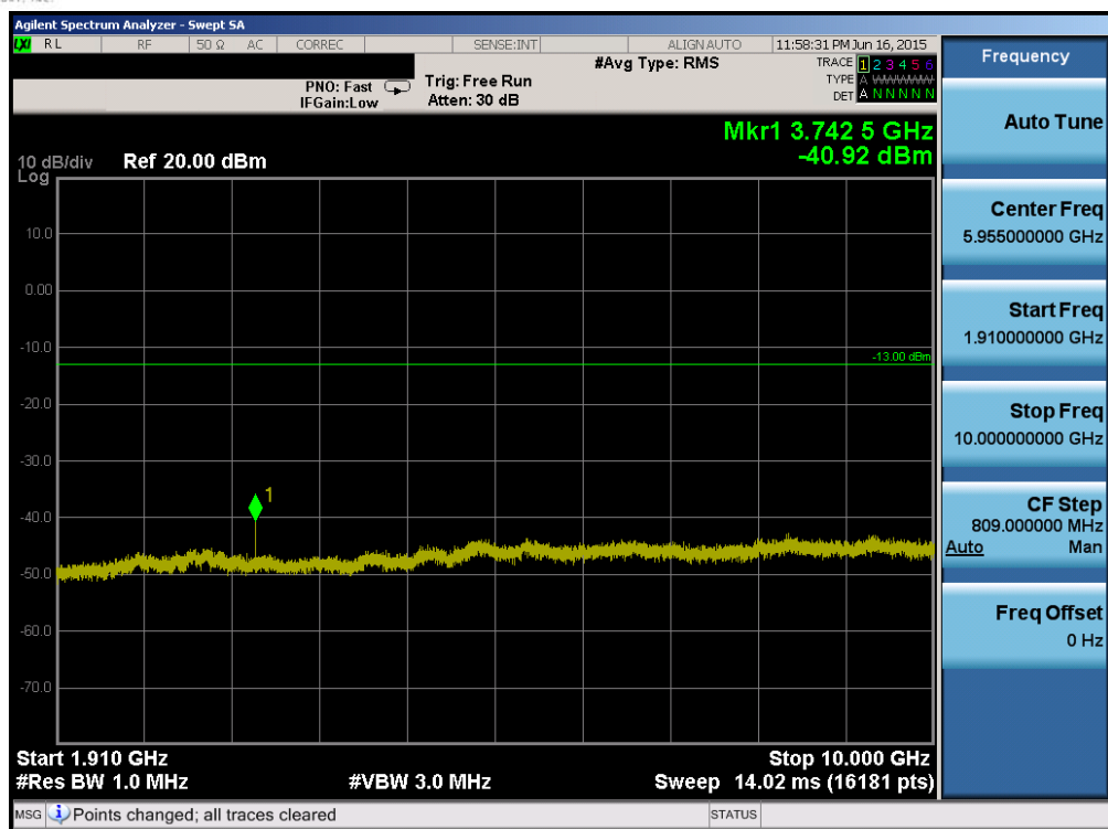
Plot 6-83. Conducted Spurious Plot (Band 2 – 20.0MHz QPSK – RB Size 1, RB Offset 0 – Mid Channel)
