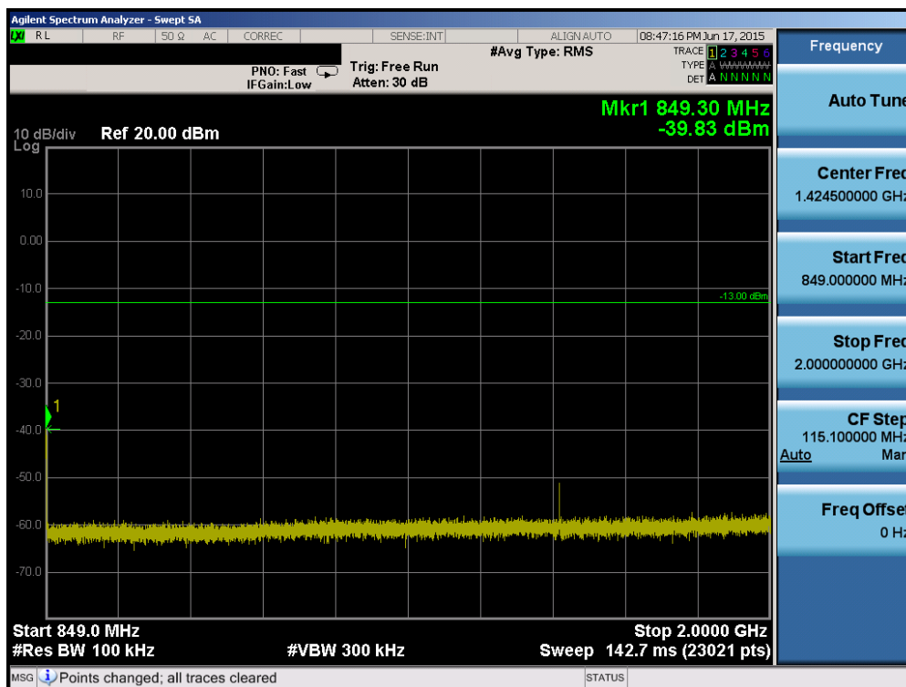
Plot 6-56. Conducted Spurious Plot (Band 5 – 10.0MHz QPSK – RB Size 1, RB Offset 0 – Mid Channel)
