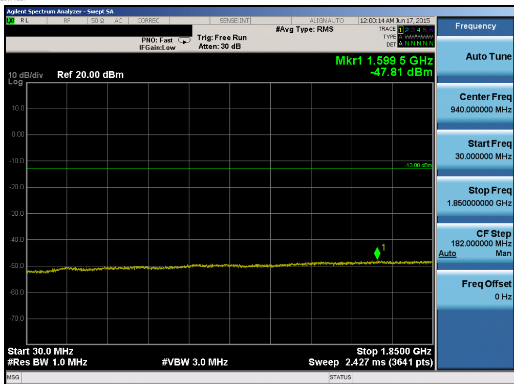
Plot 6-85. Conducted Spurious Plot (Band 2 – 20.0MHz QPSK – RB Size 1, RB Offset 0 – High Channel)
