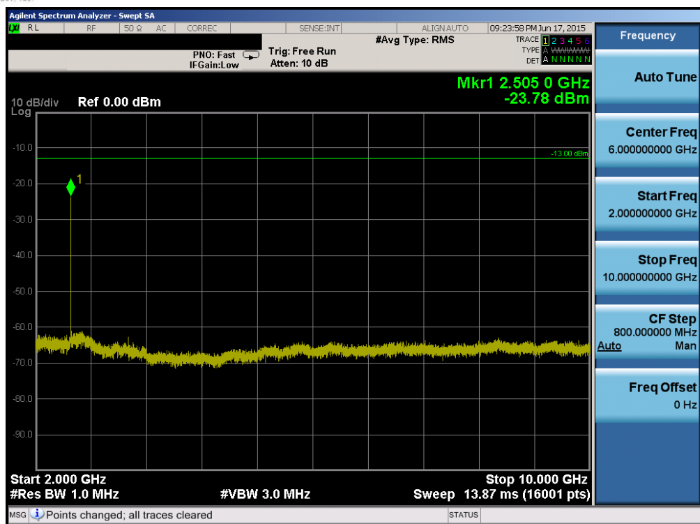
Plot 6-69. Conducted Spurious Plot (Band 26 – 15.0MHz QPSK – RB Size 1, RB Offset 0 – High Channel)
