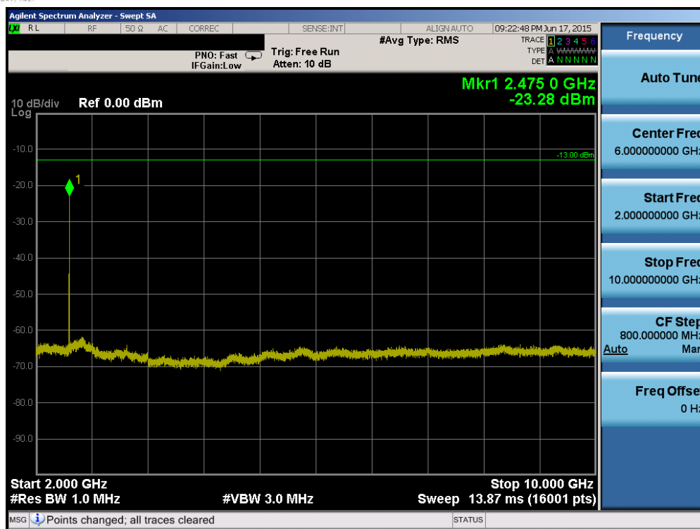
Plot 6-63. Conducted Spurious Plot (Band 26 – 15.0MHz QPSK – RB Size 1, RB Offset 0 – Low Channel)
