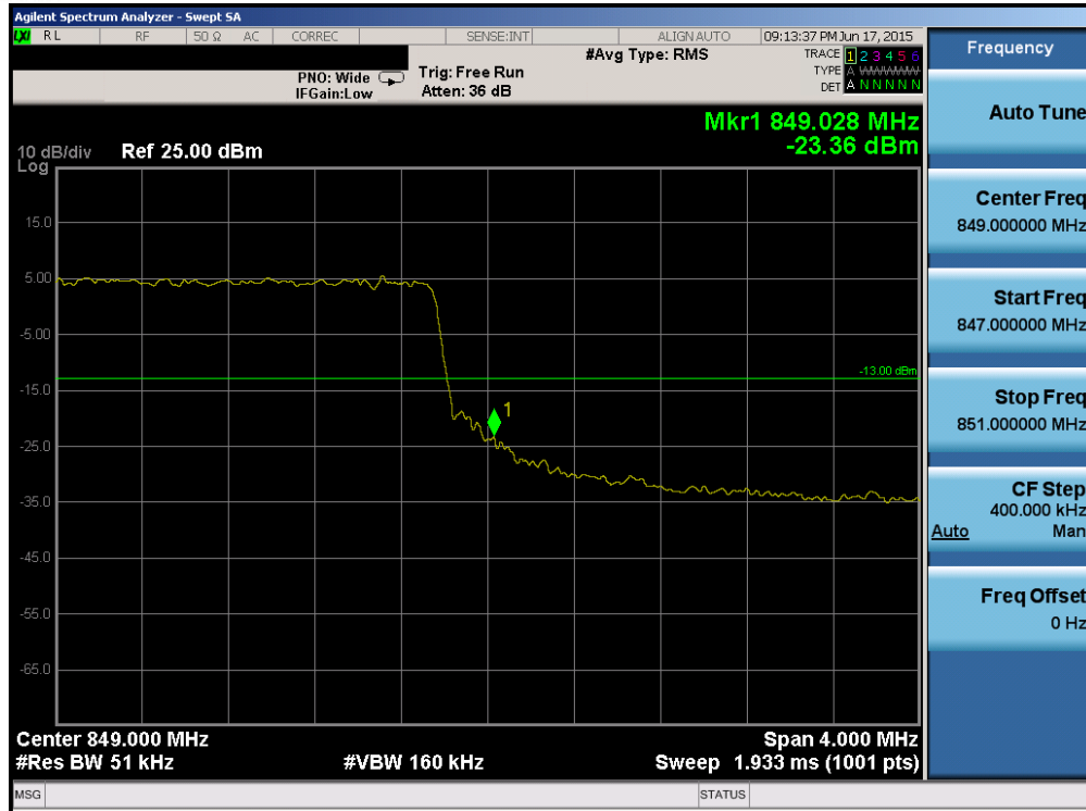
Plot 6-112. Upper Band Edge Plot (Band 5/26 - 5.0MHz QPSK - RB Size 25)
