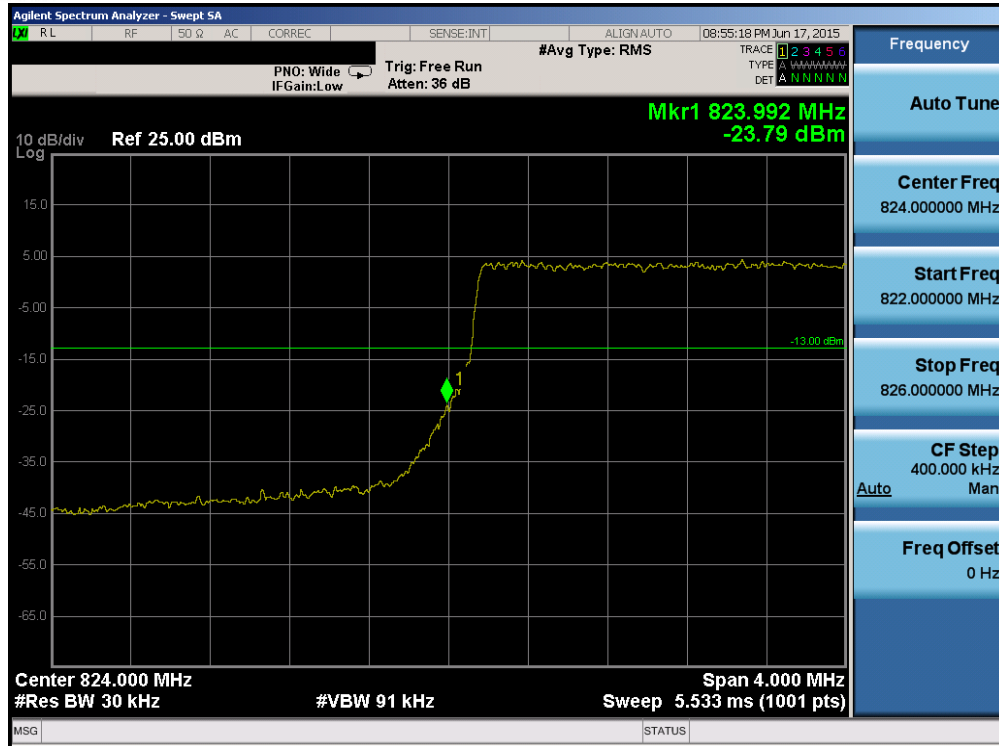
Plot 6-106. Lower Band Edge Plot (Band 5/26 – 3.0MHz QPSK – RB Size 15)
