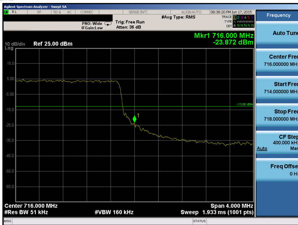
Plot 6-98. Upper Band Edge Plot (Band 12/17 - 5.0MHz QPSK - RB Size 25)
