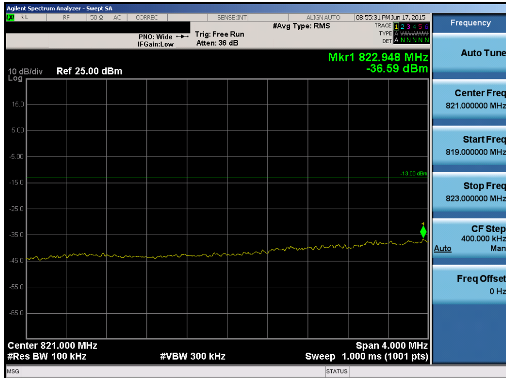
Plot 6-107. Lower Extended Band Edge Plot (Band 5/26 – 3.0MHz QPSK – RB Size 15)
