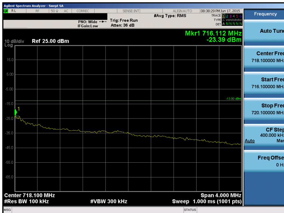
Plot 6-99. Upper Extended Band Edge Plot (Band 12/17 - 5.0MHz QPSK - RB Size 25)
