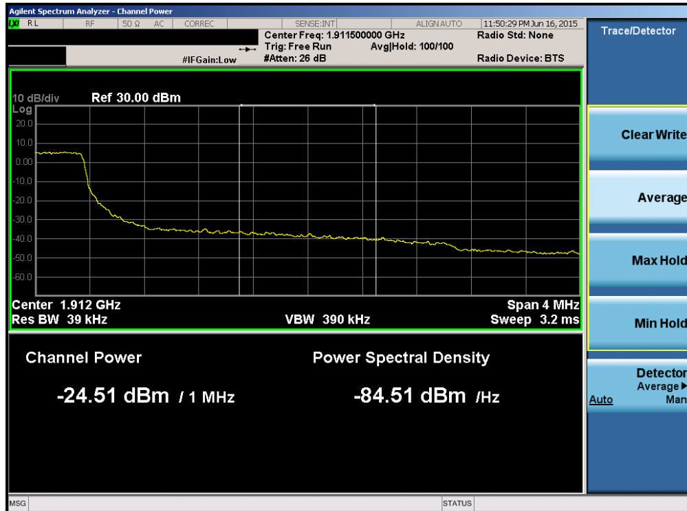
Plot 6-149. Upper Extended Band Edge Plot (Band 2 – 3.0MHz QPSK – RB Size 15)
