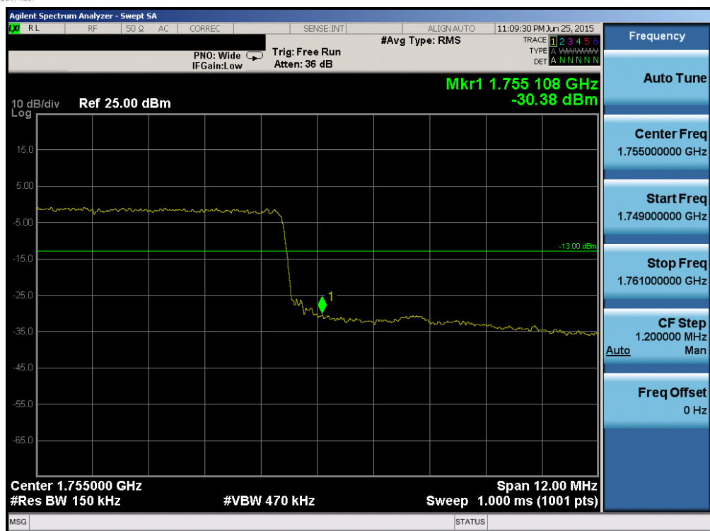
Plot 6-136. Upper Band Edge Plot (Band 4 – 15.0MHz QPSK – RB Size 75)
