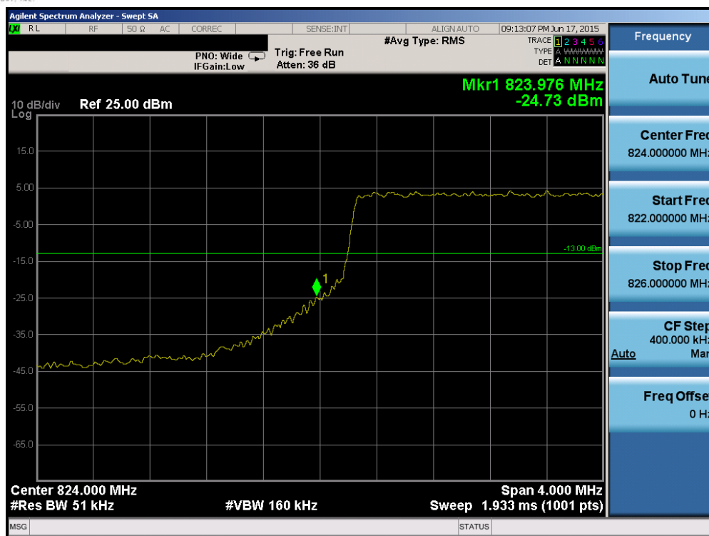
Plot 6-110. Lower Band Edge Plot (Band 5/26 – 5.0MHz QPSK – RB Size 25)
