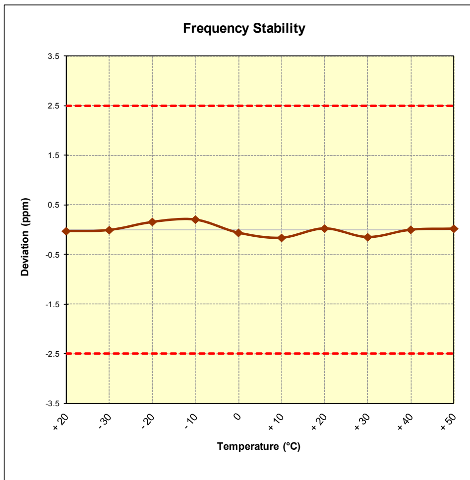
Figure 6-7. Frequency Stability Graph (Band 12/17)
