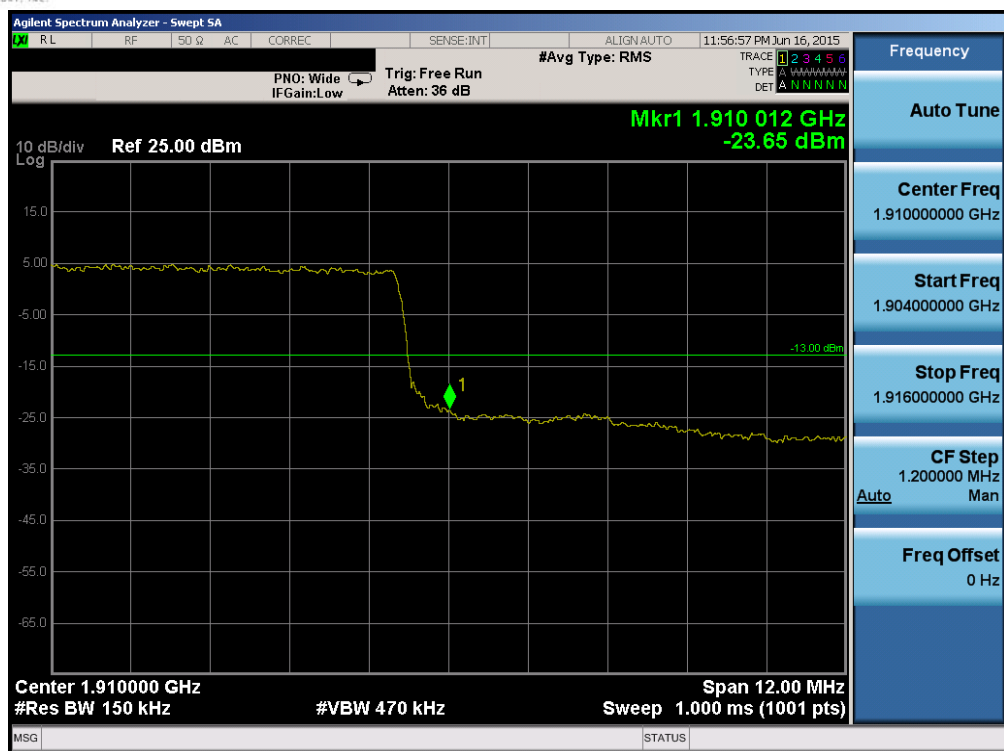
Plot 6-160. Upper Band Edge Plot (Band 2 – 15.0MHz QPSK – RB Size 75)
