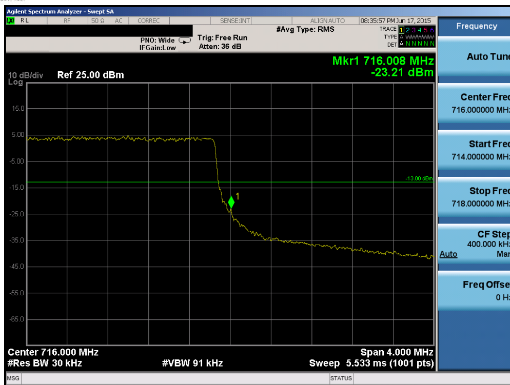
Plot 6-94. Upper Band Edge Plot (Band 12 – 3.0MHz QPSK – RB Size 15)
