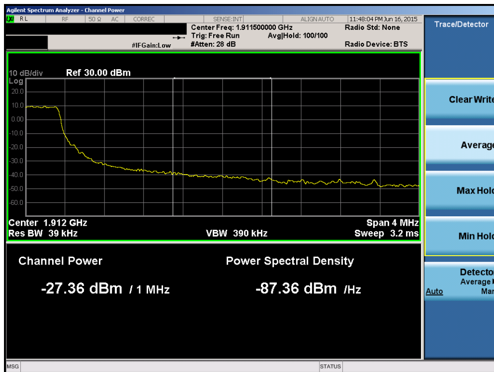
Plot 6-145. Upper Extended Band Edge Plot (Band 2 – 1.4MHz QPSK – RB Size 6)
