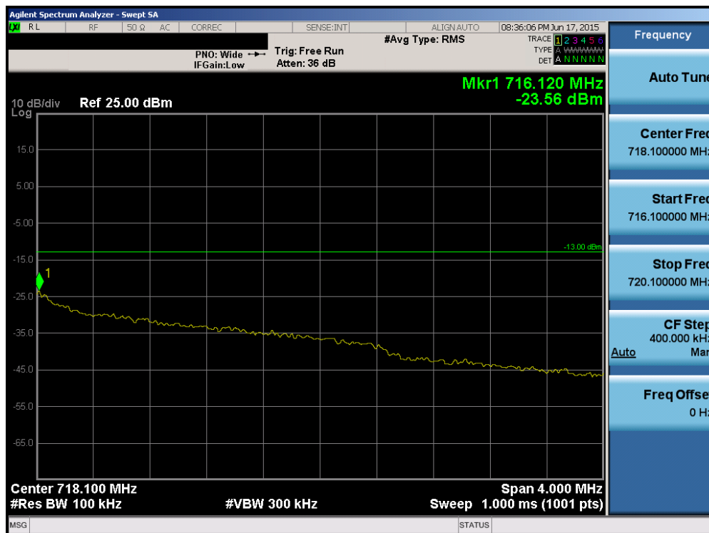
Plot 6-95. Upper Extended Band Edge Plot (Band 12 – 3.0MHz QPSK – RB Size 15)
