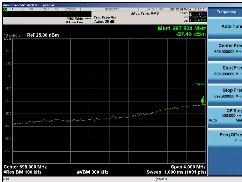
Plot 6-93. Lower Extended Band Edge Plot (Band 12 – 3.0MHz QPSK – RB Size 15)
