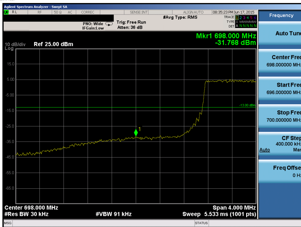
Plot 6-92. Lower Band Edge Plot (Band 12 – 3.0MHz QPSK – RB Size 15)
