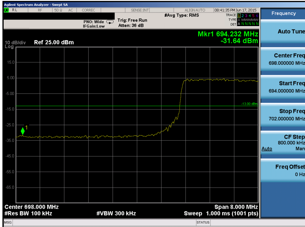
Plot 6-100. Lower Band Edge Plot (Band 12/17 – 10.0MHz QPSK – RB Size 50)
