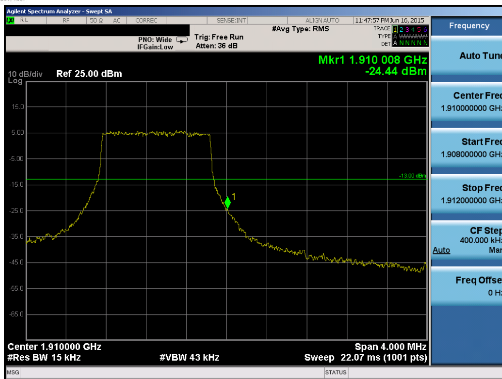
Plot 6-144. Upper Band Edge Plot (Band 2 – 1.4MHz QPSK – RB Size 6)
