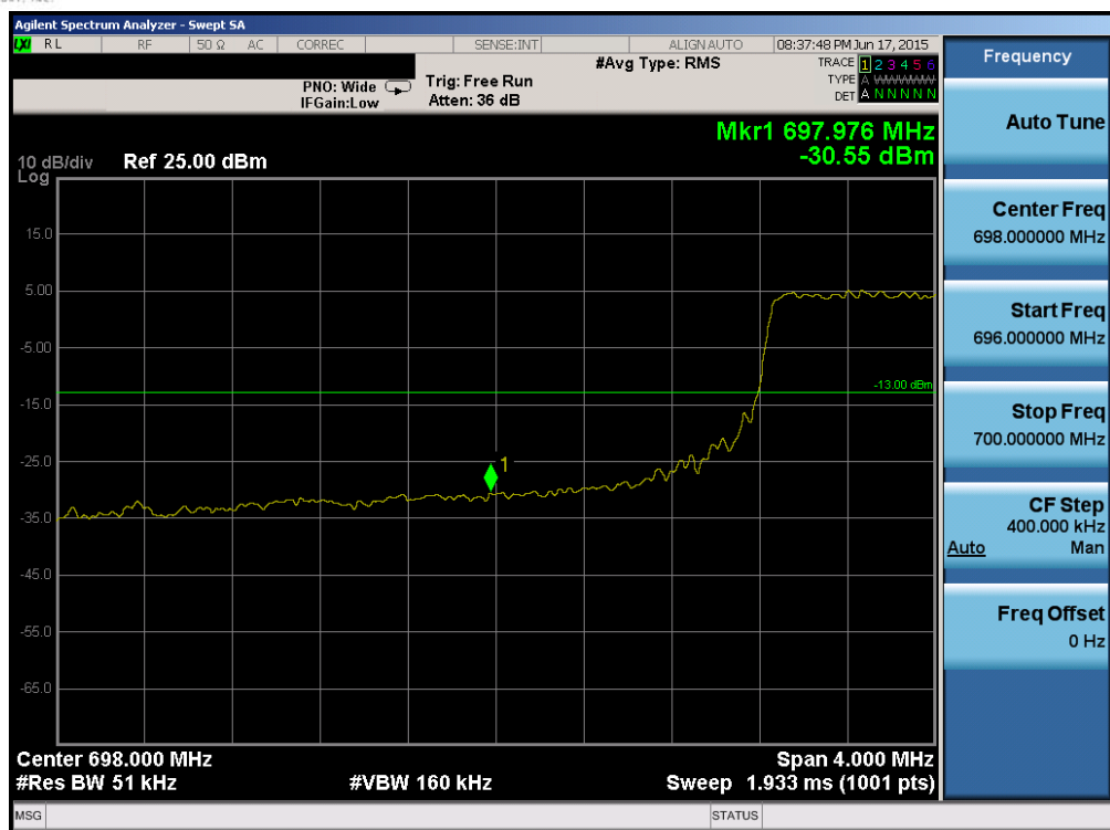
Plot 6-96. Lower Band Edge Plot (Band 12/17 – 5.0MHz QPSK – RB Size 25)
