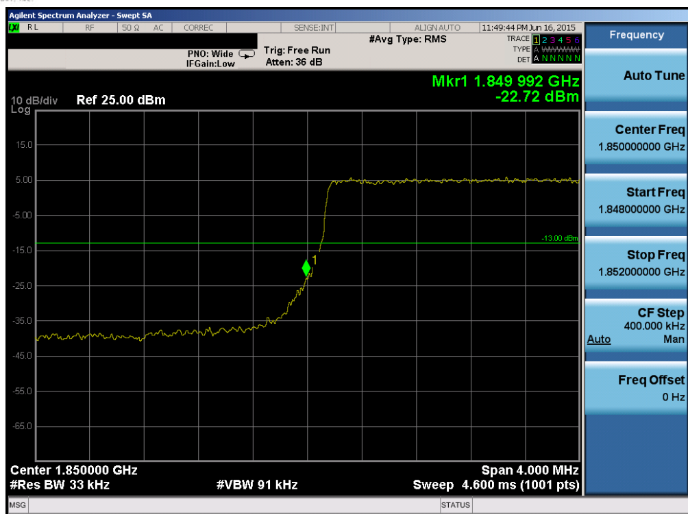
Plot 6-146. Lower Band Edge Plot (Band 2 – 3.0MHz QPSK – RB Size 15)
