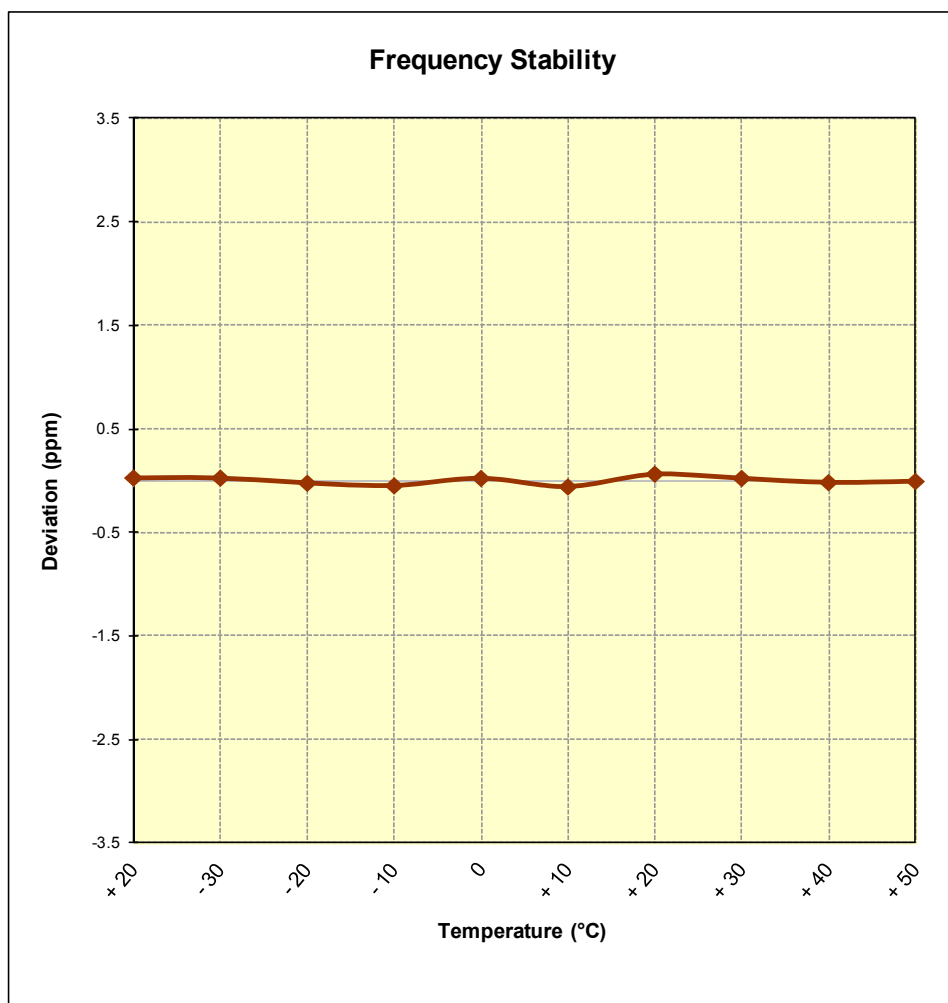
Figure 6-10. Frequency Stability Graph (Band 2)
