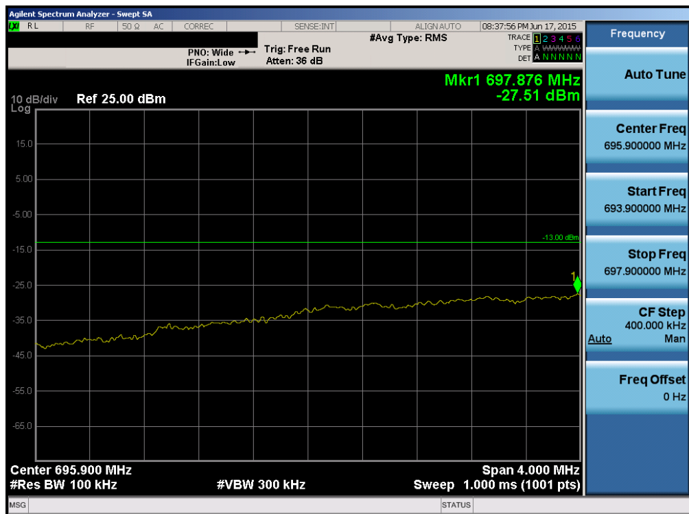
Plot 6-97. Lower Extended Band Edge Plot (Band 12/17 – 5.0MHz QPSK – RB Size 25)
