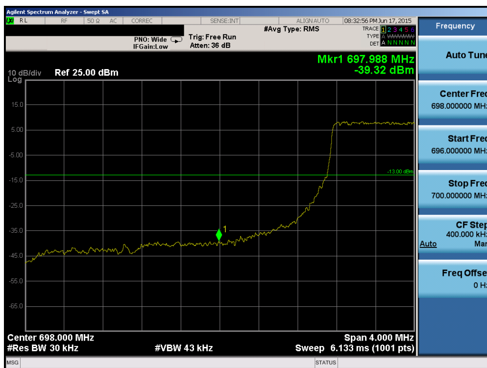
Plot 6-88. Lower Band Edge Plot (Band 12 – 1.4MHz QPSK – RB Size 6)
