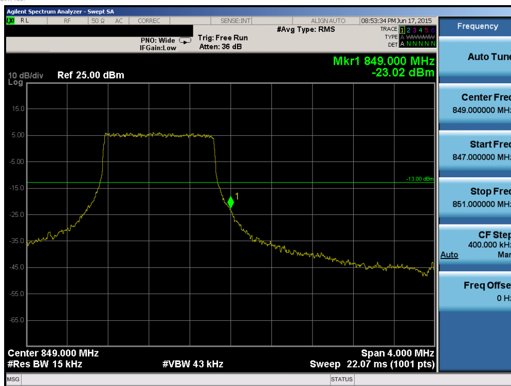
Plot 6-104. Upper Band Edge Plot (Band 5/26 – 1.4MHz QPSK – RB Size 6)
