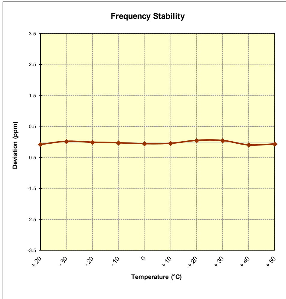
Figure 6-9. Frequency Stability Graph (Band 4)
