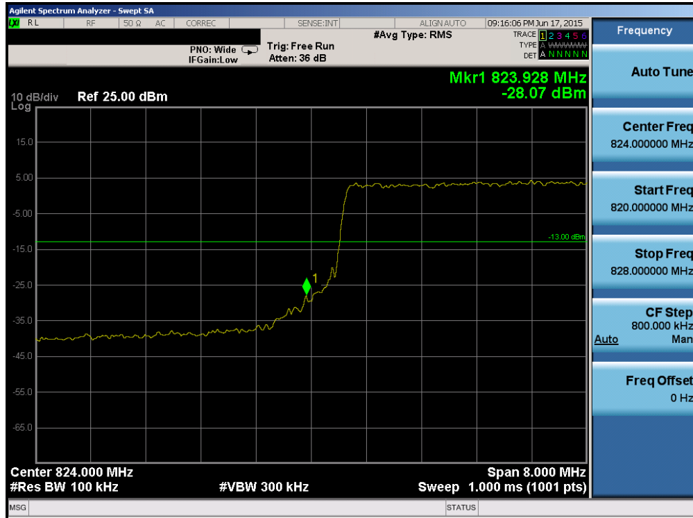
Plot 6-114. Lower Band Edge Plot (Band 5/26 – 10.0MHz QPSK – RB Size 50)
