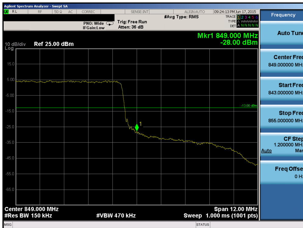
Plot 6-117. Upper Band Edge Plot (Band 26 – 15.0MHz QPSK – RB Size 75)
