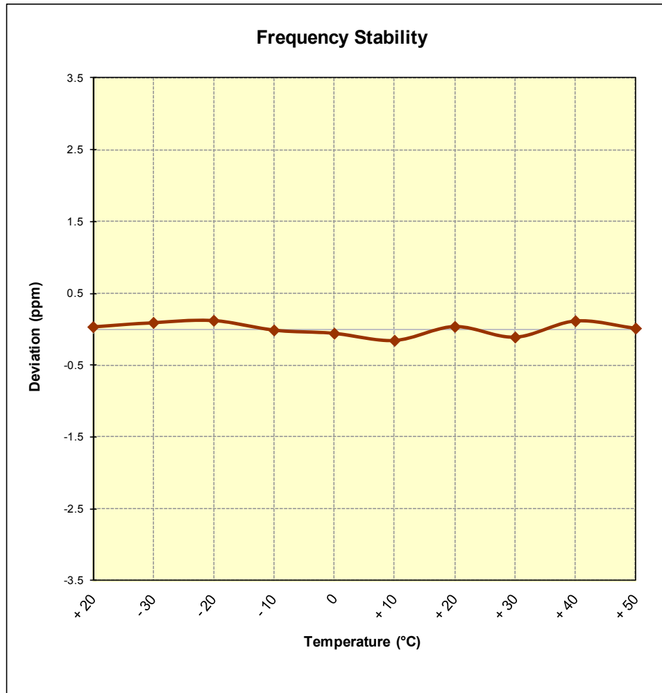
Figure 6-8. Frequency Stability Graph (Band 5/26)
