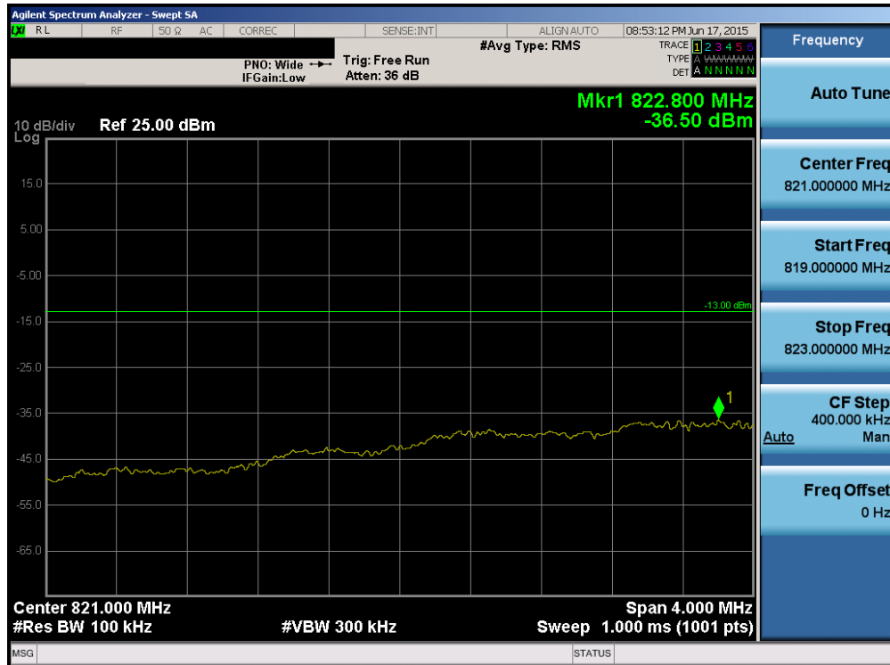
Plot 6-103. Lower Extended Band Edge Plot (Band 5/26 – 1.4MHz QPSK – RB Size 6)
