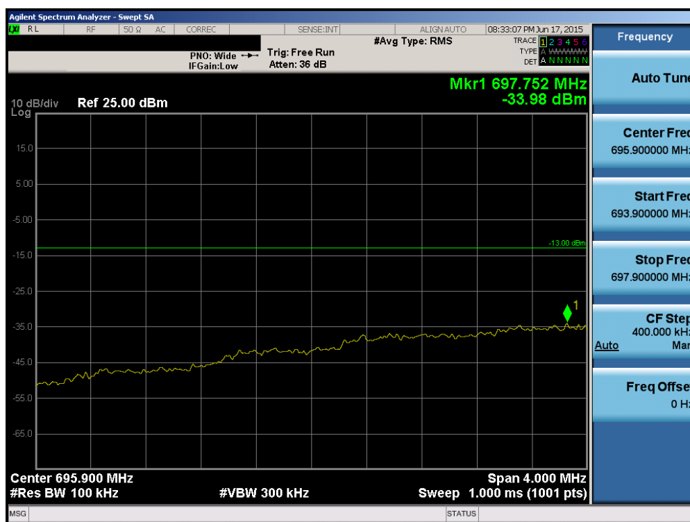
Plot 6-89. Lower Extended Band Edge Plot (Band 12 – 1.4MHz QPSK – RB Size 6)
