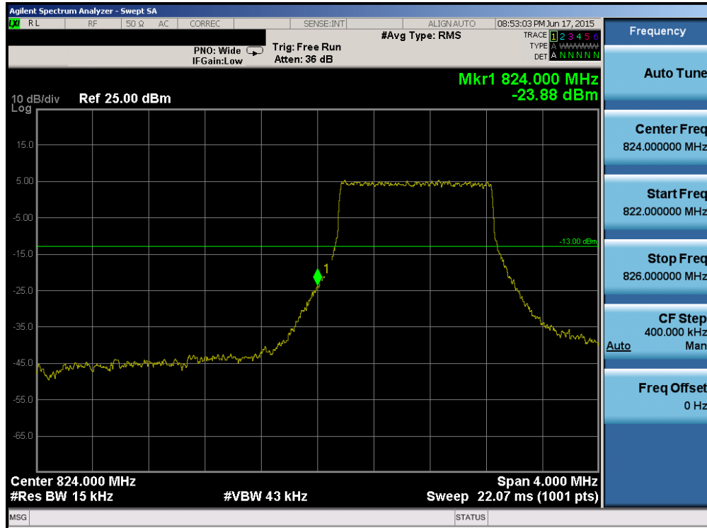
Plot 6-102. Lower Band Edge Plot (Band 5/26 – 1.4MHz QPSK – RB Size 6)
