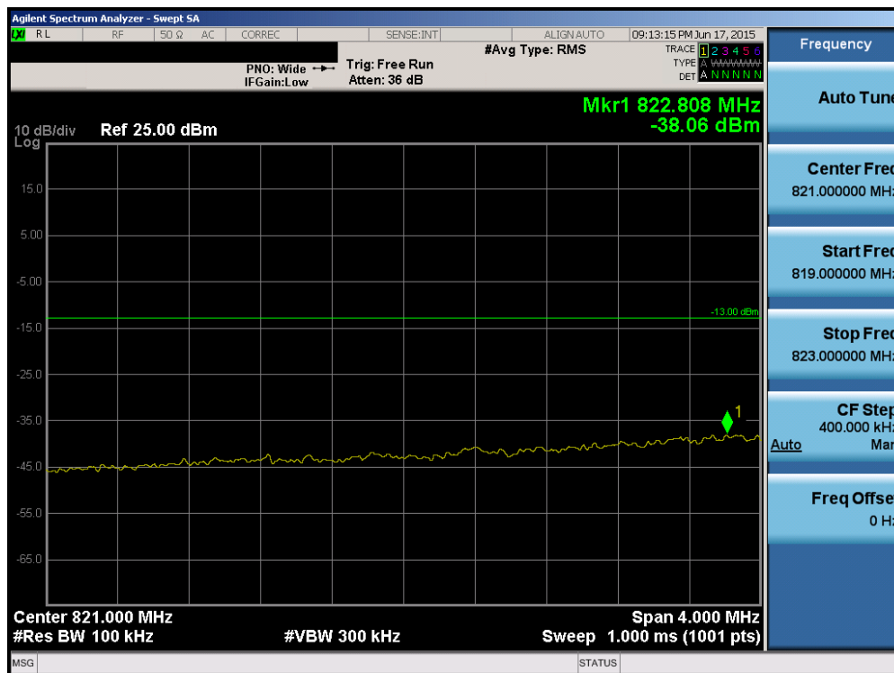
Plot 6-111. Lower Extended Band Edge Plot (Band 5/26 – 5.0MHz QPSK – RB Size 25)
