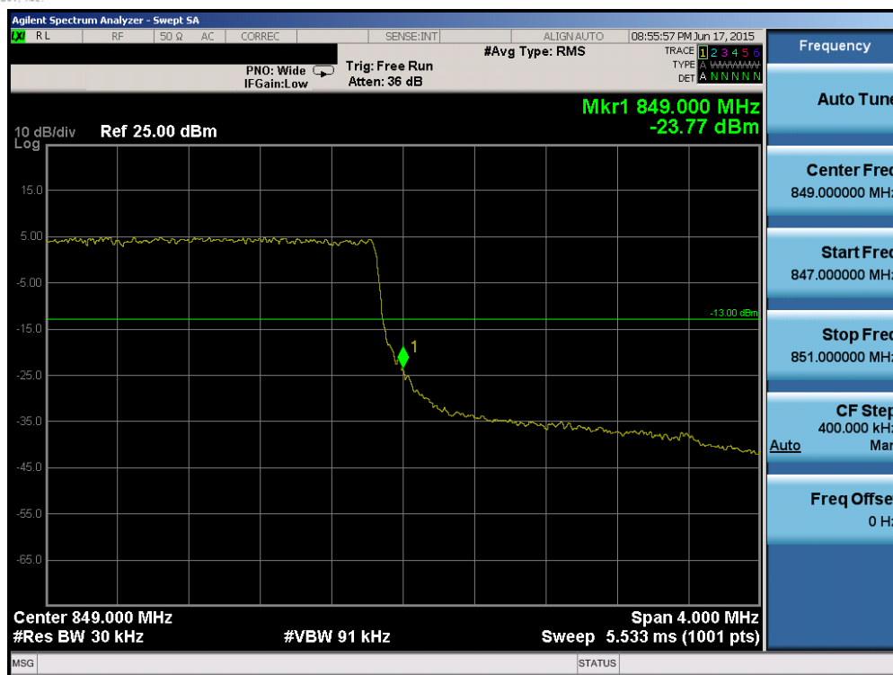
Plot 6-108. Upper Band Edge Plot (Band 5/26 – 3.0MHz QPSK – RB Size 15)
