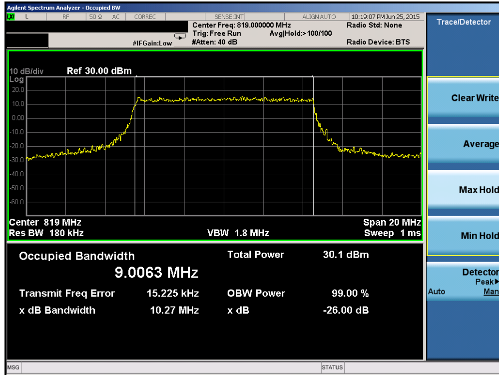
Plot 7-18. Occupied Bandwidth Plot (10MHz 16-QAM – RB Size 50)
