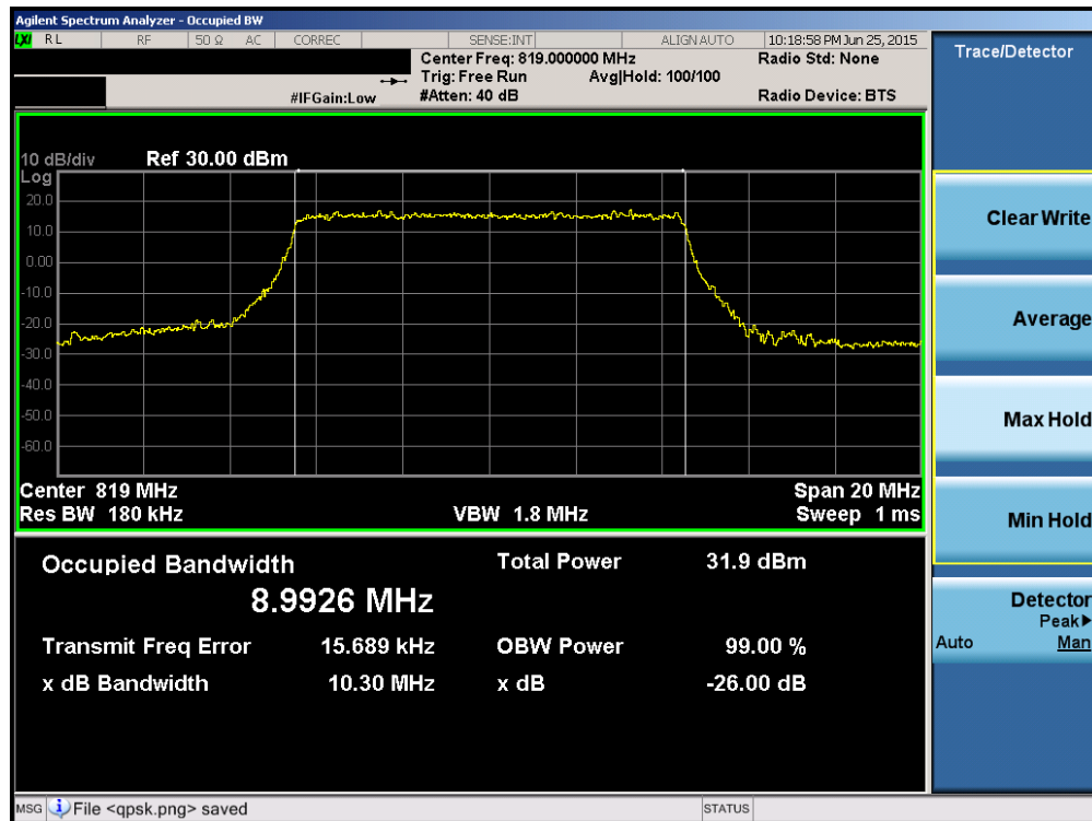
Plot 7-17. Occupied Bandwidth Plot (10MHz QPSK – RB Size 50)
