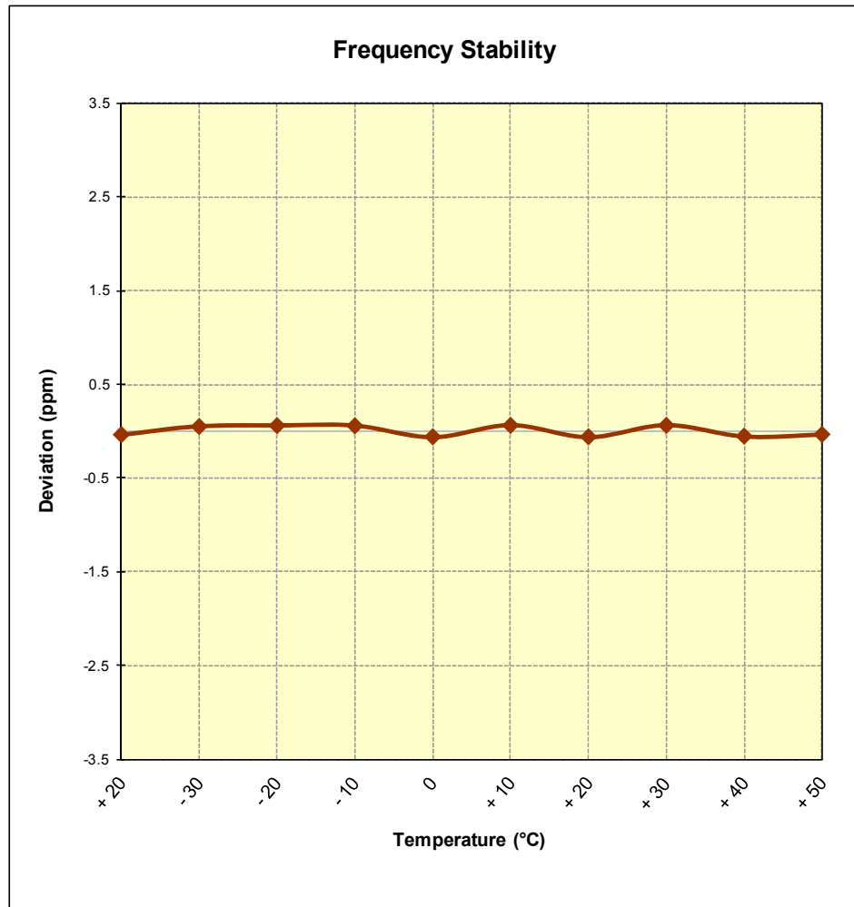
Figure 6-9. Frequency Stability Graph (AWS WCDMA Mode – Ch. 1412)
