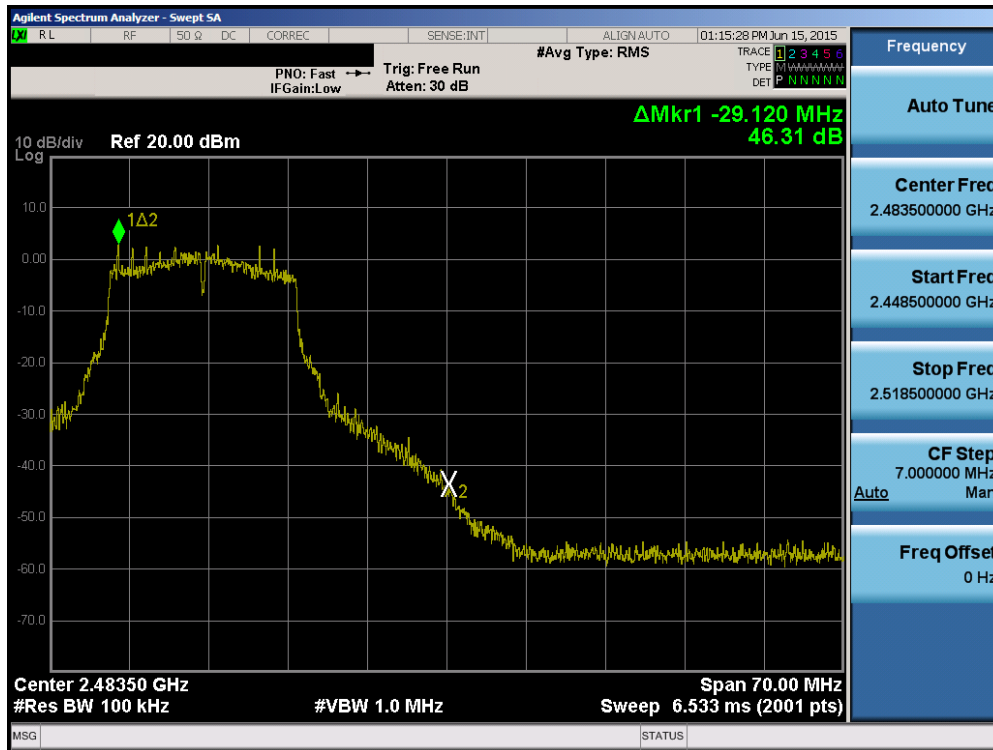
Plot 6-50. Band Edge Plot (802.11g – Ch. 11)
