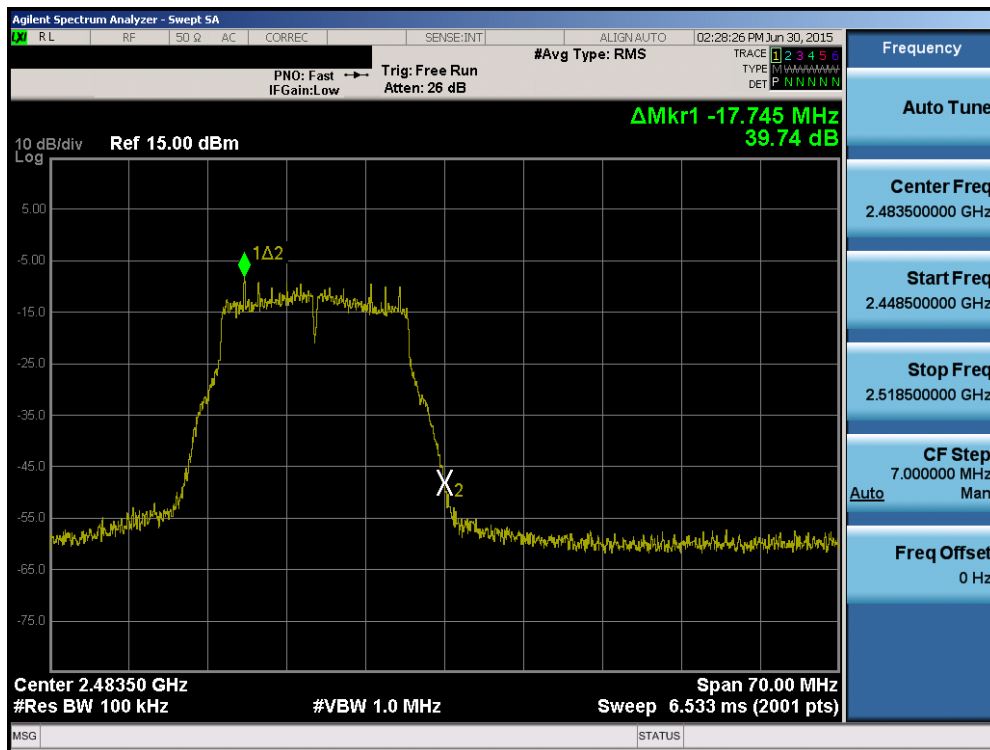
Plot 6-42. Band Edge Plot (802.11g – Ch. 13)
