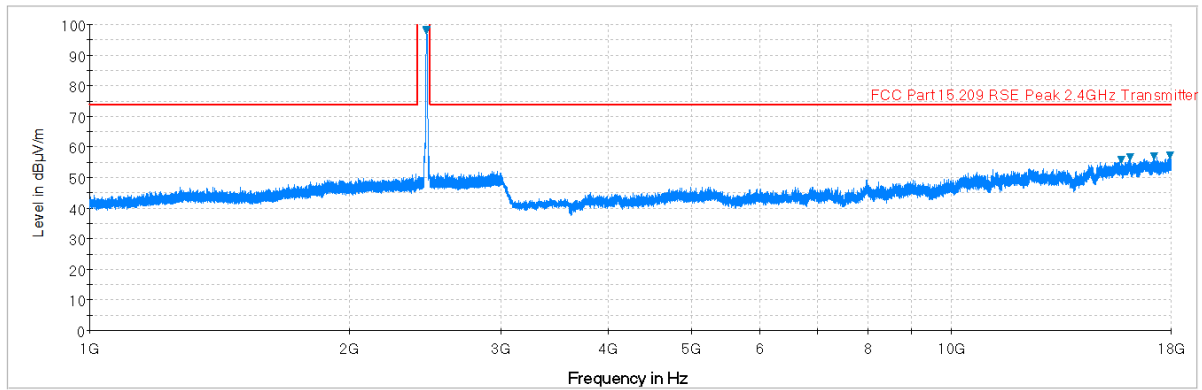
Plot 6-71. Radiated Spurious Plot above 1GHz (802.11b – Ch. 11, Ant. Pol. H)
