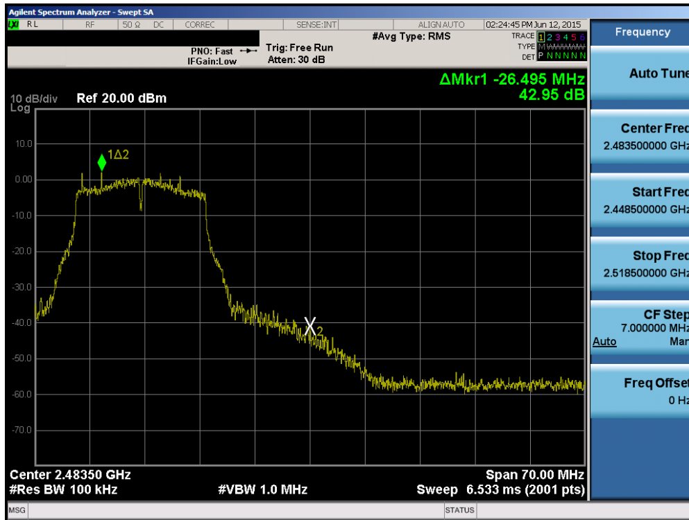
Plot 6-41. Band Edge Plot (802.11g – Ch. 11)
