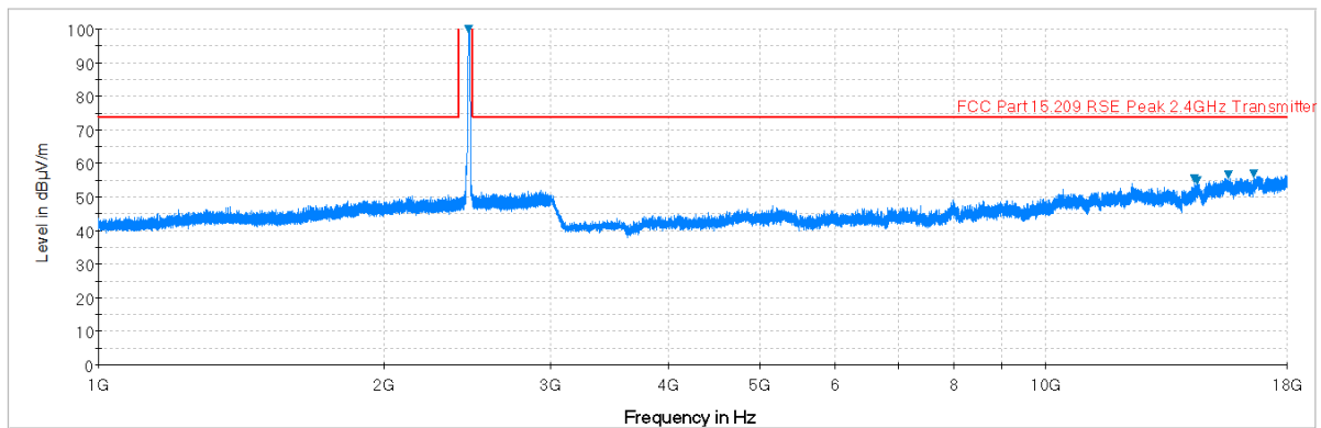
Plot 6-79. Radiated Spurious Plot above 1GHz (802.11b – Ch. 11, Ant. Pol. H)
