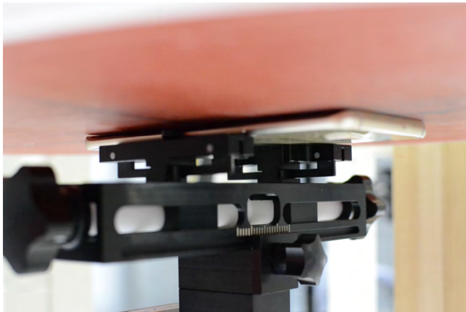
SAR Test Setup Photo 8— Front Side at 0.0 cm (Extremity)
