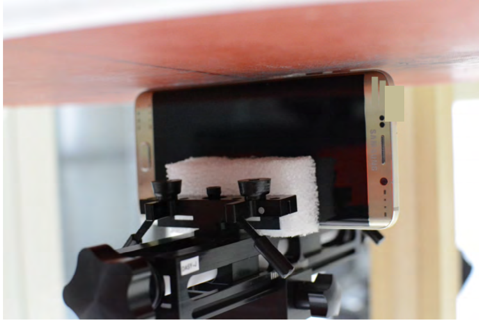
SAR Test Setup Photo 15 – Left Edge at 0.0 cm (Extremity)
