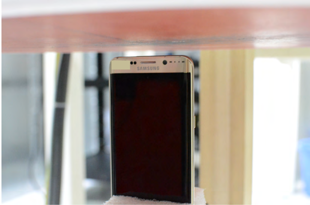
SAR Test Setup Photo 11- Top Edge at 1.0 cm (Hotspot)
