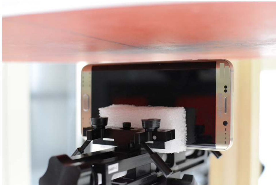
SAR Test Setup Photo 6 – Left Edge at 1.0 cm (Hotspot)
