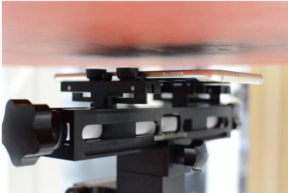
SAR Test Setup Photo 2– Back Side at 1.5 cm (Body-Worn)
