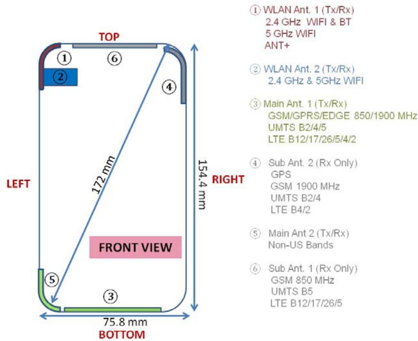
Figure F-1 DUT Antenna Locations
