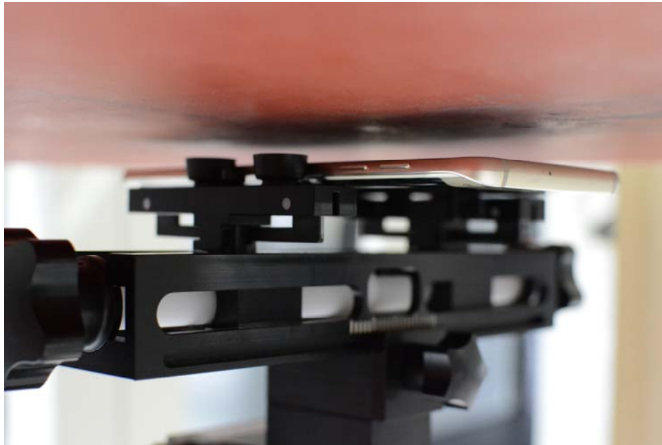
SAR Test Setup Photo 1– Back Side at 1.0 cm (Hotspot)
