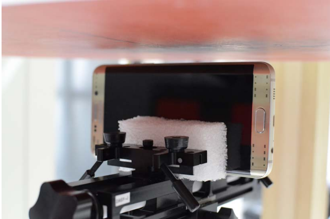
SAR Test Setup Photo 5 – Right Edge at 1.0 cm (Hotspot)
