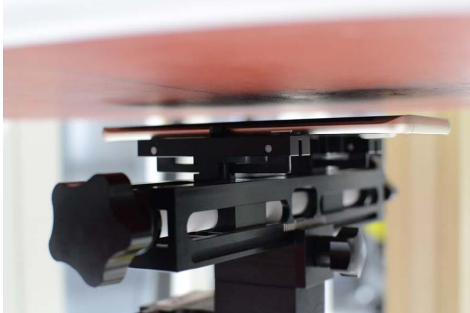
SAR Test Setup Photo 3- Front Side at 1.0 cm (Hotspot)
