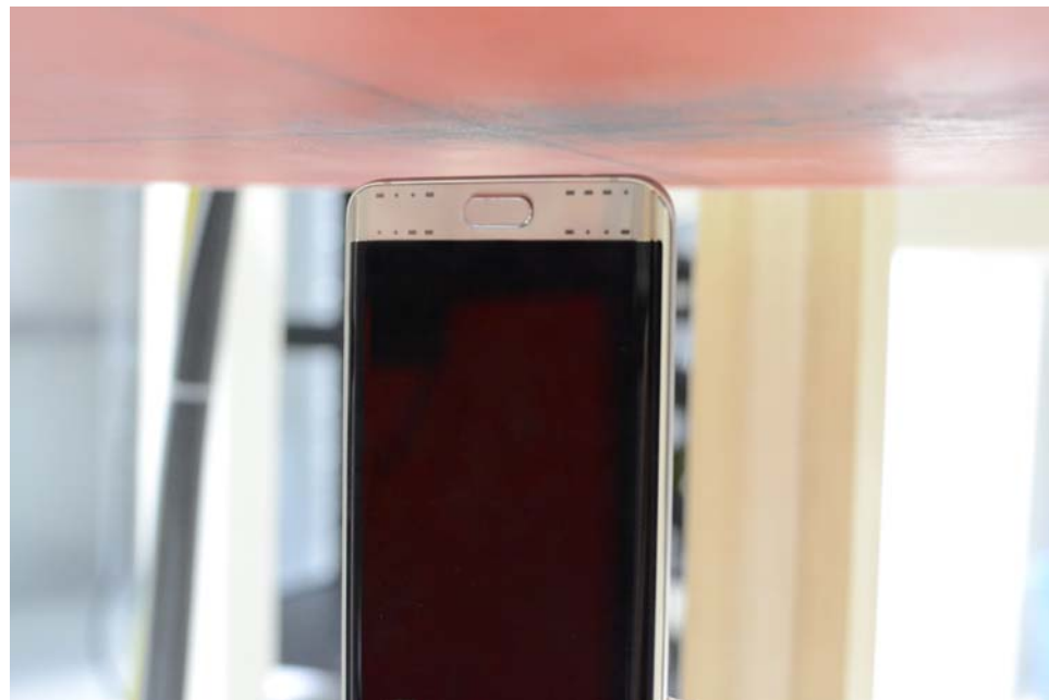
SAR Test Setup Photo 4 – Bottom Edge at 1.0 cm (Hotspot)
