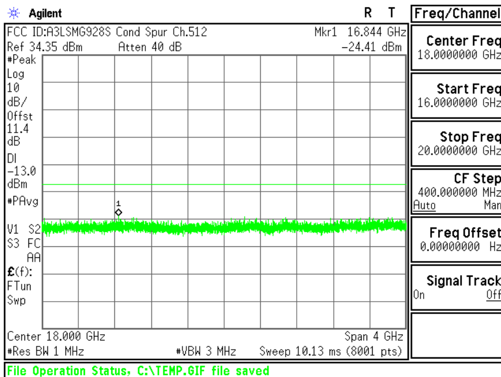
Plot 6-9. Conducted Spurious Plot (PCS GSM Mode - Ch.512)
