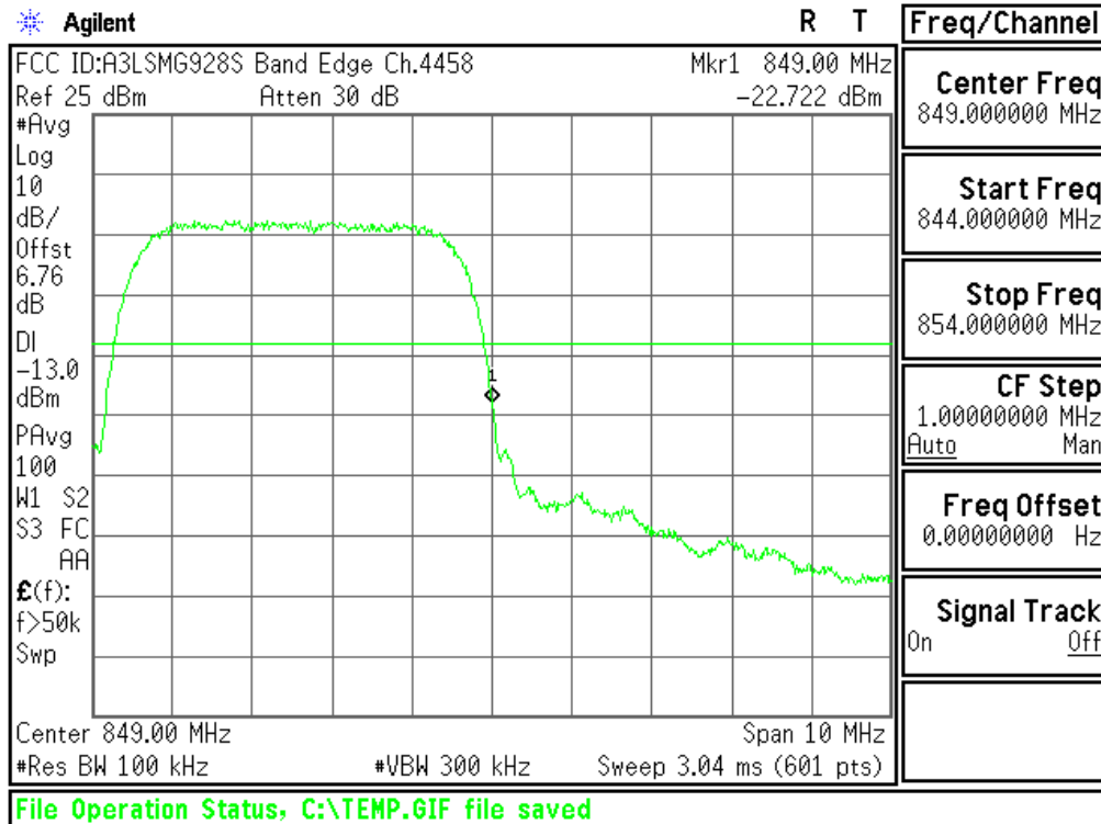
Plot 6-50. Upper Band Edge Plot (Cellular WCDMA Mode - Ch.4233(DL4458))
