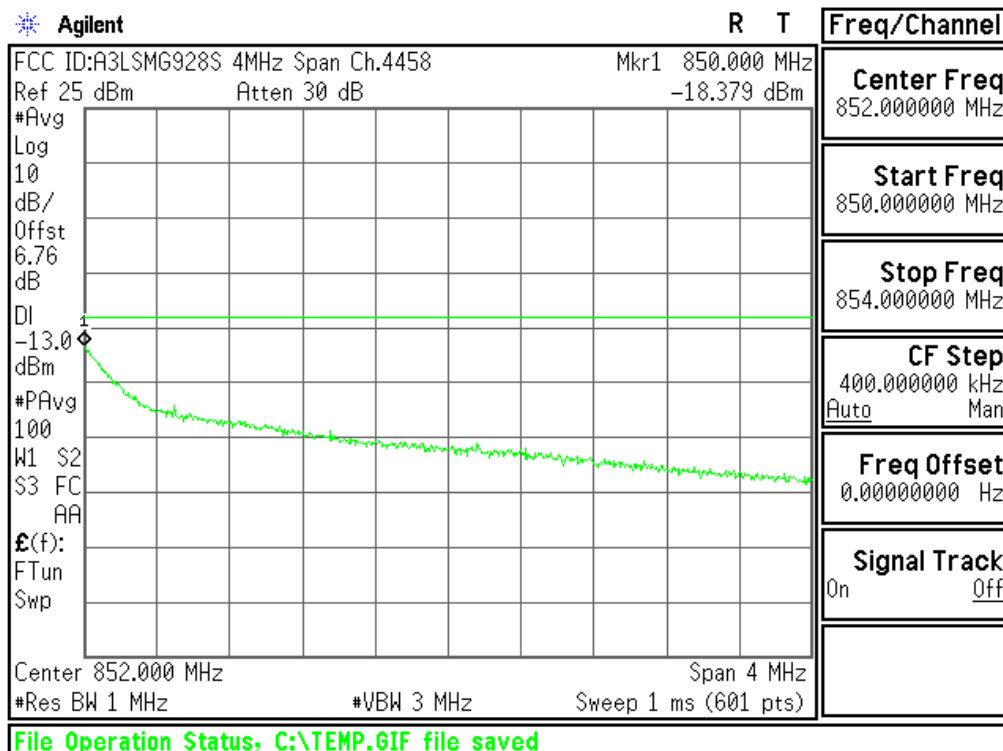
Plot 6-51. Extended Upper Band Edge Plot (Cellular WCDMA Mode - Ch.4233(DL4458))
