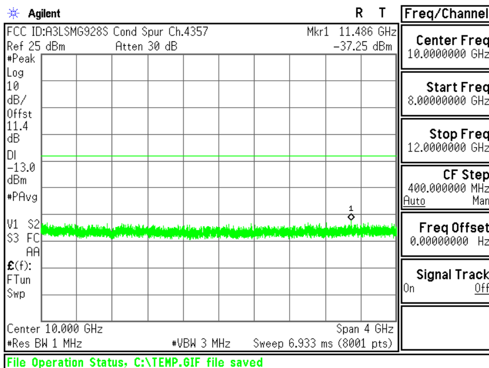
Plot 6-22. Conducted Spurious Plot (Cellular WCDMA Mode - Ch.4132(DL4357))
