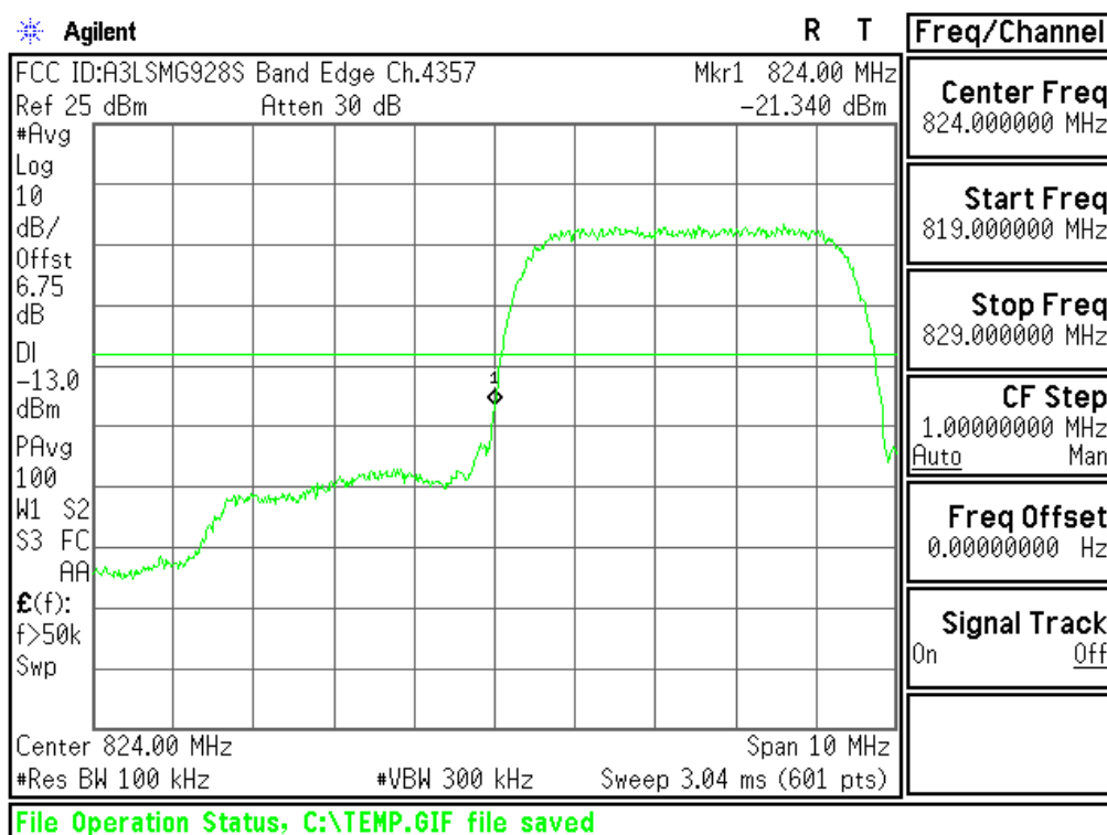
Plot 6-48. Lower Band Edge Plot (Cellular WCDMA Mode - Ch.4132(DL4357))
