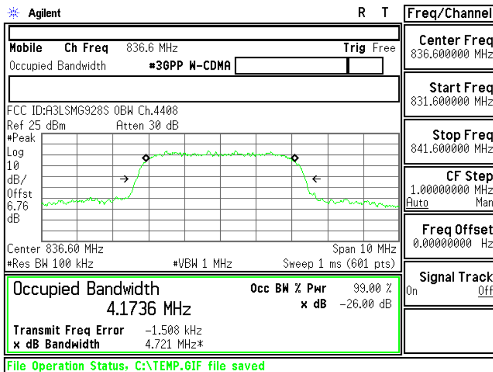
Plot 6-3. Occupied Bandwidth Plot (Cellular WCDMA Mode - Ch.4183(DL4408))
