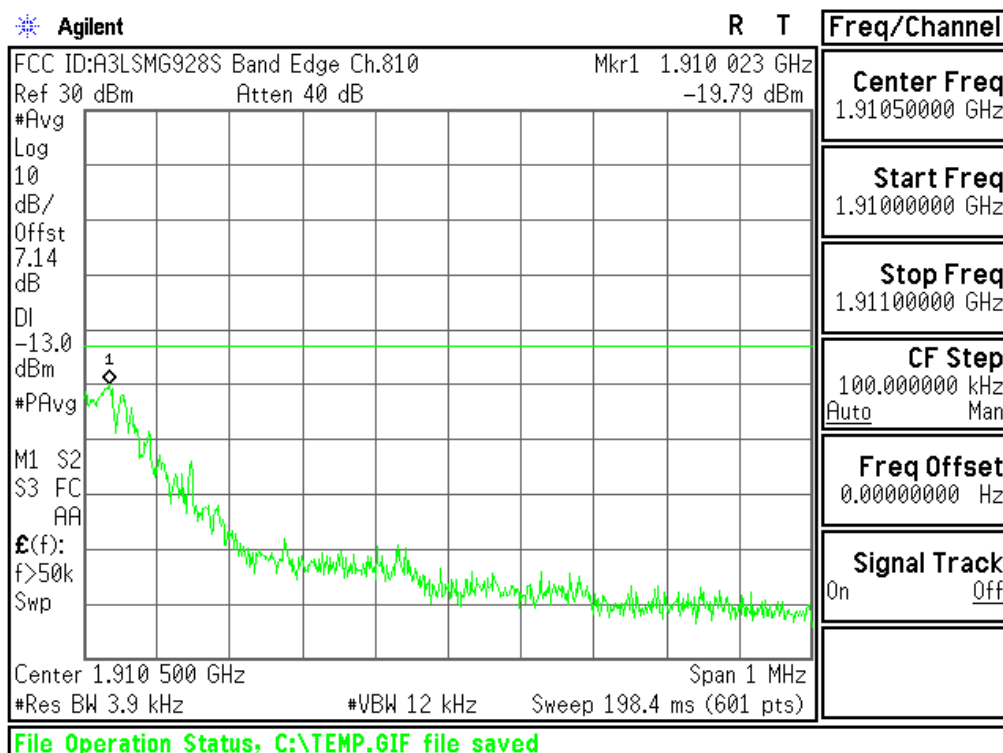
Plot 6-47. Upper Band Edge Plot (PCS GSM Mode – Ch.810)
