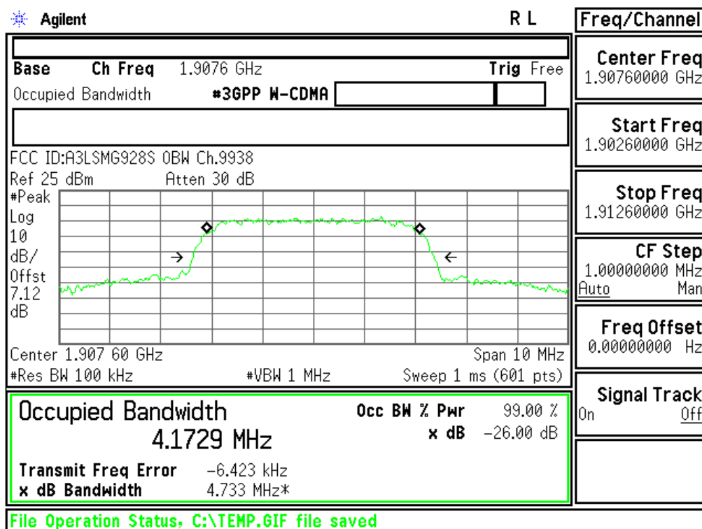
Plot 6-4. Occupied Bandwidth Plot (PCS WCDMA Mode - Ch.9538(DL9938))
