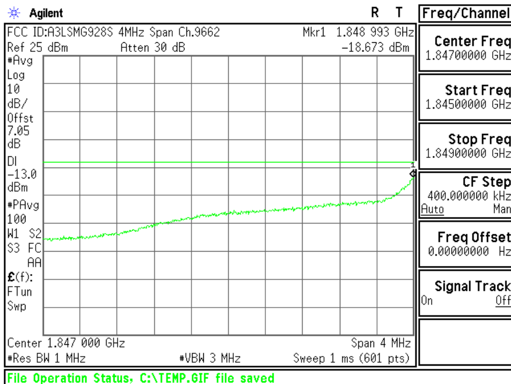
Plot 6-53. Extended Lower Band Edge Plot (PCS WCDMA Mode - Ch.9262(DL9662))
