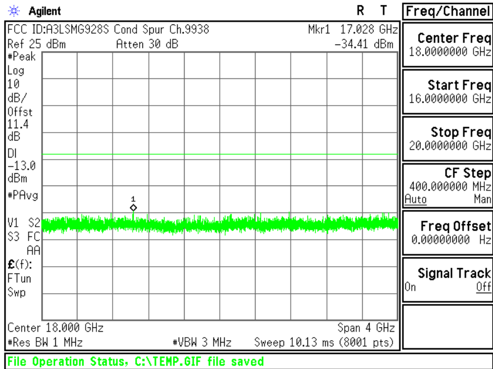
Plot 6-43. Conducted Spurious Plot (PCS WCDMA Mode - Ch.9538(DL9938))
