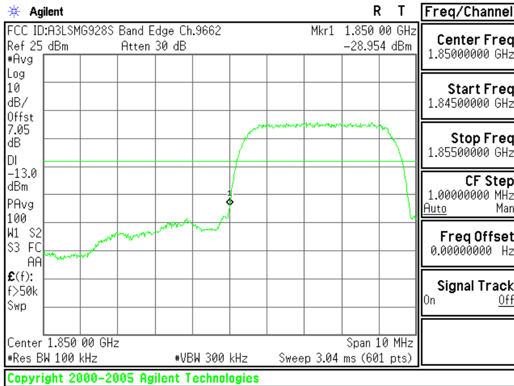
Plot 6-52. Lower Band Edge Plot (PCS WCDMA Mode - Ch.9262(DL9662))
