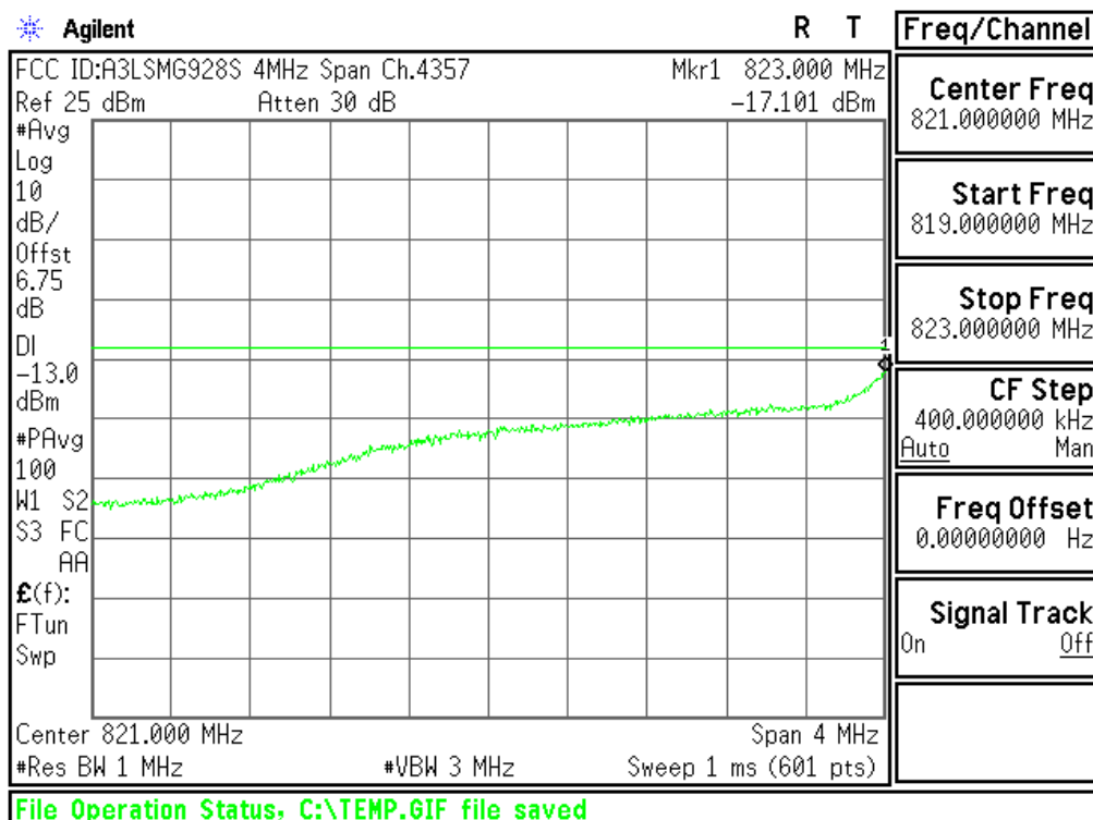
Plot 6-49. Extended Lower Band Edge Plot (Cellular WCDMA Mode - Ch.4132(DL4357))
