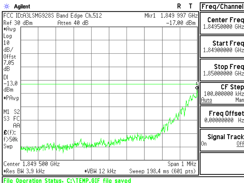
Plot 6-45. Lower Band Edge Plot (PCS GSM Mode – Ch.512)
