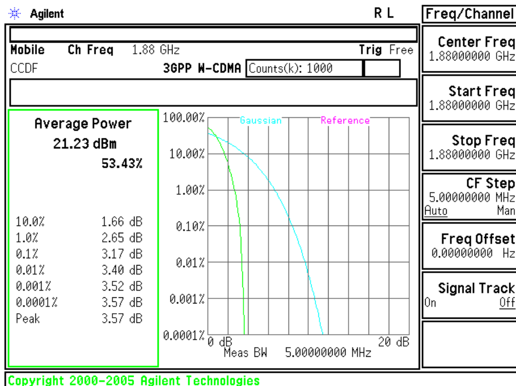
Plot 6-58. Peak-Average Ratio Plot (PCS WCDMA Mode - Ch.9400(DL9800))
