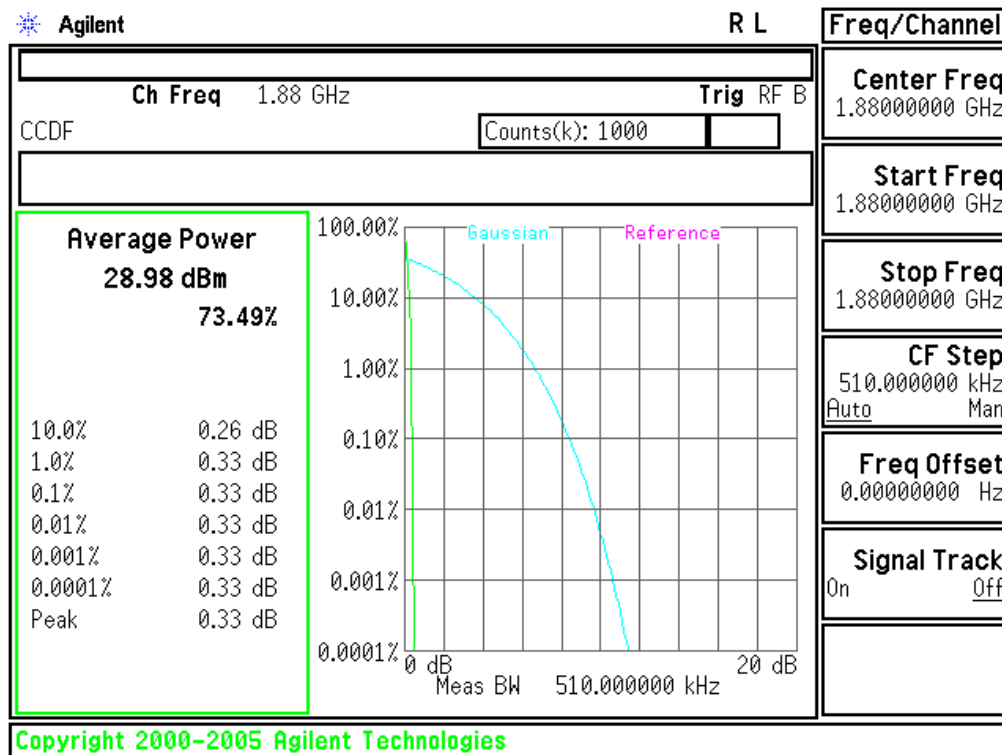
Plot 6-56. Peak-Average Ratio Plot (PCS GSM Mode - Ch.661)
