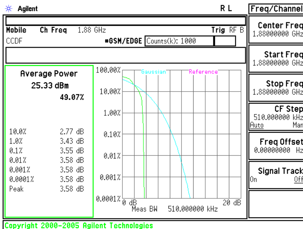
Plot 6-57. Peak-Average Ratio Plot (EDGE1900 Mode - Ch.661)
