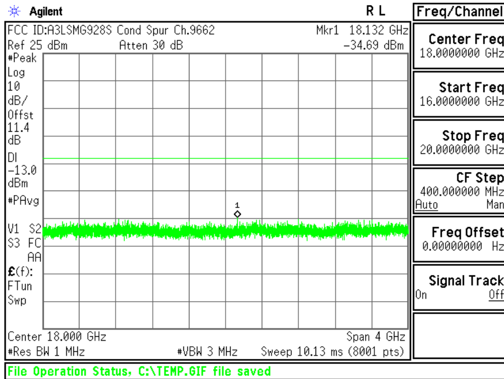
Plot 6-33. Conducted Spurious Plot (PCS WCDMA Mode - Ch.9262(DL9662))
