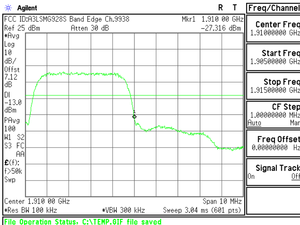
Plot 6-54. Upper Band Edge Plot (PCS WCDMA Mode - Ch.9538(DL9938))
