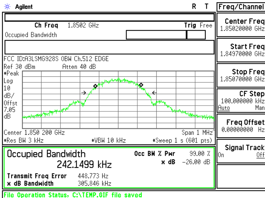
Plot 6-2. Occupied Bandwidth Plot (EDGE1900 Mode - Ch.512)
