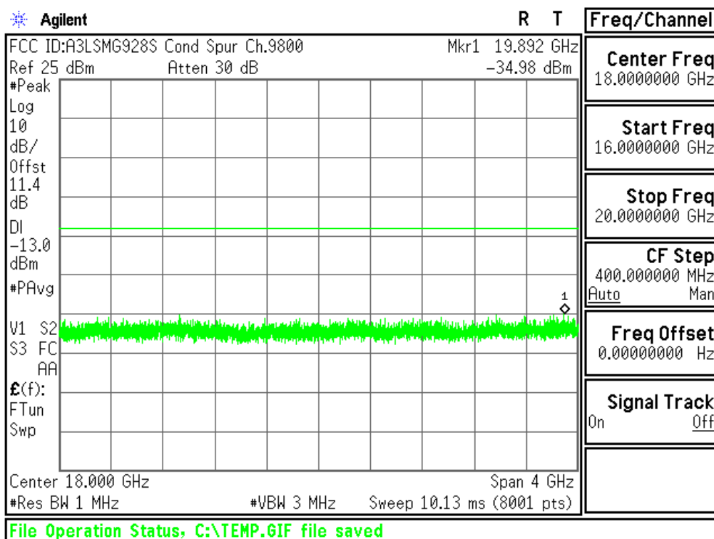
Plot 6-38. Conducted Spurious Plot (PCS WCDMA Mode - Ch.9400(DL9800))
