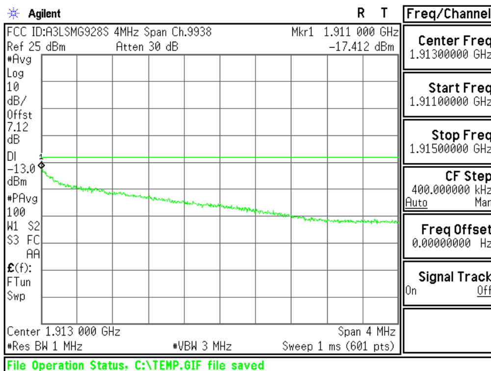
Plot 6-55. Extended Upper Band Edge Plot (PCS WCDMA Mode - Ch.9538(DL9938))
