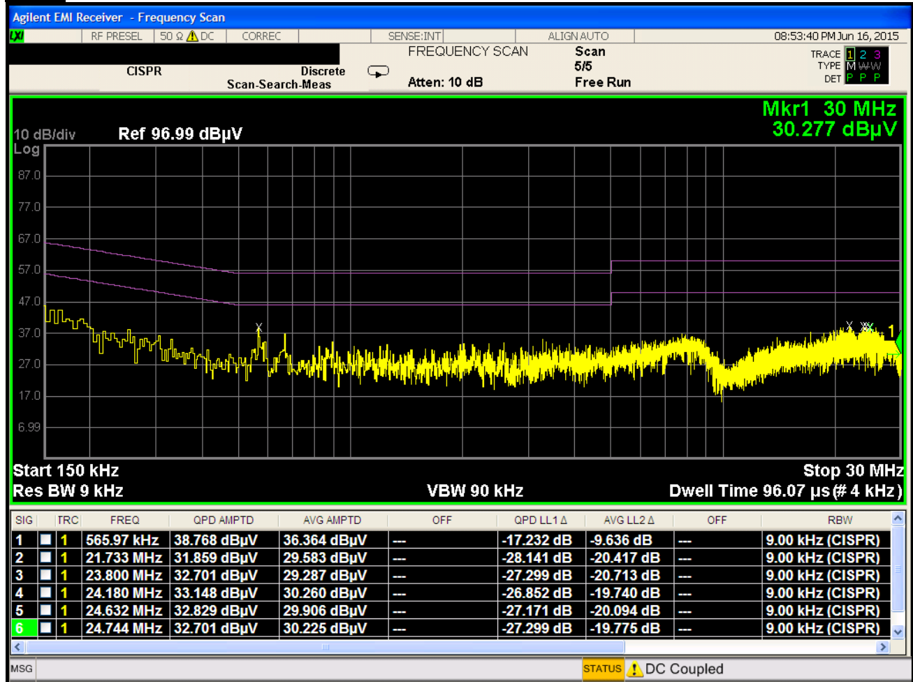
Plot 7-3. Line-Conducted Test Plot (L1) NFC Antenna Terminated in 50Ohms
