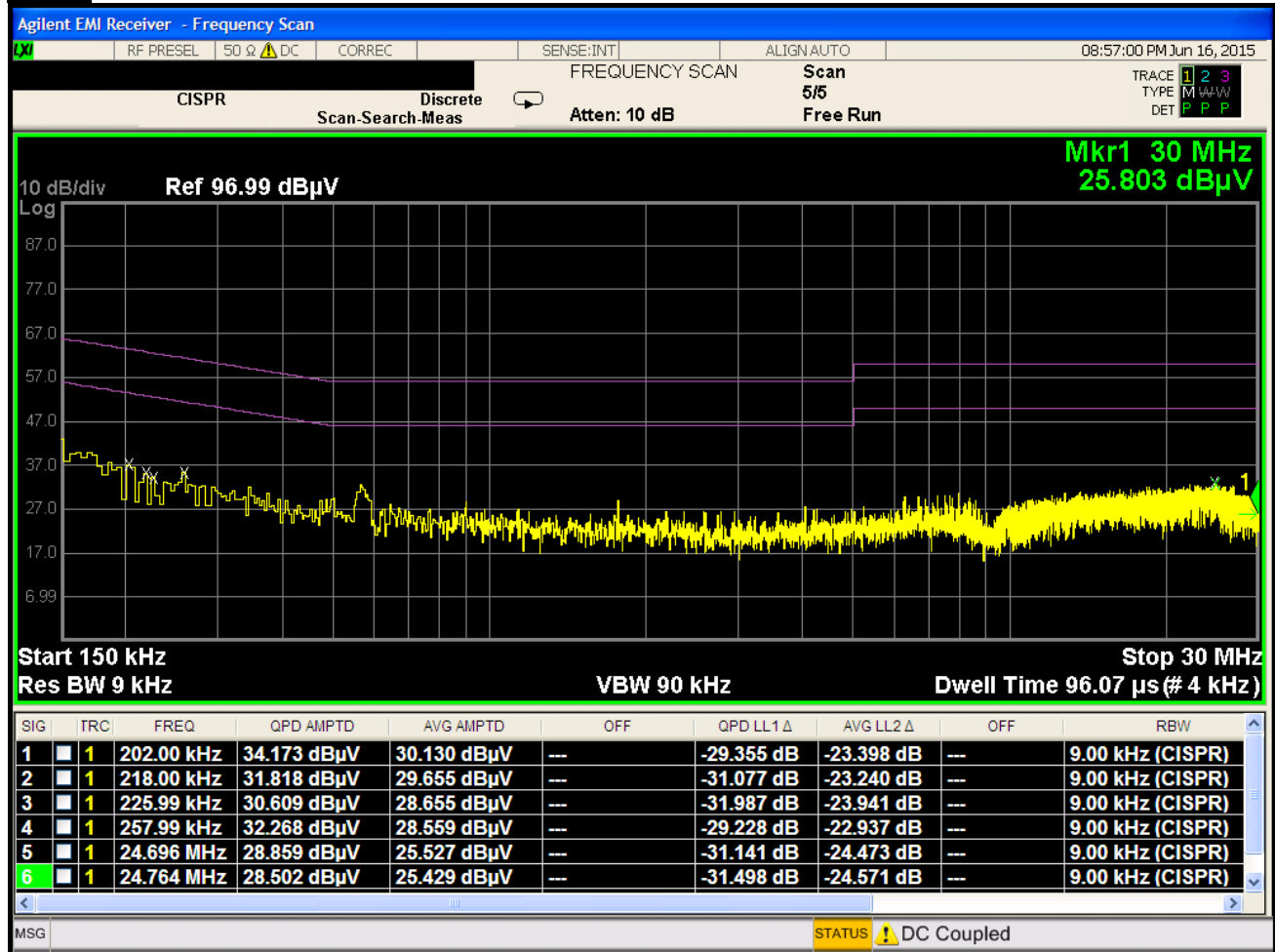
Plot 7-4. Line-Conducted Test Plot (N) NFC Antenna Terminated in 50 Ohms
