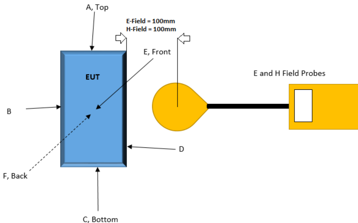
Figure 2. Test Positions and Probe Distance for Mobile Condition
