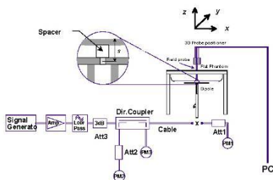
Figure 9 System Verification Setup Diagram
