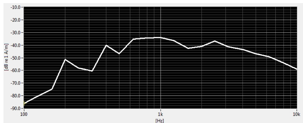
Figure 6-2 Worst-case ABM2 Plot for GSM
