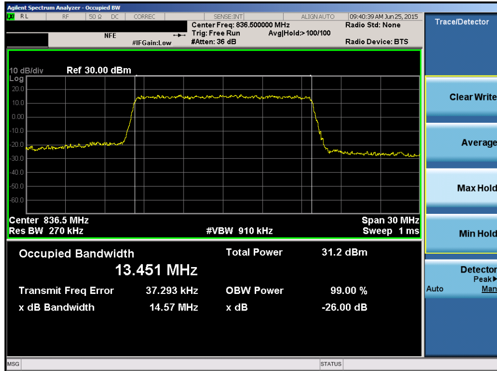
Plot 6-17. Occupied Bandwidth Plot (Band 5/26 – 15.0MHz QPSK – RB Size 75)
