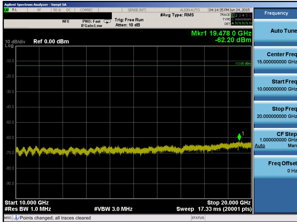
Plot 6-83. Conducted Spurious Plot (Band 25/2 – 5.0MHz QPSK – RB Size 1, RB Offset 0 – Mid Channel)
