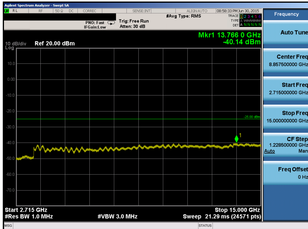
Plot 6-94. Conducted Spurious Plot (Band 41 – 5.0MHz QPSK – RB Size 1, RB Offset 0 – High Channel)
