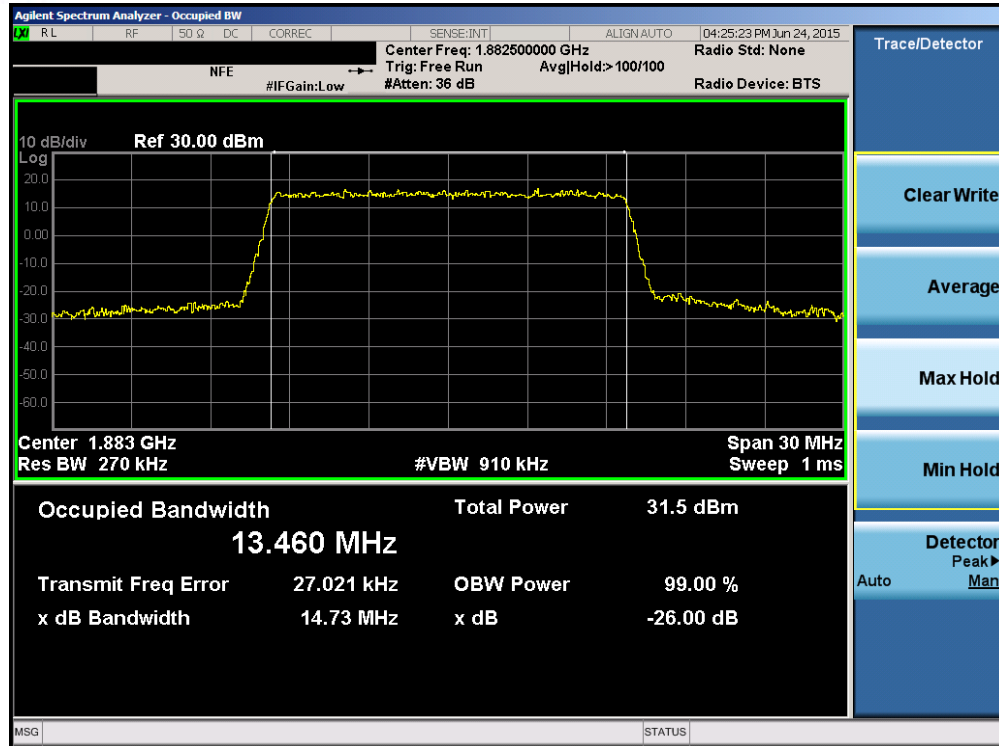
Plot 6-39. Occupied Bandwidth Plot (Band 25/2 – 15.0MHz QPSK – RB Size 75)
