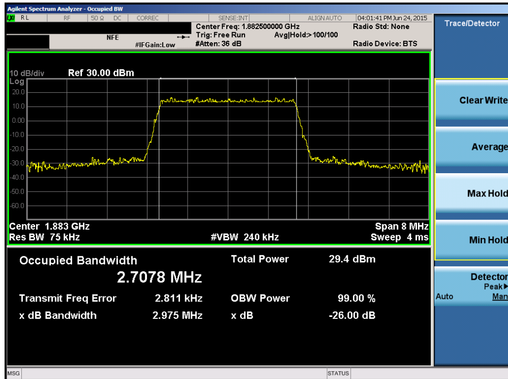
Plot 6-34. Occupied Bandwidth Plot (Band 25/2 – 3.0MHz 16-QAM – RB Size 15)
