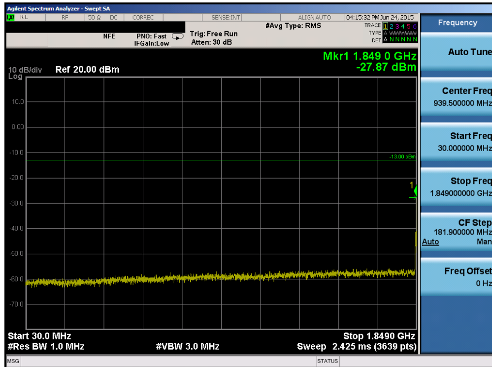
Plot 6-78. Conducted Spurious Plot (Band 25/2 – 5.0MHz QPSK – RB Size 1, RB Offset 0 – Low Channel)
