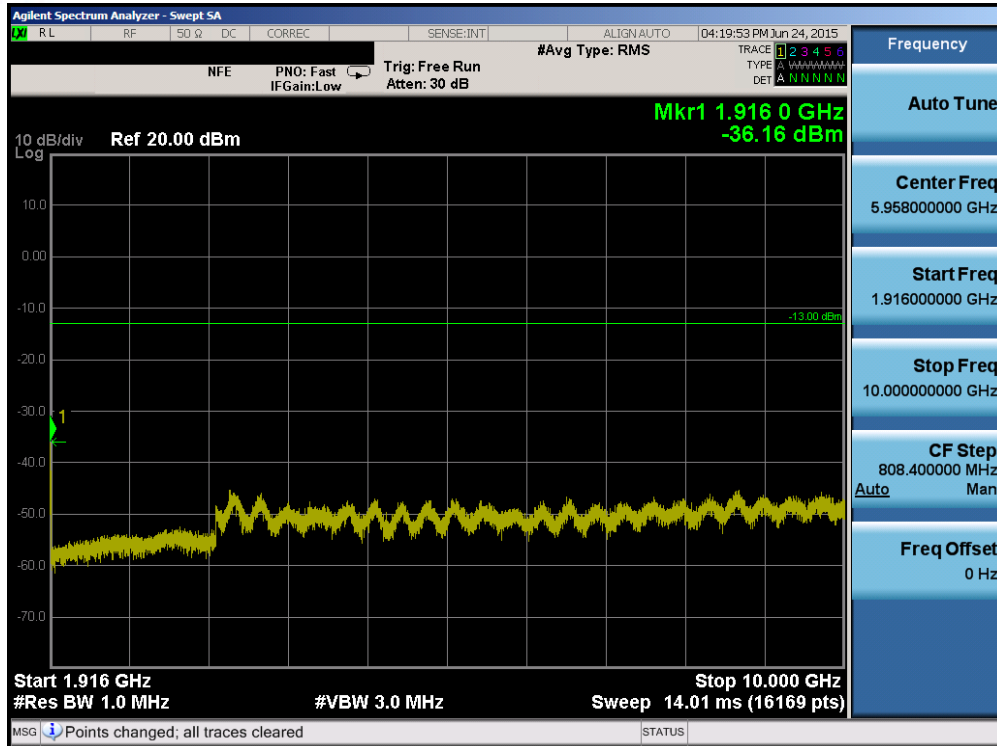
Plot 6-85. Conducted Spurious Plot (Band 25/2 – 5.0MHz QPSK – RB Size 1, RB Offset 0 – High Channel)
