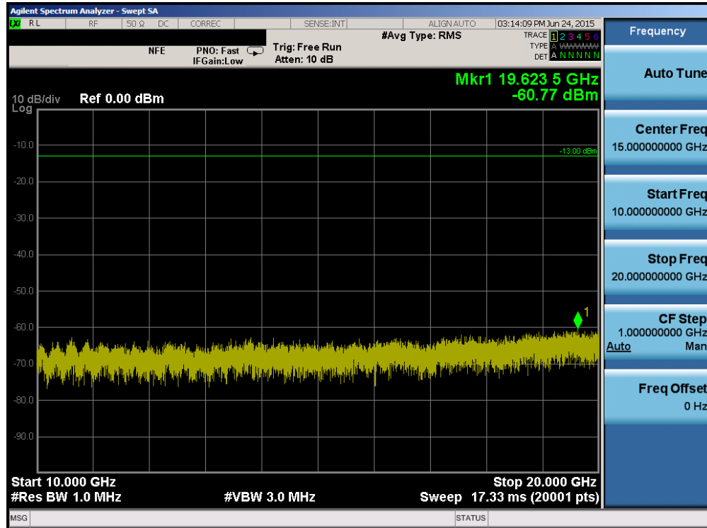
Plot 6-77. Conducted Spurious Plot (Band 4 – 10.0MHz QPSK – RB Size 1, RB Offset 0 – High Channel)
