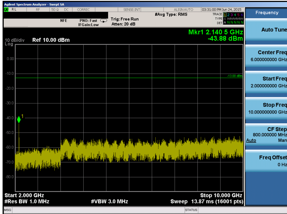
Plot 6-59. Conducted Spurious Plot (Band 12 – 5.0MHz QPSK – RB Size 1, RB Offset 0 – High Channel)
