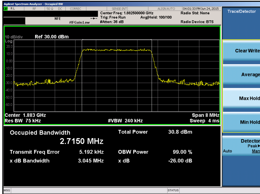
Plot 6-33. Occupied Bandwidth Plot (Band 25/2 – 3.0MHz QPSK – RB Size 15)
