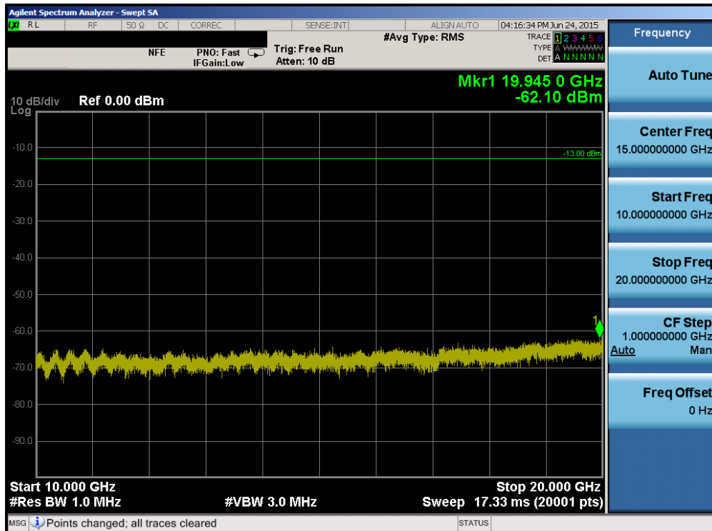
Plot 6-80. Conducted Spurious Plot (Band 25/2 – 5.0MHz QPSK – RB Size 1, RB Offset 0 – Low Channel)
