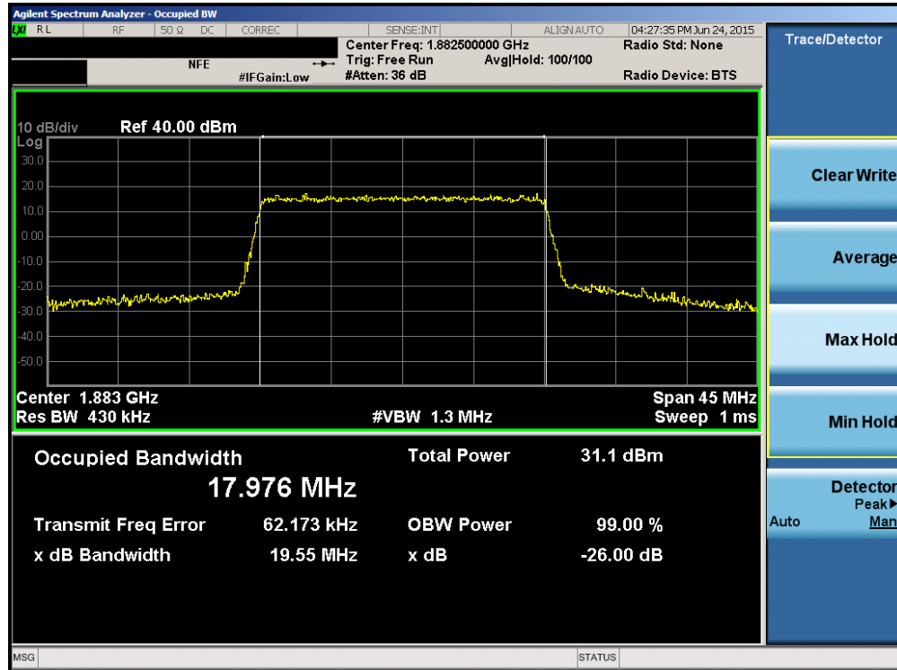
Plot 6-41. Occupied Bandwidth Plot (Band 25/2 – 20.0MHz QPSK – RB Size 100)
