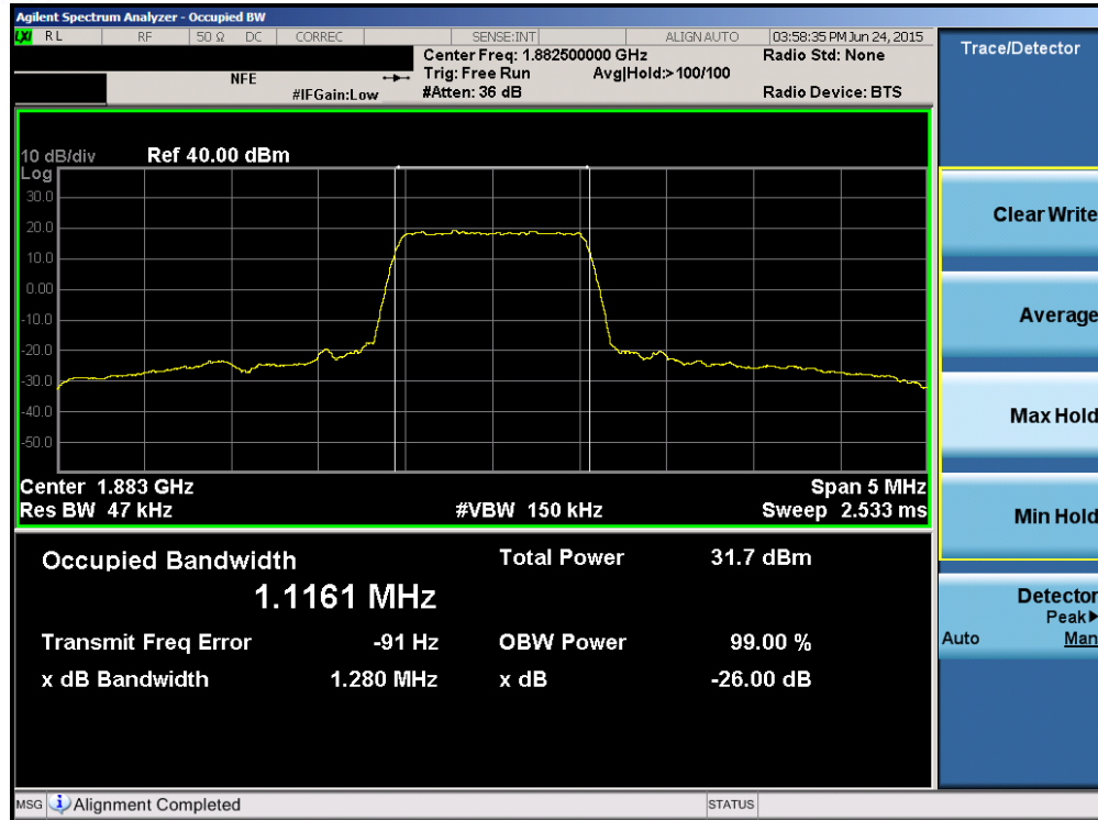
Plot 6-31. Occupied Bandwidth Plot (Band 25/2 – 1.4MHz QPSK – RB Size 6)
