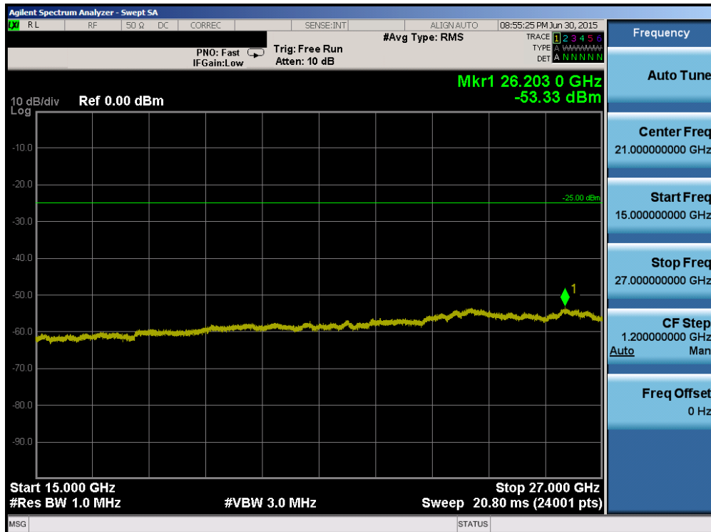
Plot 6-92. Conducted Spurious Plot (Band 41 – 5.0MHz QPSK – RB Size 1, RB Offset 0 – Mid Channel)
