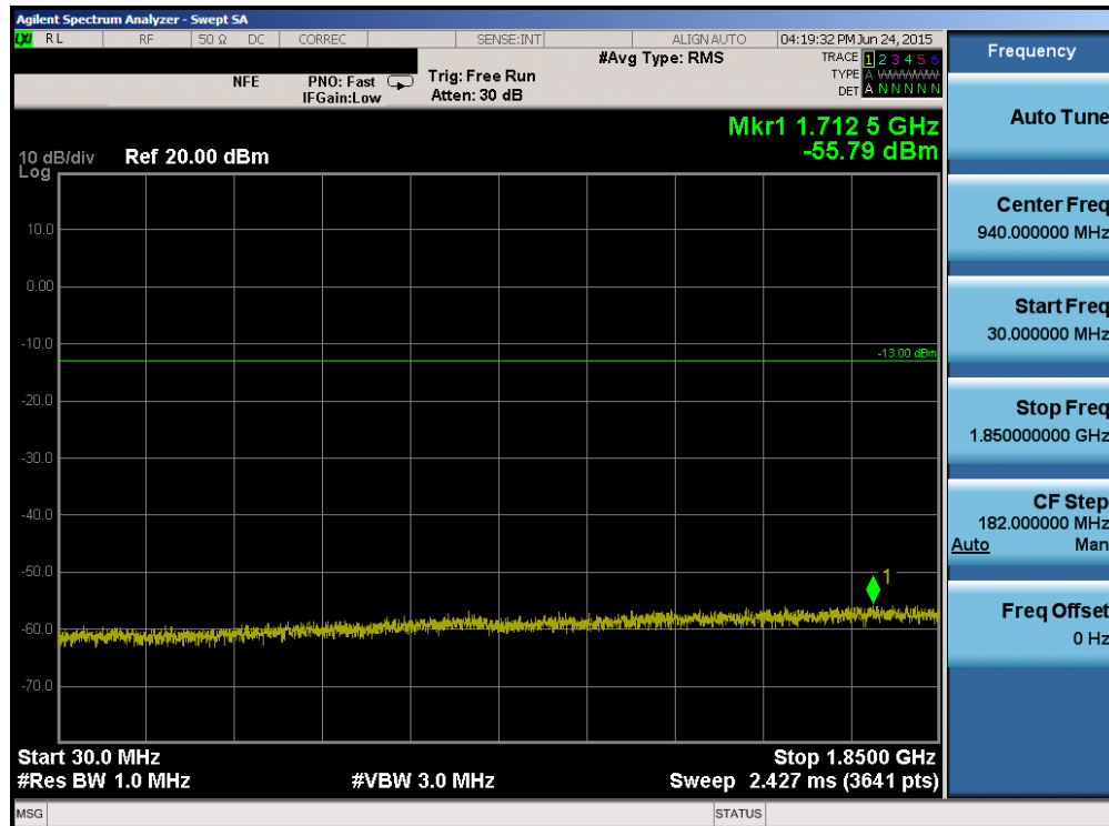
Plot 6-84. Conducted Spurious Plot (Band 25/2 – 5.0MHz QPSK – RB Size 1, RB Offset 0 – High Channel)
