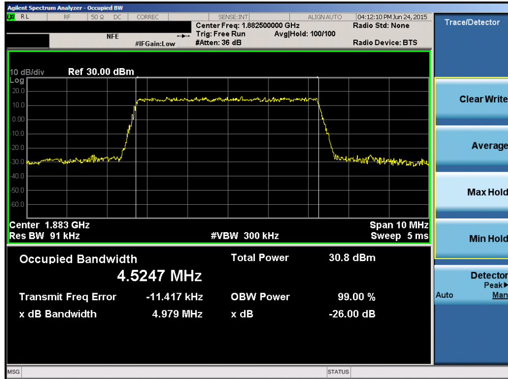
Plot 6-35. Occupied Bandwidth Plot (Band 25/2 – 5.0MHz QPSK – RB Size 25)
