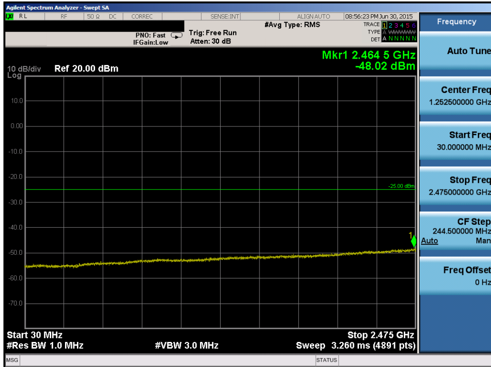
Plot 6-87. Conducted Spurious Plot (Band 41 – 5.0MHz QPSK – RB Size 1, RB Offset 0 – Low Channel)
