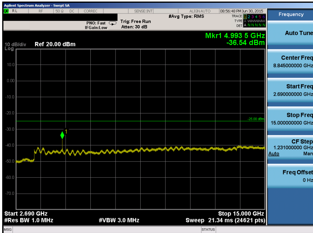
Plot 6-88. Conducted Spurious Plot (Band 41 – 5.0MHz QPSK – RB Size 1, RB Offset 0 – Low Channel)
