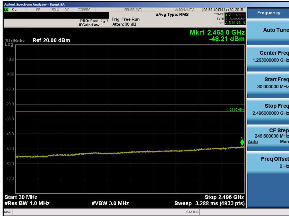
Plot 6-93. Conducted Spurious Plot (Band 41 – 5.0MHz QPSK – RB Size 1, RB Offset 0 – High Channel)
