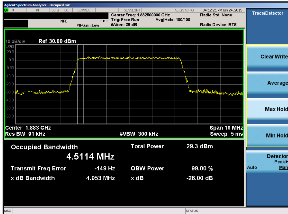
Plot 6-36. Occupied Bandwidth Plot (Band 25/2 – 5.0MHz 16-QAM – RB Size 25)
