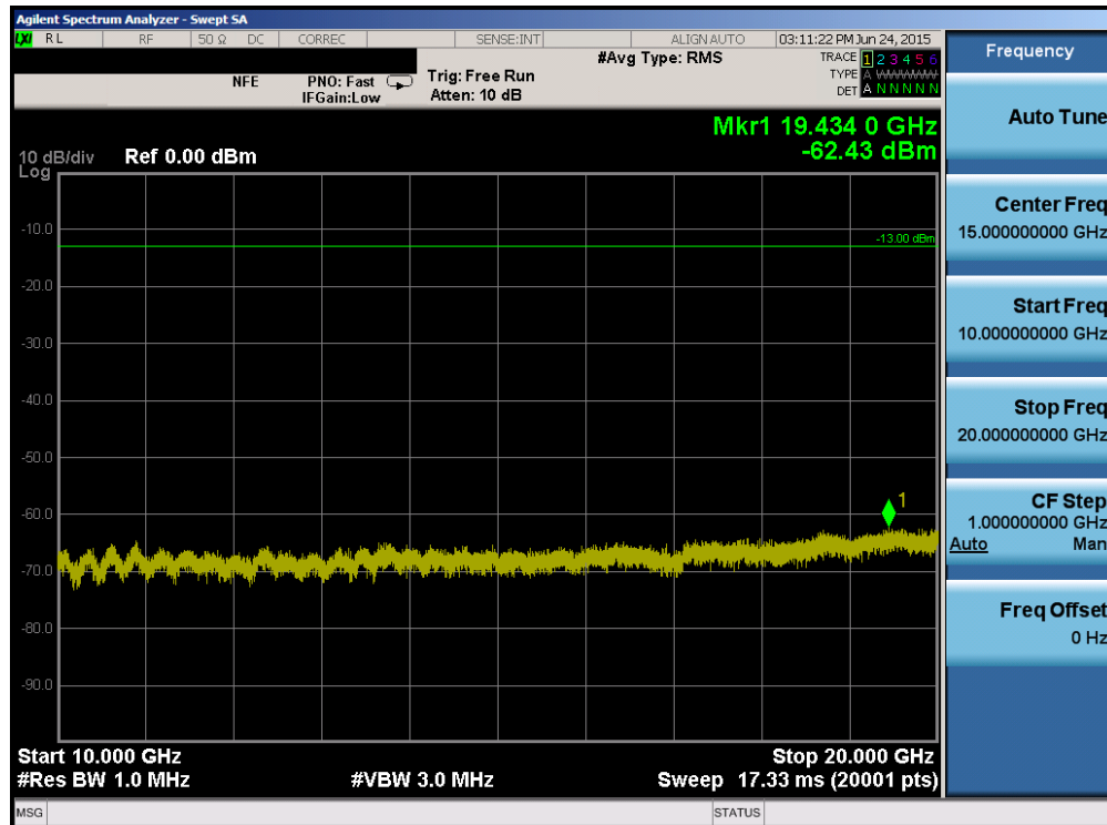
Plot 6-74. Conducted Spurious Plot (Band 4 – 10.0MHz QPSK – RB Size 1, RB Offset 0 – Mid Channel)
