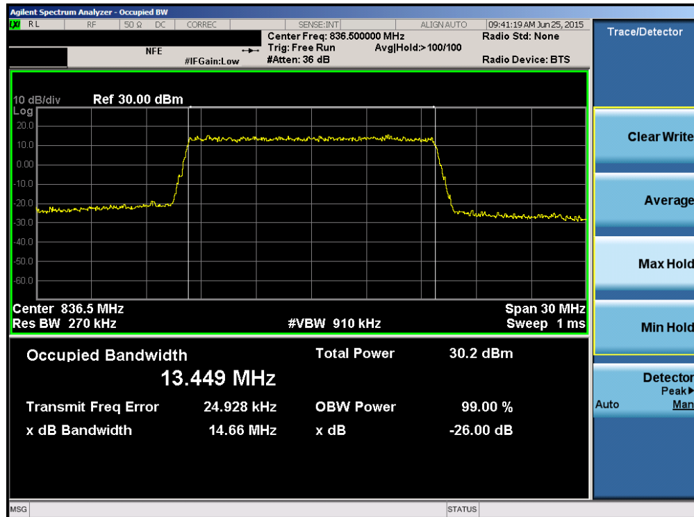
Plot 6-18. Occupied Bandwidth Plot (Band 5/26 – 15.0MHz 16-QAM – RB Size 75)
