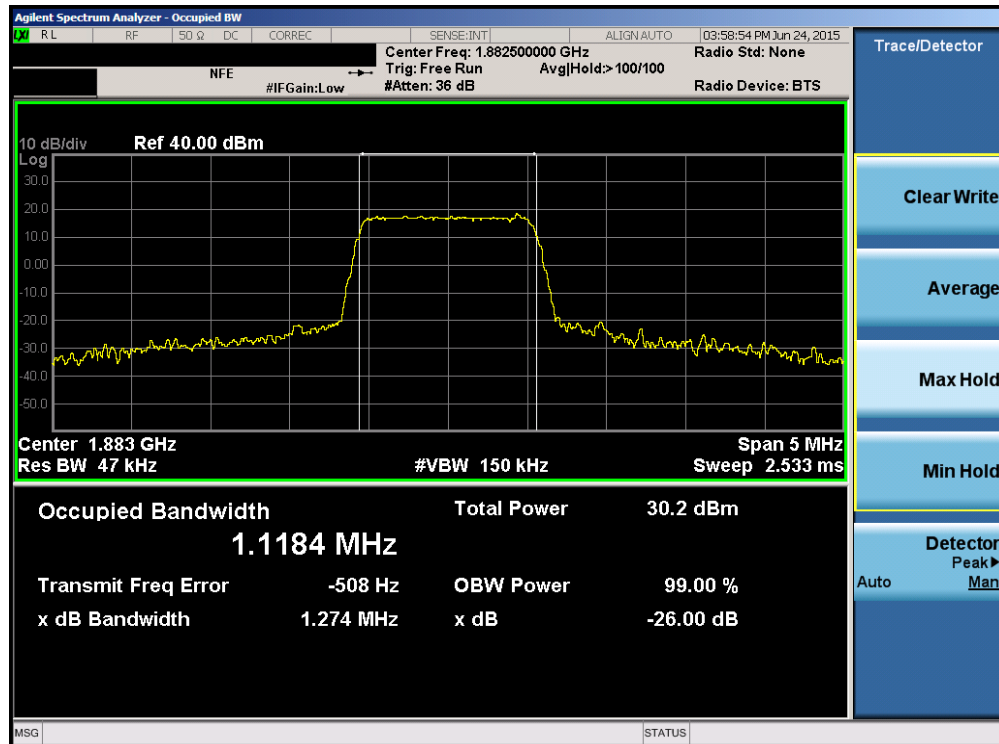
Plot 6-32. Occupied Bandwidth Plot (Band 25/2 – 1.4MHz 16-QAM – RB Size 6)
