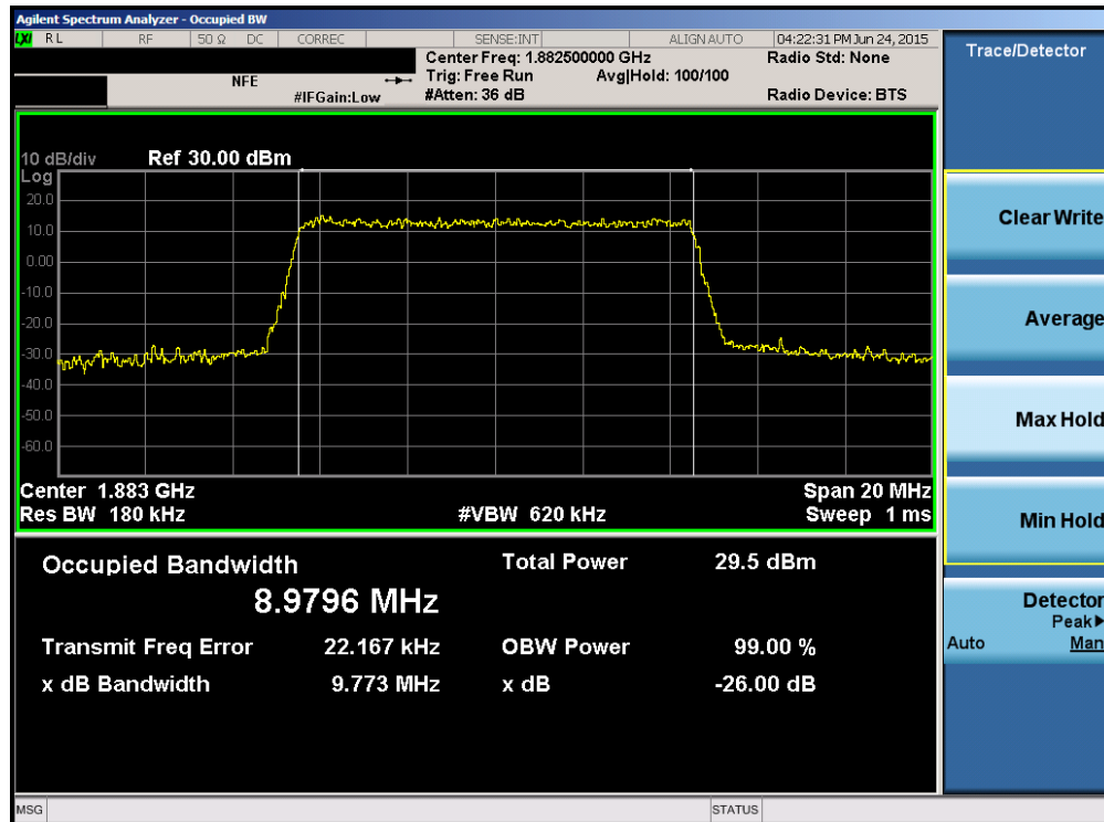
Plot 6-38. Occupied Bandwidth Plot (Band 25/2 – 10.0MHz 16-QAM – RB Size 50)
