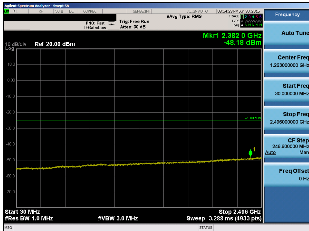
Plot 6-90. Conducted Spurious Plot (Band 41 – 5.0MHz QPSK – RB Size 1, RB Offset 0 – Mid Channel)
