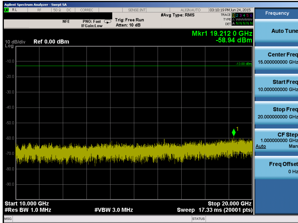
Plot 6-71. Conducted Spurious Plot (Band 4 – 10.0MHz QPSK – RB Size 1, RB Offset 0 – Low Channel)
