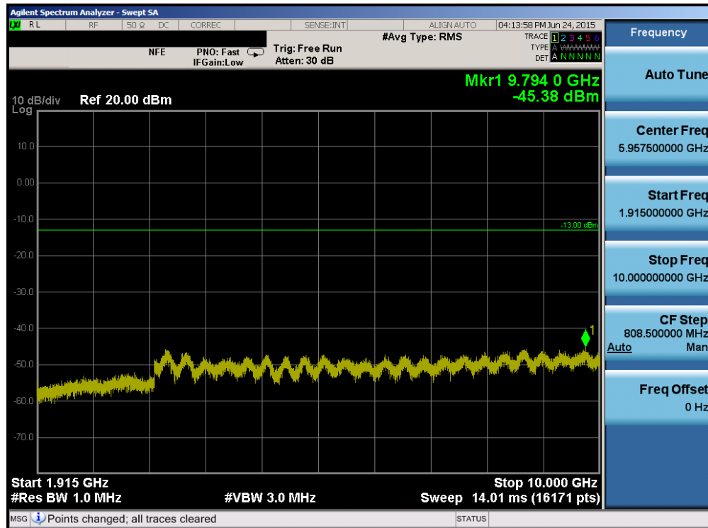
Plot 6-82. Conducted Spurious Plot (Band 25/2 – 5.0MHz QPSK – RB Size 1, RB Offset 0 – Mid Channel)
