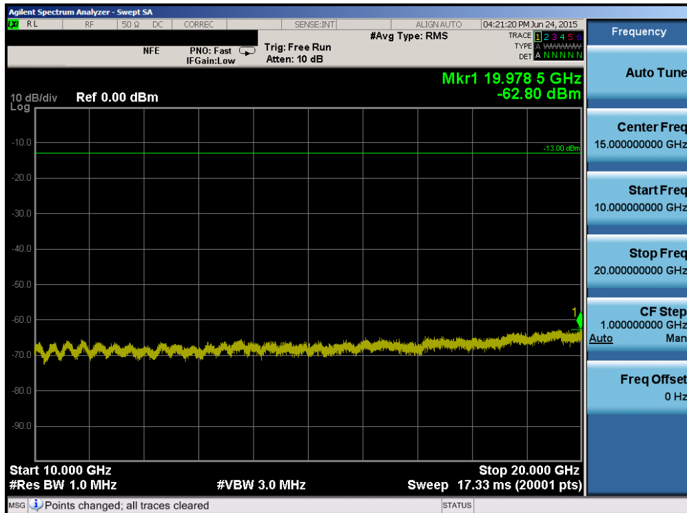
Plot 6-86. Conducted Spurious Plot (Band 25/2 – 5.0MHz QPSK – RB Size 1, RB Offset 0 – High Channel)
