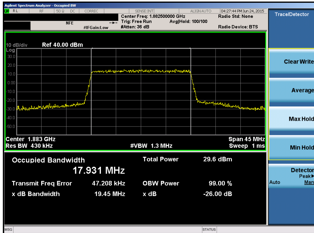
Plot 6-42. Occupied Bandwidth Plot (Band 25/2 – 20.0MHz 16-QAM – RB Size 100)
