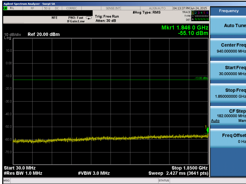
Plot 6-81. Conducted Spurious Plot (Band 25/2 – 5.0MHz QPSK – RB Size 1, RB Offset 0 – Mid Channel)
