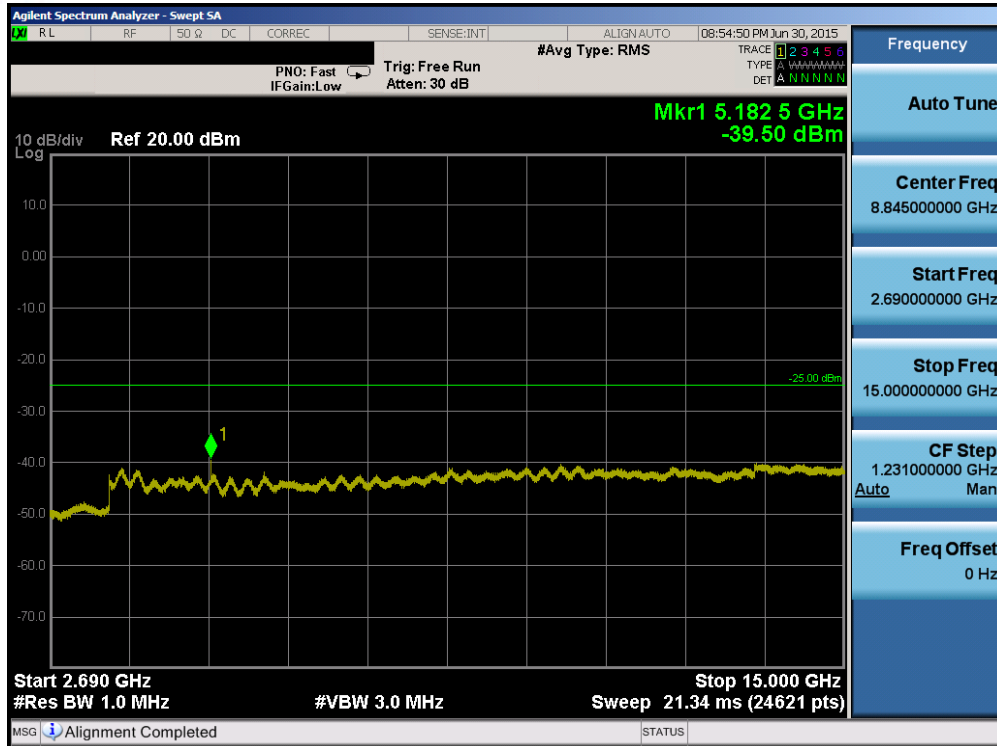
Plot 6-91. Conducted Spurious Plot (Band 41 – 5.0MHz QPSK – RB Size 1, RB Offset 0 – Mid Channel)
