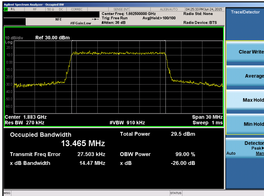
Plot 6-40. Occupied Bandwidth Plot (Band 25/2 – 15.0MHz 16-QAM – RB Size 75)
