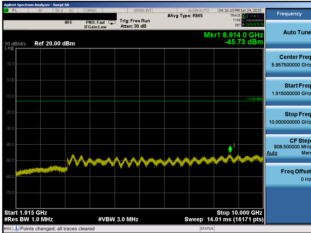
Plot 6-79. Conducted Spurious Plot (Band 25/2 – 5.0MHz QPSK – RB Size 1, RB Offset 0 – Low Channel)
