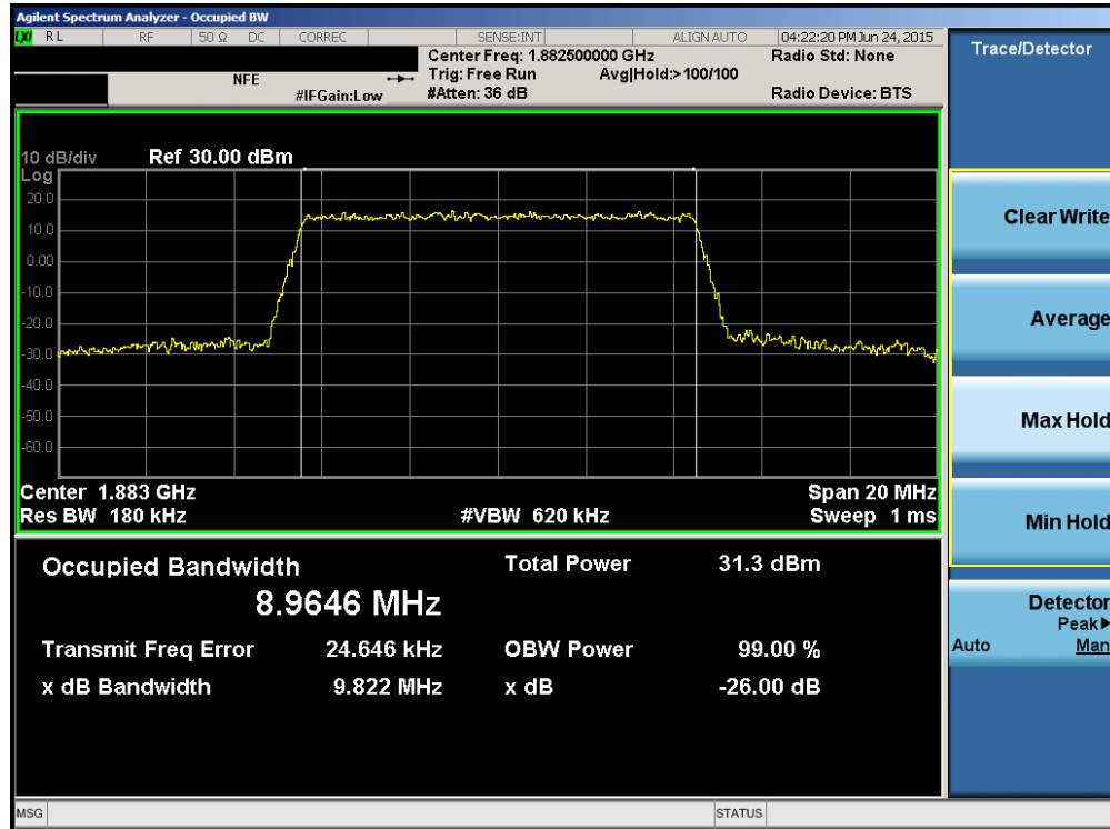
Plot 6-37. Occupied Bandwidth Plot (Band 25/2 – 10.0MHz QPSK – RB Size 50)
