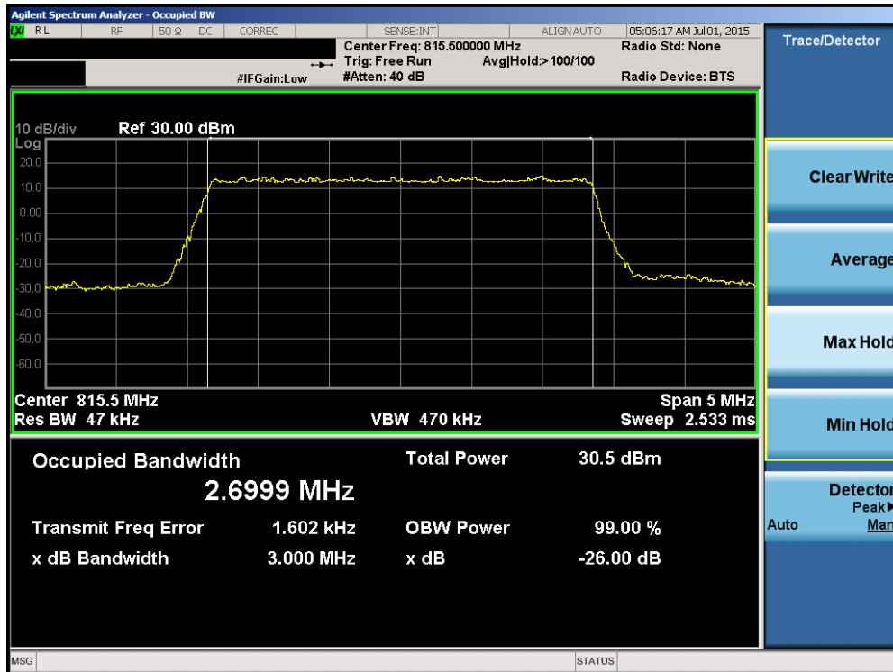
Plot 8-9. Occupied Bandwidth Plot (3MHz 16-QAM – RB Size 15– Low Channel)
