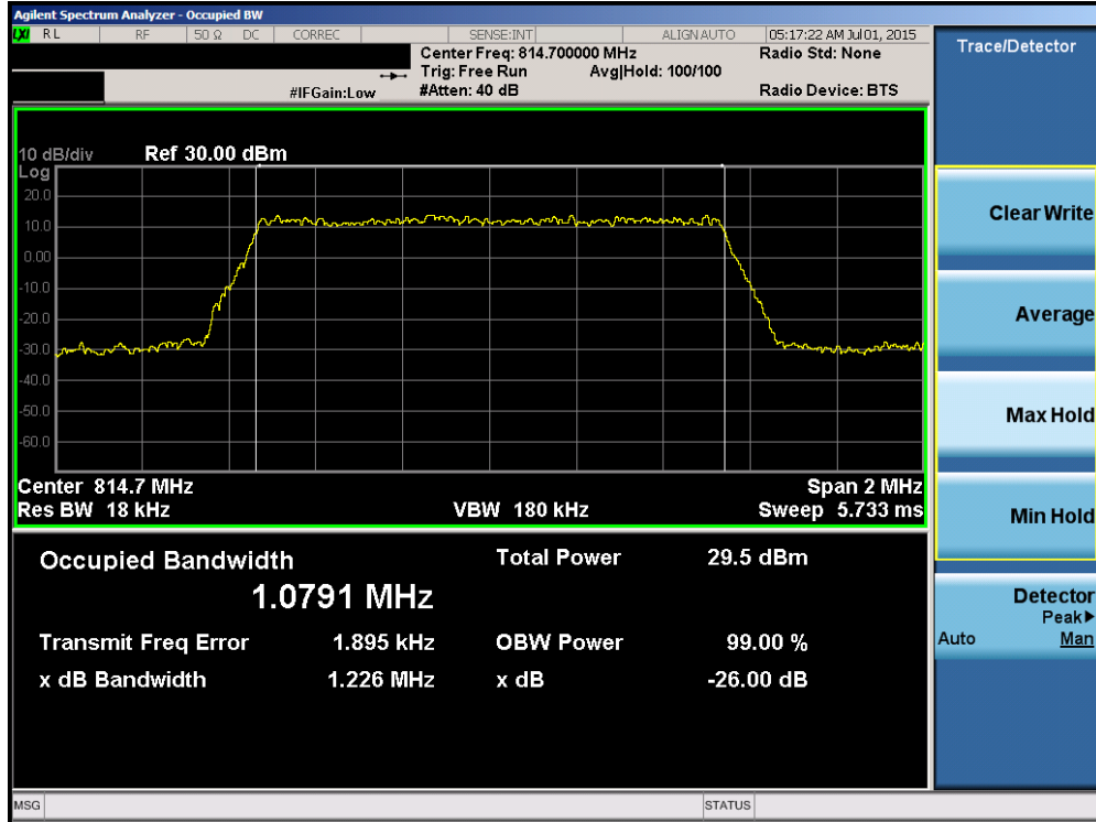
Plot 8-3. Occupied Bandwidth Plot (1.4MHz 16-QAM – RB Size 6– Low Channel)
