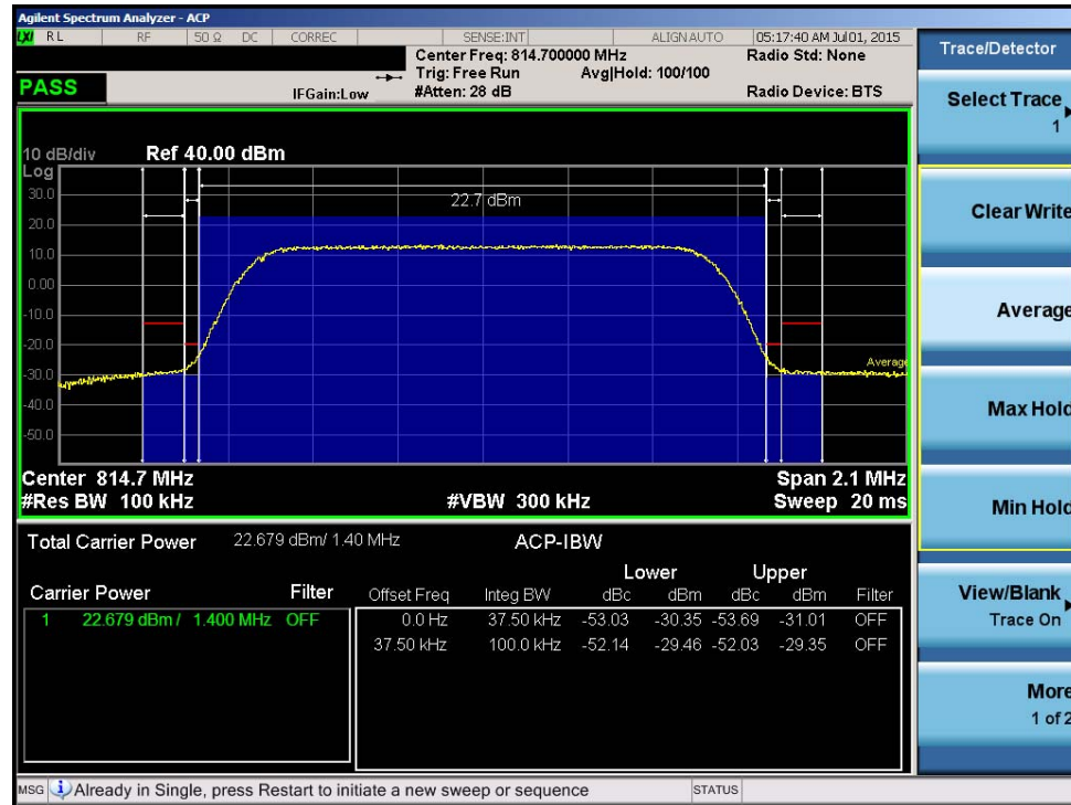
Plot 8-1. Channel Edge Plot (1.4MHz QPSK - RB Size 6- Low Channel)
