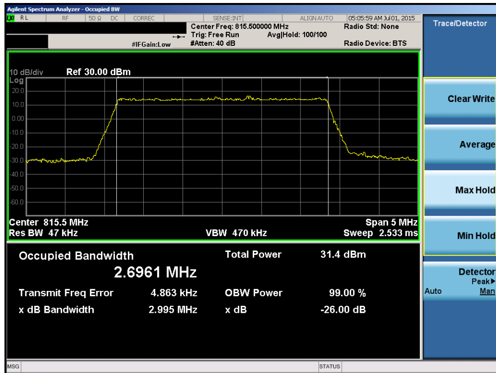
Plot 8-8. Occupied Bandwidth Plot (3MHz QPSK – RB Size 15– Low Channel)
