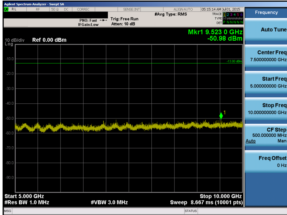
Plot 8-11. Conducted Spurious Plot (1.4MHz QPSK – RB Size 1, RB Offset 0 – High Channel)
