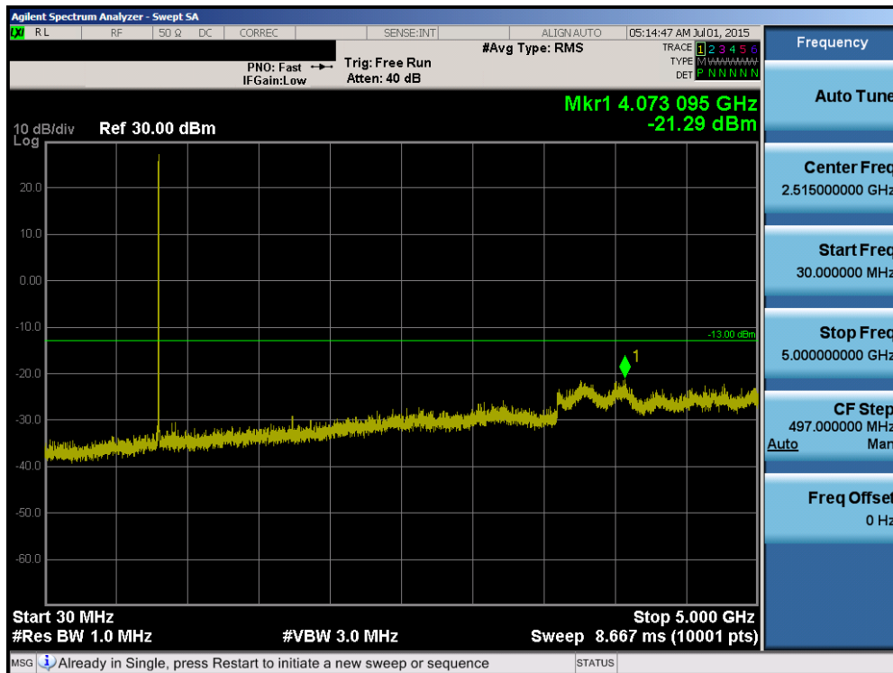
Plot 8-10. Conducted Spurious Plot (1.4MHz QPSK – RB Size 1, RB Offset 0 – High Channel)
