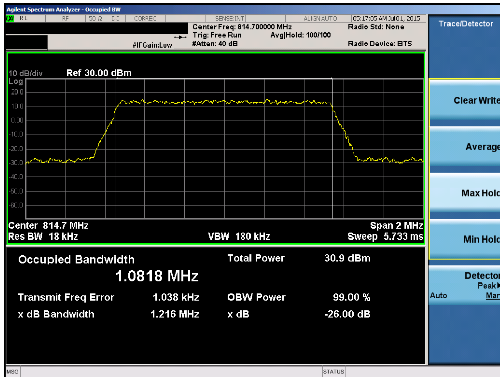
Plot 8-2. Occupied Bandwidth Plot (1.4MHz QPSK - RB Size 6- Low Channel)
