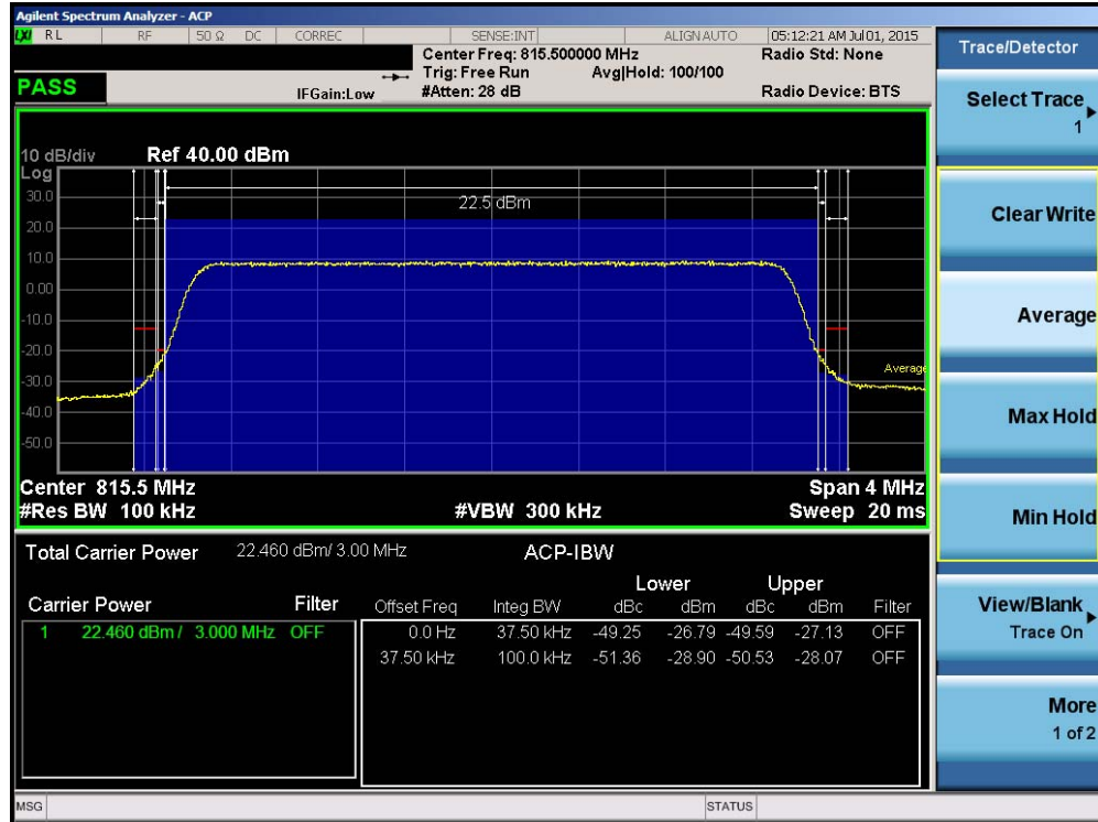
Plot 8-7. Channel Edge Plot (3MHz QPSK – RB Size 15– Low Channel)
