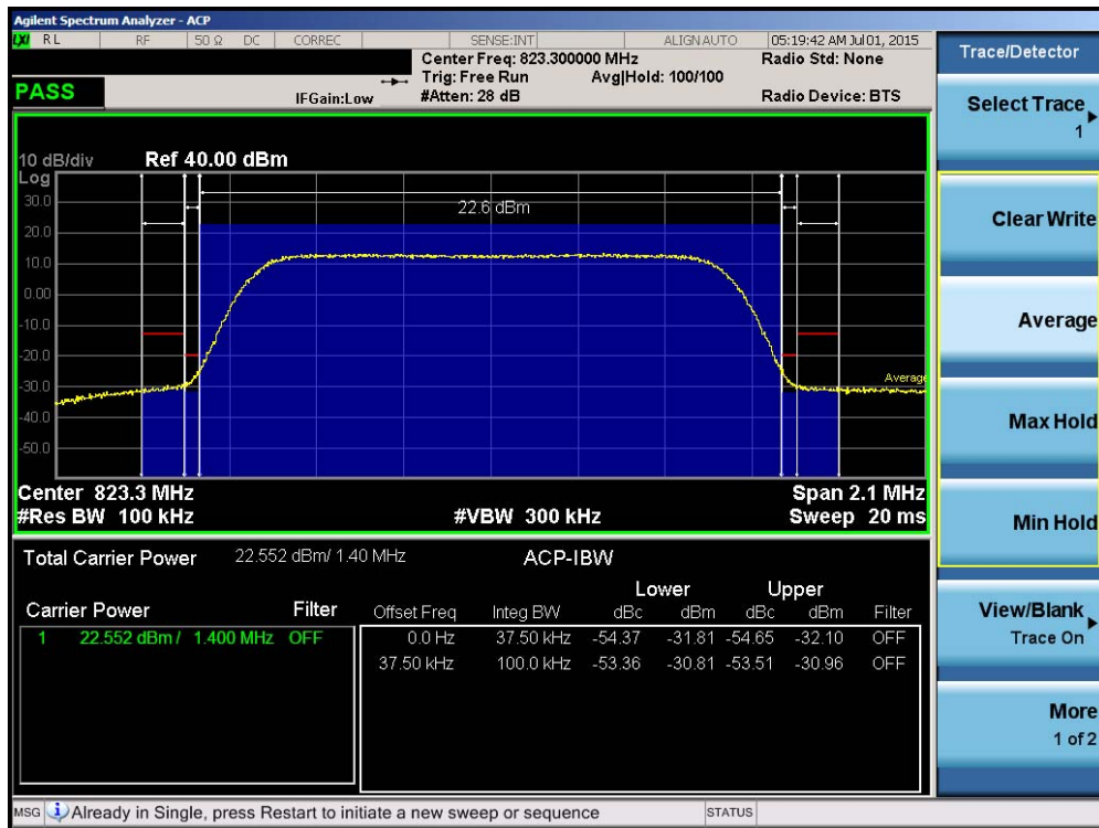
Plot 8-4. Channel Edge Plot (1.4MHz QPSK – RB Size 6 – High Channel)
