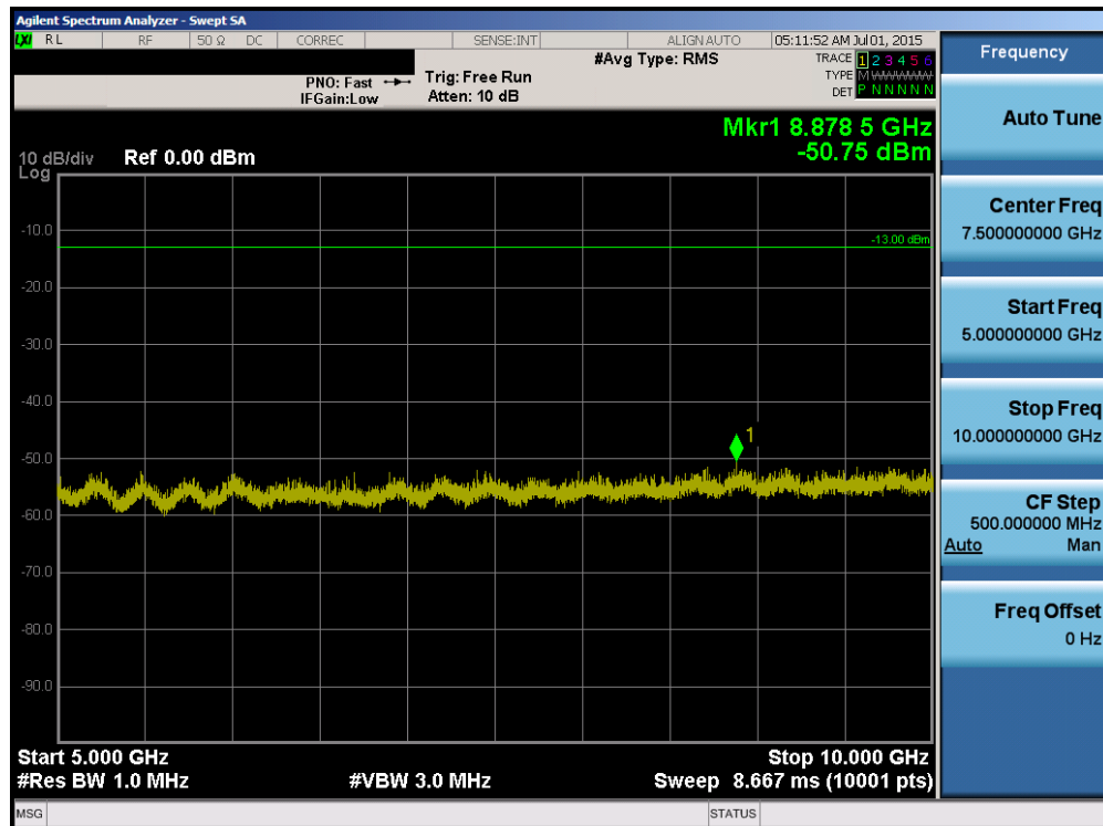
Plot 8-6. Conducted Spurious Plot (1.4MHz QPSK – RB Size 1, RB Offset 0 – Low Channel)
