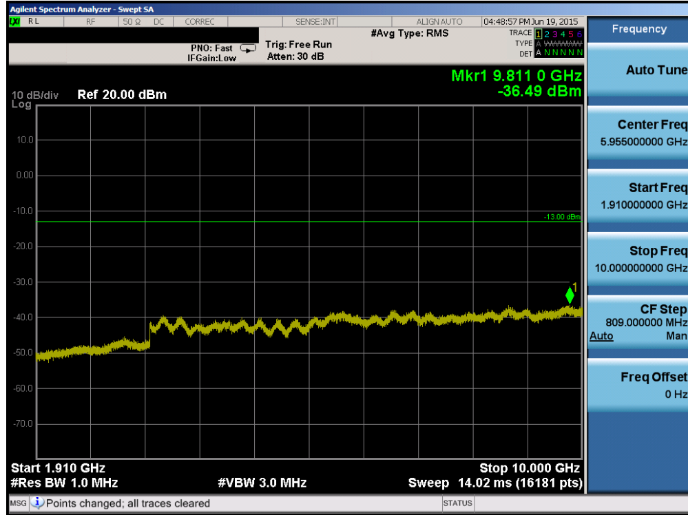
Plot 6-55. Conducted Spurious Plot (PCS WCDMA Mode – Ch. 9262)
