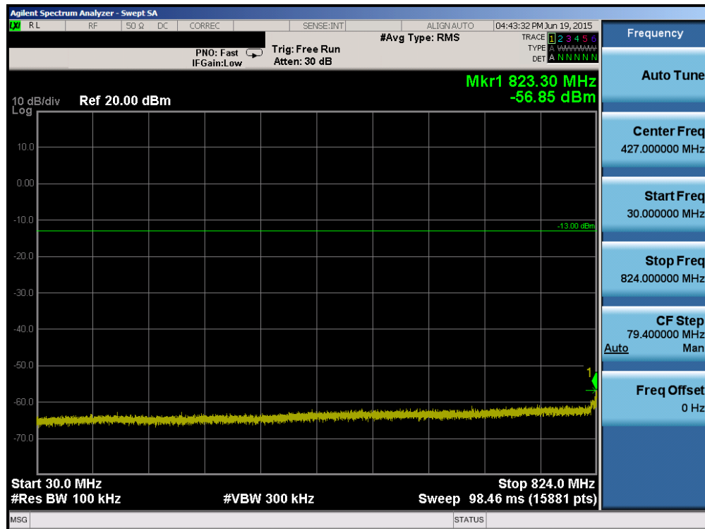
Plot 6-48. Conducted Spurious Plot (Cellular WCDMA Mode – Ch. 4183)
