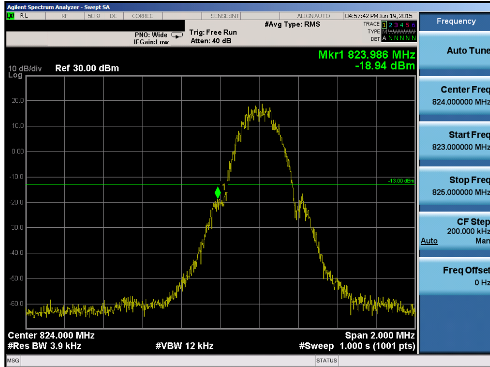
Plot 6-63. Band Edge Plot (Cellular GSM Mode – Ch. 128)
