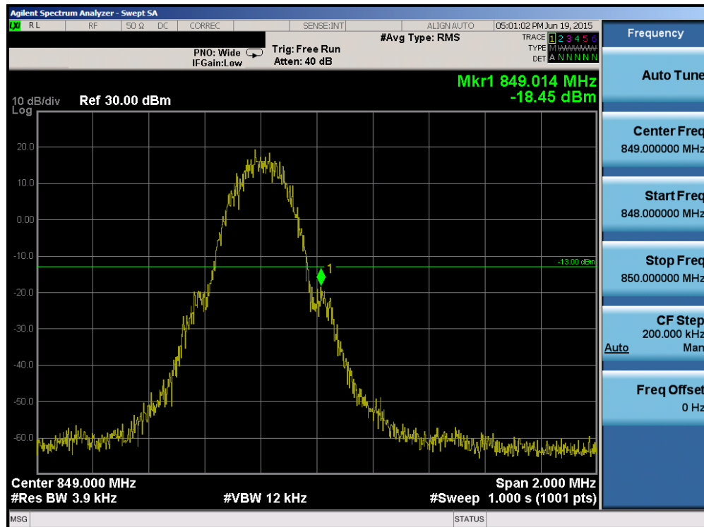
Plot 6-64. Band Edge Plot (Cellular GSM Mode – Ch. 251)
