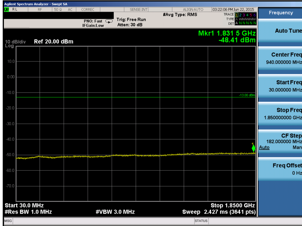
Plot 6-39. Conducted Spurious Plot (PCS CDMA Mode – Ch. 600)
