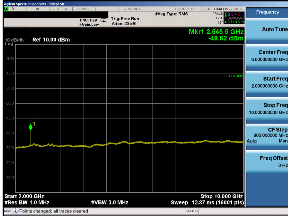
Plot 6-35. Conducted Spurious Plot (Cellular CDMA Mode – Ch. 777)
