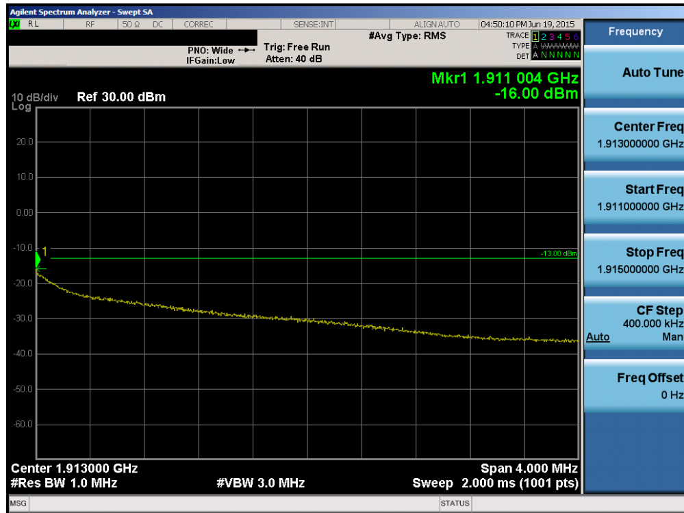
Plot 6-82. 4MHz Span Plot (PCS WCDMA Mode – Ch. 9538)
