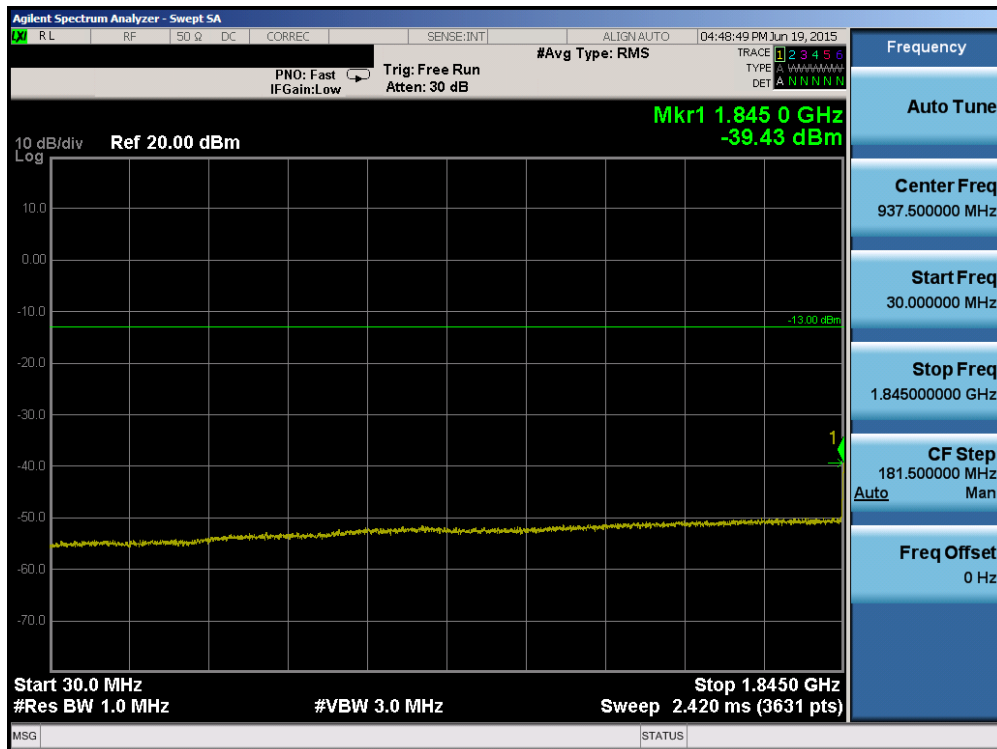
Plot 6-54. Conducted Spurious Plot (PCS WCDMA Mode – Ch. 9262)
