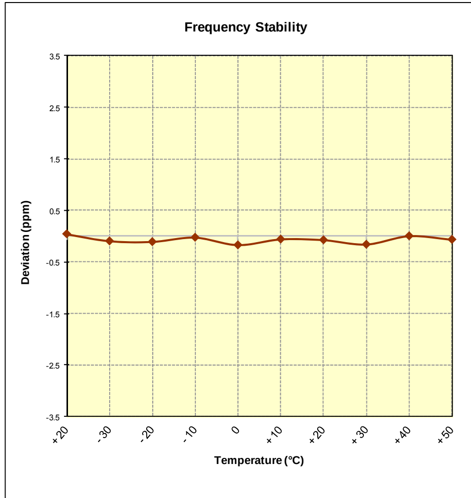
Figure 6-11. Frequency Stability Graph (PCS CDMA Mode – Ch. 600)
