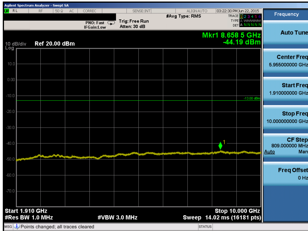
Plot 6-40. Conducted Spurious Plot (PCS CDMA Mode – Ch. 600)
