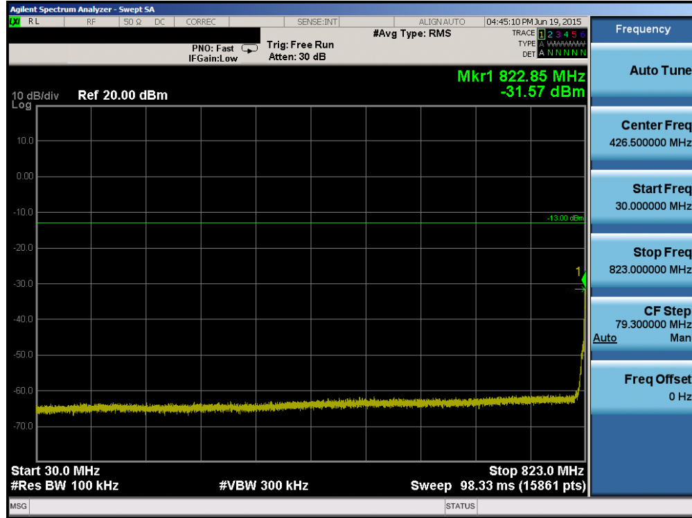
Plot 6-45. Conducted Spurious Plot (Cellular WCDMA Mode – Ch. 4132)
