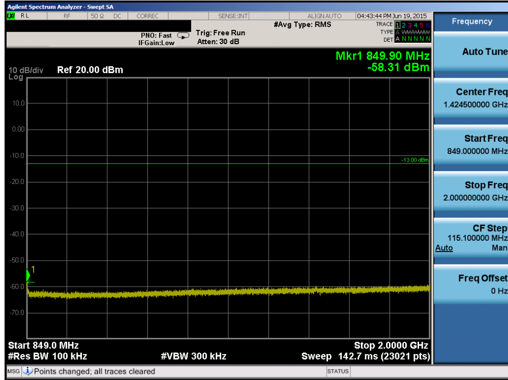
Plot 6-49. Conducted Spurious Plot (Cellular WCDMA Mode – Ch. 4183)
