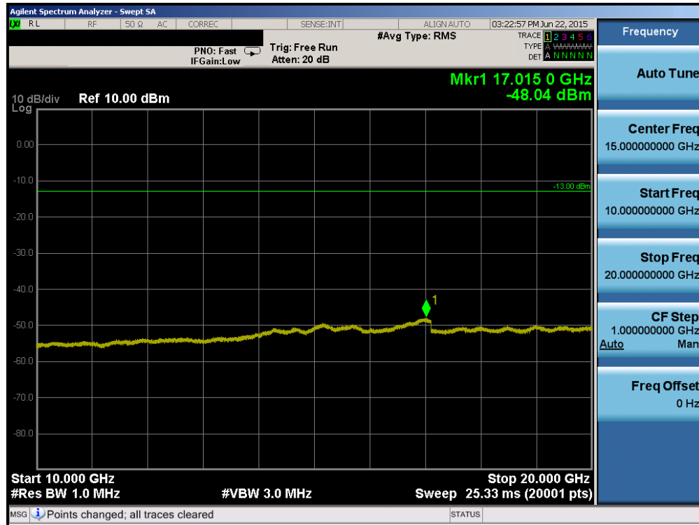
Plot 6-41. Conducted Spurious Plot (PCS CDMA Mode – Ch. 600)
