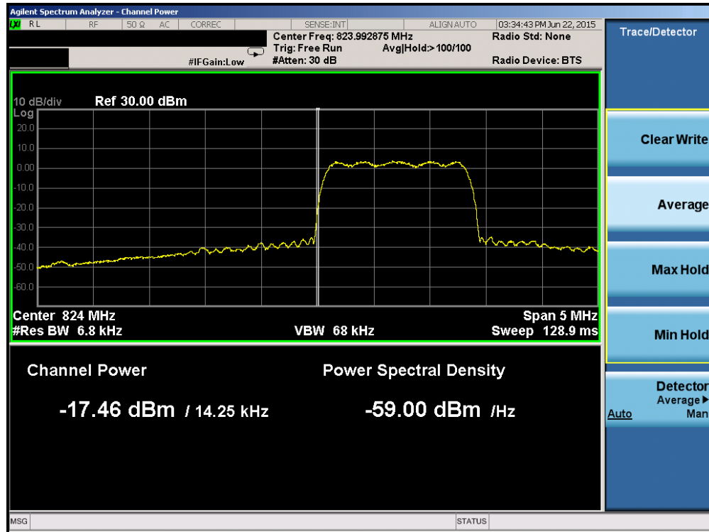
Plot 6-69. Band Edge Plot (Cellular CDMA Mode – Ch. 1013)
