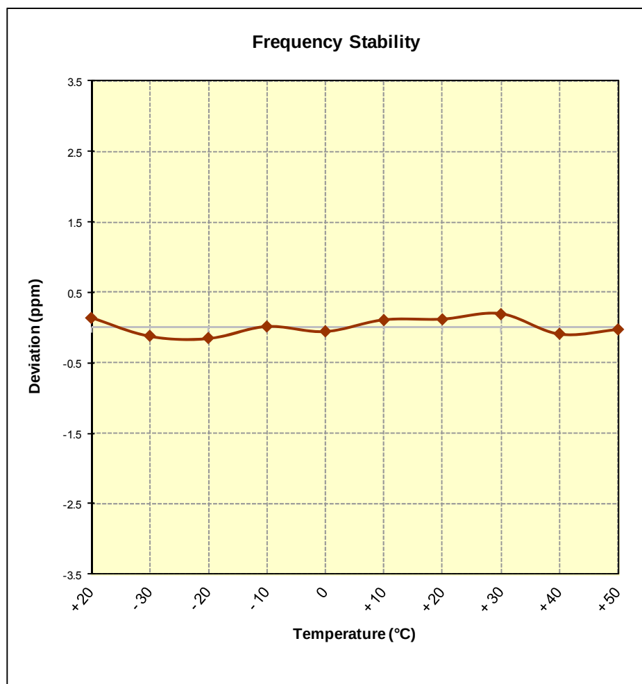
Figure 6-10. Frequency Stability Graph (PCS GSM Mode – Ch. 661)
