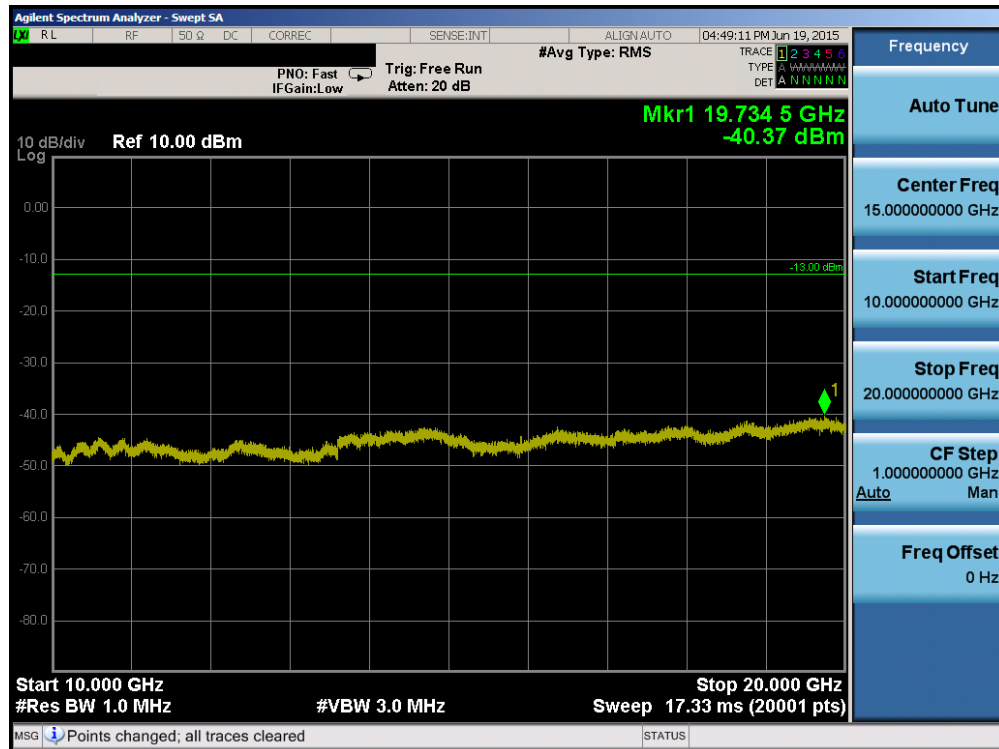
Plot 6-56. Conducted Spurious Plot (PCS WCDMA Mode – Ch. 9262)
