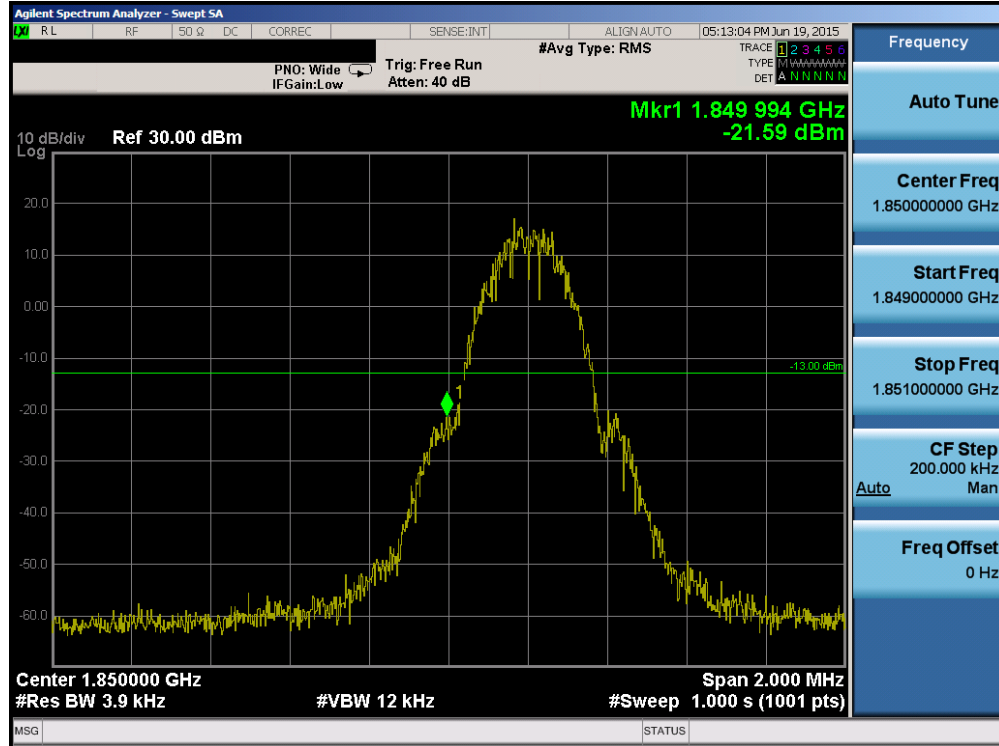
Plot 6-65. Band Edge Plot (PCS GSM Mode – Ch. 512)
