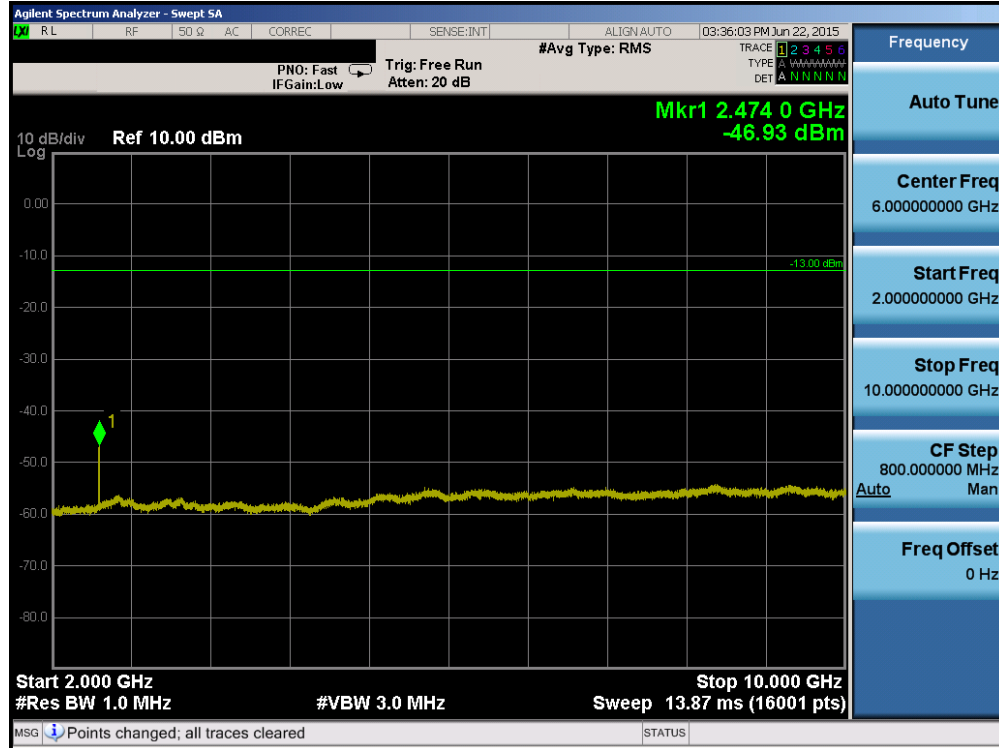
Plot 6-29. Conducted Spurious Plot (Cellular CDMA Mode – Ch. 1013)
