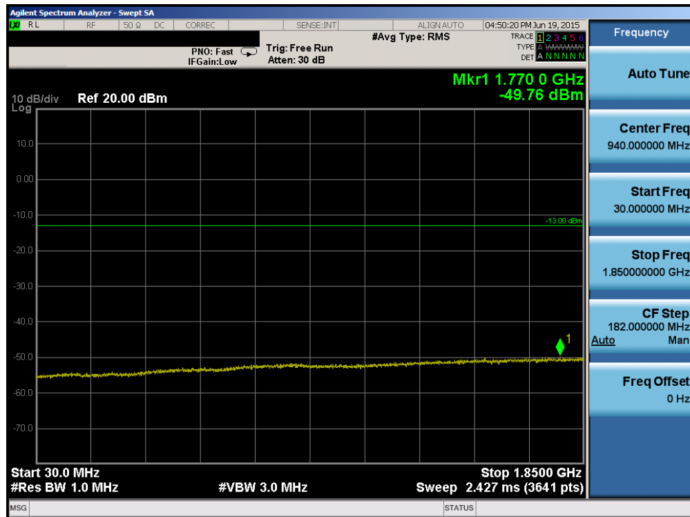
Plot 6-60. Conducted Spurious Plot (PCS WCDMA Mode – Ch. 9538)
