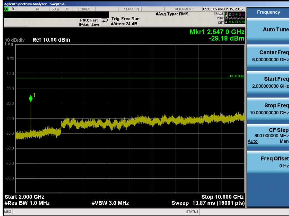
Plot 6-17. Conducted Spurious Plot (Cellular GSM Mode – Ch. 251)
