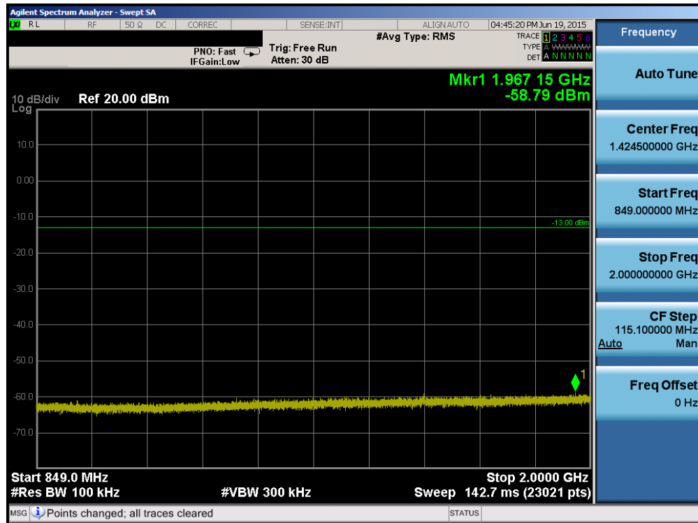
Plot 6-46. Conducted Spurious Plot (Cellular WCDMA Mode – Ch. 4132)
