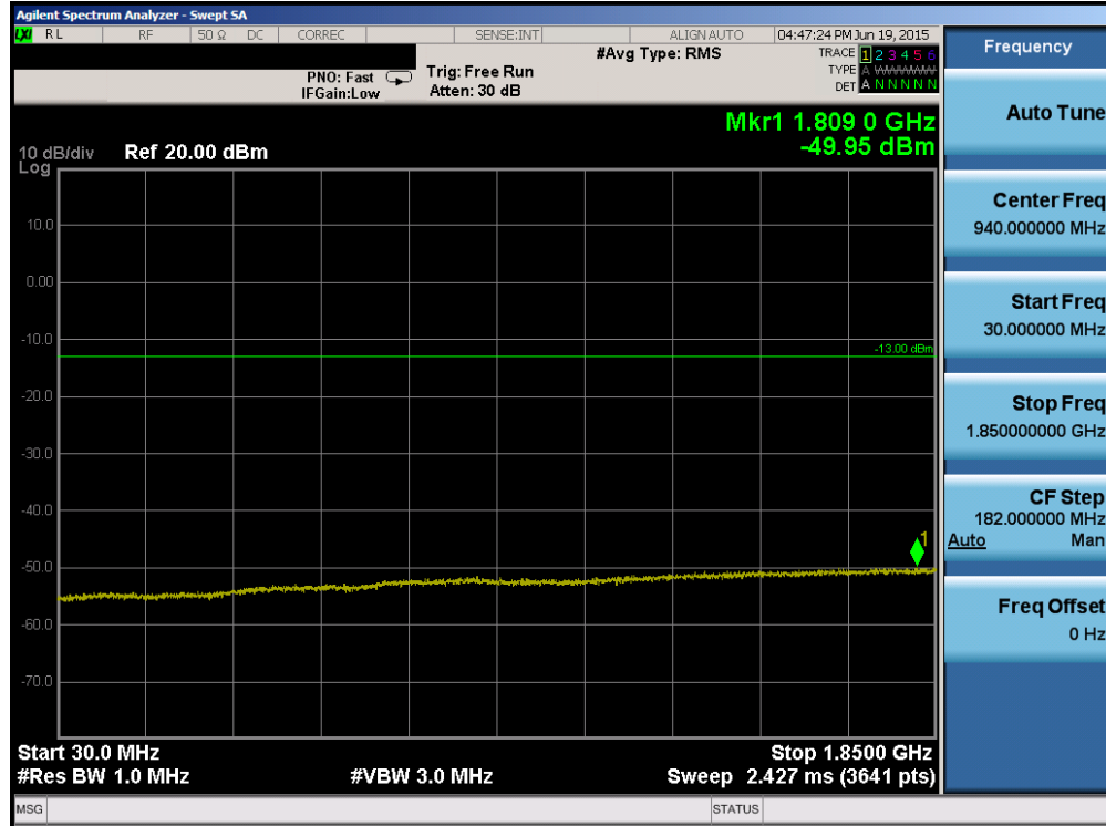
Plot 6-57. Conducted Spurious Plot (PCS WCDMA Mode – Ch. 9400)
