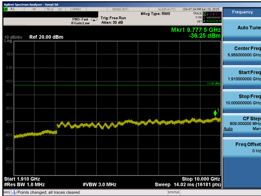
Plot 6-58. Conducted Spurious Plot (PCS WCDMA Mode – Ch. 9400)
