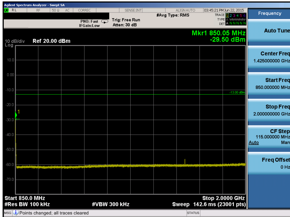
Plot 6-34. Conducted Spurious Plot (Cellular CDMA Mode – Ch. 777)
