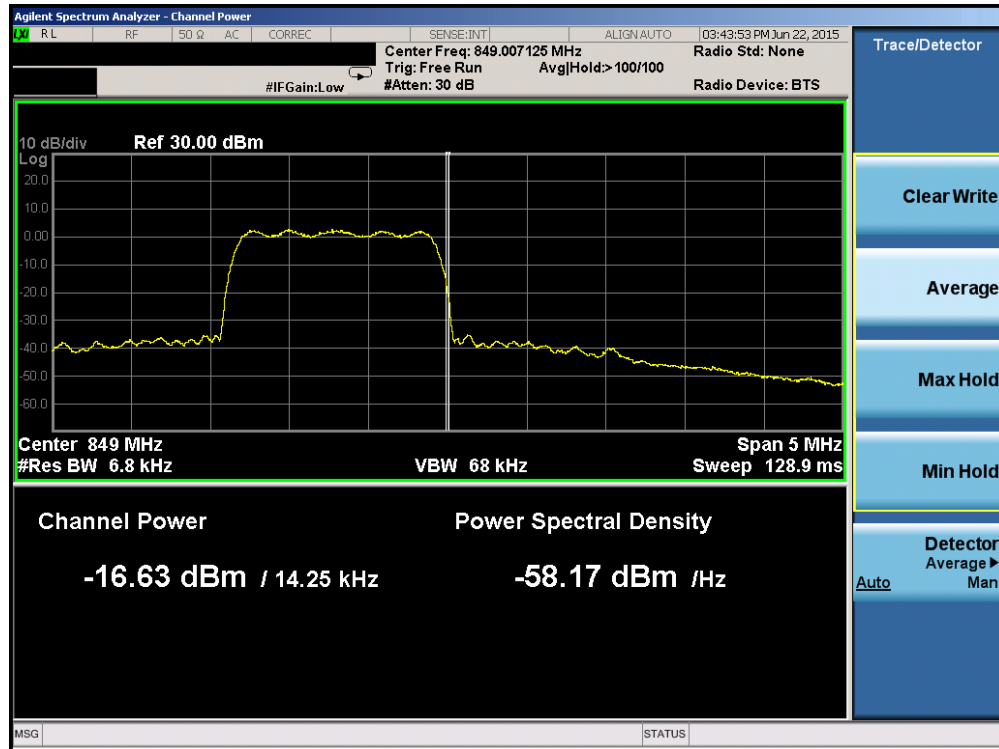
Plot 6-71. Band Edge Plot (Cellular CDMA Mode – Ch. 777)
