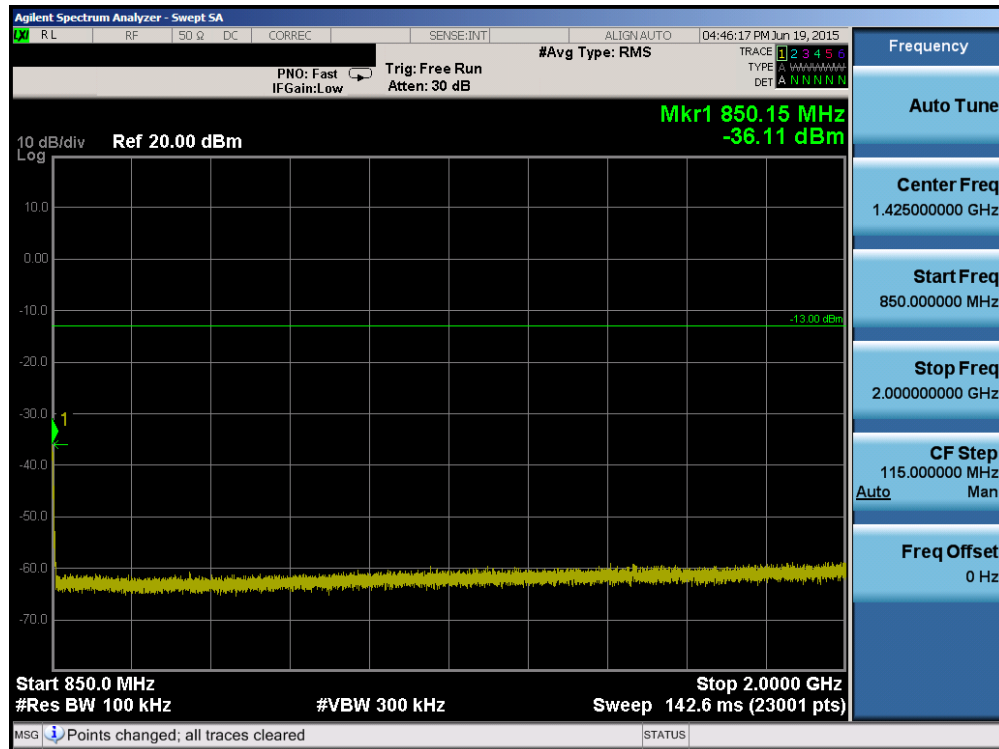
Plot 6-52. Conducted Spurious Plot (Cellular WCDMA Mode – Ch. 4233)
