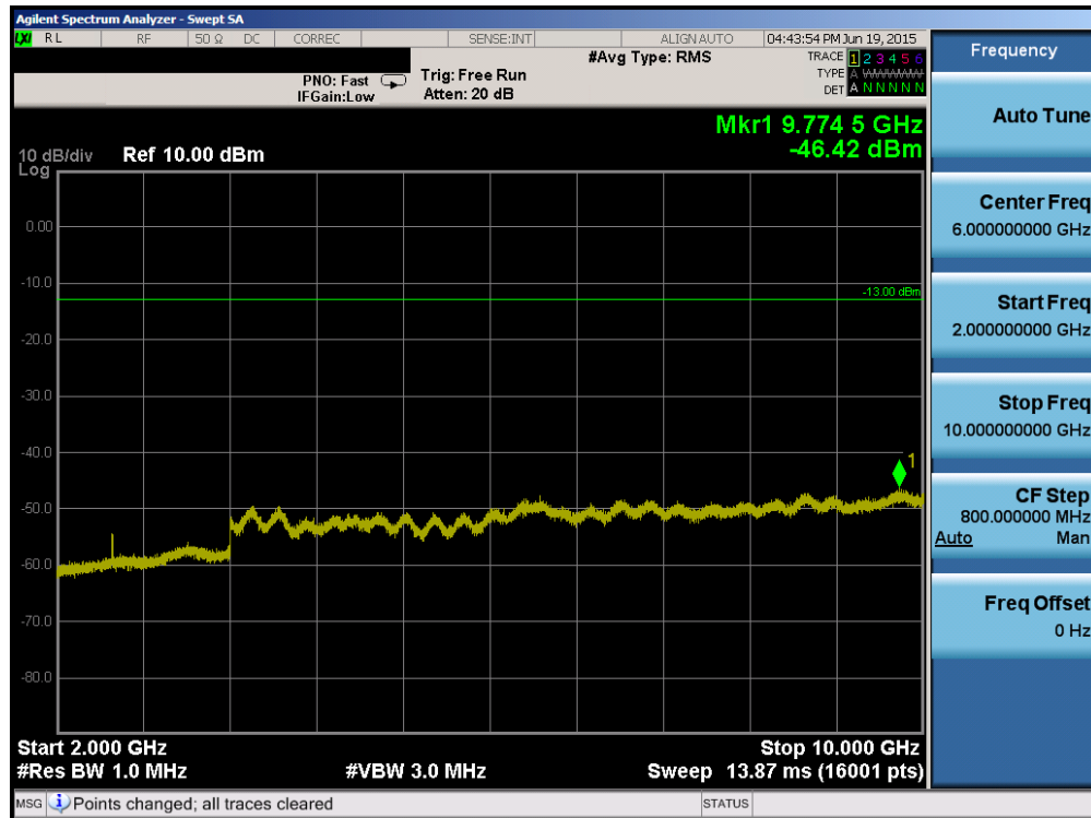
Plot 6-50. Conducted Spurious Plot (Cellular WCDMA Mode – Ch. 4183)
