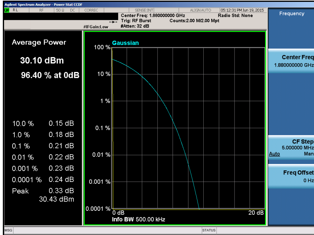
Plot 6-83. Peak-Average Ratio Plot (PCS GSM Mode – Ch. 661)
