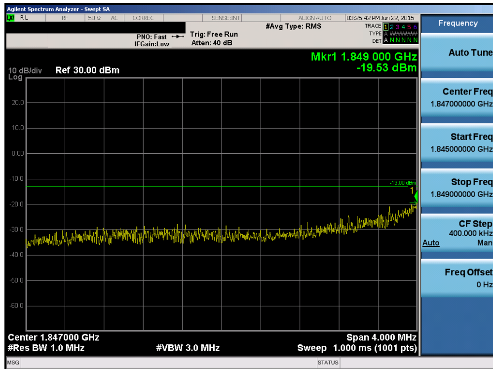
Plot 6-74. 4MHz Span Plot (PCS CDMA Mode – Ch. 25)
