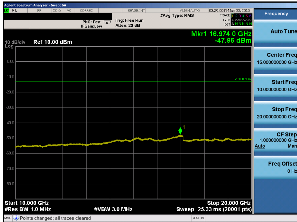
Plot 6-44. Conducted Spurious Plot (PCS CDMA Mode – Ch. 1175)
