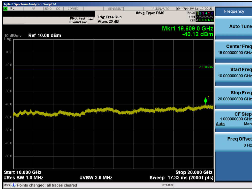
Plot 6-59. Conducted Spurious Plot (PCS WCDMA Mode – Ch. 9400)
