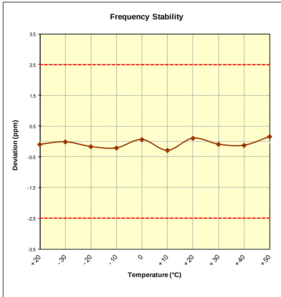
Figure 6-9. Frequency Stability Graph (Cellular WCDMA Mode – Ch. 4183)
