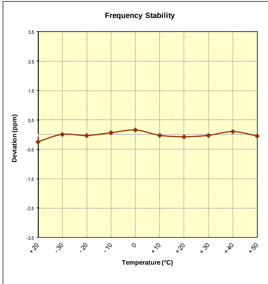
Figure 6-12. Frequency Stability Graph (PCS WCDMA Mode – Ch. 9400)
