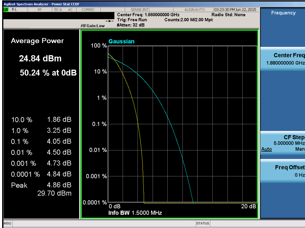
Plot 6-85. Peak-Average Ratio Plot (PCS CDMA Mode – Ch. 600)
