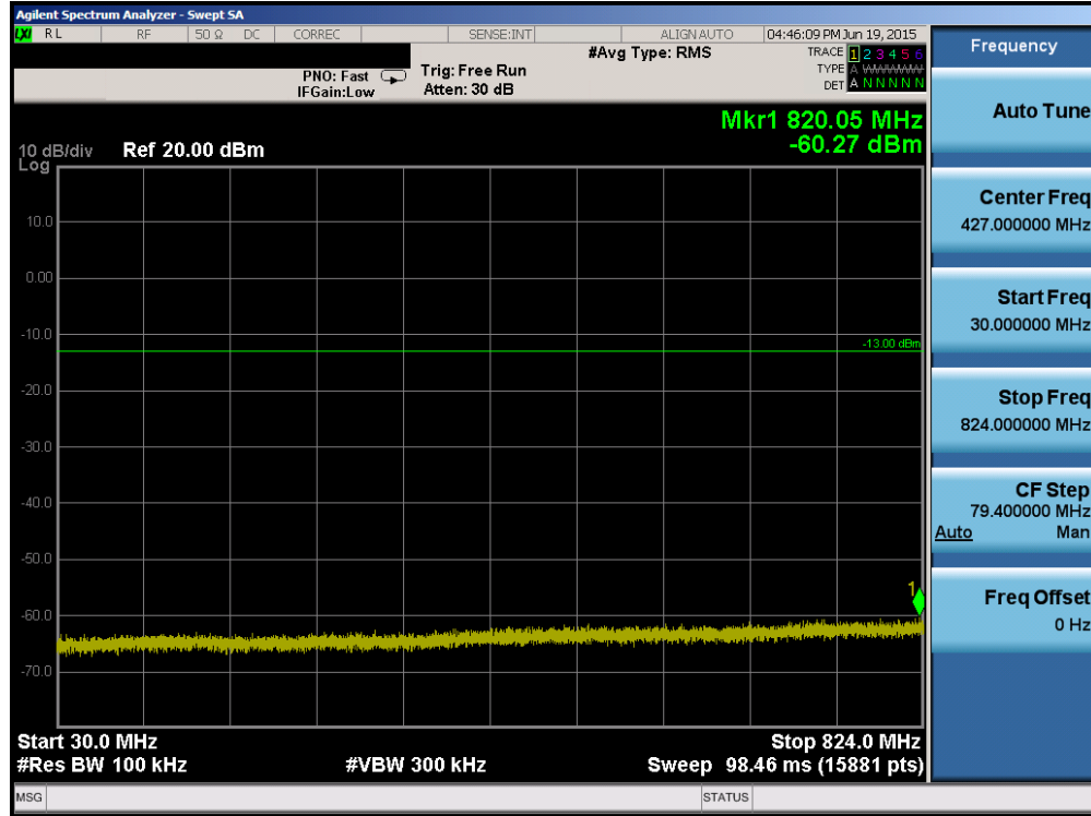
Plot 6-51. Conducted Spurious Plot (Cellular WCDMA Mode – Ch. 4233)
