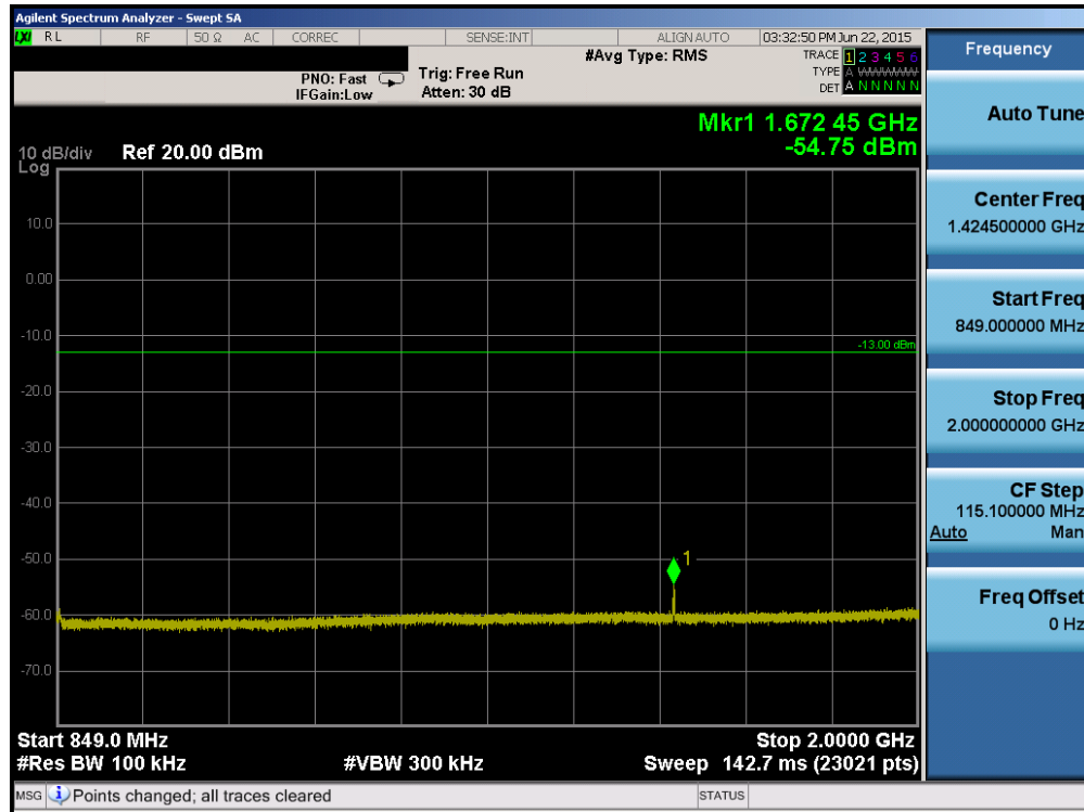
Plot 6-31. Conducted Spurious Plot (Cellular CDMA Mode – Ch. 384)
