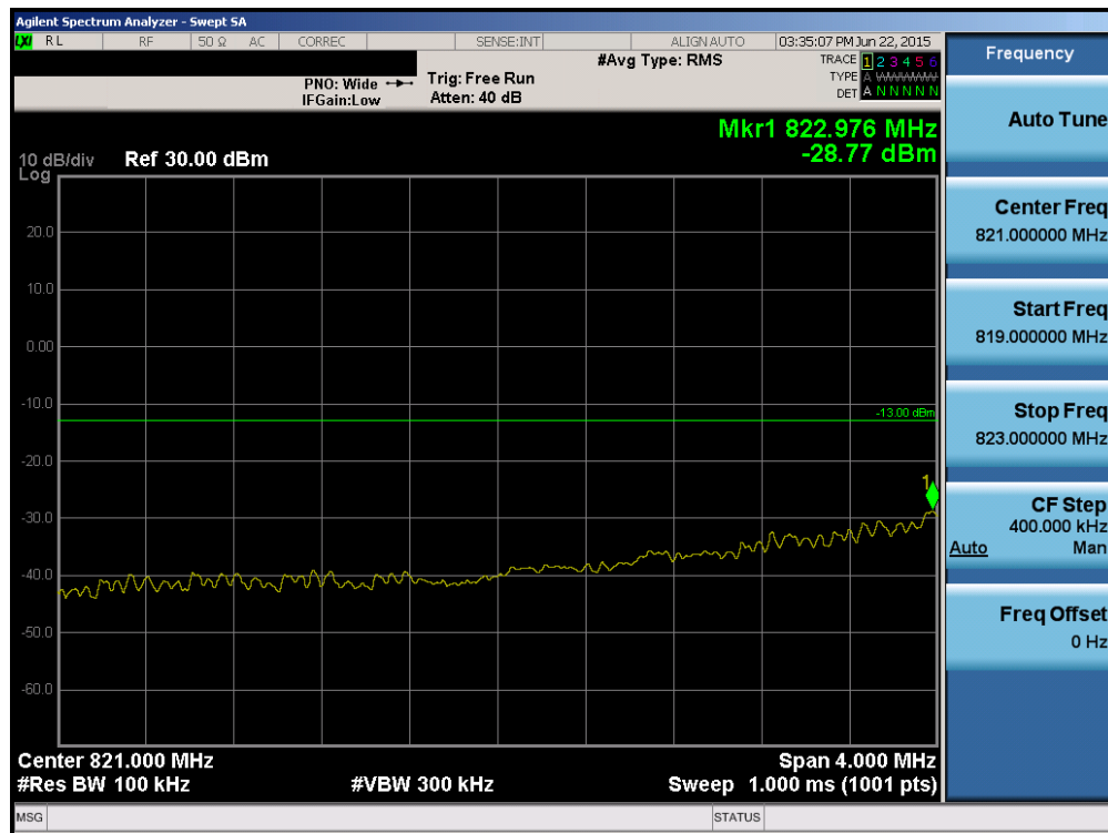
Plot 6-70. 4MHz Span Plot (Cellular CDMA Mode – Ch. 1013)
