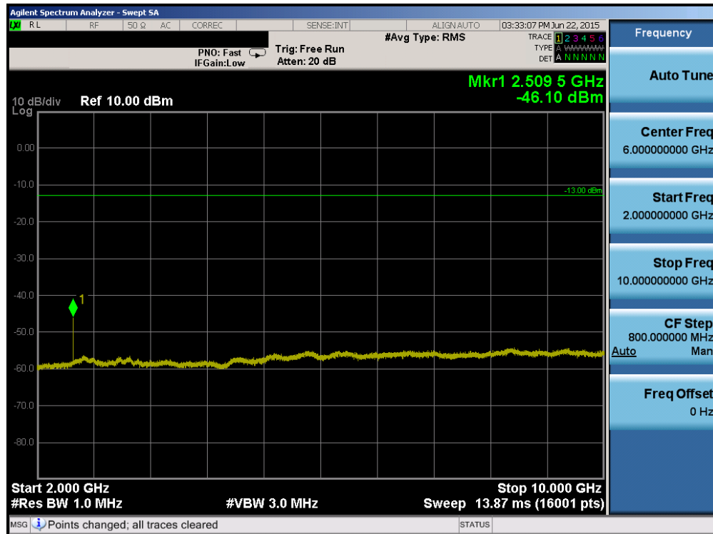
Plot 6-32. Conducted Spurious Plot (Cellular CDMA Mode – Ch. 384)
