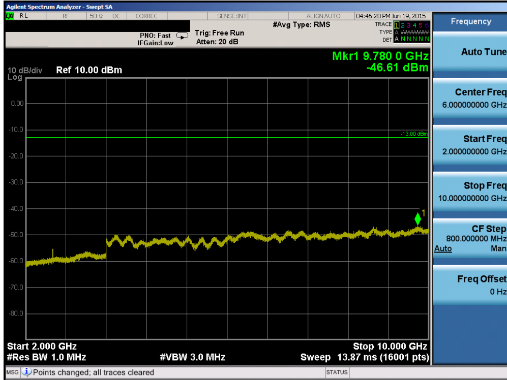
Plot 6-53. Conducted Spurious Plot (Cellular WCDMA Mode – Ch. 4233)
