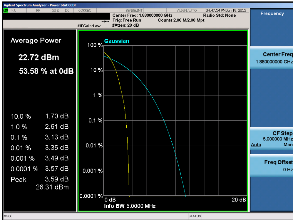
Plot 6-86. Peak-Average Ratio Plot (PCS WCDMA Mode – Ch. 9400)
