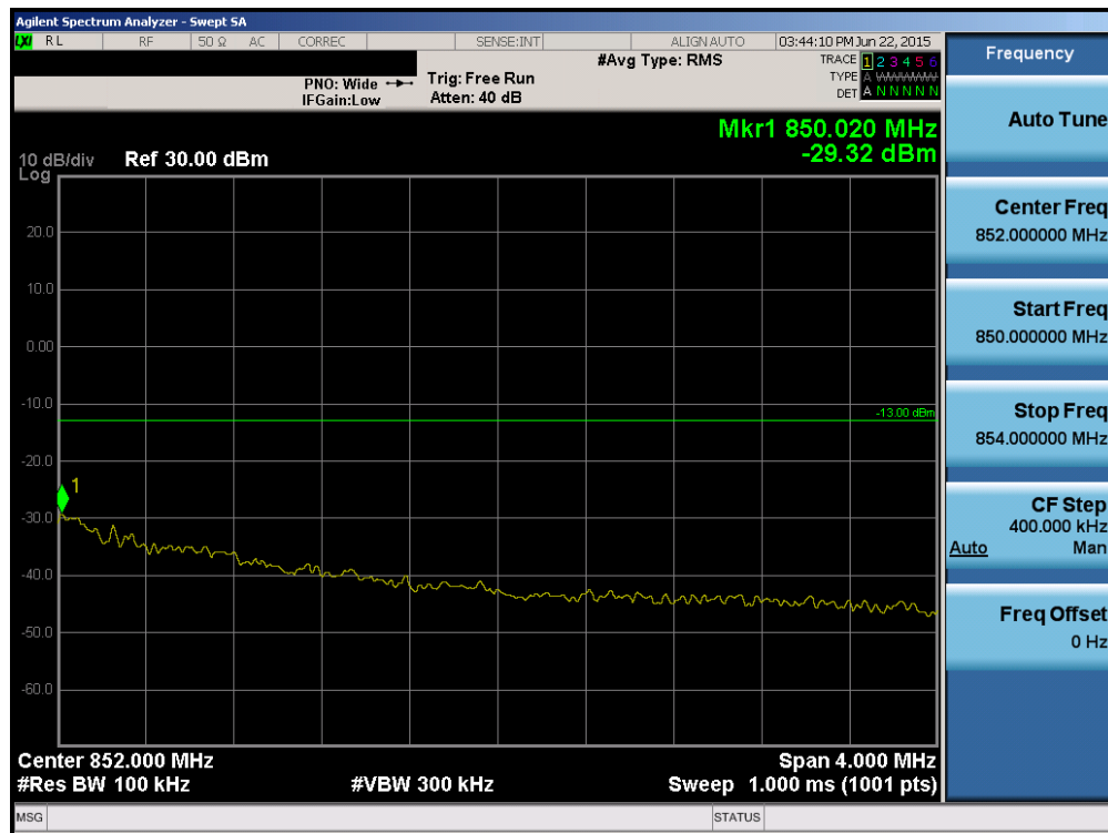
Plot 6-72. 4MHz Span Plot (Cellular CDMA Mode – Ch. 777)
