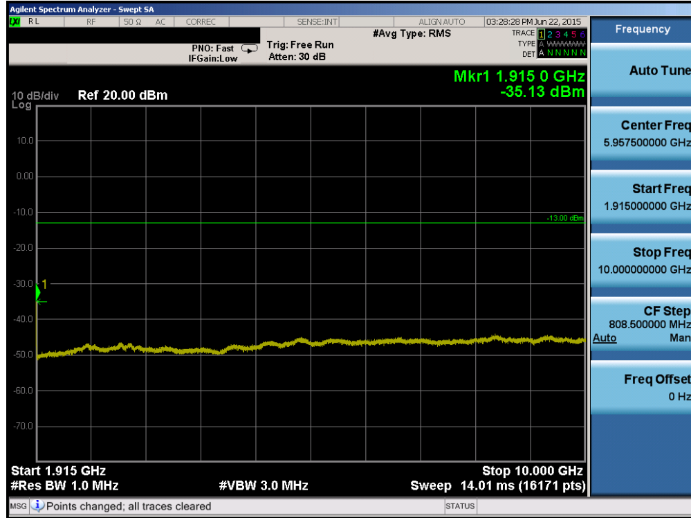
Plot 6-43. Conducted Spurious Plot (PCS CDMA Mode – Ch. 1175)
