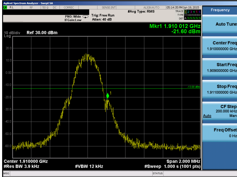
Plot 6-67. Band Edge Plot (PCS GSM Mode – Ch. 810)
