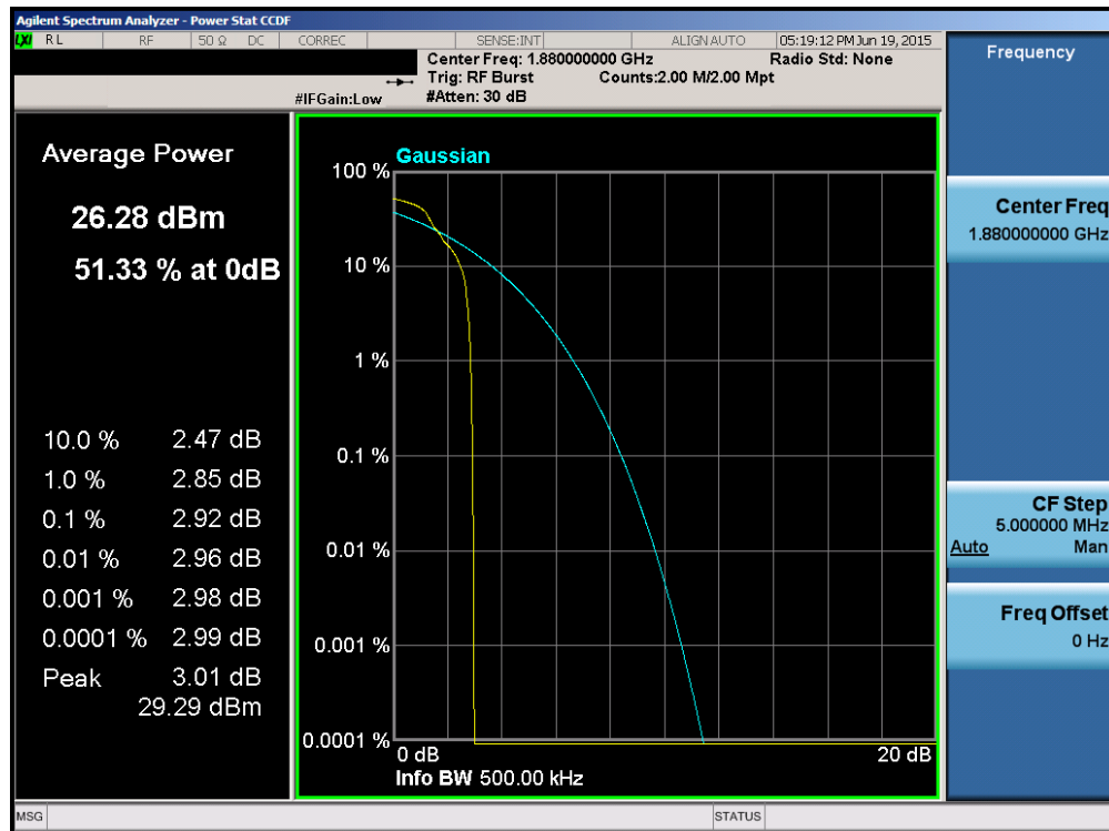
Plot 6-84. Peak-Average Ratio Plot (EDGE1900 Mode – Ch. 661)
