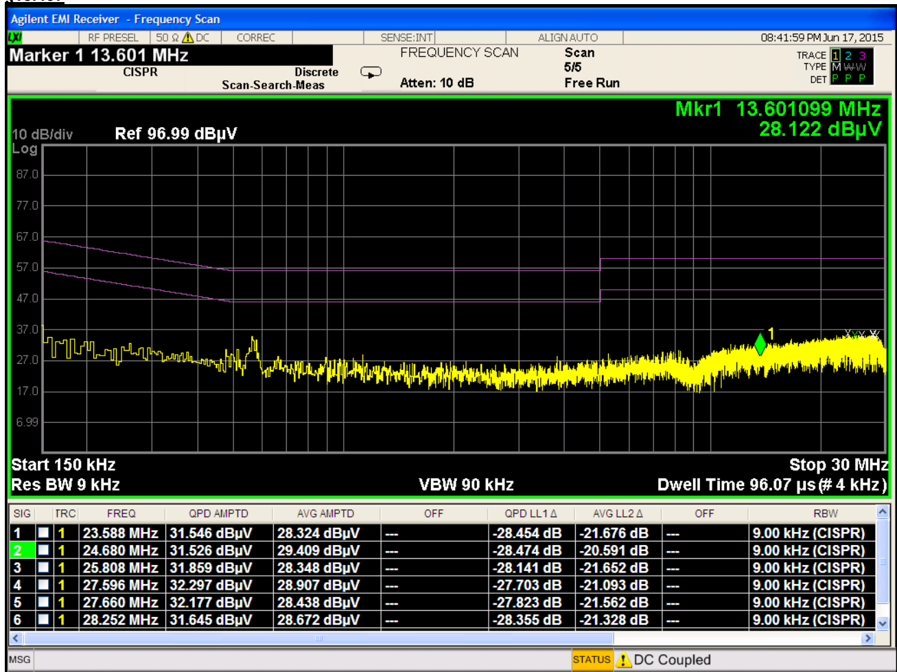
Plot 6-252. Line Conducted Plot with 802.11a UNII Band 3 (N)
