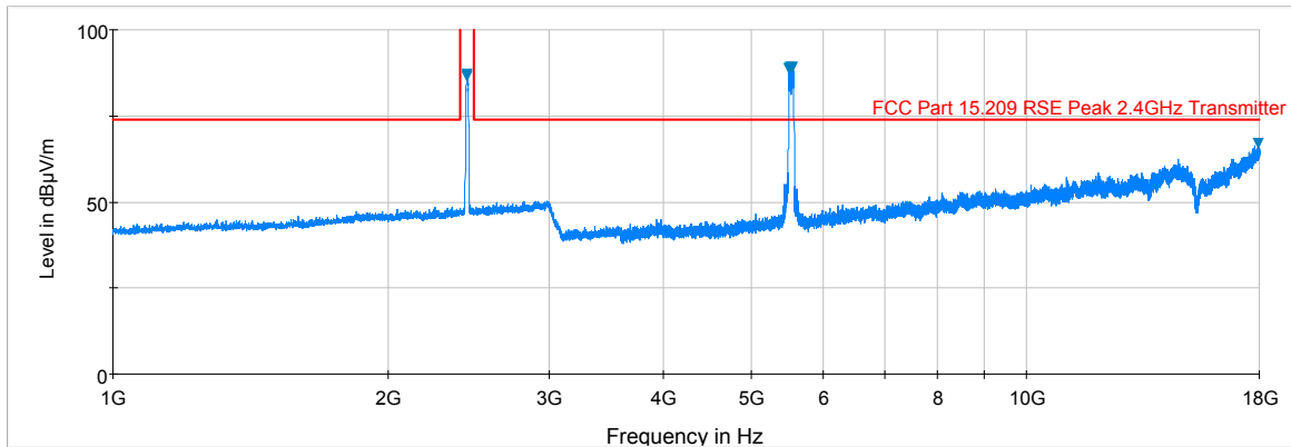
Plot 6-174. Radiated Spurious Plot above 1GHz (SIMULTANEOUS TX 2.4GHz – 5 GHz, Ant. Pol. V)
