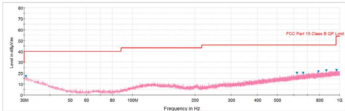
Plot 6-242. Radiated Spurious Plot below 1GHz (802.11a – U3 Ch. 157, Ant. Pol. V)
