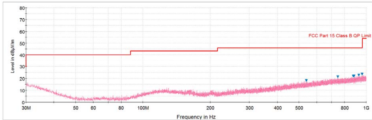
Plot 6-241. Radiated Spurious Plot below 1GHz (802.11a – U3 Ch. 157, Ant. Pol. H)
