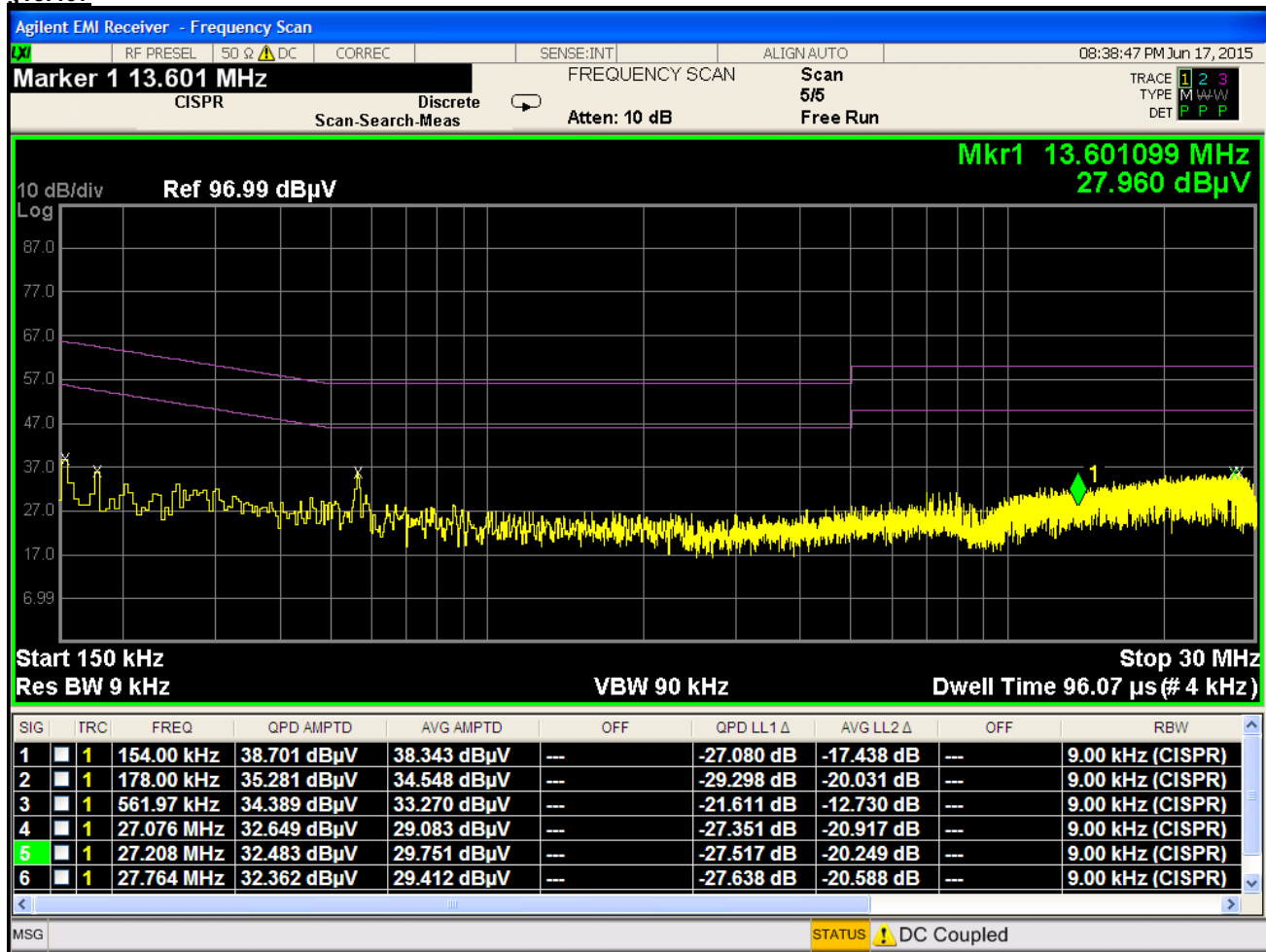
Plot 6-250. Line Conducted Plot with 802.11a UNII Band 2C (N)
