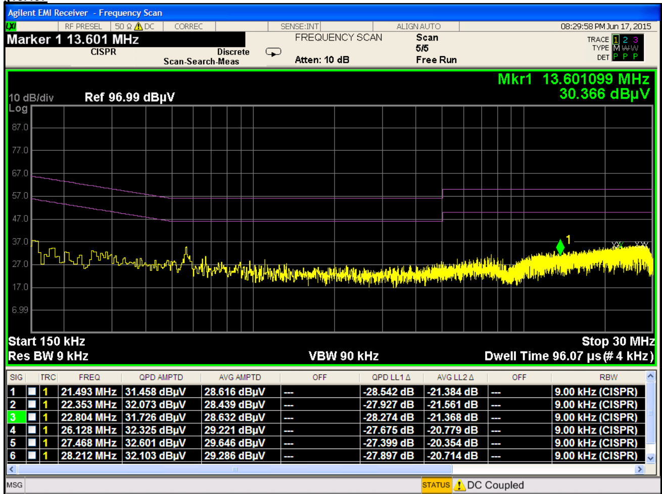
Plot 6-248. Line Conducted Plot with 802.11a UNII Band 2A (N)
