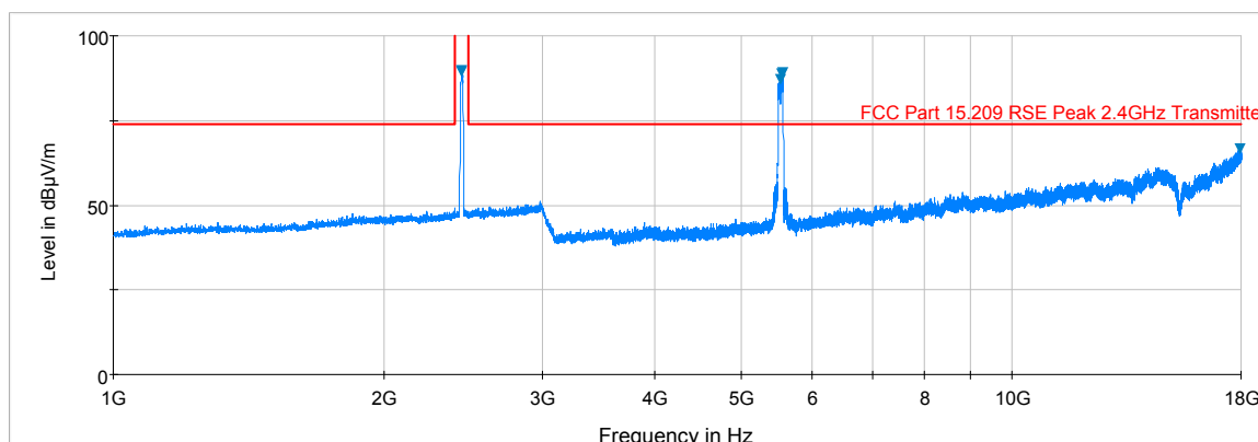
Plot 6-173. Radiated Spurious Plot above 1GHz (SIMULTANEOUS TX 2.4GHz – 5 GHz, Ant. Pol. H)
