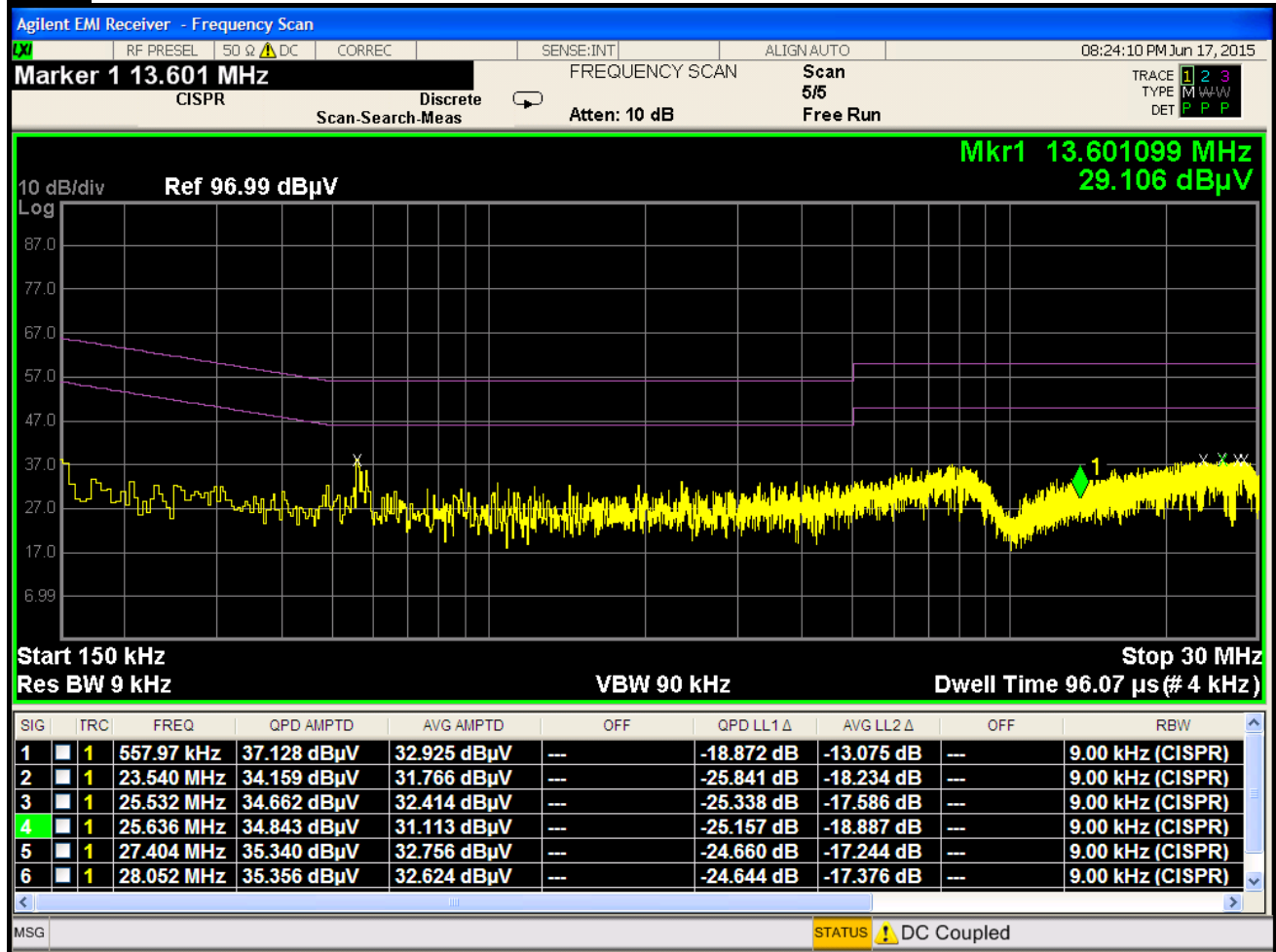
Plot 6-245. Line Conducted Plot with 802.11a UNII Band 1 (L1)
