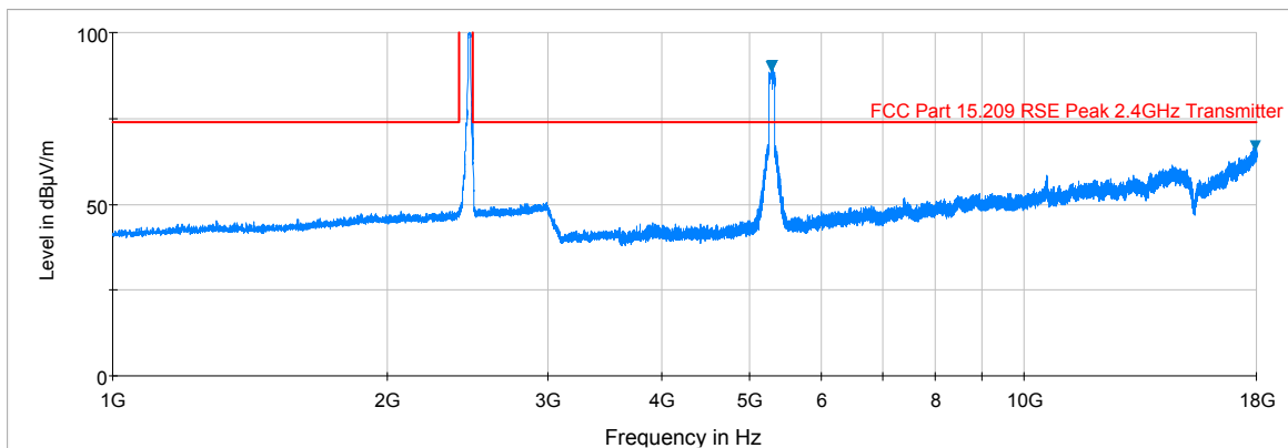
Plot 6-176. Radiated Spurious Plot above 1GHz (SIMULTANEOUS TX 5 GHz – 2.4 GHz, Ant. Pol. V)
