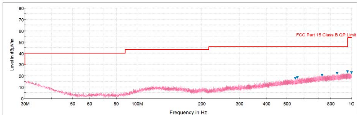
Plot 6-244. Radiated Spurious Plot below 1GHz (802.11a – U3 Ch. 157, Ant. Pol. V)
