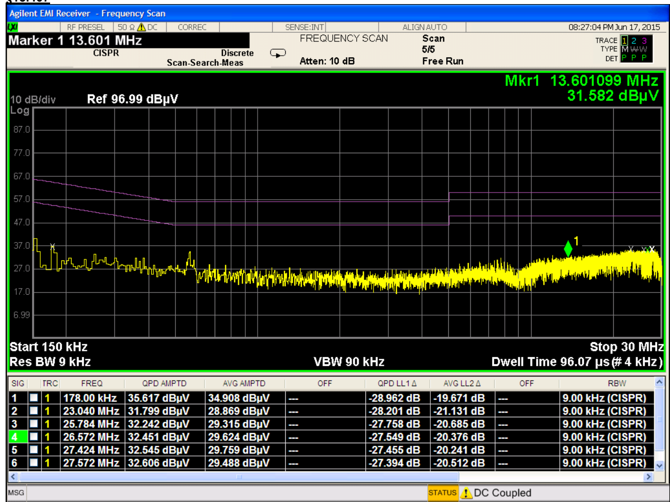
Plot 6-246. Line Conducted Plot with 802.11a UNII Band 1 (N)
