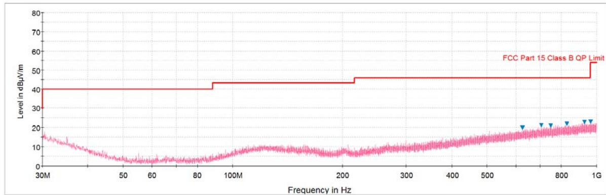
Plot 6-243. Radiated Spurious Plot below 1GHz (802.11a – U3 Ch. 157, Ant. Pol. H)
