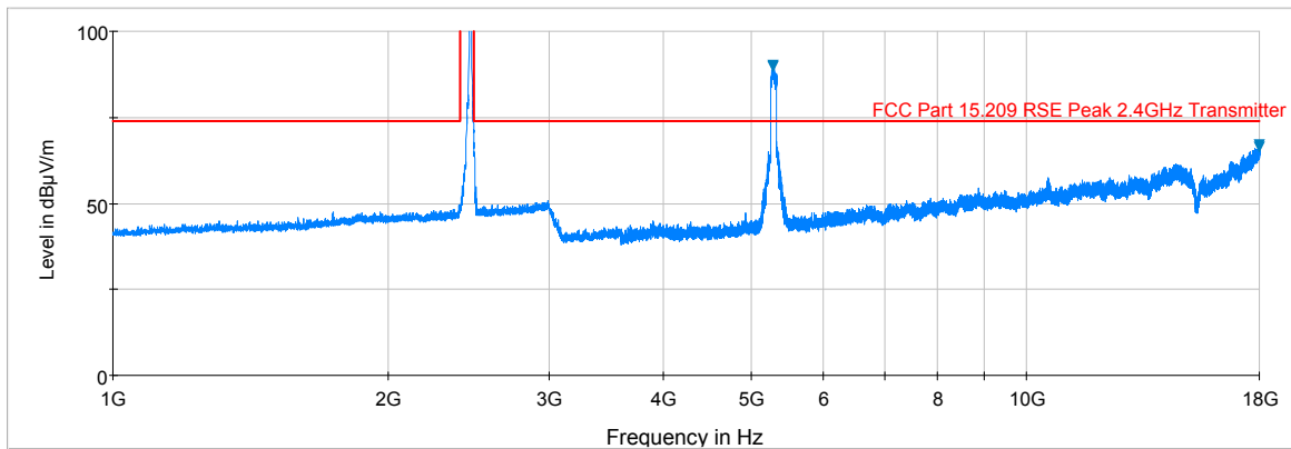
Plot 6-175. Radiated Spurious Plot above 1GHz (SIMULTANEOUS TX 5 GHz – 2.4 GHz, Ant. Pol. H)
