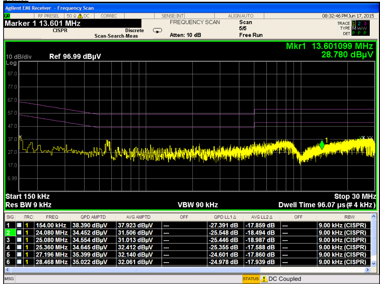
Plot 6-247. Line Conducted Plot with 802.11a UNII Band 2A (L1)
