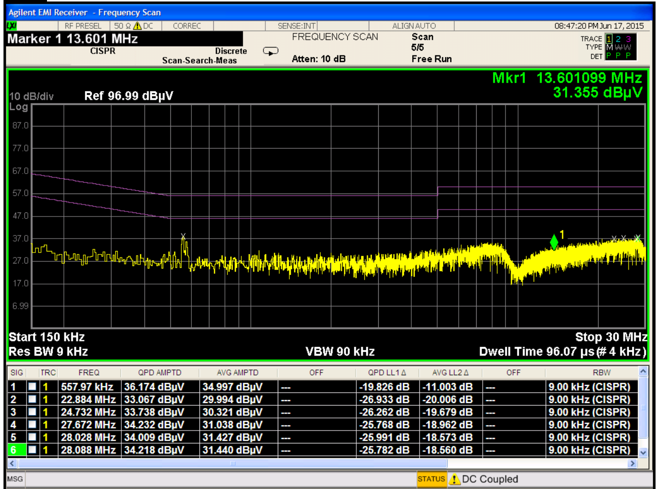
Plot 6-251. Line Conducted Plot with 802.11a UNII Band 3 (L1)
