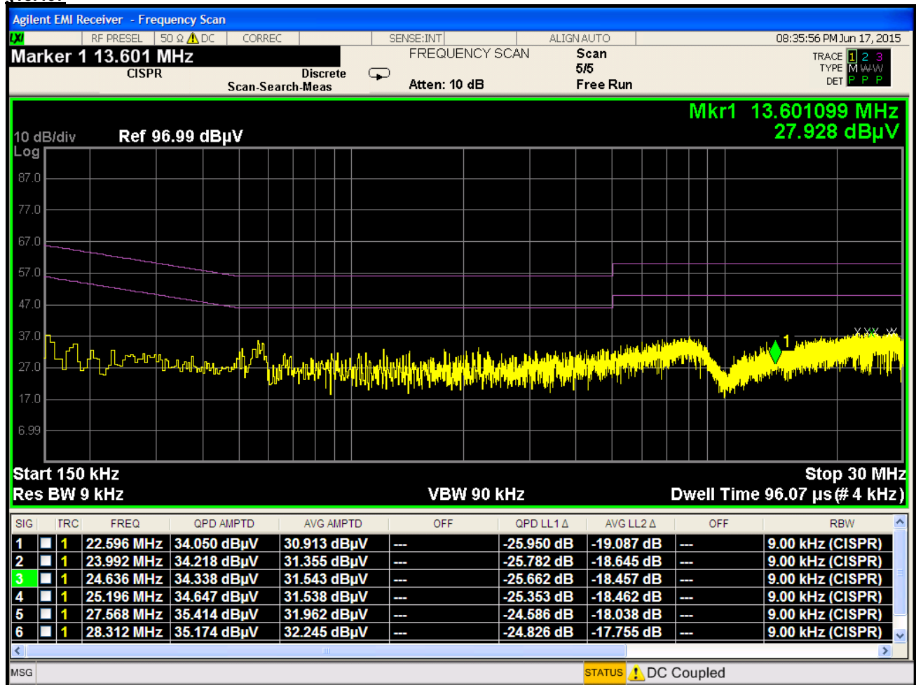
Plot 6-249. Line Conducted Plot with 802.11a UNII Band 2C (L1)
