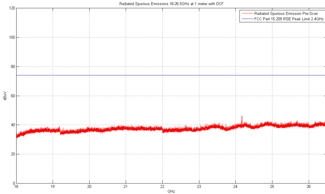
Plot 6-75. Radiated Spurious Plot above 18GHz (Pol. H)
