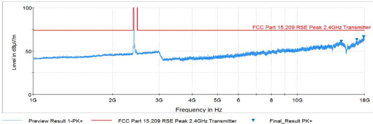
Plot 6-69. Radiated Spurious Plot above 1GHz (802.11b – Ch. 1, Ant. Pol. H)
