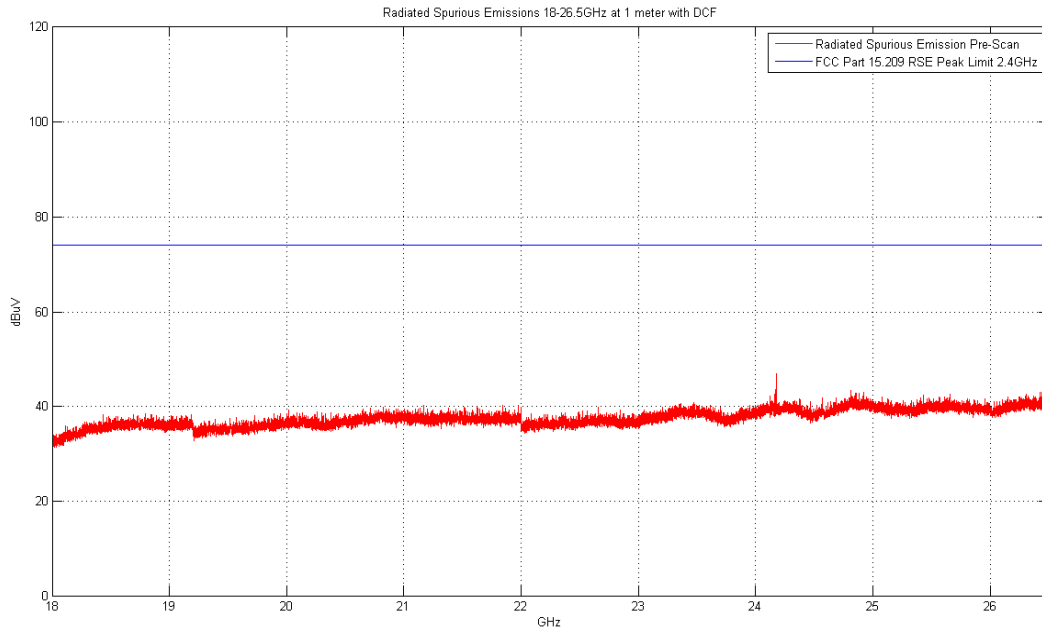
Plot 6-67. Radiated Spurious Plot above 18GHz (Pol. H)
