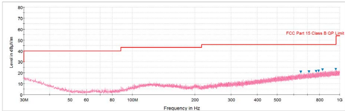
Plot 6-89. Radiated Spurious Plot below 1GHz (Pol. H)
