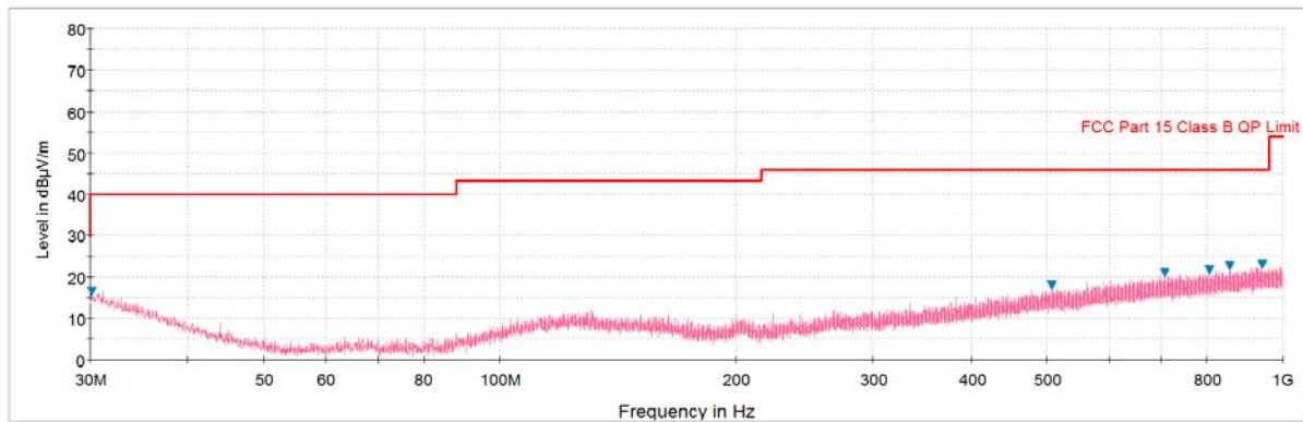
Plot 6-92. Radiated Spurious Plot below 1GHz (Pol. V)
