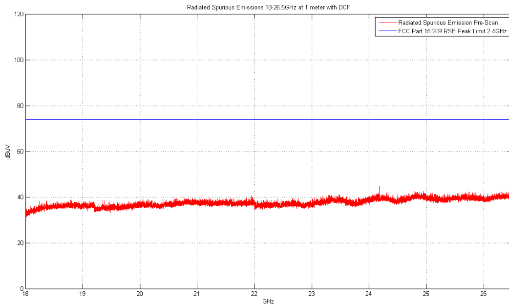
Plot 6-68. Radiated Spurious Plot above 18GHz (Pol. V)
