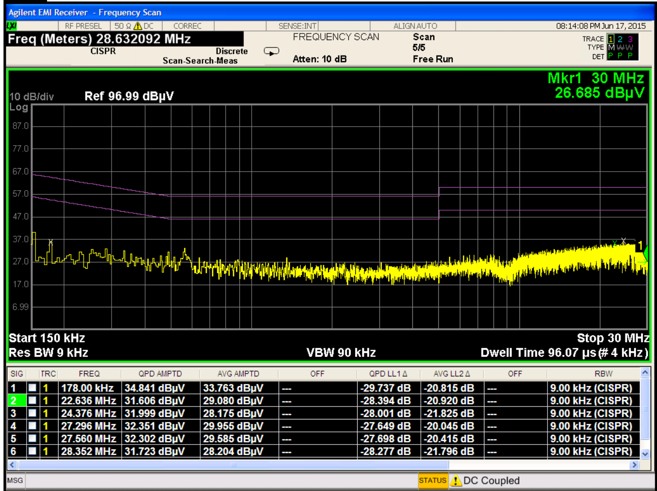
Plot 6-94. Line Conducted Plot with 802.11b (N)
