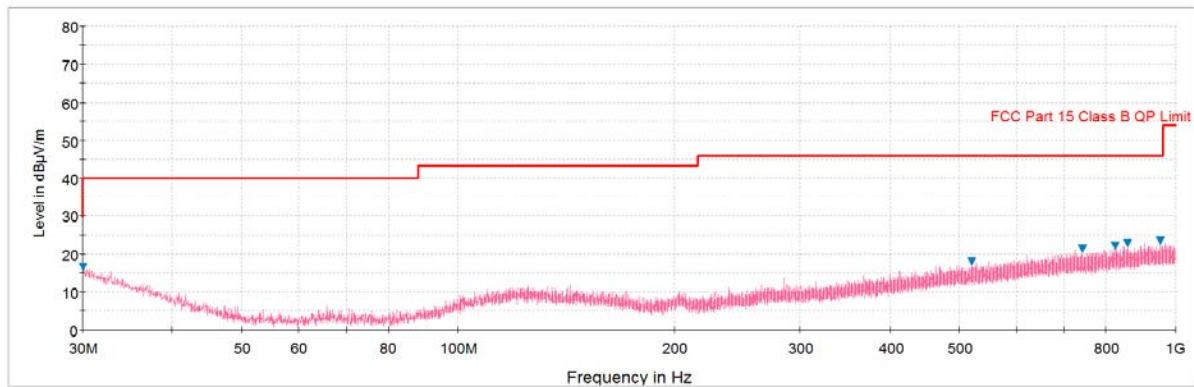
Plot 6-90. Radiated Spurious Plot below 1GHz (Pol. V)
