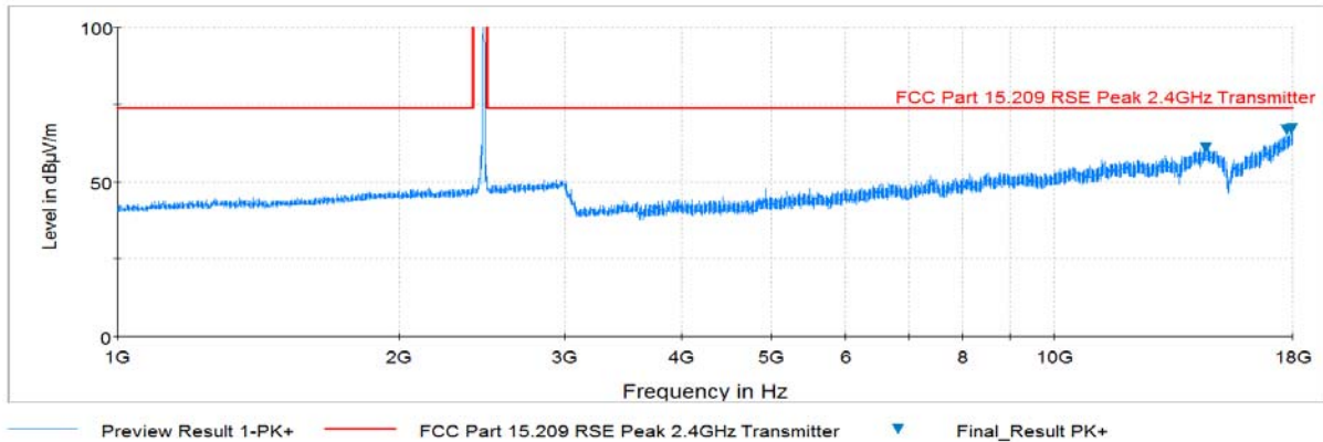
Plot 6-74. Radiated Spurious Plot above 1GHz (802.11b – Ch. 11, Ant. Pol. V)
