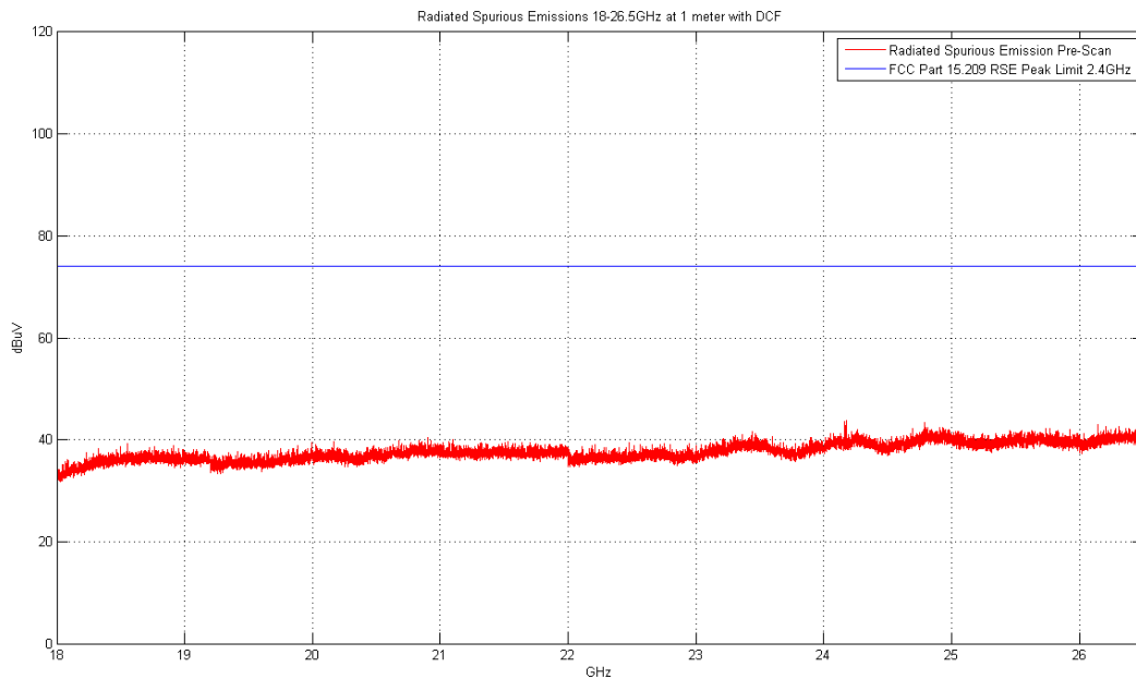
Plot 6-76. Radiated Spurious Plot above 18GHz (Pol. V)
