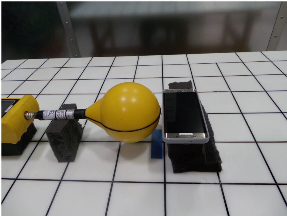
Figure 10. H-Field Measurement (Position D)
