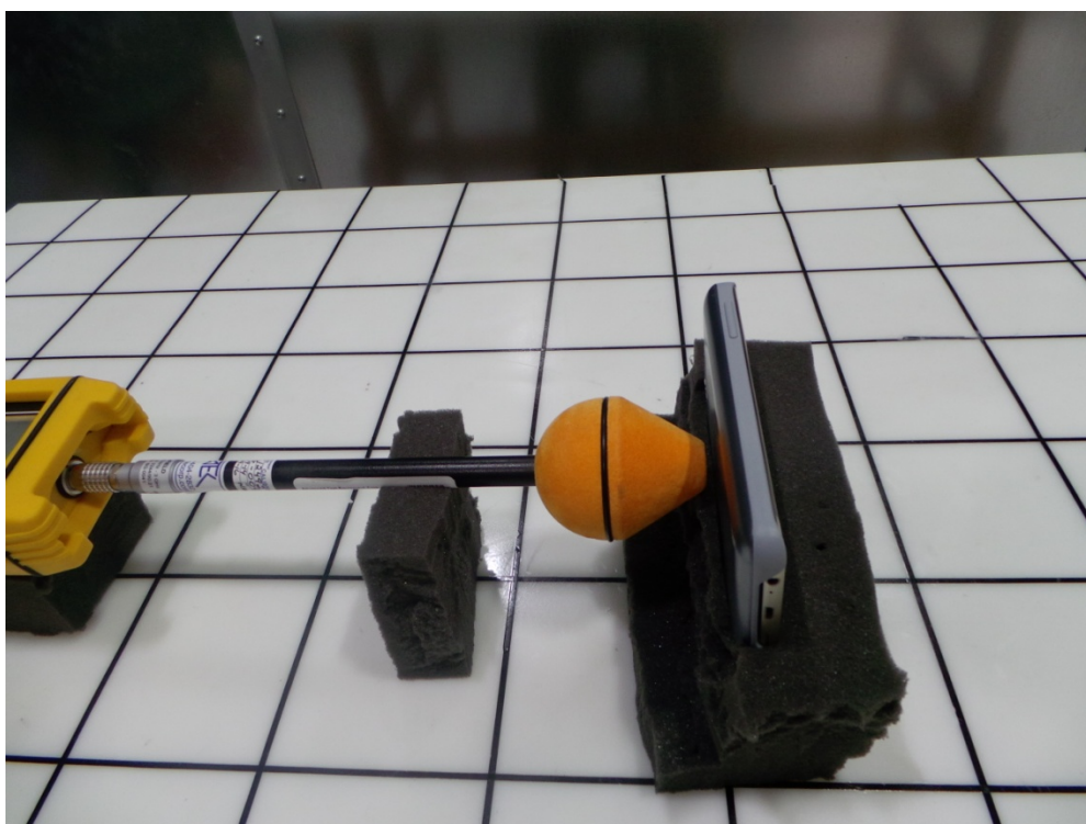
Figure 6. E-Field Measurement (Position F)
