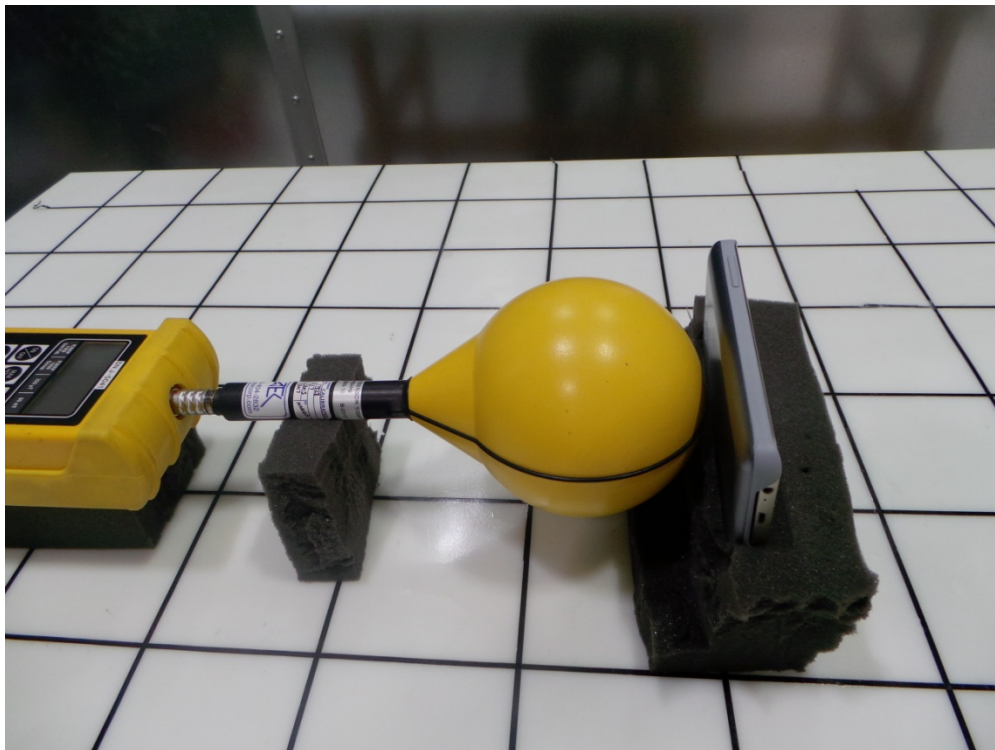
Figure 12. H-Field Measurement (Position F)
