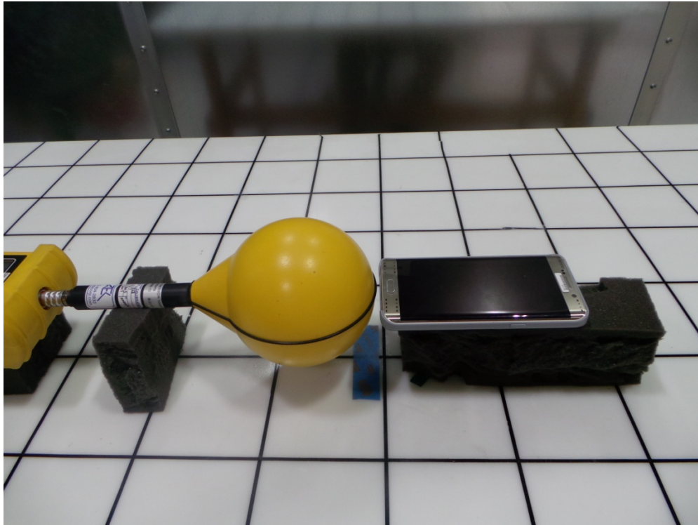
Figure 9. H-Field Measurement (Position C)
