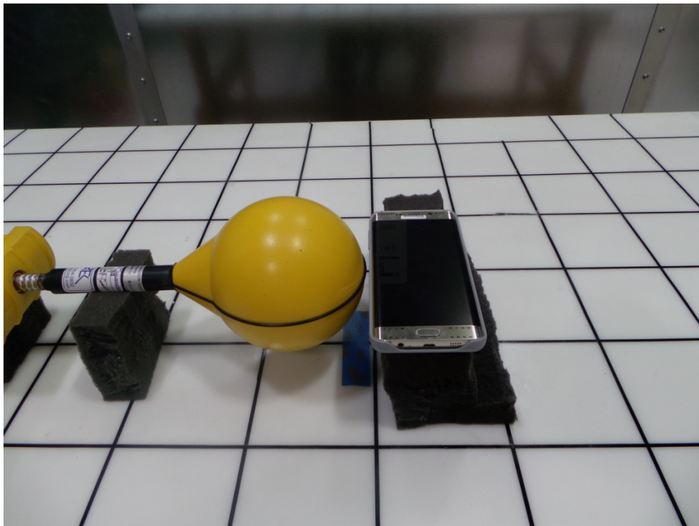
Figure 8. H-Field Measurement (Position B)
