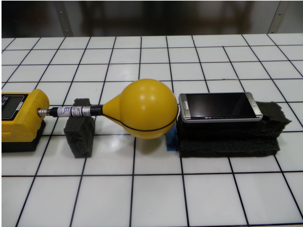
Figure 7. H-Field Measurement (Position A)
