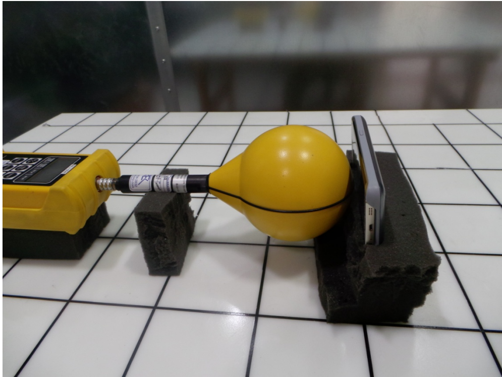
Figure 11. H-Field Measurement (Position E)
