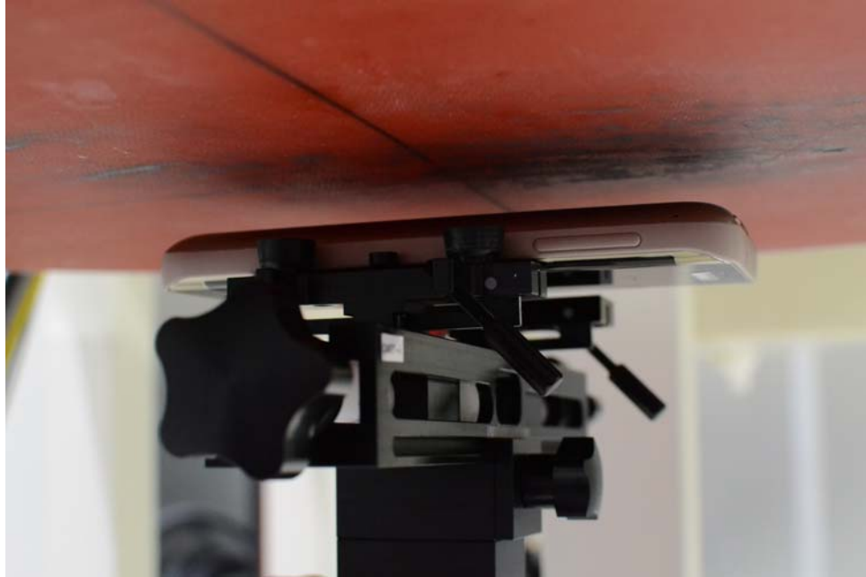
SAR Test Setup Photo 3: Back Side at 1.5 cm with Wireless Charging Cover
