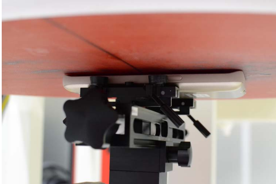
SAR Test Setup Photo 9: Front Side at 0.0 cm with Wireless Charging Cover
