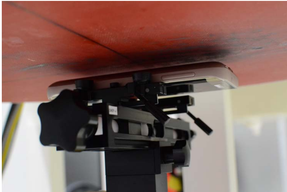
SAR Test Setup Photo 4: Back Side at 1.0 cm with Wireless Charging Cover
