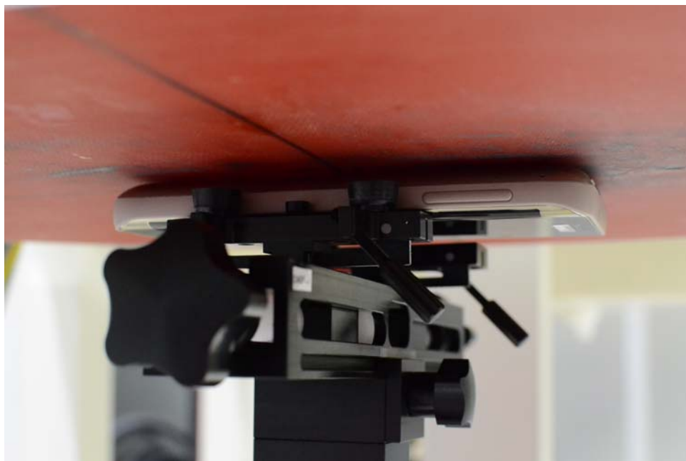
SAR Test Setup Photo 6: Back Side at 0.0 cm with Wireless Charging Cover
