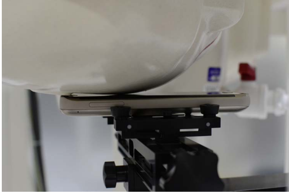
SAR Test Setup Photo 1: Right Cheek with Wireless Charging Cover
