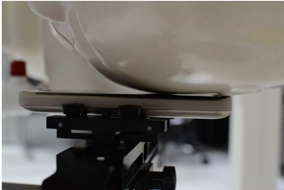
SAR Test Setup Photo 2: Left Cheek with Wireless Charging Cover
