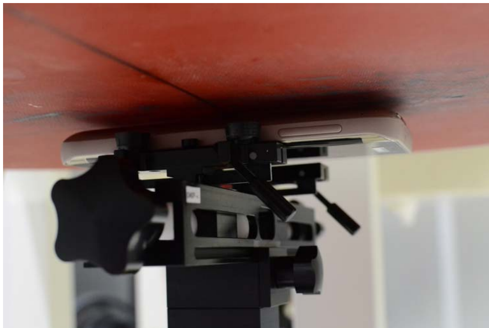
SAR Test Setup Photo 5: Back Side at 0.2 cm with Wireless Charging Cover
