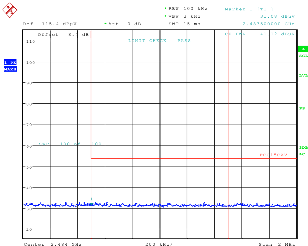
Plot 6-18. Radiated Restricted Upper Band Edge Measurement (Average)
