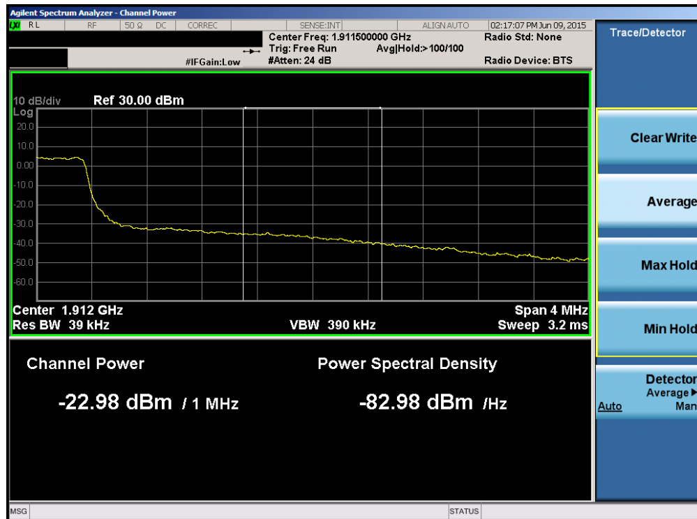
Plot 6-138. Upper Extended Band Edge Plot (Band2/25 – 3.0MHz QPSK – RB Size 15)
