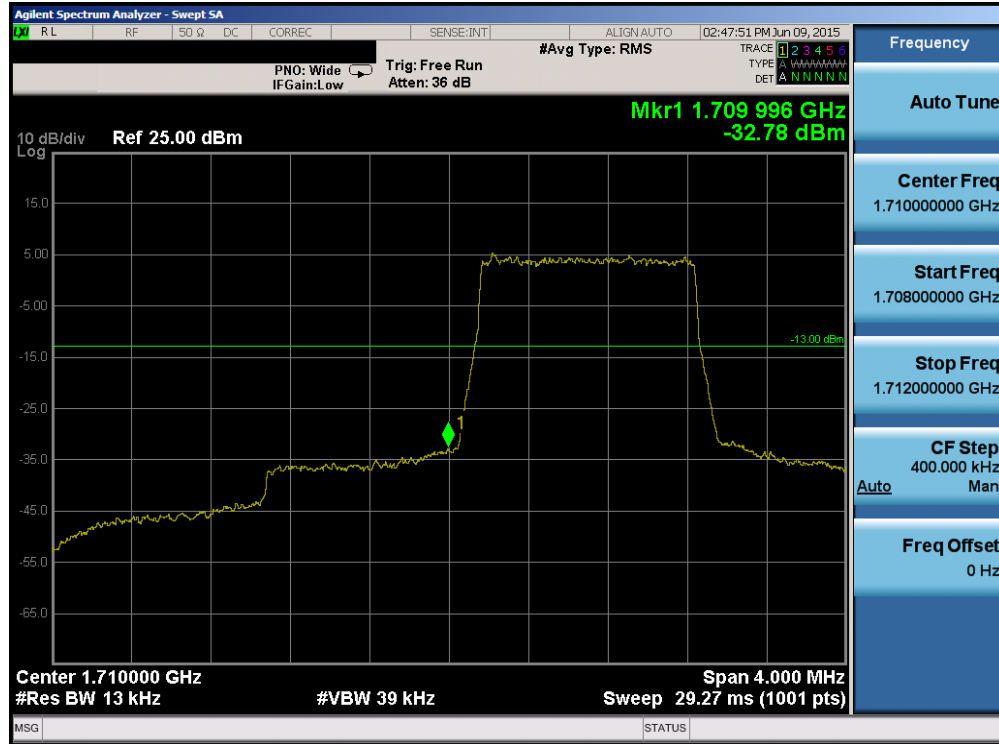
Plot 6-107. Lower Band Edge Plot (Band 4 – 1.4MHz QPSK – RB Size 6)
