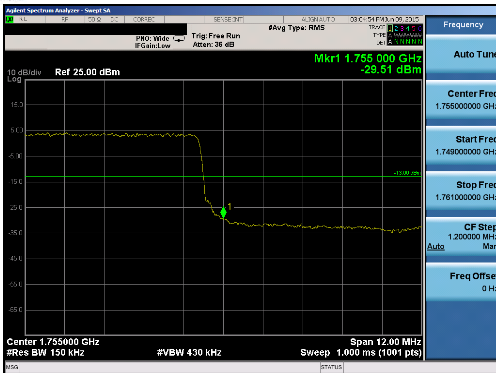
Plot 6-125. Upper Band Edge Plot (Band 4 – 15.0MHz QPSK – RB Size 75)
