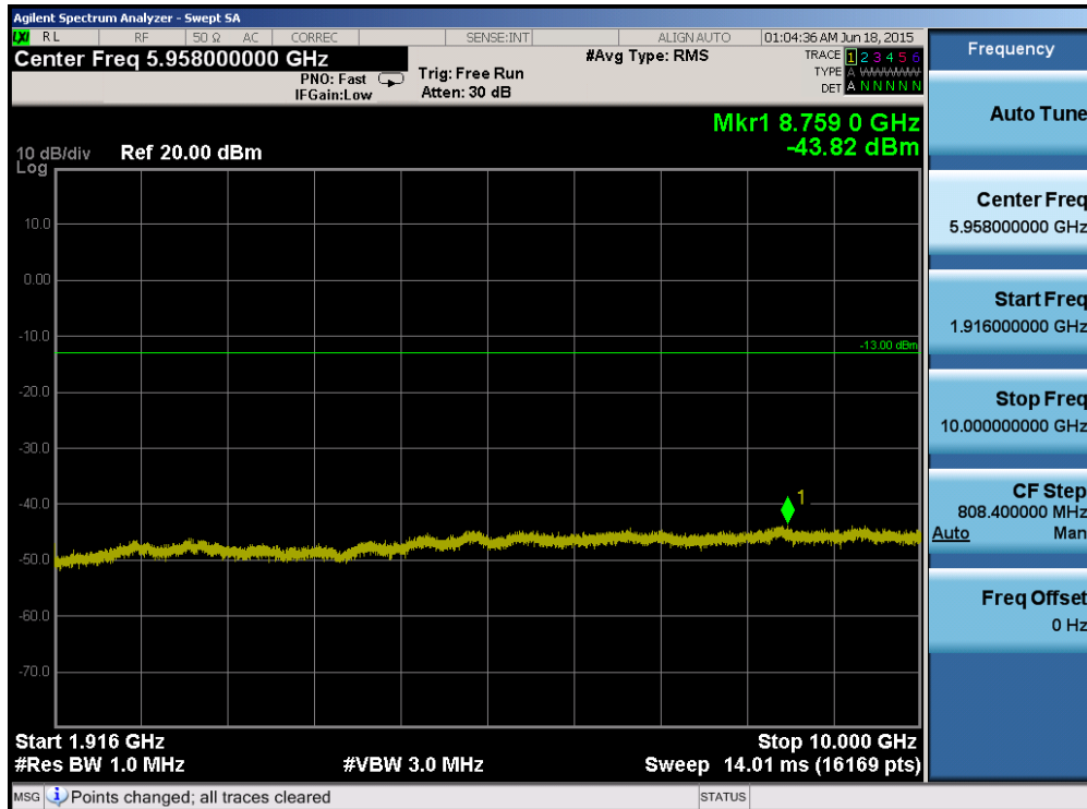
Plot 6-78. Conducted Spurious Plot (Band 25/2 – 20.0MHz QPSK – RB Size 1, RB Offset 0 – High Channel)
