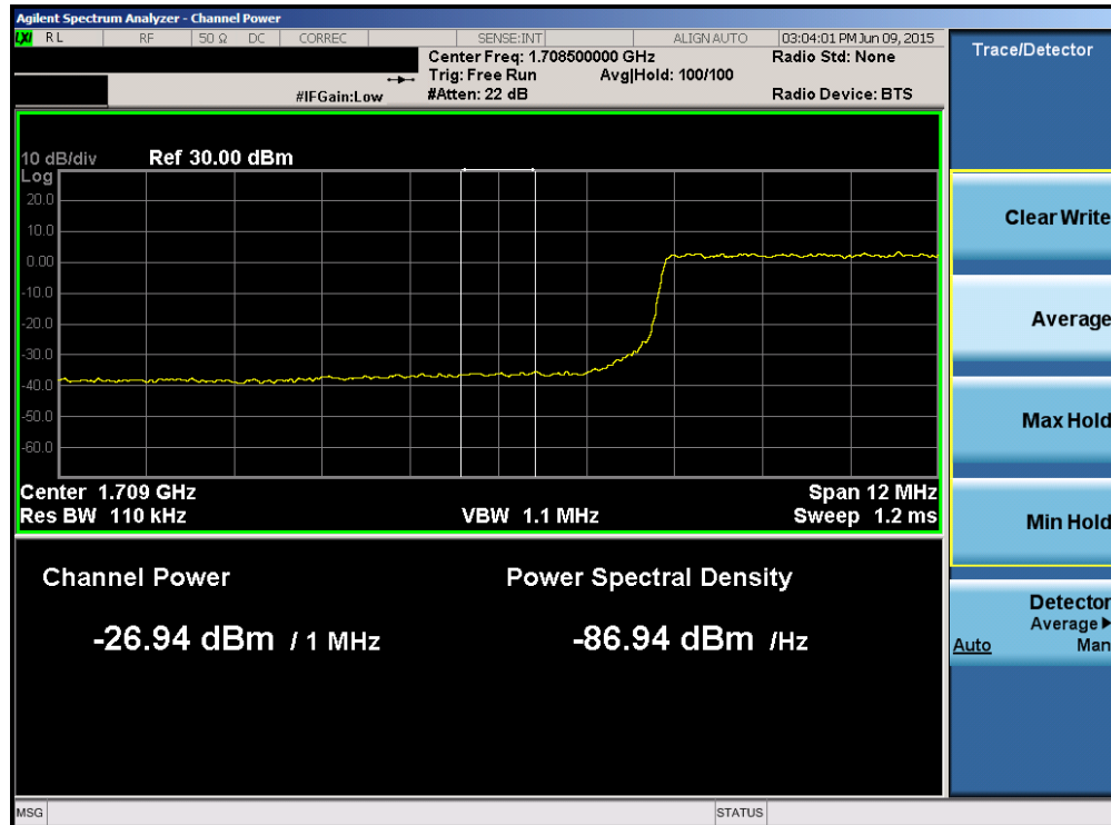
Plot 6-124. Lower Extended Band Edge Plot (Band 4 – 15.0MHz QPSK – RB Size 75)
