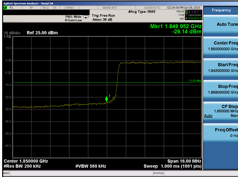
Plot 6-151. Lower Band Edge Plot (Band2/25 – 20.0MHz QPSK – RB Size 100)
