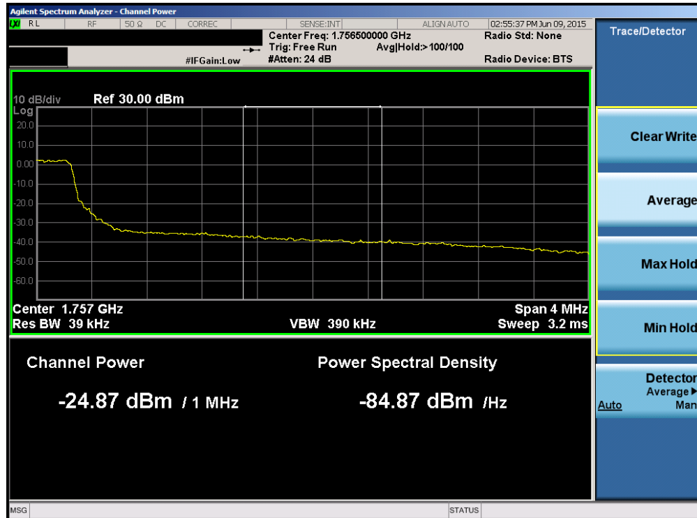
Plot 6-118. Upper Extended Band Edge Plot (Band 4 – 5.0MHz QPSK – RB Size 25)
