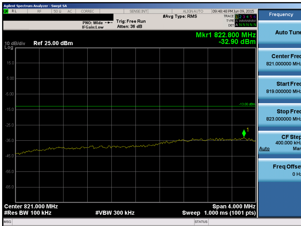
Plot 6-99. Lower Extended Band Edge Plot (Band 5 – 3.0MHz QPSK – RB Size 15)
