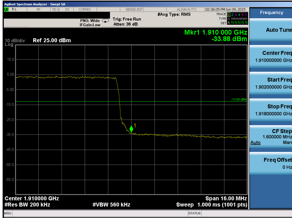
Plot 6-153. Upper Band Edge Plot (Band2/25 – 20.0MHz QPSK – RB Size 100)
