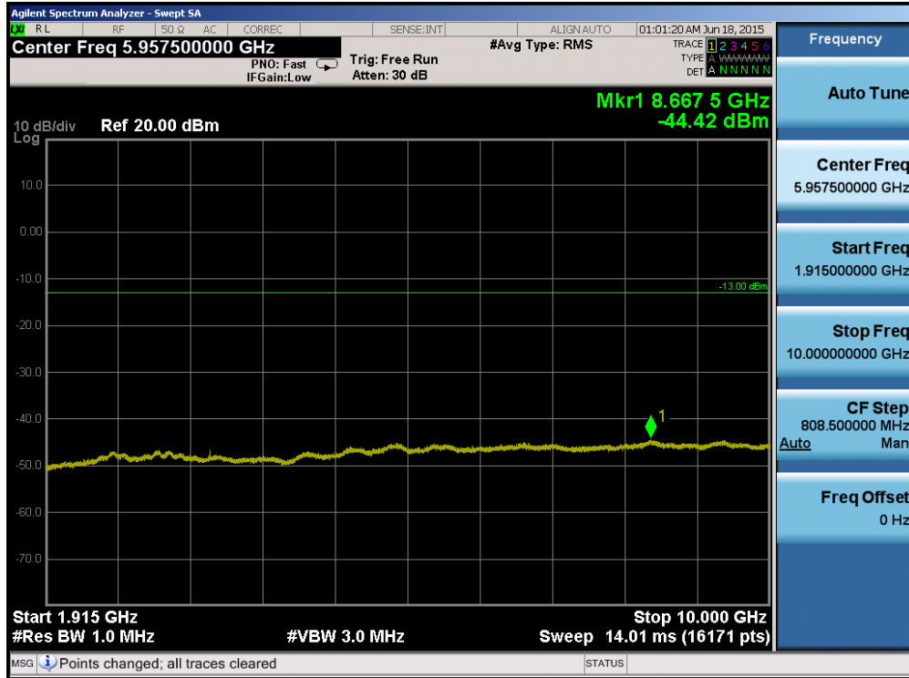
Plot 6-75. Conducted Spurious Plot (Band 25/2 – 20.0MHz QPSK – RB Size 1, RB Offset 0 – Mid Channel)
