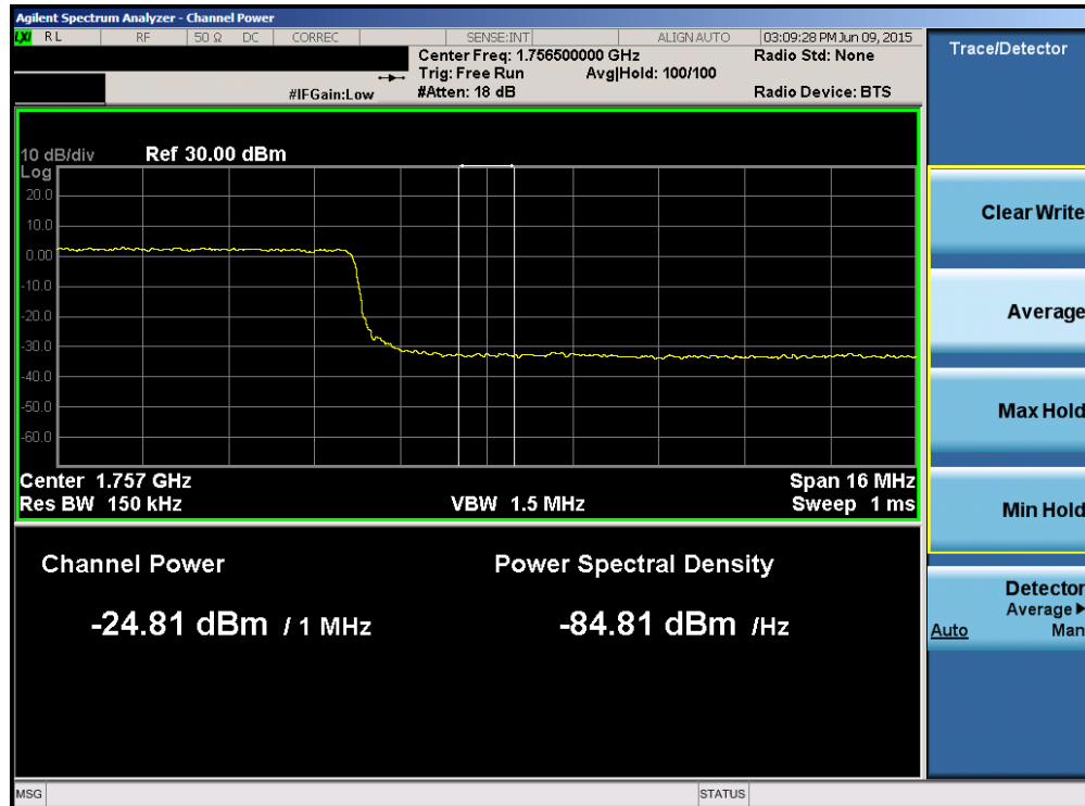
Plot 6-130. Upper Extended Band Edge Plot (Band 4 – 20.0MHz QPSK – RB Size 100)
