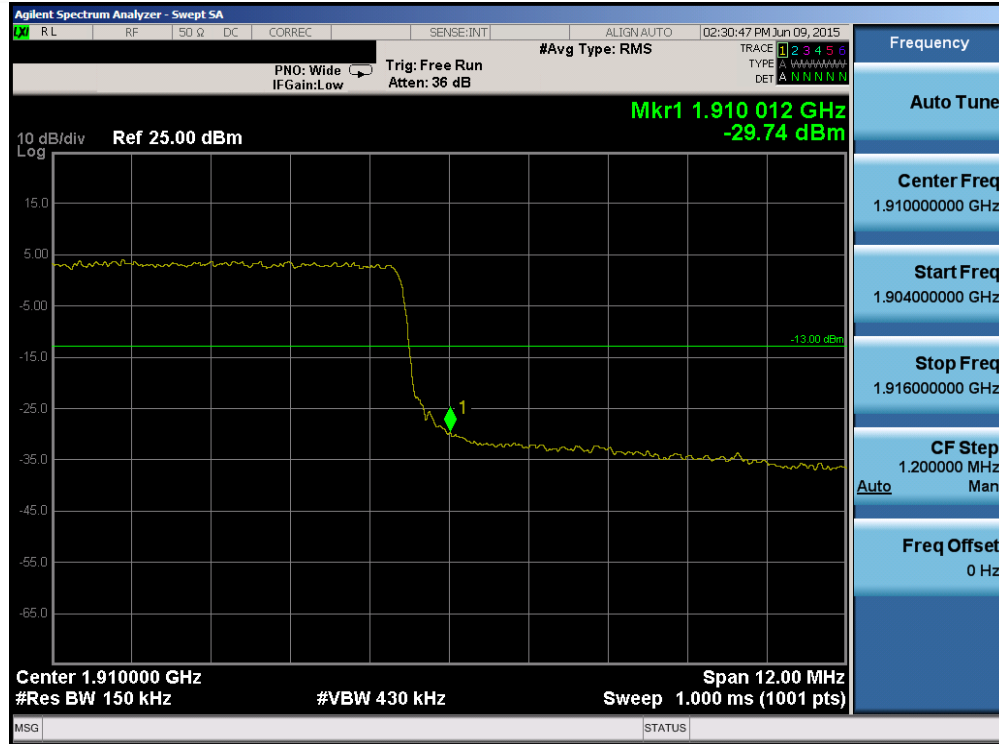
Plot 6-149. Upper Band Edge Plot (Band2/25 – 15.0MHz QPSK – RB Size 75)
