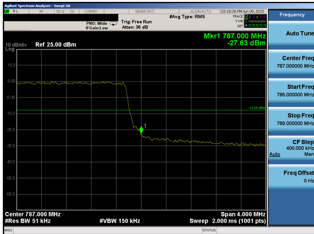
Plot 6-88. Upper Band Edge Plot (Band 13 – 5.0MHz QPSK – RB Size 25)
