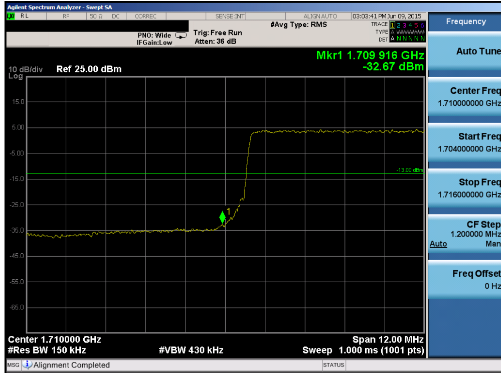
Plot 6-123. Lower Band Edge Plot (Band 4 – 15.0MHz QPSK – RB Size 75)
