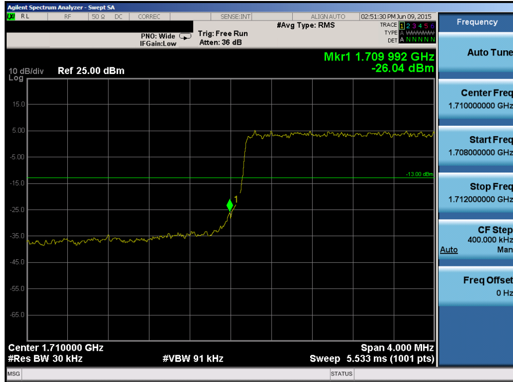
Plot 6-111. Lower Band Edge Plot (Band 4 – 3.0MHz QPSK – RB Size 15)
