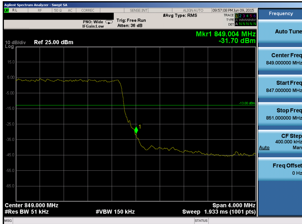
Plot 6-104. Upper Band Edge Plot (Band 5 – 5.0MHz QPSK – RB Size 25)
