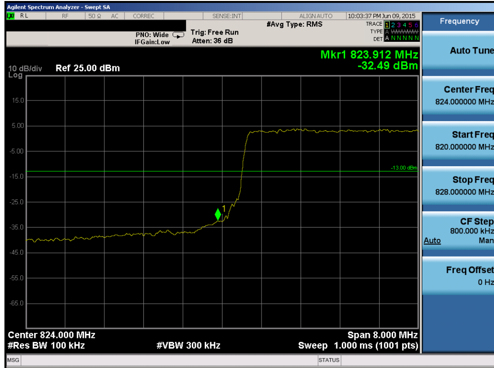
Plot 6-105. Lower Band Edge Plot (Band 5 - 10.0MHz QPSK - RB Size 50)
