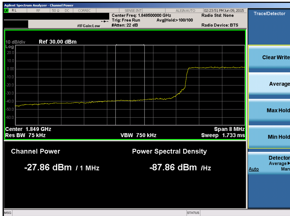
Plot 6-144. Lower Extended Band Edge Plot (Band2/25 – 10.0MHz QPSK – RB Size 50)
