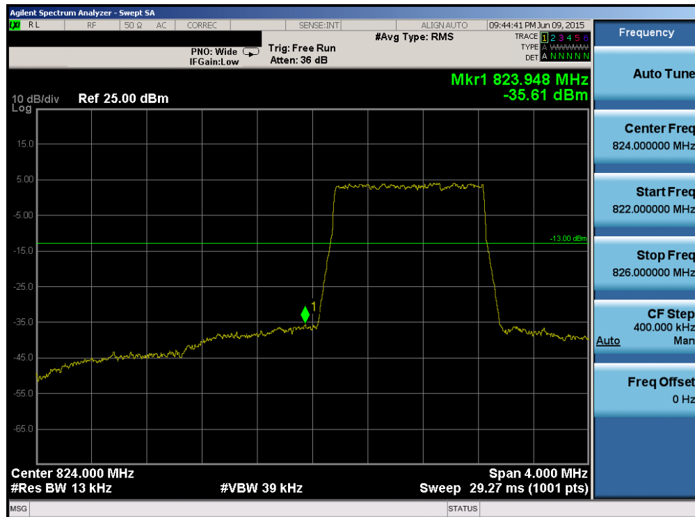
Plot 6-94. Lower Band Edge Plot (Band 5 – 1.4MHz QPSK – RB Size 6)
