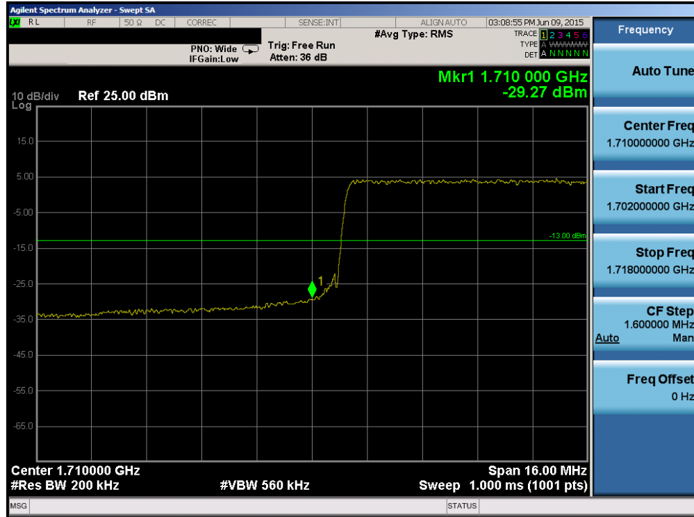
Plot 6-127. Lower Band Edge Plot (Band 4 – 20.0MHz QPSK – RB Size 100)
