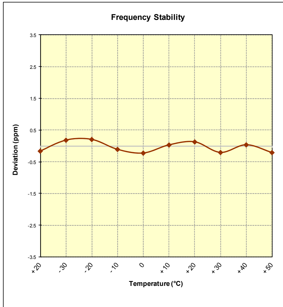
Figure 6-11. Frequency Stability Graph (Band 25/21)
