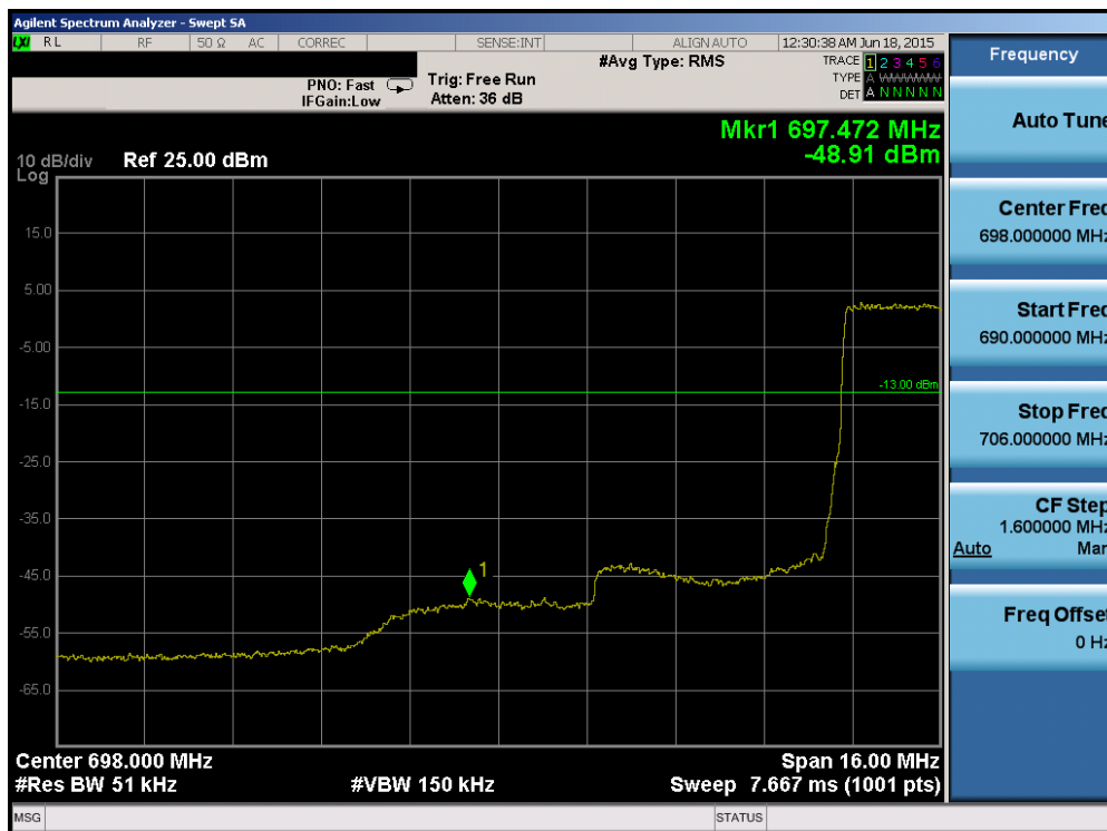
Plot 6-80. Lower Band Edge Plot (Band 12/17 – 5.0MHz QPSK – RB Size 25)
