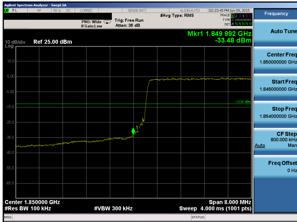
Plot 6-143. Lower Band Edge Plot (Band2/25 – 10.0MHz QPSK – RB Size 50)
