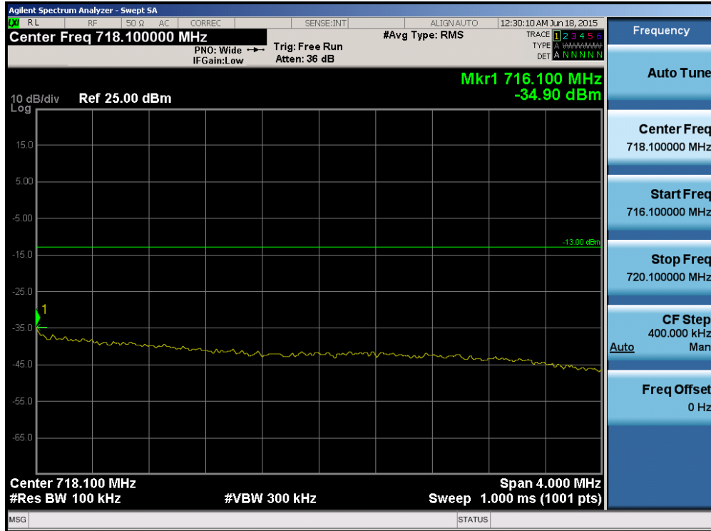
Plot 6-83. Upper Extended Band Edge Plot (Band 12/17 - 5.0MHz QPSK - RB Size 25)
