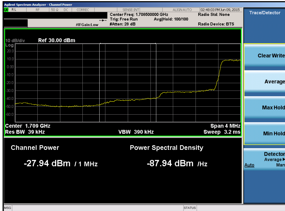
Plot 6-108. Lower Extended Band Edge Plot (Band 4 – 1.4MHz QPSK – RB Size 6)
