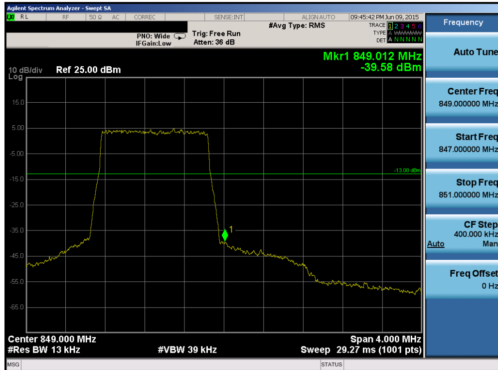
Plot 6-96. Upper Band Edge Plot (Band 5 – 1.4MHz QPSK – RB Size 6)
