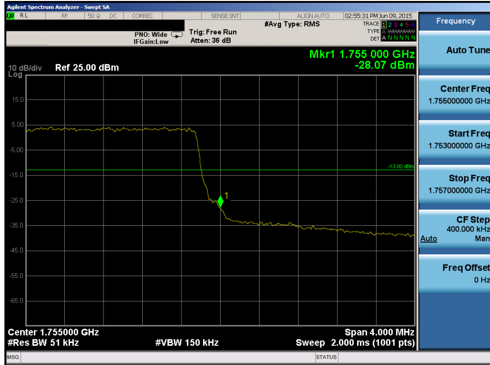
Plot 6-117. Upper Band Edge Plot (Band 4 – 5.0MHz QPSK – RB Size 25)
