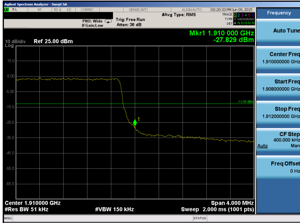
Plot 6-141. Upper Band Edge Plot (Band2/25 – 5.0MHz QPSK – RB Size 25)
