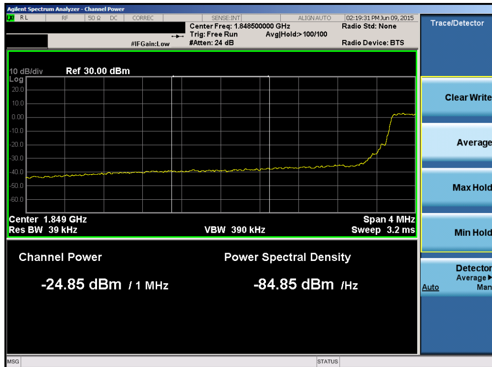
Plot 6-140. Lower Extended Band Edge Plot (Band2/25 – 5.0MHz QPSK – RB Size 25)
