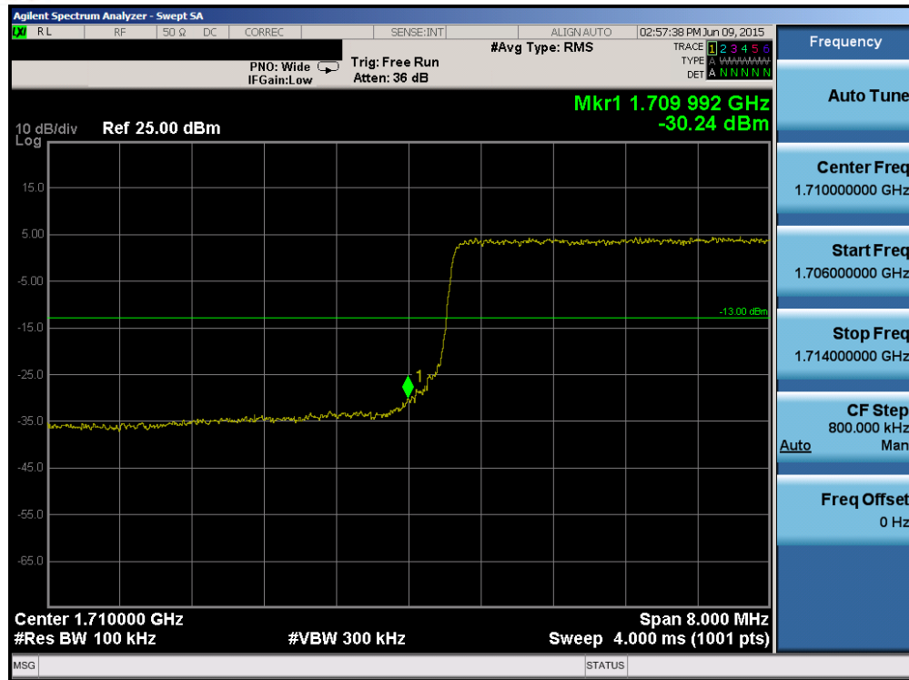
Plot 6-119. Lower Band Edge Plot (Band 4 – 10.0MHz QPSK – RB Size 50)
