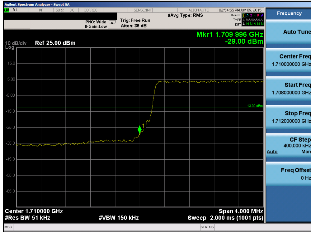
Plot 6-115. Lower Band Edge Plot (Band 4 – 5.0MHz QPSK – RB Size 25)
