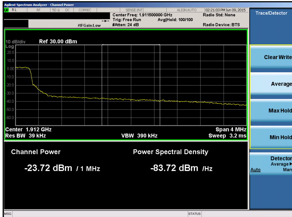
Plot 6-142. Upper Extended Band Edge Plot (Band2/25 – 5.0MHz QPSK – RB Size 25)
