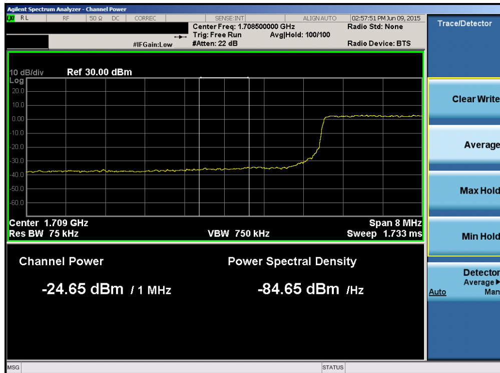
Plot 6-120. Lower Extended Band Edge Plot (Band 4 – 10.0MHz QPSK – RB Size 50)
