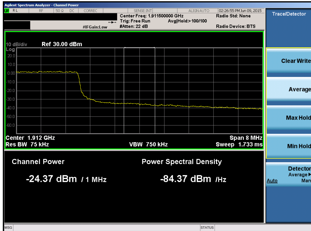
Plot 6-146. Upper Extended Band Edge Plot (Band2/25 – 10.0MHz QPSK – RB Size 50)
