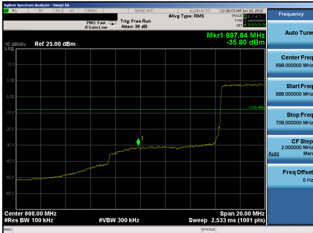
Plot 6-84. Lower Band Edge Plot (Band 12/17 - 10.0MHz QPSK - RB Size 50)
