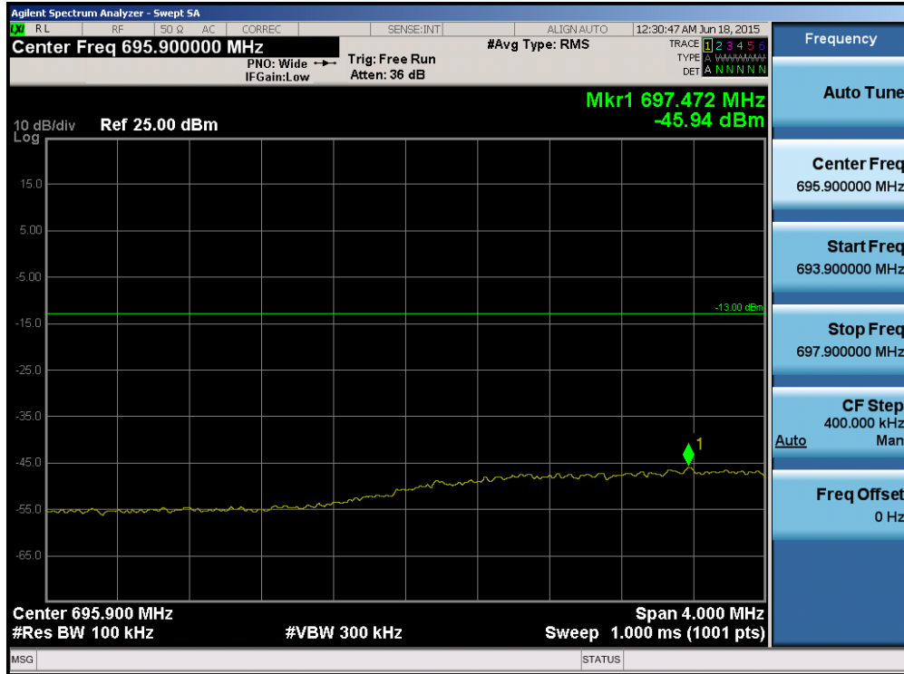
Plot 6-81. Lower Extended Band Edge Plot (Band 12/17 - 5.0MHz QPSK - RB Size 25)
