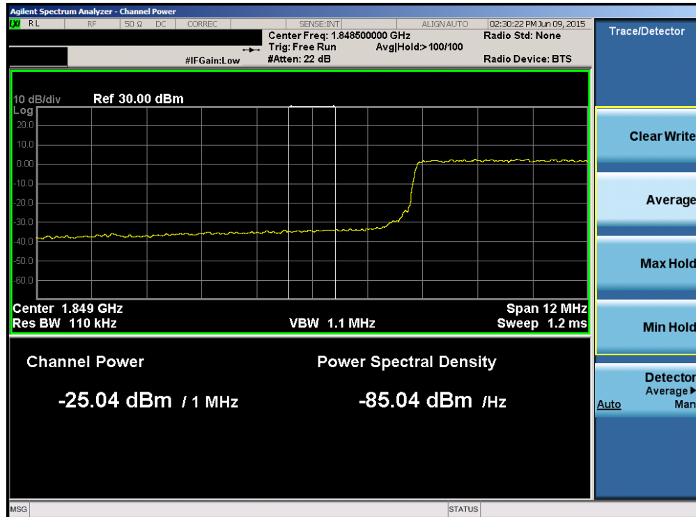
Plot 6-148. Lower Extended Band Edge Plot (Band2/25 – 15.0MHz QPSK – RB Size 75)
