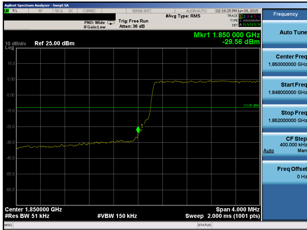
Plot 6-139. Lower Band Edge Plot (Band2/25 – 5.0MHz QPSK – RB Size 25)
