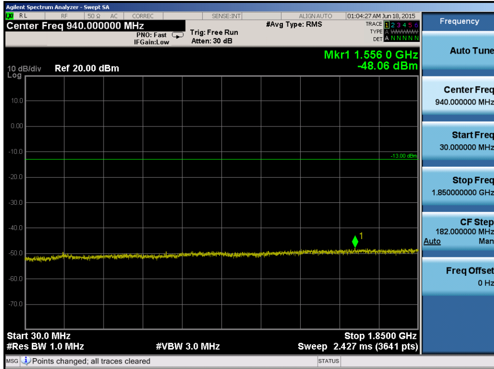
Plot 6-77. Conducted Spurious Plot (Band 25/2 – 20.0MHz QPSK – RB Size 1, RB Offset 0 – High Channel)
