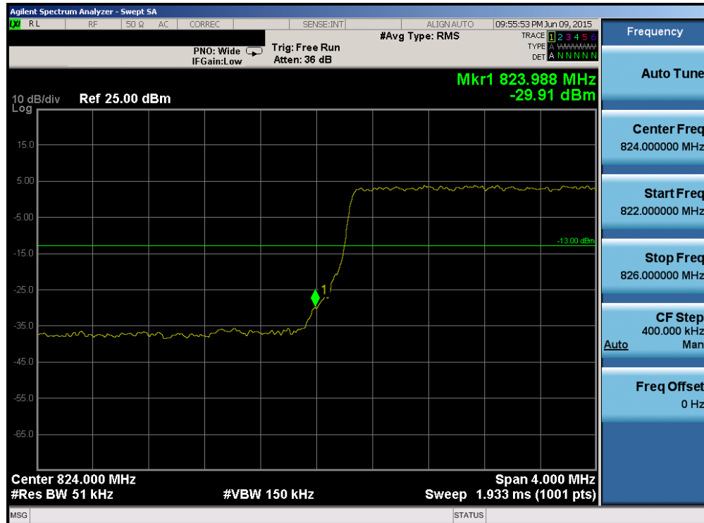
Plot 6-102. Lower Band Edge Plot (Band 5 – 5.0MHz QPSK – RB Size 25)
