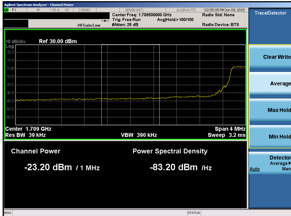
Plot 6-116. Lower Extended Band Edge Plot (Band 4 – 5.0MHz QPSK – RB Size 25)
