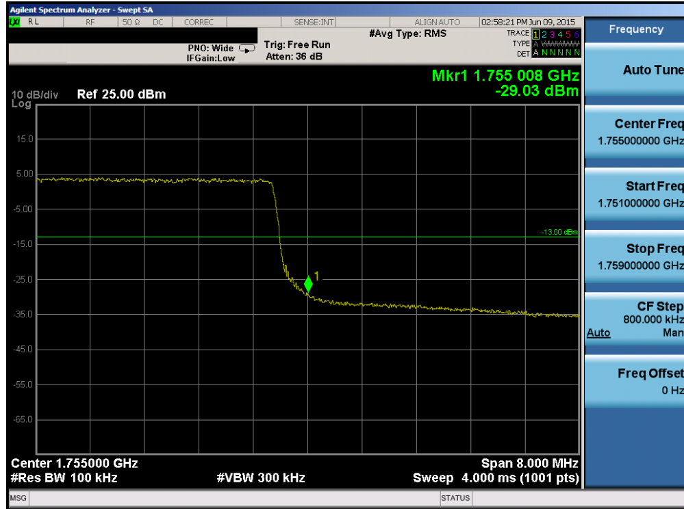
Plot 6-121. Upper Band Edge Plot (Band 4 – 10.0MHz QPSK – RB Size 50)
