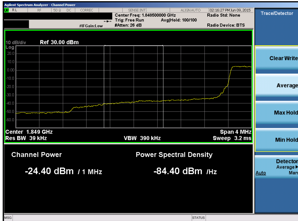
Plot 6-136. Lower Extended Band Edge Plot (Band2/25 – 3.0MHz QPSK – RB Size 15)
