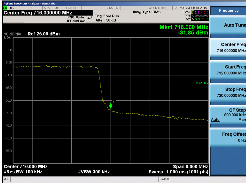
Plot 6-85. Upper Band Edge Plot (Band 12/17 – 10.0MHz QPSK – RB Size 50)
