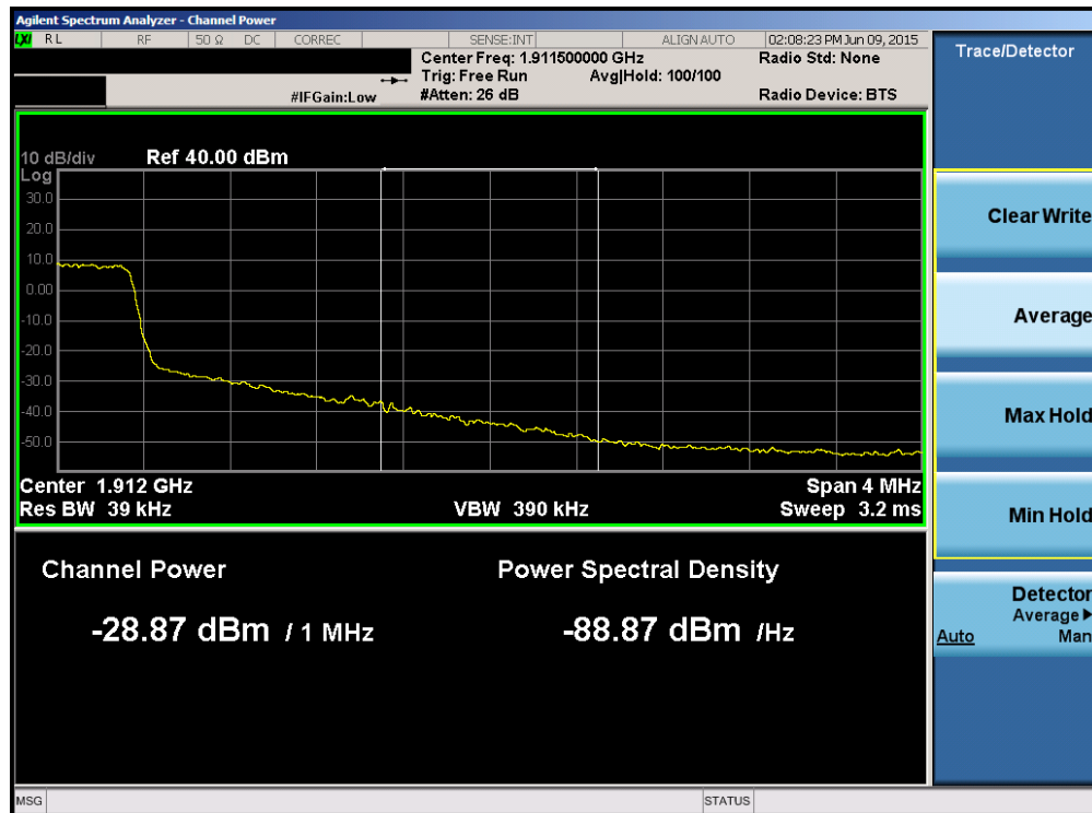
Plot 6-134. Upper Extended Band Edge Plot (Band2/25 – 1.4MHz QPSK – RB Size 6)
