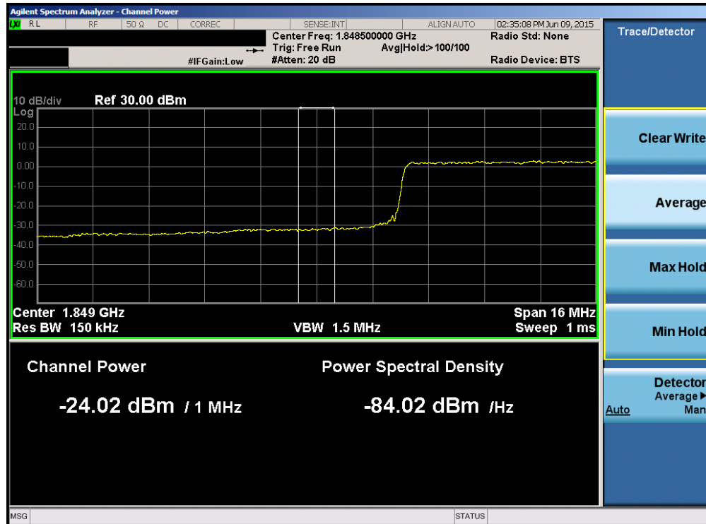
Plot 6-152. Lower Extended Band Edge Plot (Band2/25 – 20.0MHz QPSK – RB Size 100)
