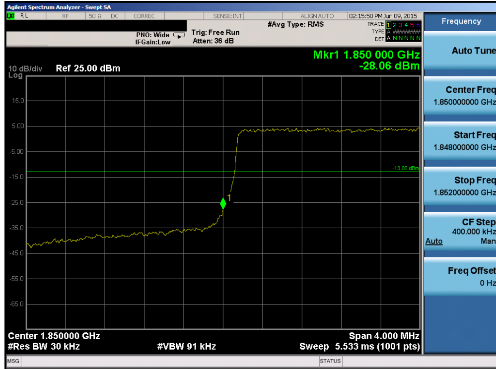
Plot 6-135. Lower Band Edge Plot (Band2/25 – 3.0MHz QPSK – RB Size 15)
