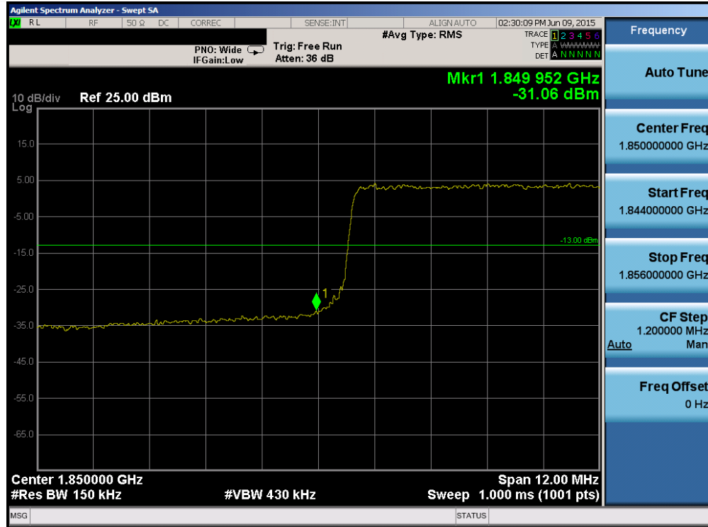
Plot 6-147. Lower Band Edge Plot (Band2/25 – 15.0MHz QPSK – RB Size 75)
