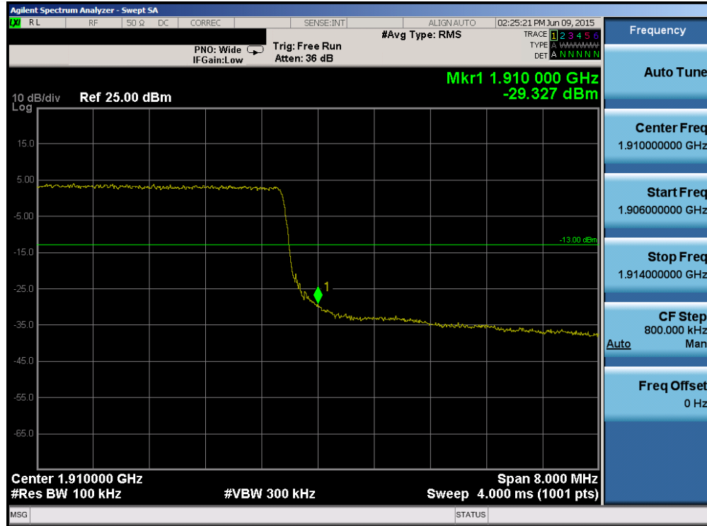
Plot 6-145. Upper Band Edge Plot (Band2/25 – 10.0MHz QPSK – RB Size 50)
