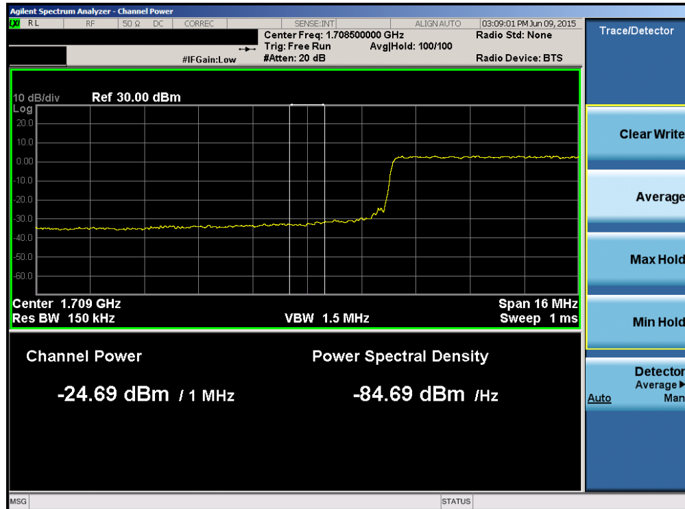
Plot 6-128. Lower Extended Band Edge Plot (Band 4 – 20.0MHz QPSK – RB Size 100)
