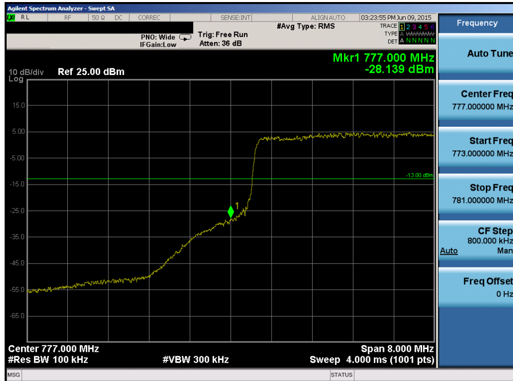
Plot 6-90. Lower Band Edge Plot (Band 13 – 10.0MHz QPSK – RB Size 50)
