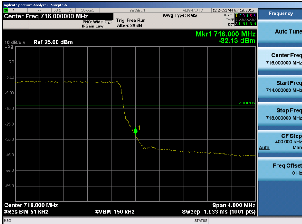
Plot 6-82. Upper Band Edge Plot (Band 12/17 - 5.0MHz QPSK - RB Size 25)
