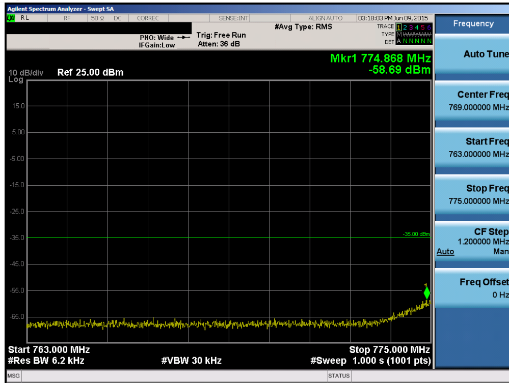
Plot 6-87. Lower Emission Mask Edge Plot (Band 13 – 5.0MHz QPSK – RB Size 25)
