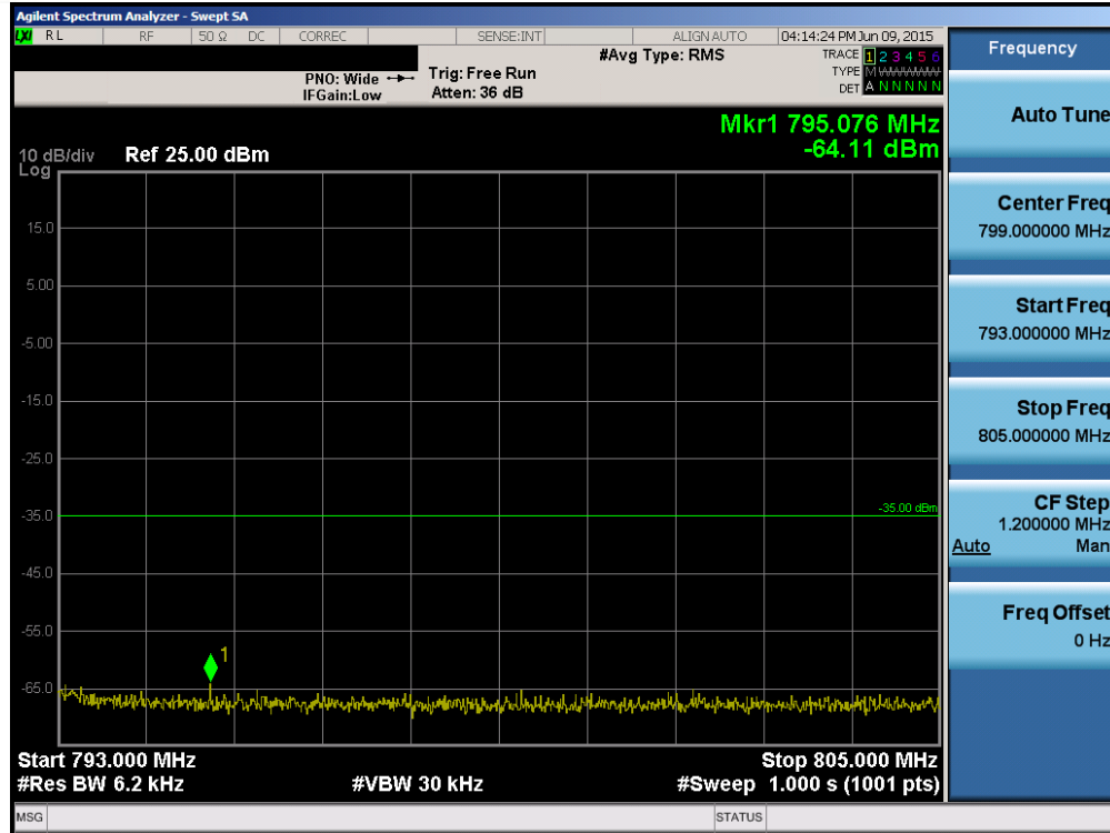
Plot 6-93. Upper Emission Mask Edge Plot (Band 13 – 10.0MHz QPSK – RB Size 50)
