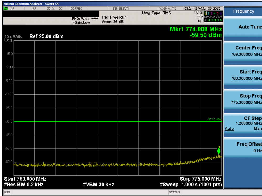
Plot 6-91. Lower Emission Mask Edge Plot (Band 13 – 10.0MHz QPSK – RB Size 50)
