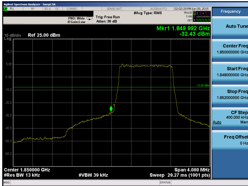
Plot 6-131. Lower Band Edge Plot (Band2/25 – 1.4MHz QPSK – RB Size 6)
