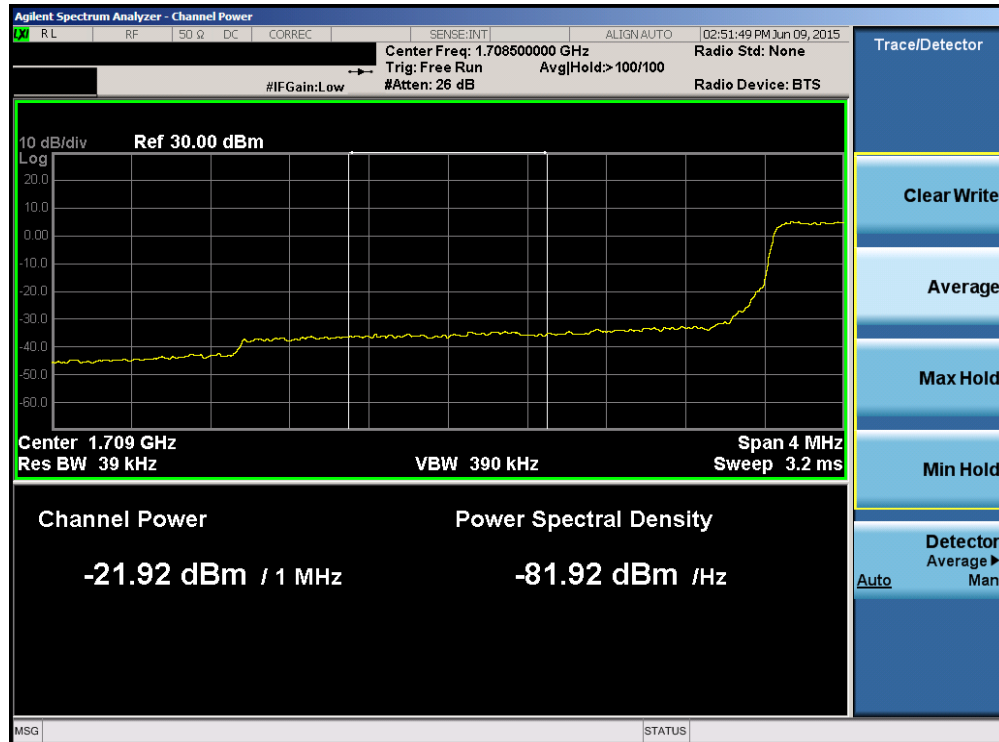
Plot 6-112. Lower Extended Band Edge Plot (Band 4 – 3.0MHz QPSK – RB Size 15)
