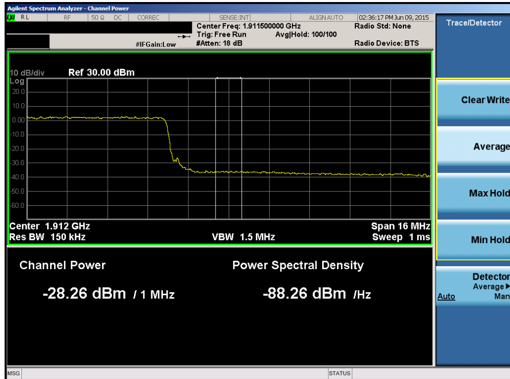
Plot 6-154. Upper Extended Band Edge Plot (Band2/25 – 20.0MHz QPSK – RB Size 100)
