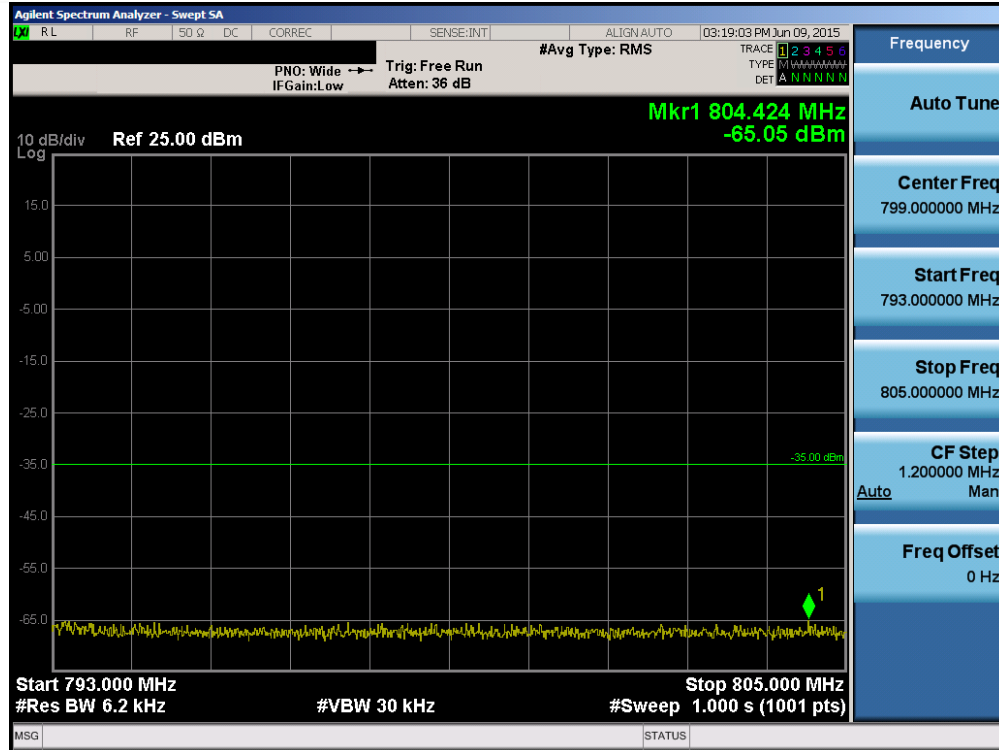
Plot 6-89. Upper Emission Mask Edge Plot (Band 13 – 5.0MHz QPSK – RB Size 25)
