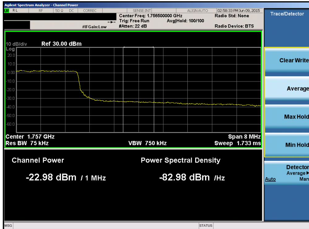
Plot 6-122. Upper Extended Band Edge Plot (Band 4 – 10.0MHz QPSK – RB Size 50)
