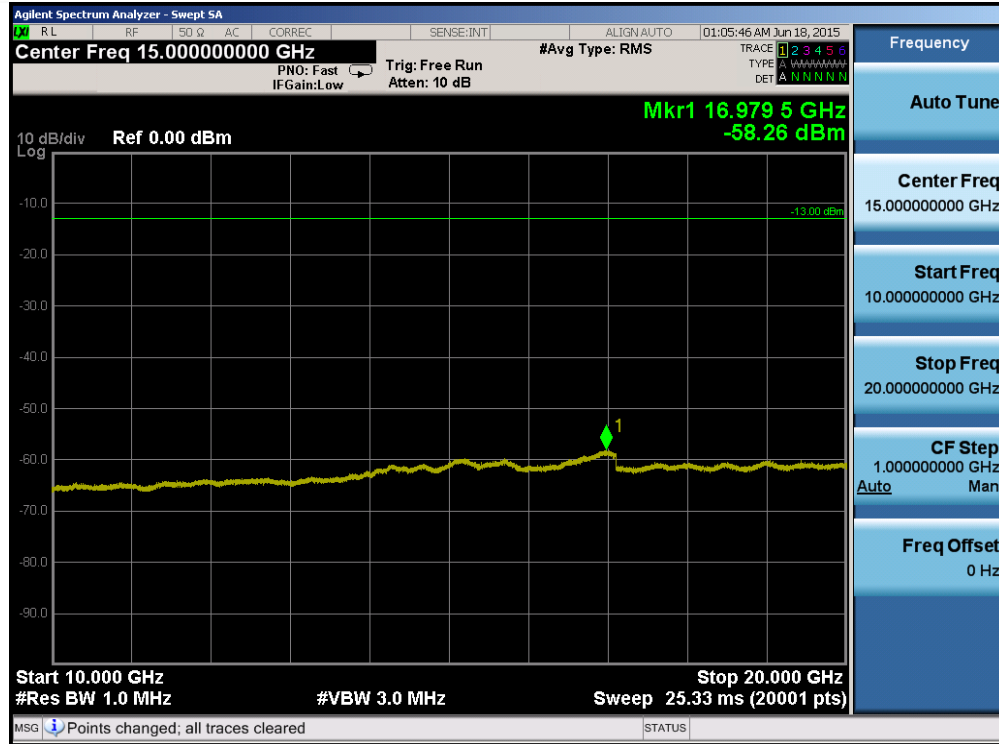
Plot 6-79. Conducted Spurious Plot (Band 25/2 – 20.0MHz QPSK – RB Size 1, RB Offset 0 – High Channel)
