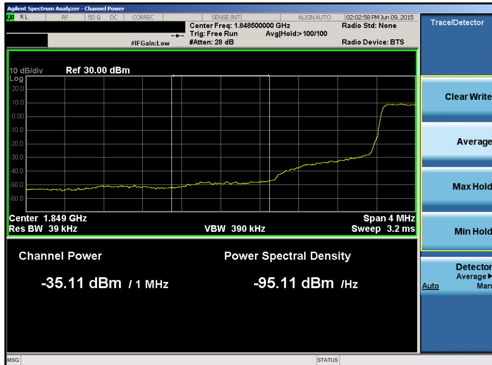
Plot 6-132. Lower Extended Band Edge Plot (Band2/25 – 1.4MHz QPSK – RB Size 6)
