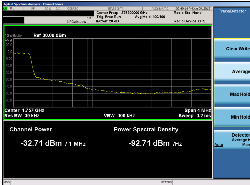
Plot 6-110. Upper Extended Band Edge Plot (Band 4 – 1.4MHz QPSK – RB Size 6)
