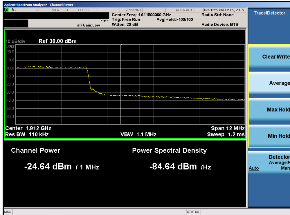
Plot 6-150. Upper Extended Band Edge Plot (Band2/25 – 15.0MHz QPSK – RB Size 75)
