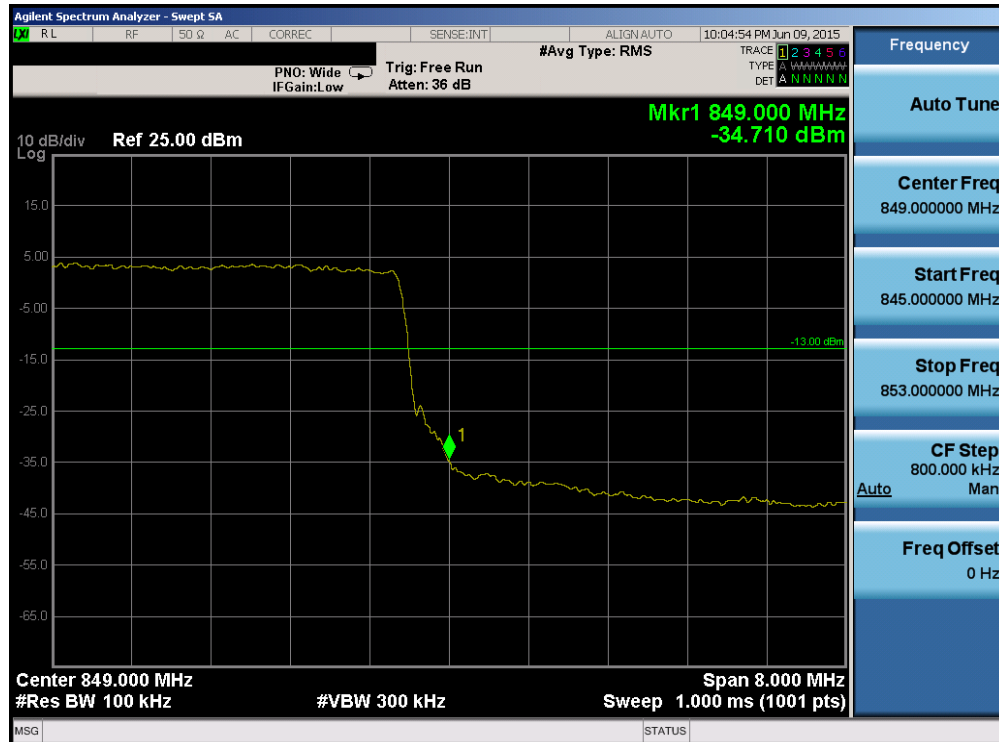
Plot 6-106. Upper Band Edge Plot (Band 5 - 10.0MHz QPSK - RB Size 50)
