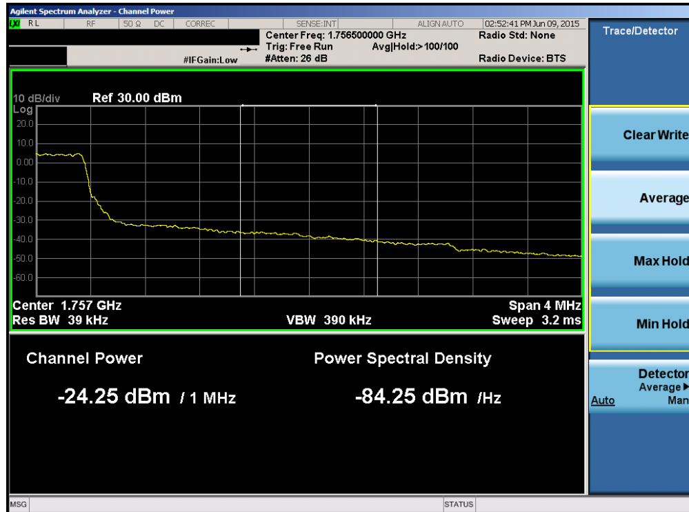
Plot 6-114. Upper Extended Band Edge Plot (Band 4 – 3.0MHz QPSK – RB Size 15)
