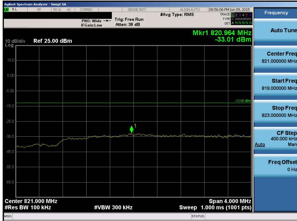
Plot 6-103. Lower Extended Band Edge Plot (Band 5 – 5.0MHz QPSK – RB Size 25)
