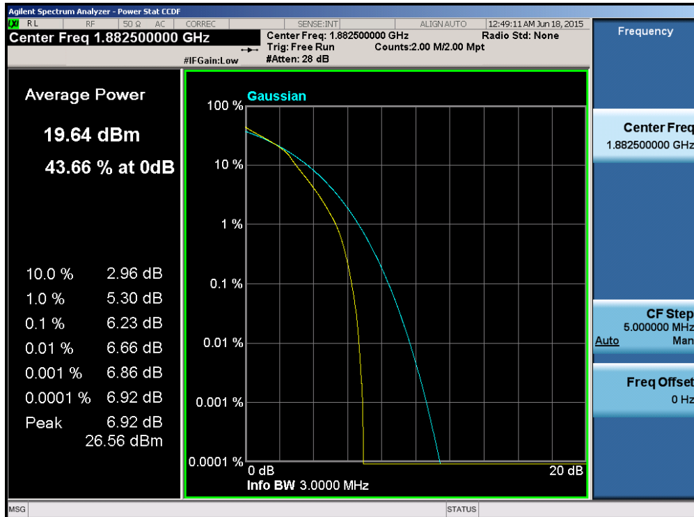
Plot 6-158. PAR Plot (Band 25/2 – 3.0MHz 16-QAM – RB Size 15)
