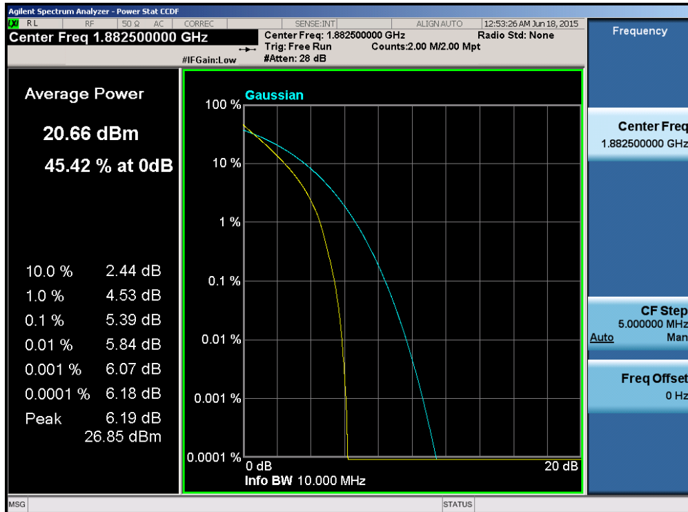
Plot 6-162. PAR Plot (Band 25/2 – 10.0MHz 16-QAM – RB Size 50)
