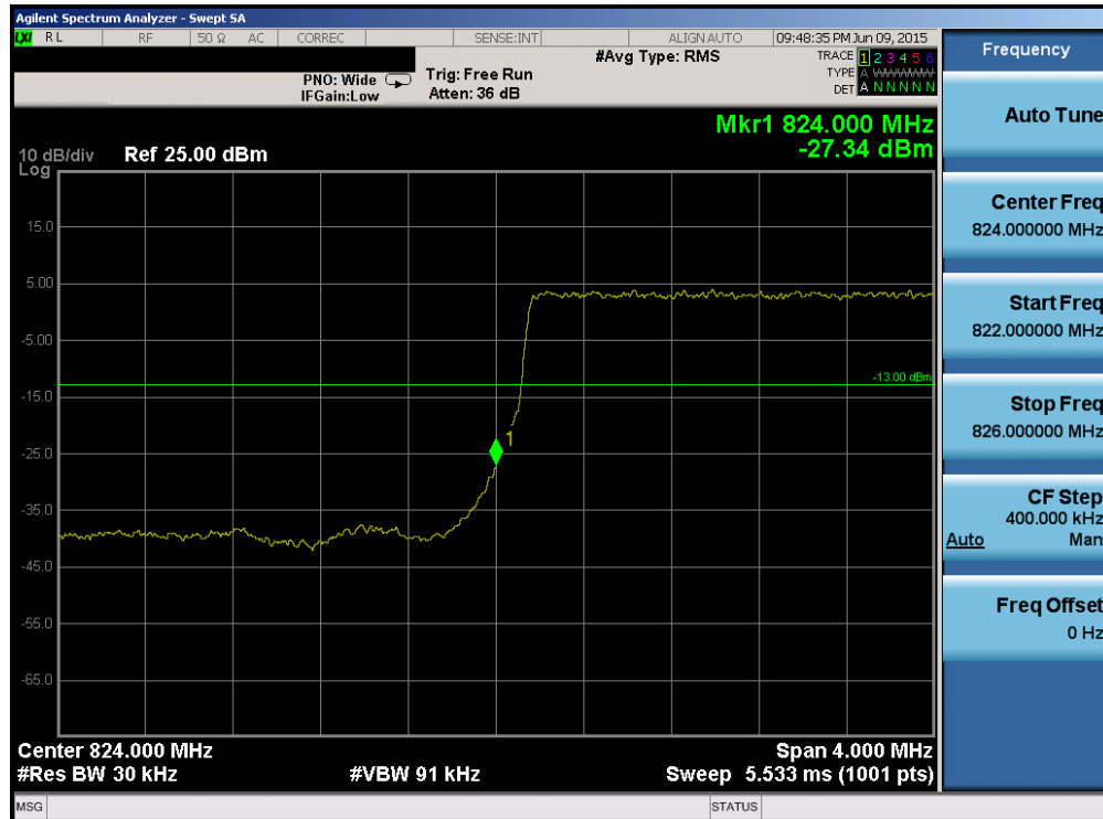
Plot 6-98. Lower Band Edge Plot (Band 5 – 3.0MHz QPSK – RB Size 15)
