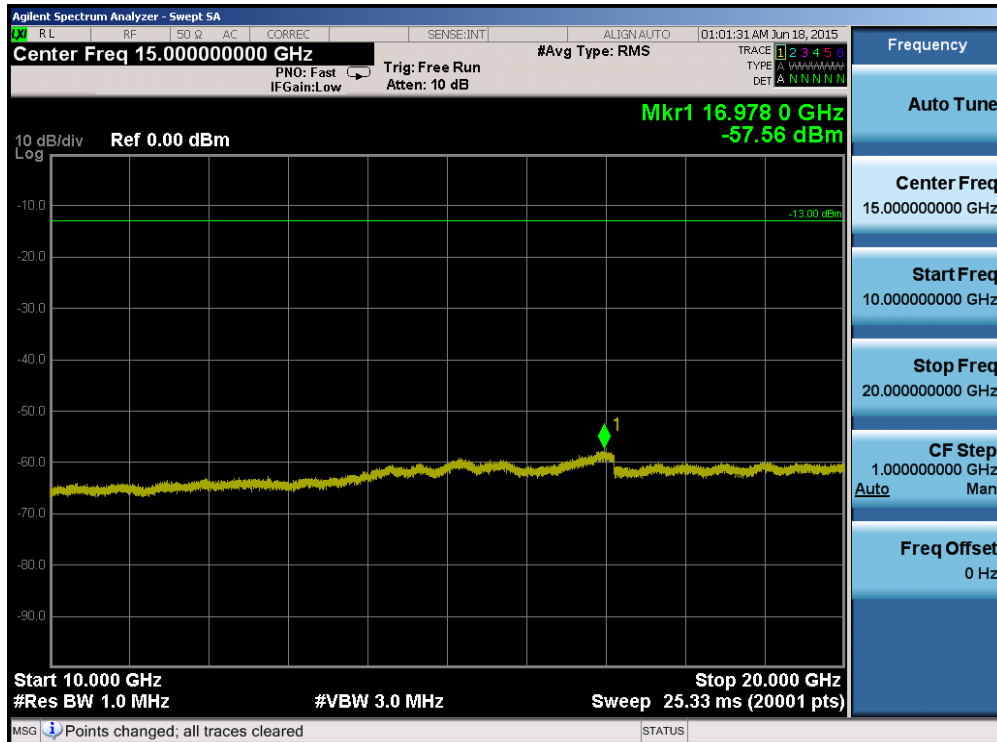
Plot 6-76. Conducted Spurious Plot (Band 25/2 – 20.0MHz QPSK – RB Size 1, RB Offset 0 – Mid Channel)
