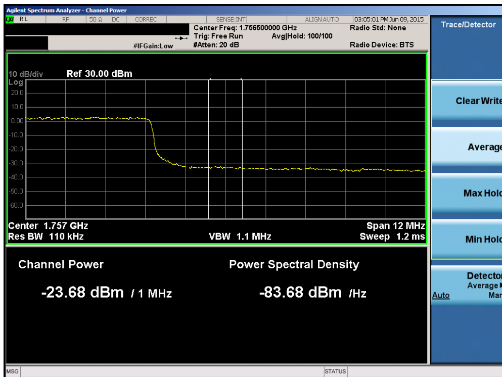
Plot 6-126. Upper Extended Band Edge Plot (Band 4 – 15.0MHz QPSK – RB Size 75)
