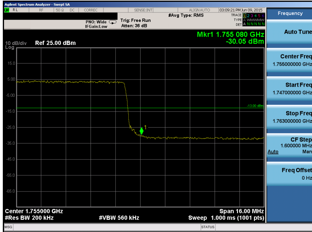
Plot 6-129. Upper Band Edge Plot (Band 4 – 20.0MHz QPSK – RB Size 100)
