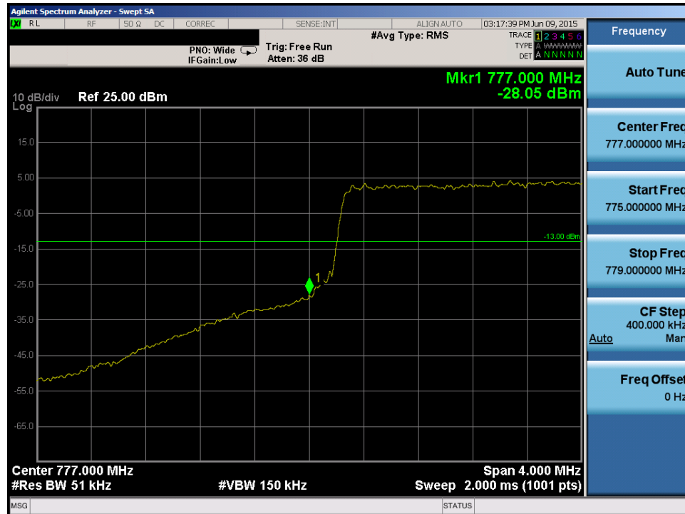
Plot 6-86. Lower Band Edge Plot (Band 13 – 5.0MHz QPSK – RB Size 25)
